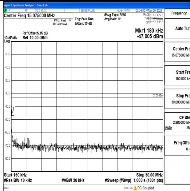
Band2_10MHz_16QAM_18650_1RB#0_0.15~30_0.15~30
