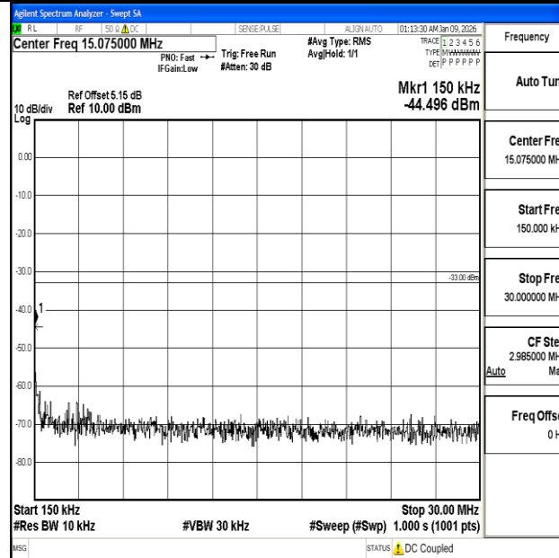
Band2_10MHz_QPSK_18650_1RB#0_0.15~30_0.15~30
