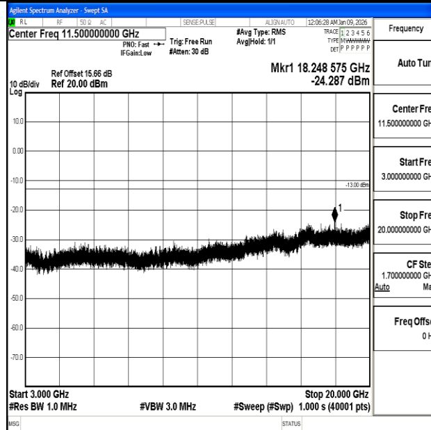
Band2_5MHz_16QAM_19175_1RB#0_3000~20000_3000~20000
