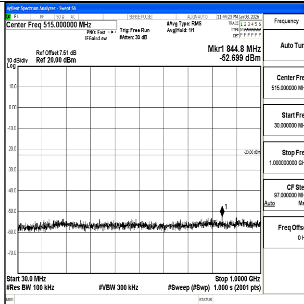
Band2_3MHz_16QAM_19185_1RB#0_30~1000_30~1000
