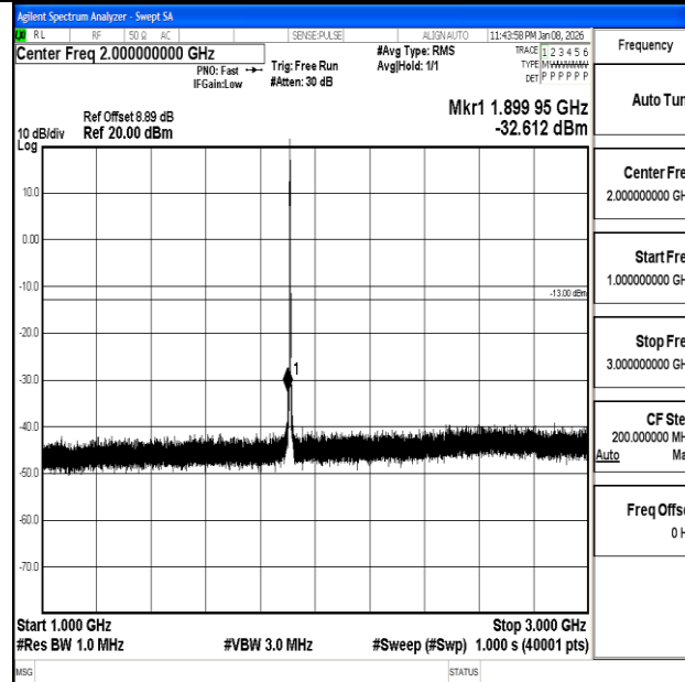
Band2_3MHz_QPSK_19185_1RB#0_1000~3000_1000~3000
