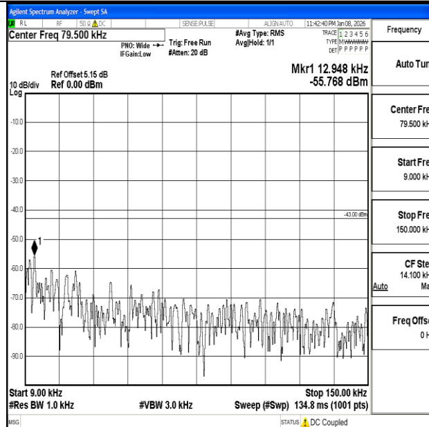
Band2_3MHz_QPSK_18900_1RB#0_0.009~0.15_0.009~0.15
