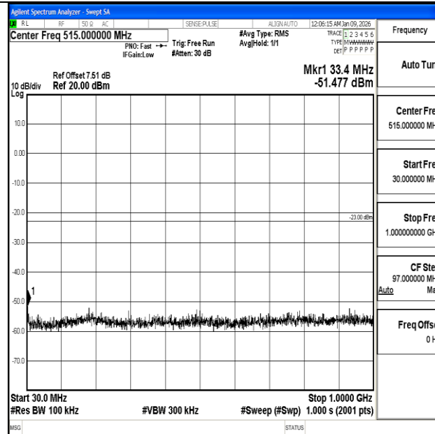
Band2_5MHz_16QAM_19175_1RB#0_30~1000_30~1000
