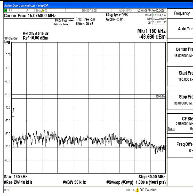
Band2_5MHz_16QAM_18625_1RB#0_0.15~30_0.15~30
