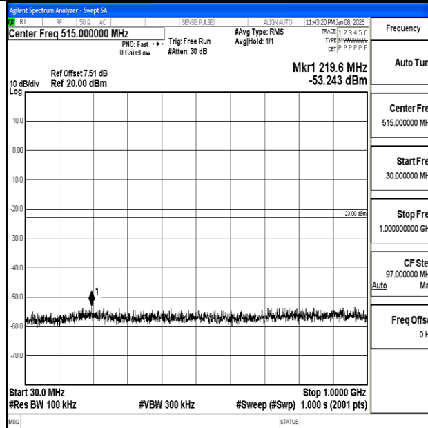
Band2_3MHz_16QAM_18900_1RB#0_30~1000_30~1000
