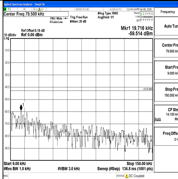
Band2_3MHz_16QAM_19185_1RB#0_0.009~0.15_0.009~0.15
