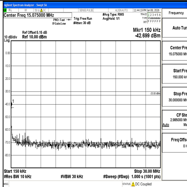
Band2_3MHz_16QAM_19185_1RB#0_0.15~30_0.15~30
