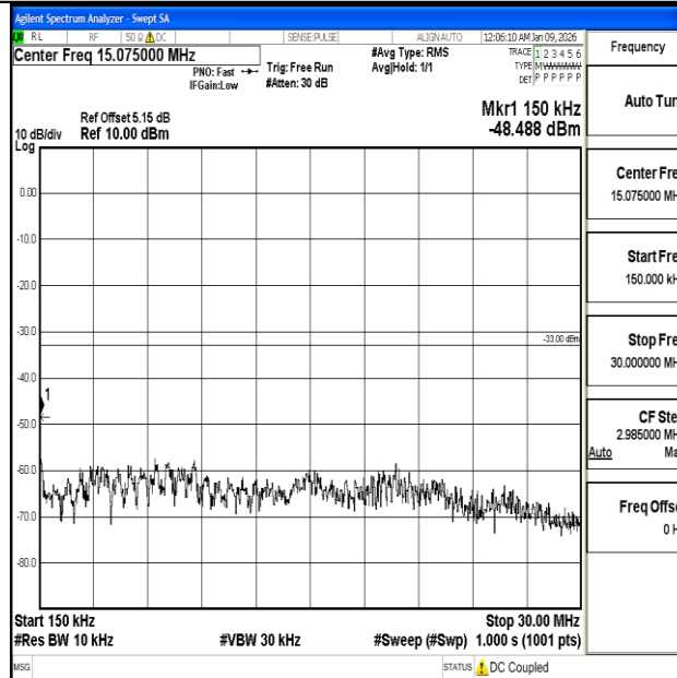
Band2_5MHz_16QAM_19175_1RB#0_0.15~30_0.15~30
