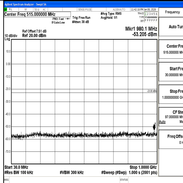
Band2_3MHz_16QAM_18615_1RB#0_30~1000_30~1000
