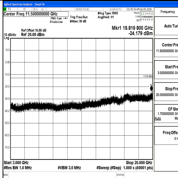
Band2_15MHz_16QAM_19125_1RB#0_3000~20000_3000~20000
