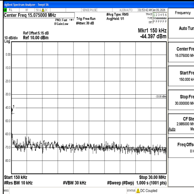
Band2_20MHz_QPSK_19100_1RB#0_0.15~30_0.15~30
