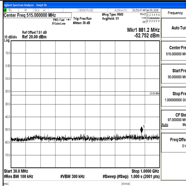
Band2_20MHz_QPSK_19100_1RB#0_30~1000_30~1000
