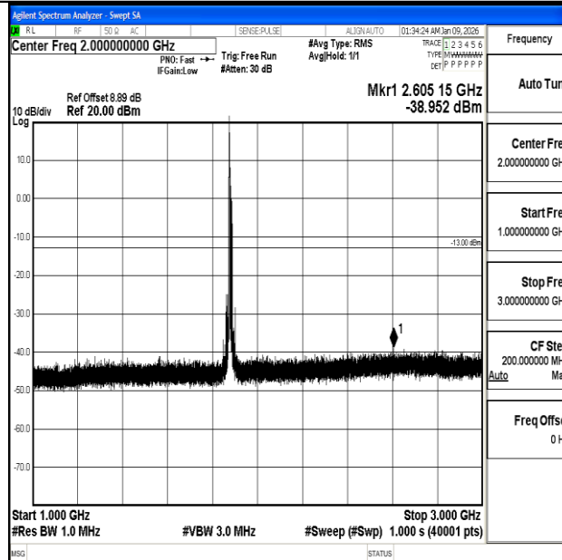
Band2_15MHz_16QAM_18900_1RB#0_1000~3000_1000~3000
