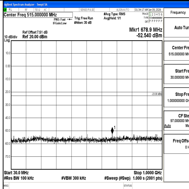
Band2_15MHz_16QAM_18900_1RB#0_30~1000_30~1000
