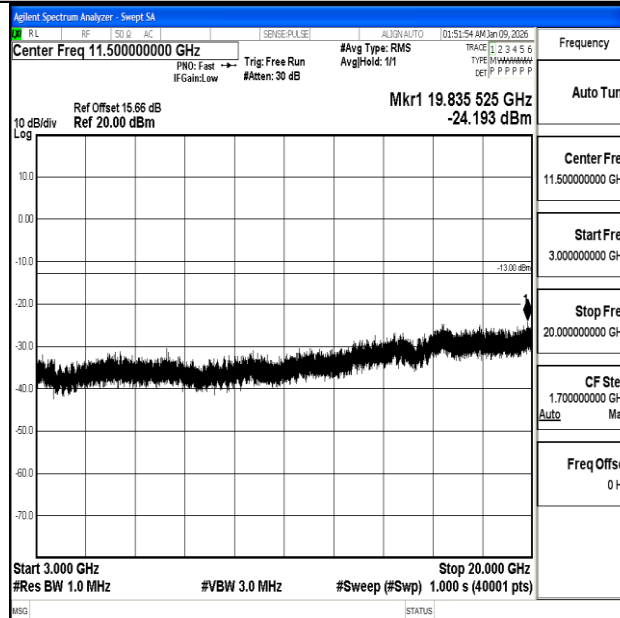
Band2_20MHz_QPSK_18700_1RB#0_3000~20000_3000~20000
