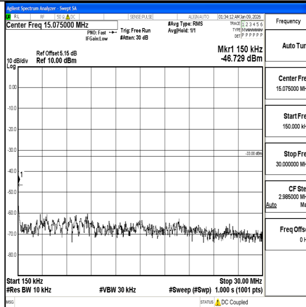
Band2_15MHz_16QAM_18900_1RB#0_0.15~30_0.15~30
