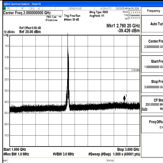
Band2_20MHz_QPSK_19100_1RB#0_1000~3000_1000~3000
