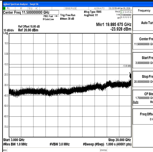
Band2_15MHz_QPSK_18900_1RB#0_3000~20000_3000~20000
