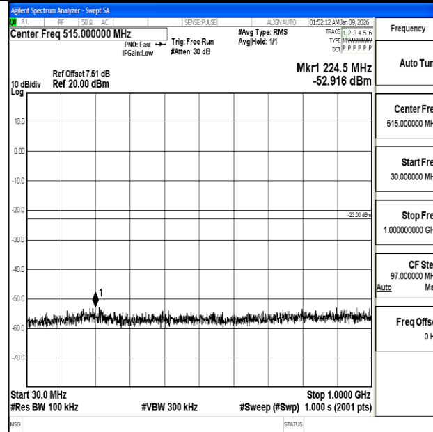
Band2_20MHz_16QAM_18700_1RB#0_30~1000_30~1000
