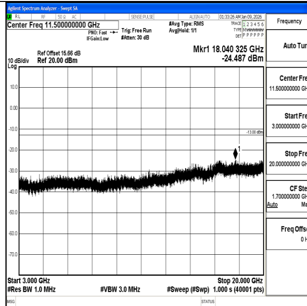
Band2_15MHz_16QAM_18675_1RB#0_3000~20000_3000~20000
