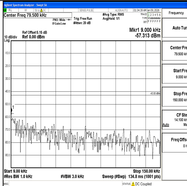
Band2_15MHz_QPSK_19125_1RB#0_0.009~0.15_0.009~0.15
