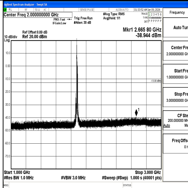
Band2_15MHz_QPSK_18900_1RB#0_1000~3000_1000~3000
