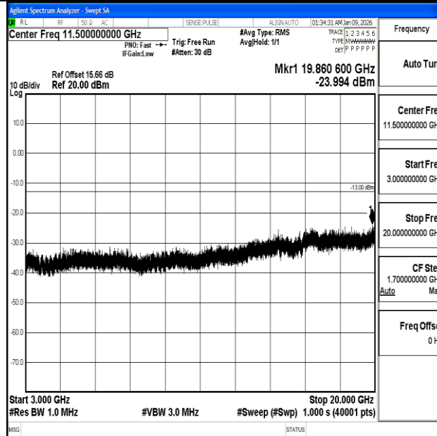
Band2_15MHz_16QAM_18900_1RB#0_3000~20000_3000~20000
