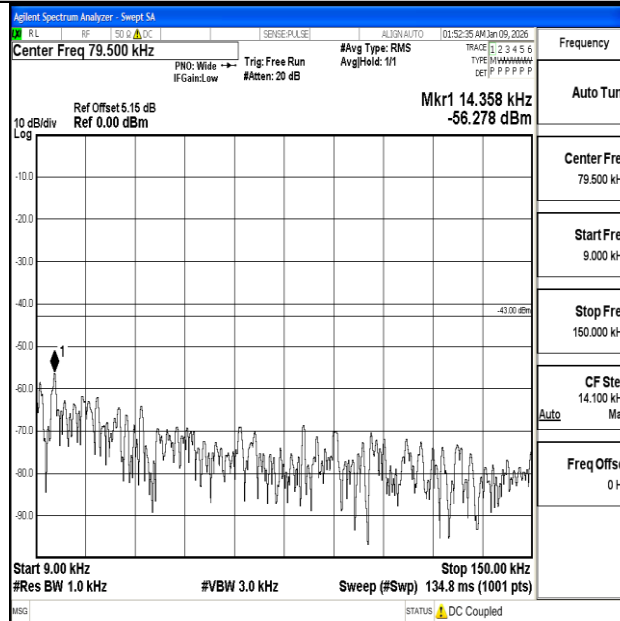
Band2_20MHz_QPSK_18900_1RB#0_0.009~0.15_0.009~0.15
