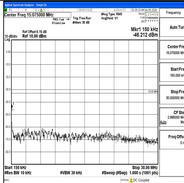
Band2_15MHz_16QAM_19125_1RB#0_0.15~30_0.15~30
