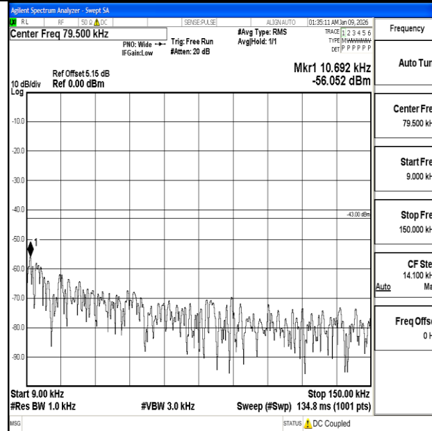
Band2_15MHz_16QAM_19125_1RB#0_0.009~0.15_0.009~0.15
