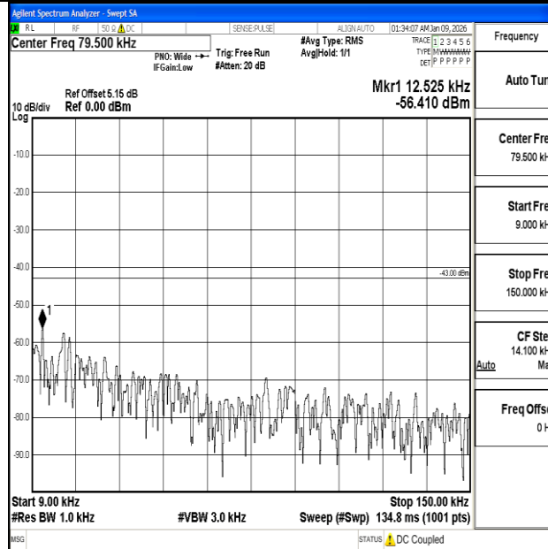
Band2_15MHz_16QAM_18900_1RB#0_0.009~0.15_0.009~0.15
