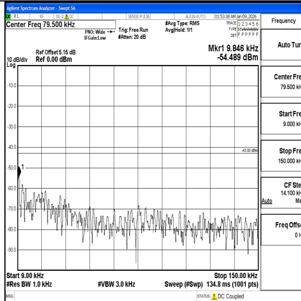
Band2_20MHz_QPSK_19100_1RB#0_0.009~0.15_0.009~0.15
