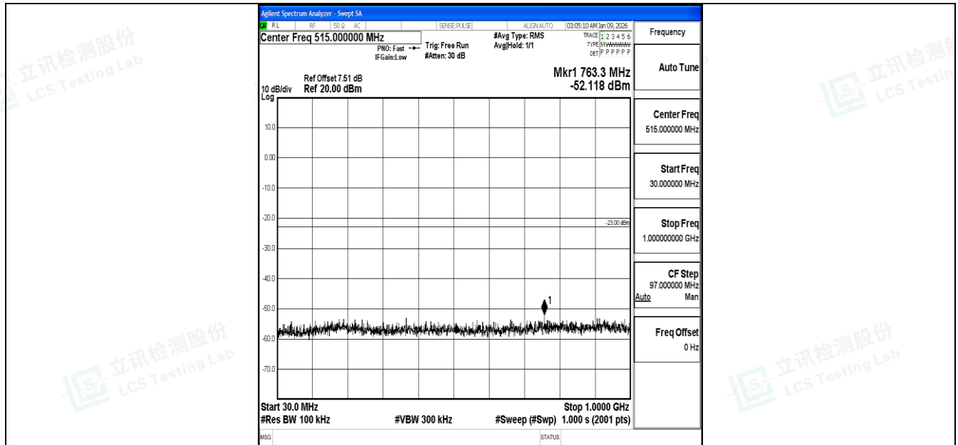
Band4_5MHz_16QAM_20375_1RB#0_30~1000_30~1000
