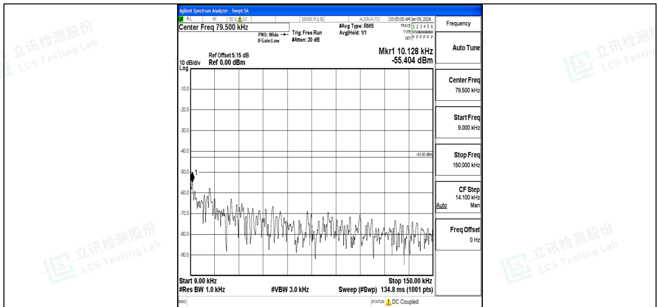
Band4_5MHz_16QAM_20375_1RB#0_0.009~0.15_0.009~0.15
