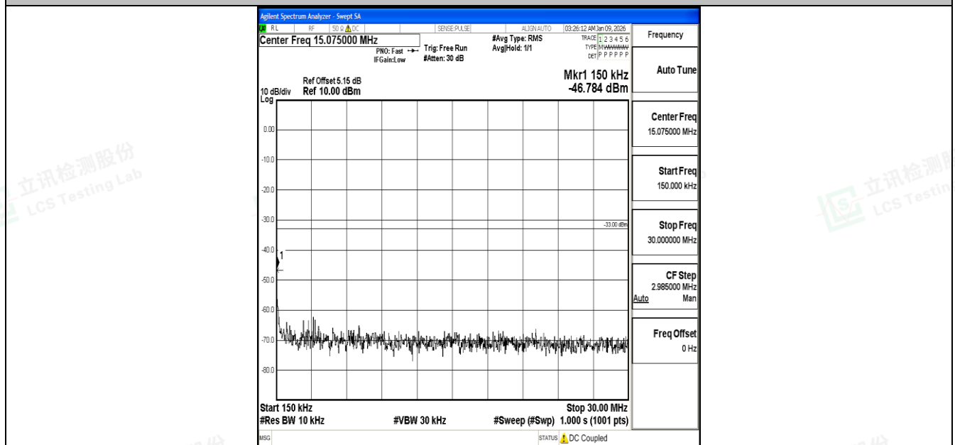
Band4_10MHz_16QAM_20350_1RB#0_0.15~30_0.15~30
