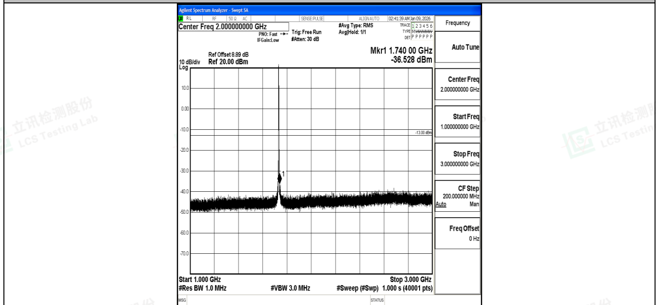
Band4_3MHz_16QAM_20175_1RB#0_1000~3000_1000~3000
