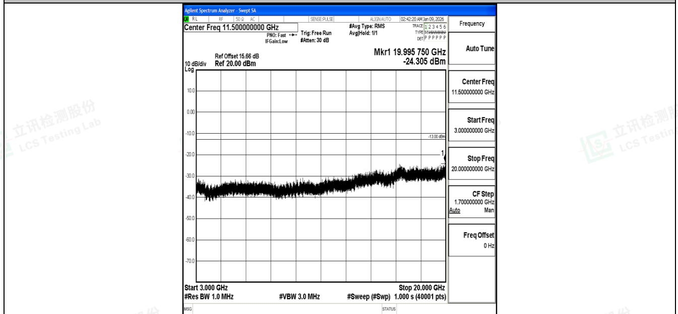
Band4_3MHz_QPSK_20385_1RB#0_3000~20000_3000~20000
