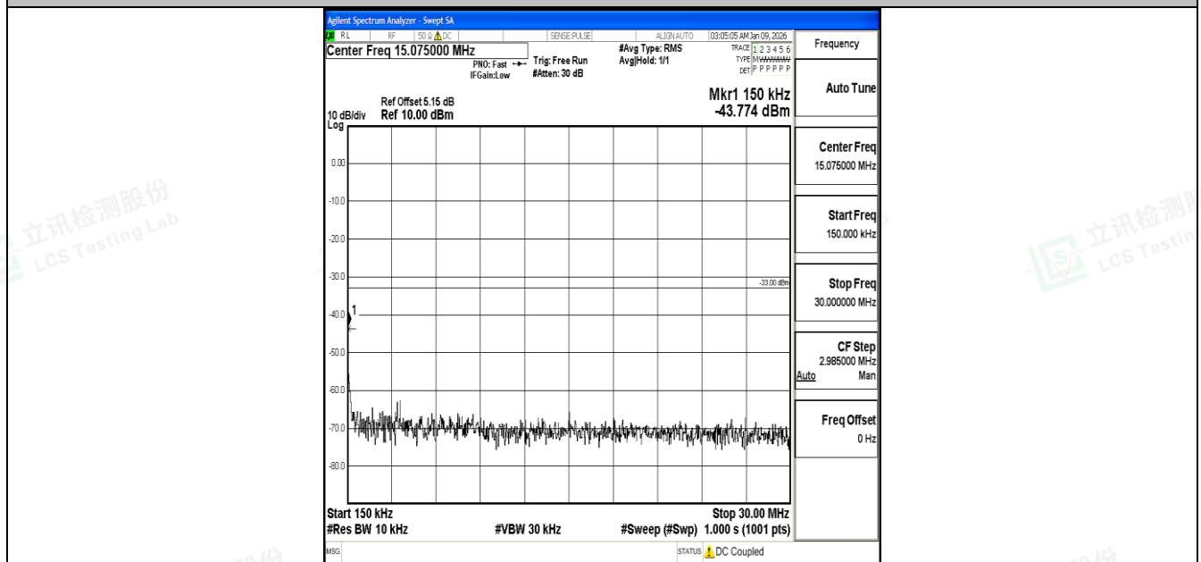
Band4_5MHz_16QAM_20375_1RB#0_0.15~30_0.15~30
