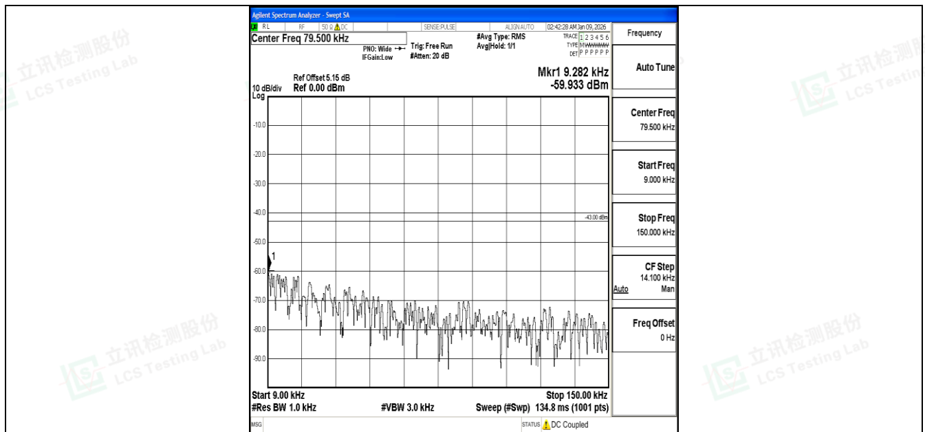
Band4_3MHz_16QAM_20385_1RB#0_0.009~0.15_0.009~0.15
