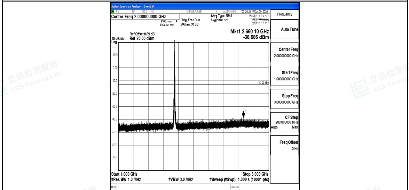
Band4_10MHz_16QAM_20350_1RB#0_1000~3000_1000~3000
