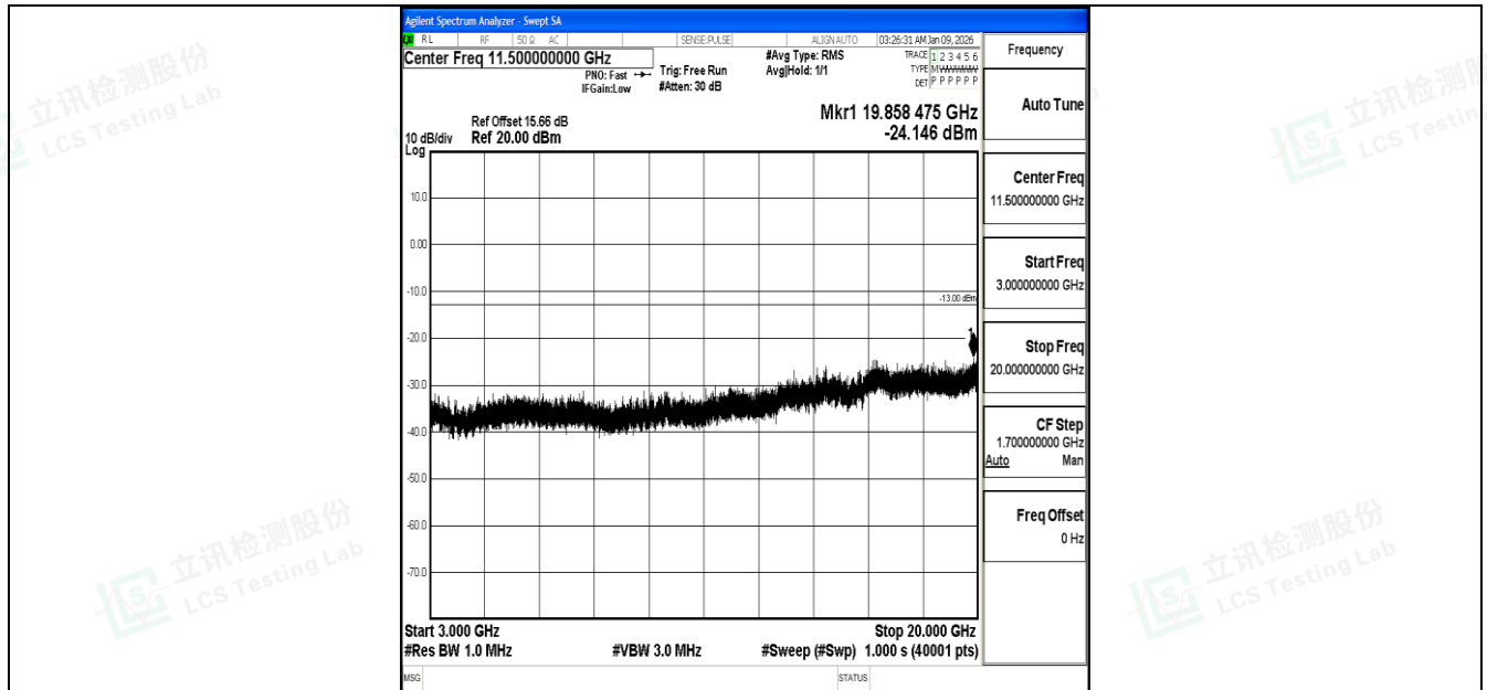
Band4_10MHz_16QAM_20350_1RB#0_3000~20000_3000~20000
