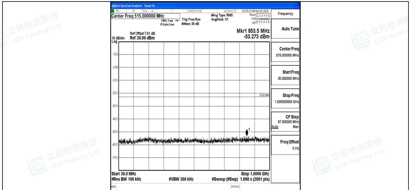
Band4_10MHz_16QAM_20175_1RB#0_30~1000_30~1000
