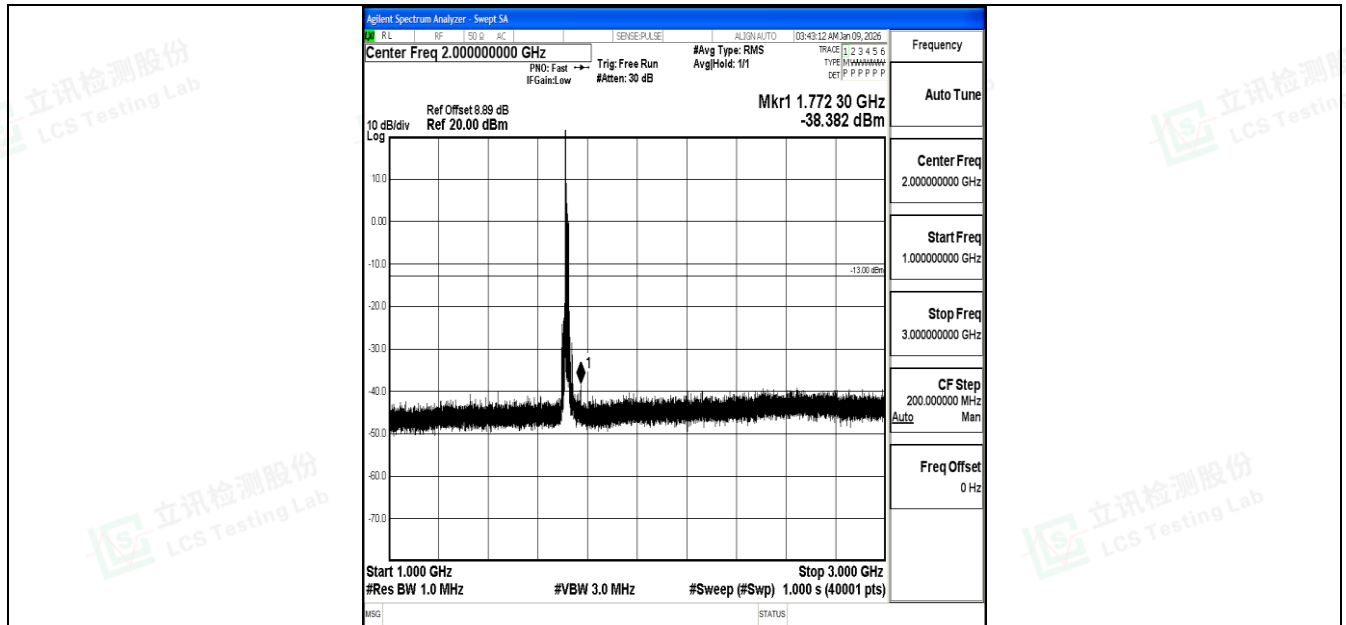
Band4_15MHz_QPSK_20025_1RB#0_1000~3000_1000~3000
