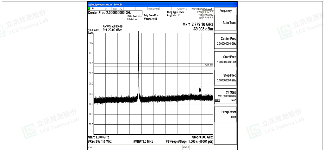
Band4_5MHz_QPSK_20375_1RB#0_1000~3000_1000~3000
