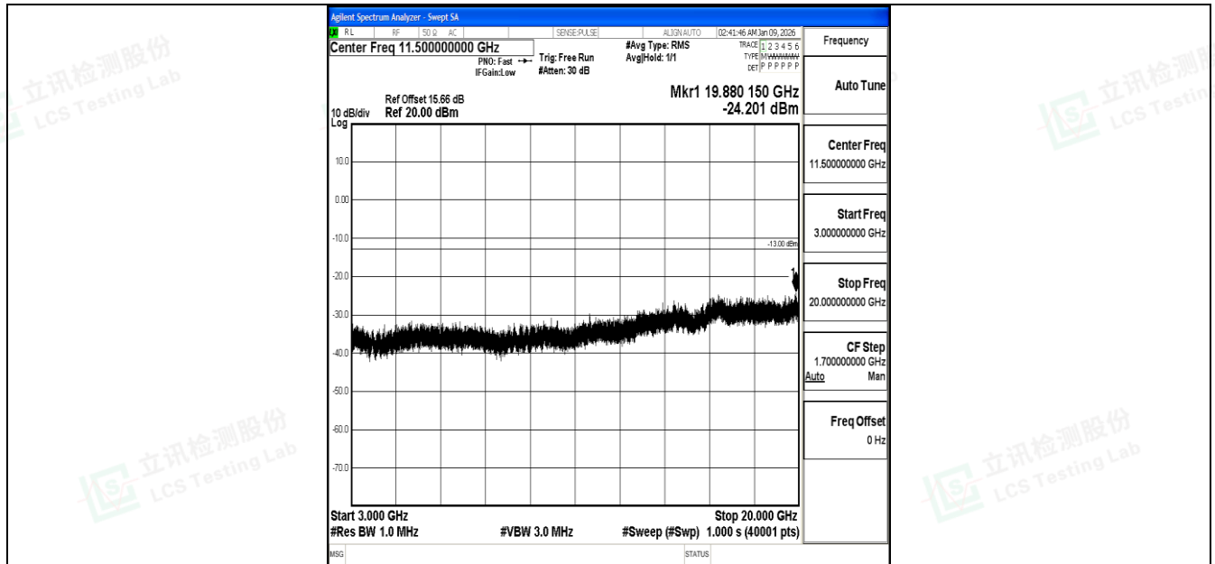
Band4_3MHz_16QAM_20175_1RB#0_3000~20000_3000~20000
