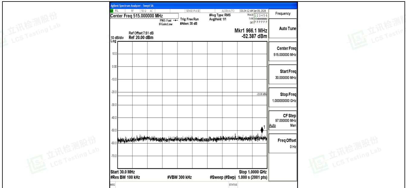
Band4_10MHz_16QAM_20000_1RB#0_30~1000_30~1000
