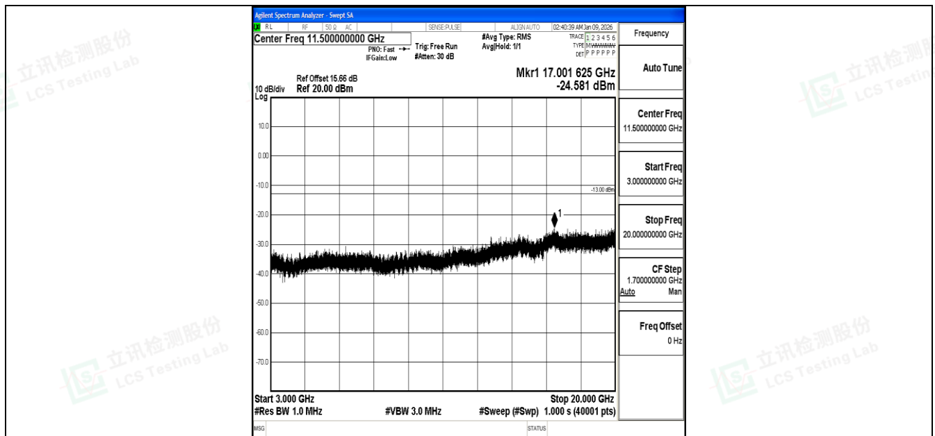
Band4_3MHz_16QAM_19965_1RB#0_3000~20000_3000~20000
