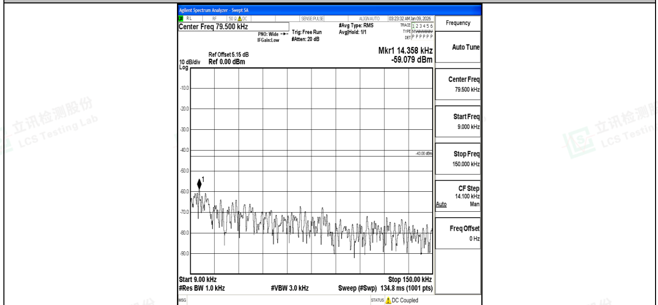
Band4_10MHz_QPSK_20000_1RB#0_0.009~0.15_0.009~0.15
