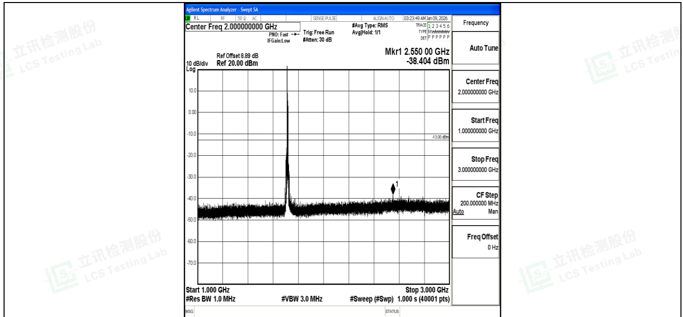
Band4_10MHz_QPSK_20000_1RB#0_1000~3000_1000~3000
