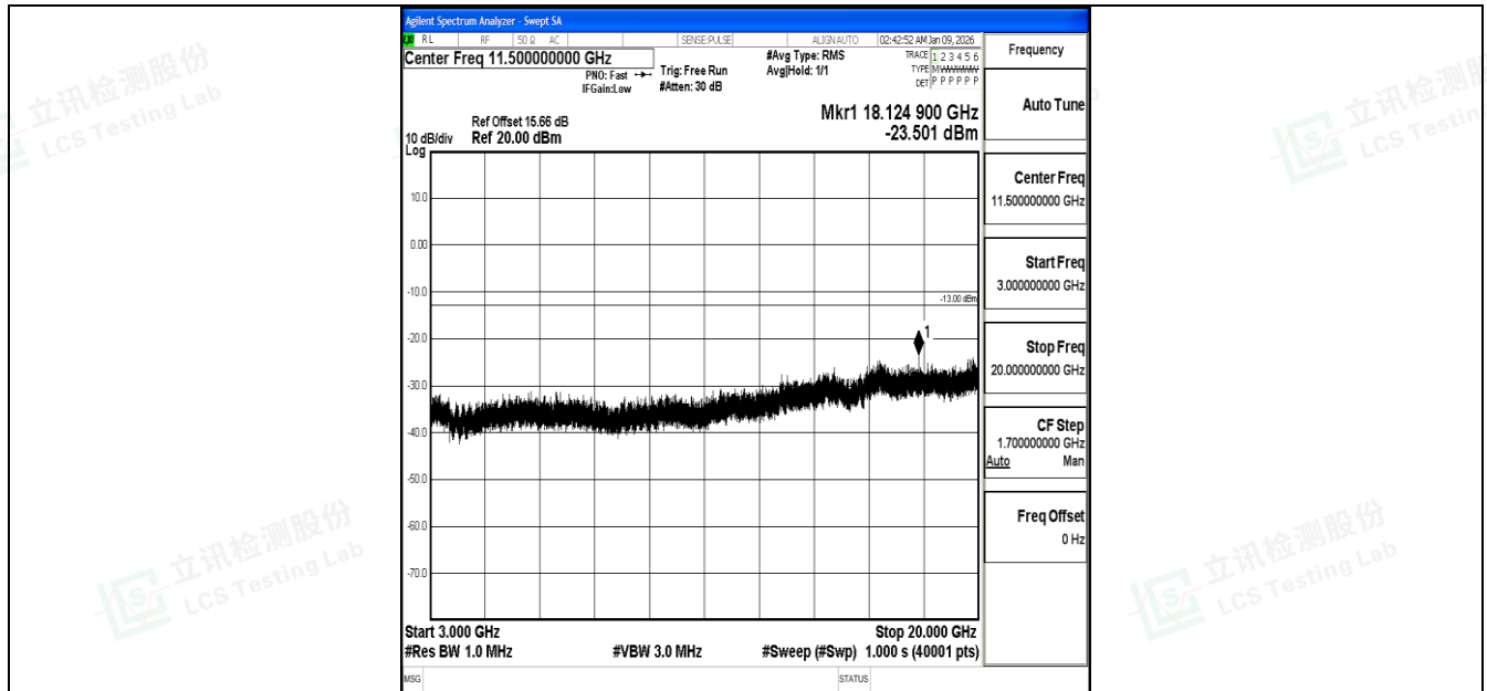
Band4_3MHz_16QAM_20385_1RB#0_3000~20000_3000~20000
