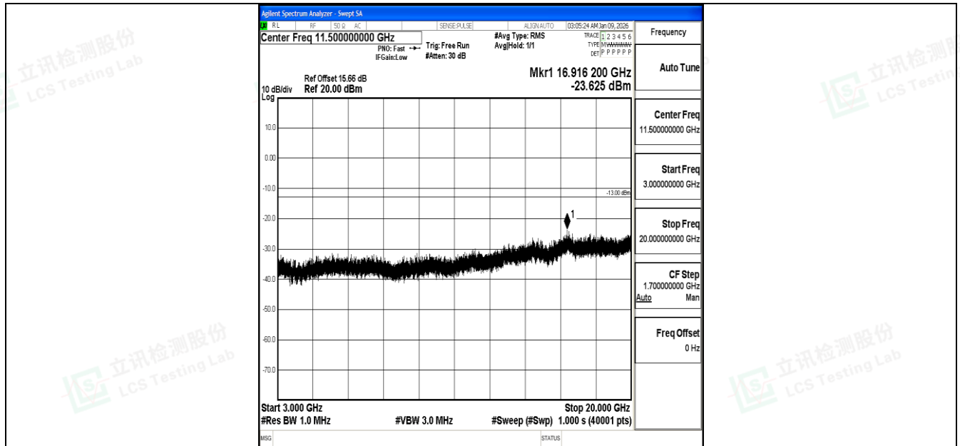
Band4_5MHz_16QAM_20375_1RB#0_3000~20000_3000~20000
