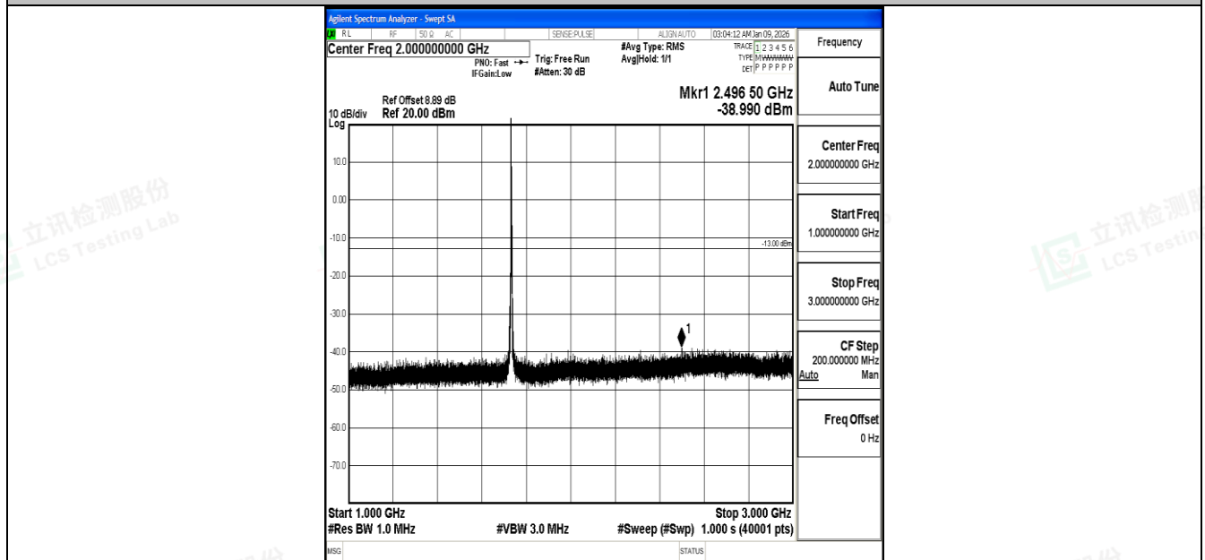
Band4_5MHz_16QAM_20175_1RB#0_1000~3000_1000~3000
