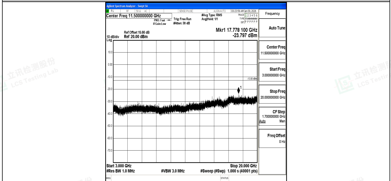
Band4_10MHz_QPSK_20000_1RB#0_3000~20000_3000~20000
