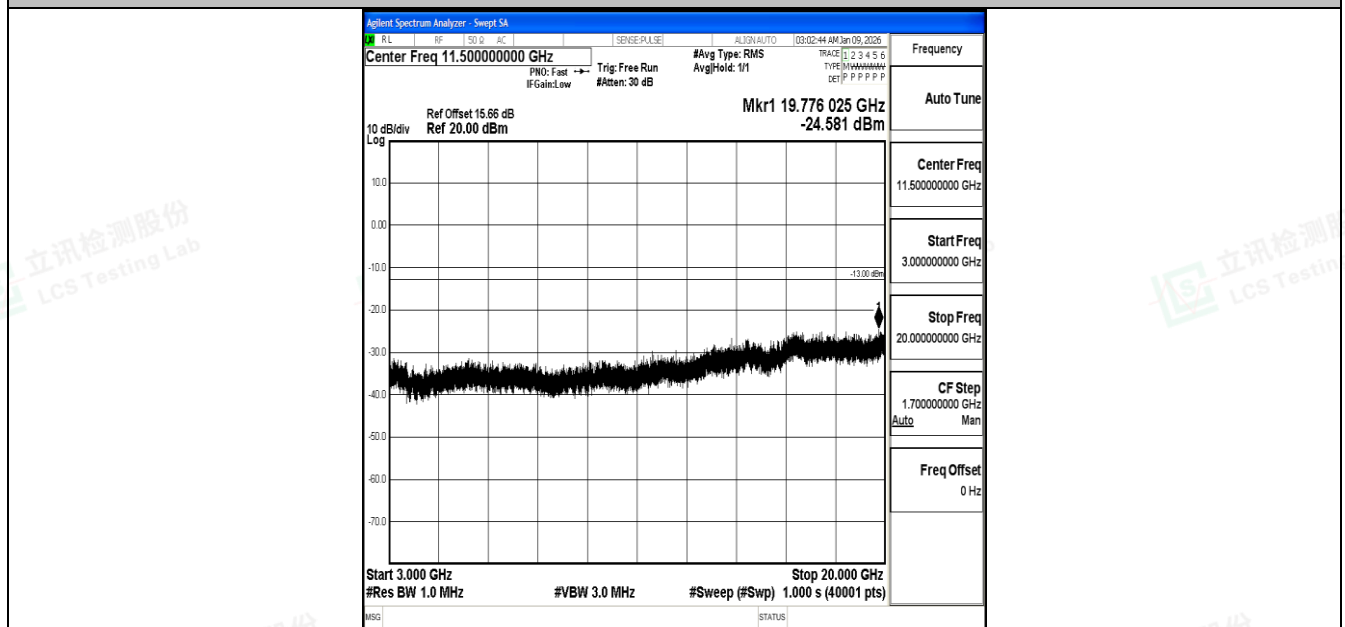
Band4_5MHz_QPSK_19975_1RB#0_3000~20000_3000~20000
