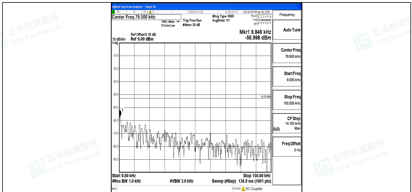
Band4_10MHz_16QAM_20350_1RB#0_0.009~0.15_0.009~0.15
