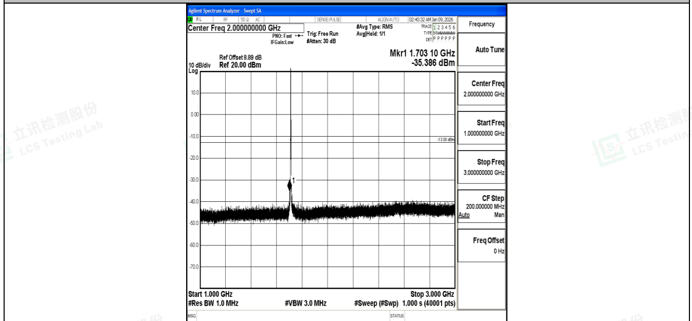
Band4_3MHz_16QAM_19965_1RB#0_1000~3000_1000~3000
