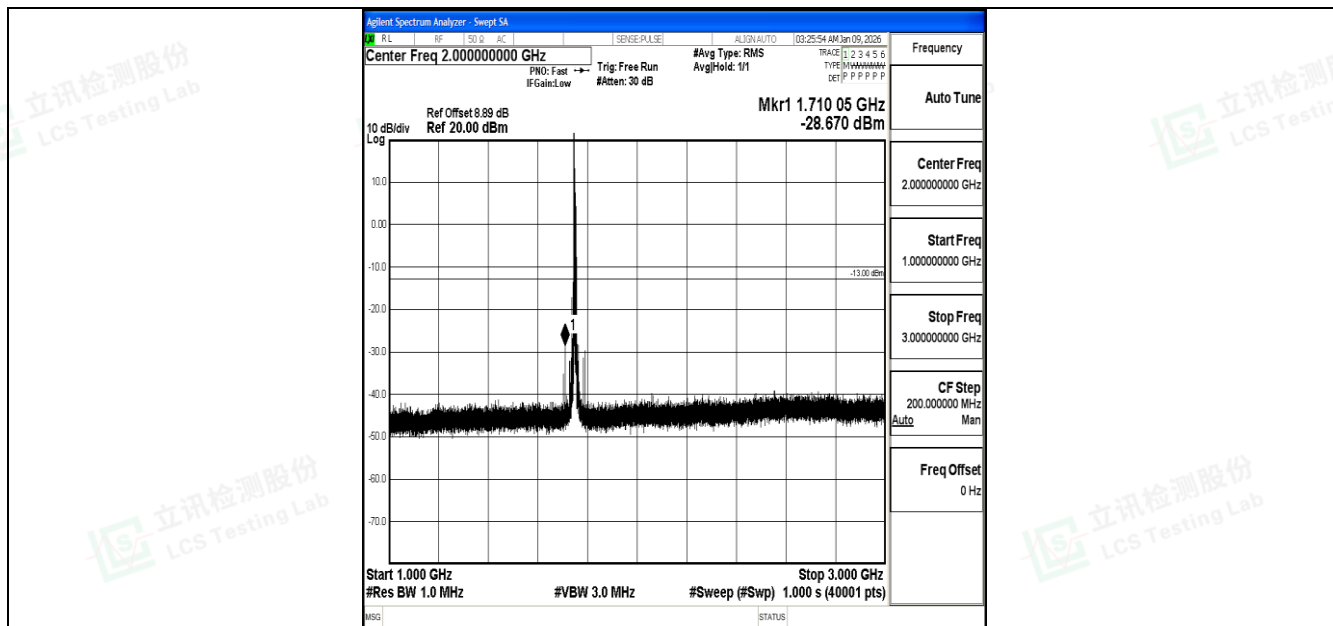
Band4_10MHz_QPSK_20350_1RB#0_1000~3000_1000~3000
