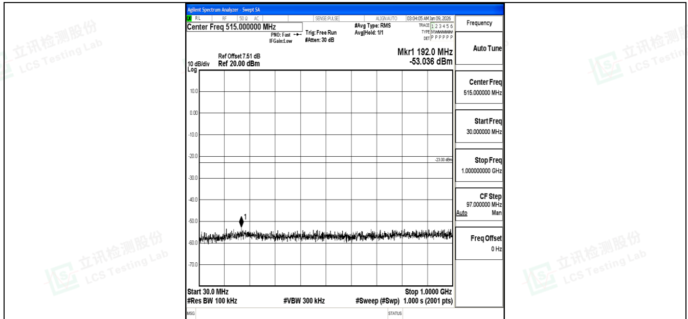
Band4_5MHz_16QAM_20175_1RB#0_30~1000_30~1000
