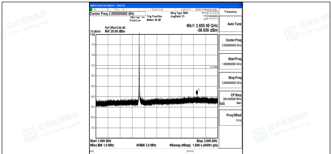
Band4_5MHz_QPSK_19975_1RB#0_1000~3000_1000~3000
