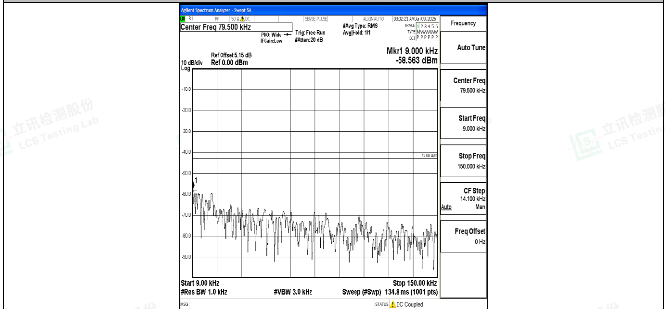
Band4_5MHz_QPSK_19975_1RB#0_0.009~0.15_0.009~0.15
