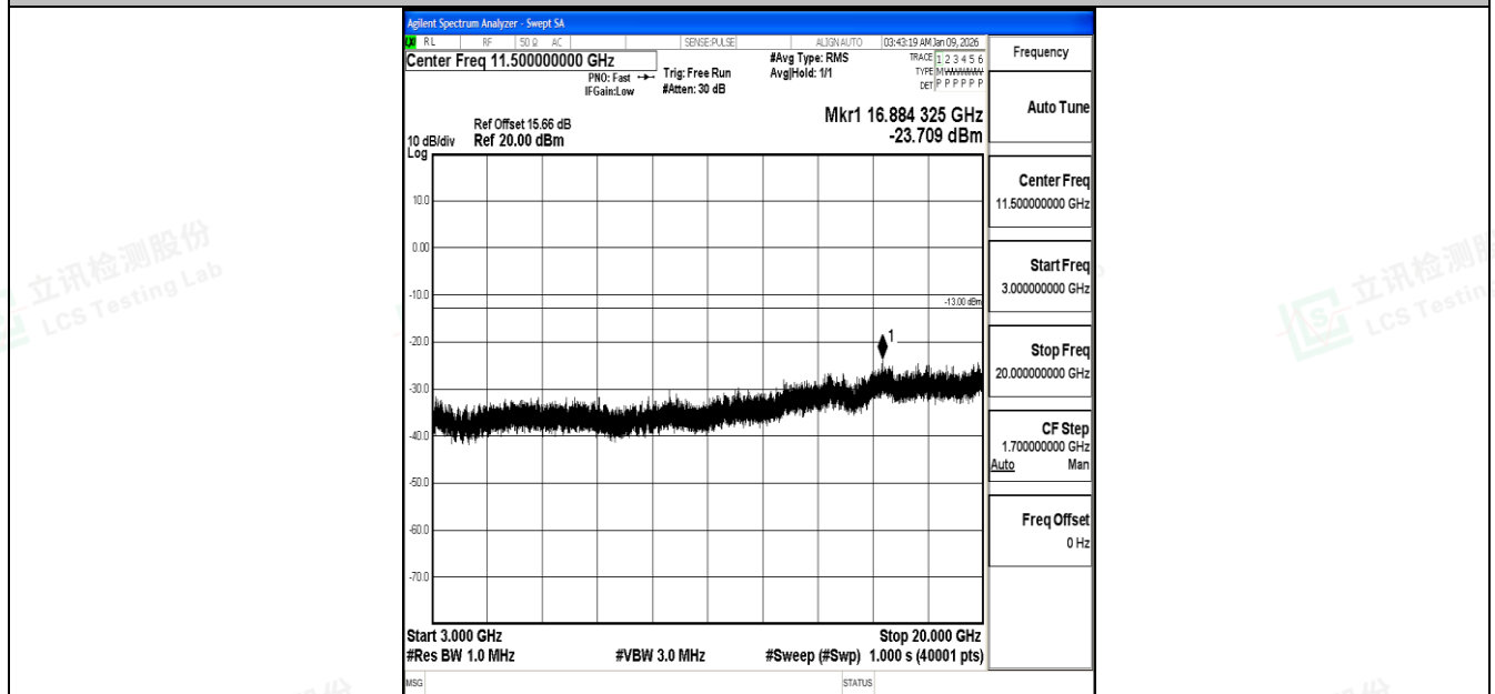
Band4_15MHz_QPSK_20025_1RB#0_3000~20000_3000~20000
