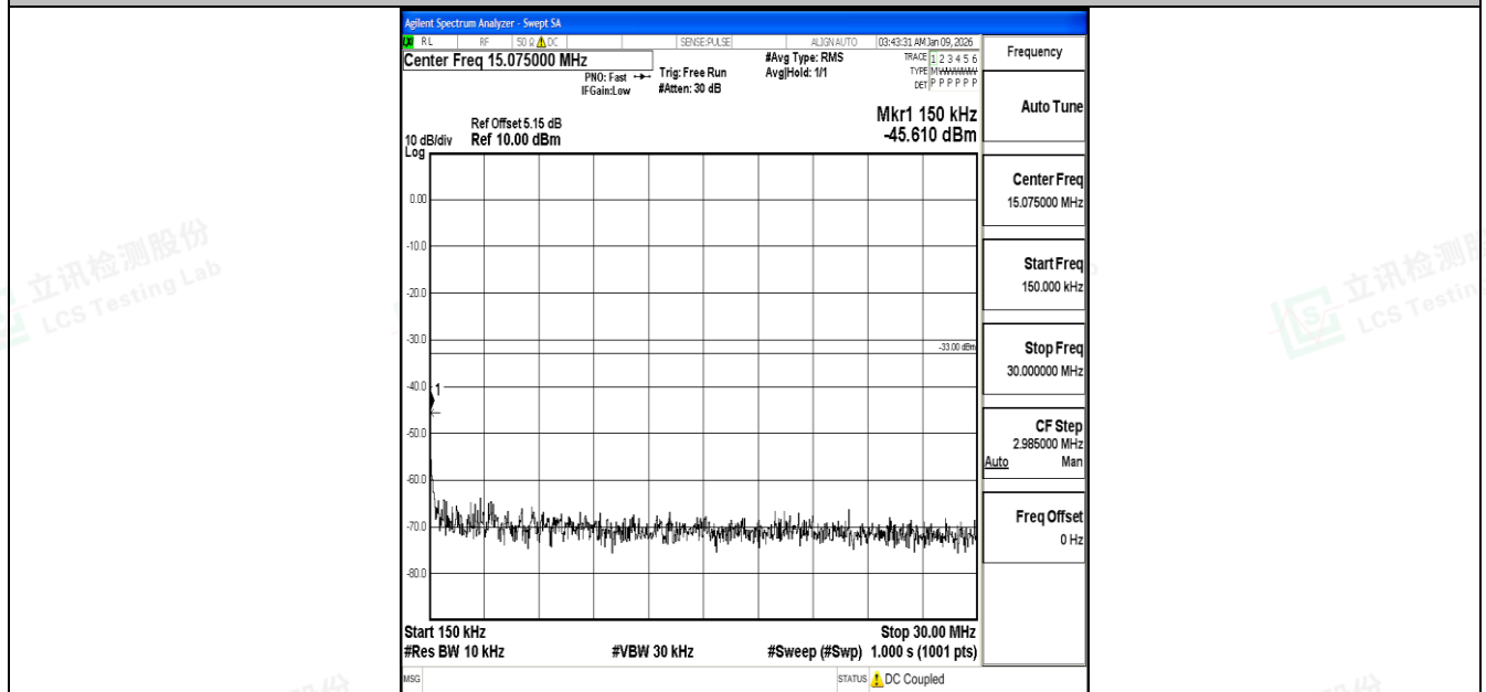
Band4_15MHz_16QAM_20025_1RB#0_0.15~30_0.15~30
