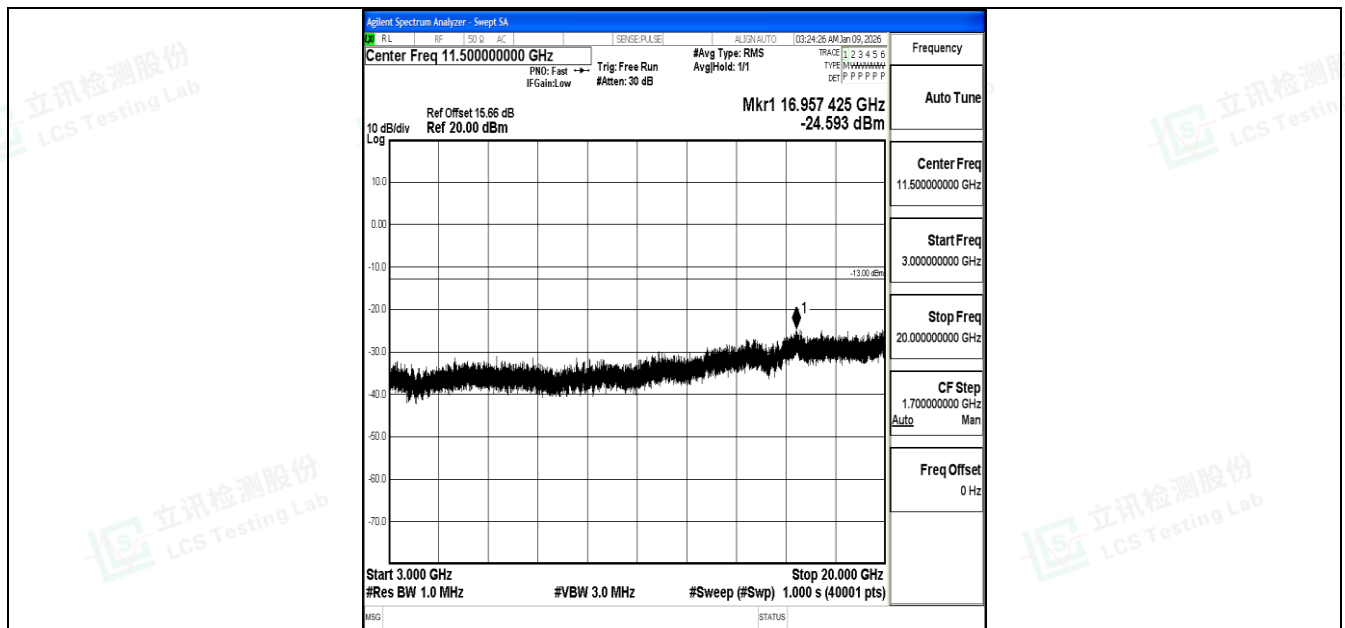
Band4_10MHz_16QAM_20000_1RB#0_3000~20000_3000~20000
