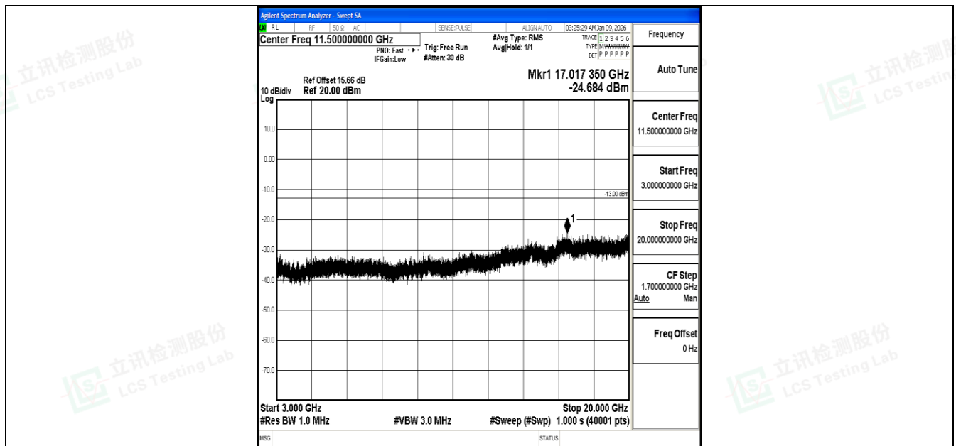
Band4_10MHz_16QAM_20175_1RB#0_3000~20000_3000~20000
