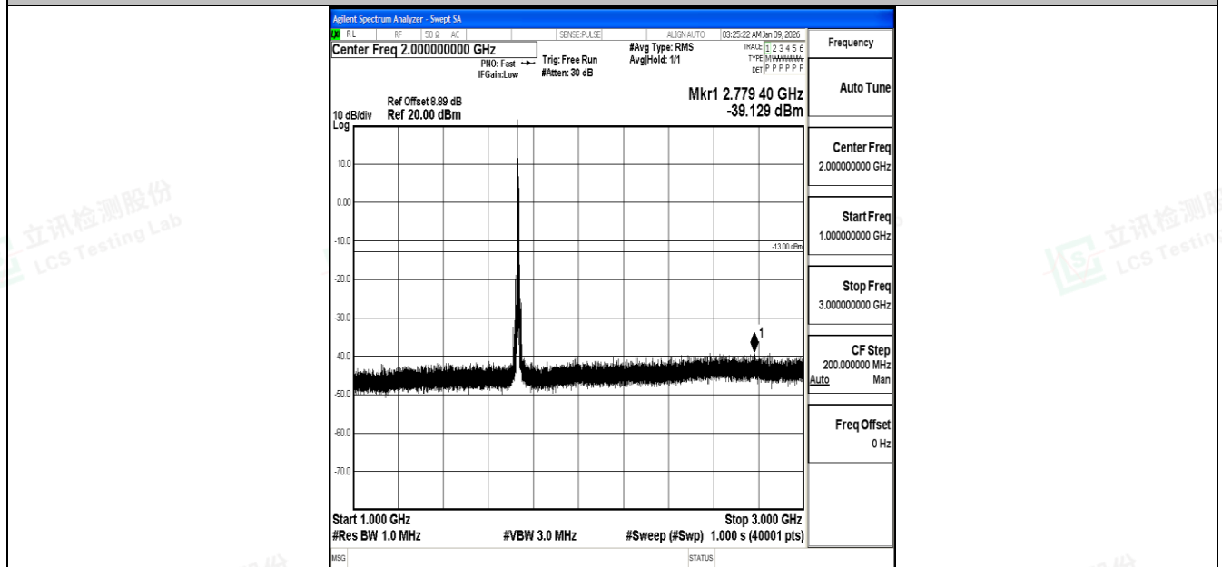
Band4_10MHz_16QAM_20175_1RB#0_1000~3000_1000~3000
