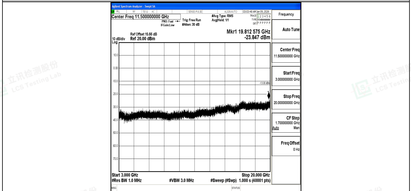
Band4_5MHz_QPSK_20175_1RB#0_3000~20000_3000~20000
