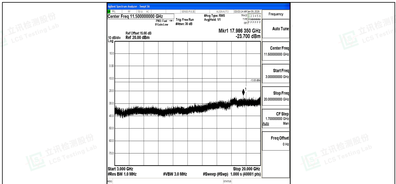
Band4_5MHz_16QAM_19975_1RB#0_3000~20000_3000~20000
