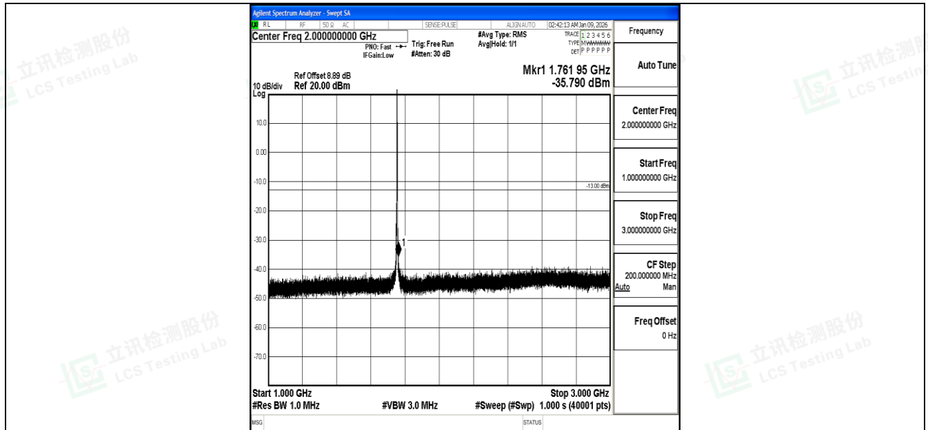
Band4_3MHz_QPSK_20385_1RB#0_1000~3000_1000~3000
