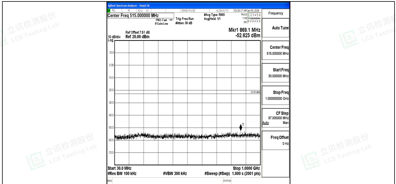
Band4_10MHz_16QAM_20350_1RB#0_30~1000_30~1000
