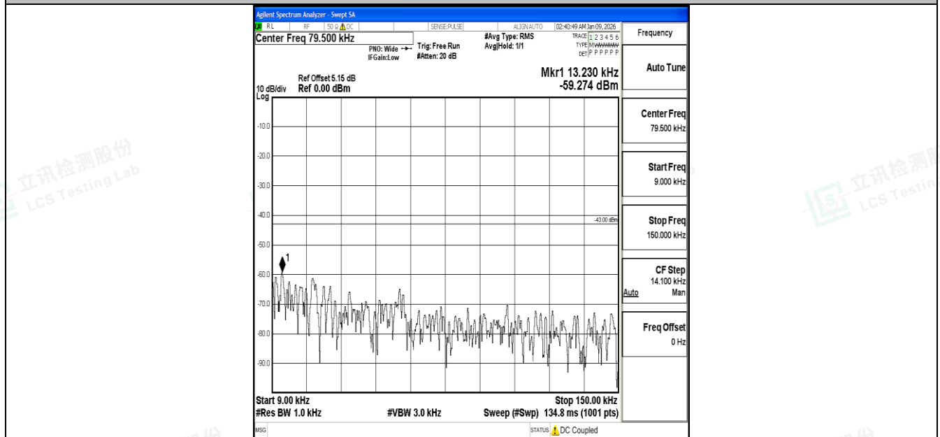
Band4_3MHz_QPSK_20175_1RB#0_0.009~0.15_0.009~0.15
