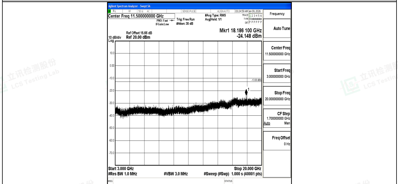
Band4_10MHz_QPSK_20175_1RB#0_3000~20000_3000~20000
