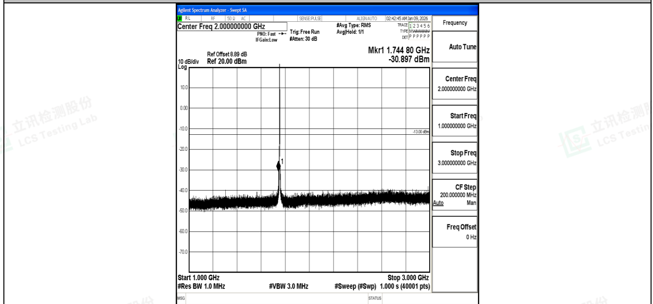
Band4_3MHz_16QAM_20385_1RB#0_1000~3000_1000~3000
