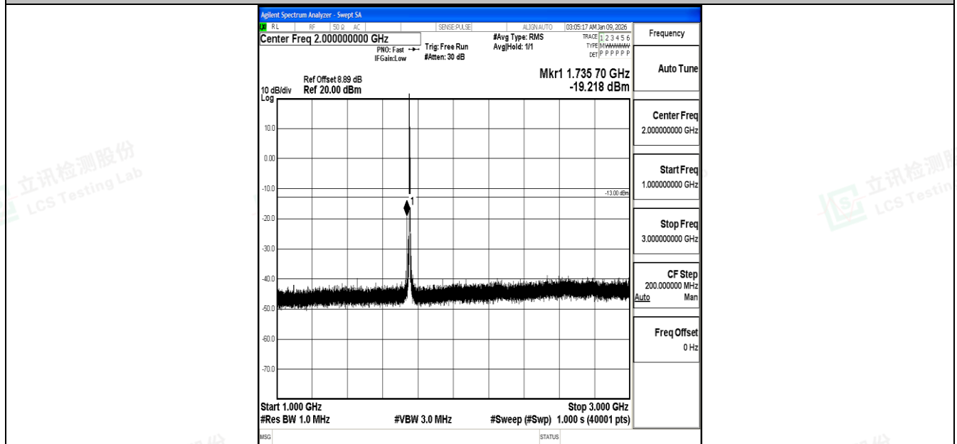
Band4_5MHz_16QAM_20375_1RB#0_1000~3000_1000~3000
