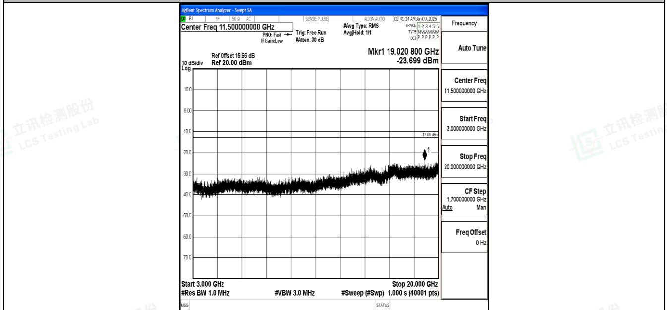
Band4_3MHz_QPSK_20175_1RB#0_3000~20000_3000~20000
