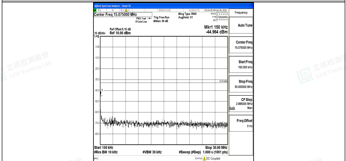
Band4_5MHz_16QAM_20175_1RB#0_0.15~30_0.15~30
