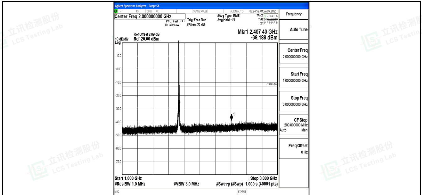
Band4_10MHz_QPSK_20175_1RB#0_1000~3000_1000~3000
