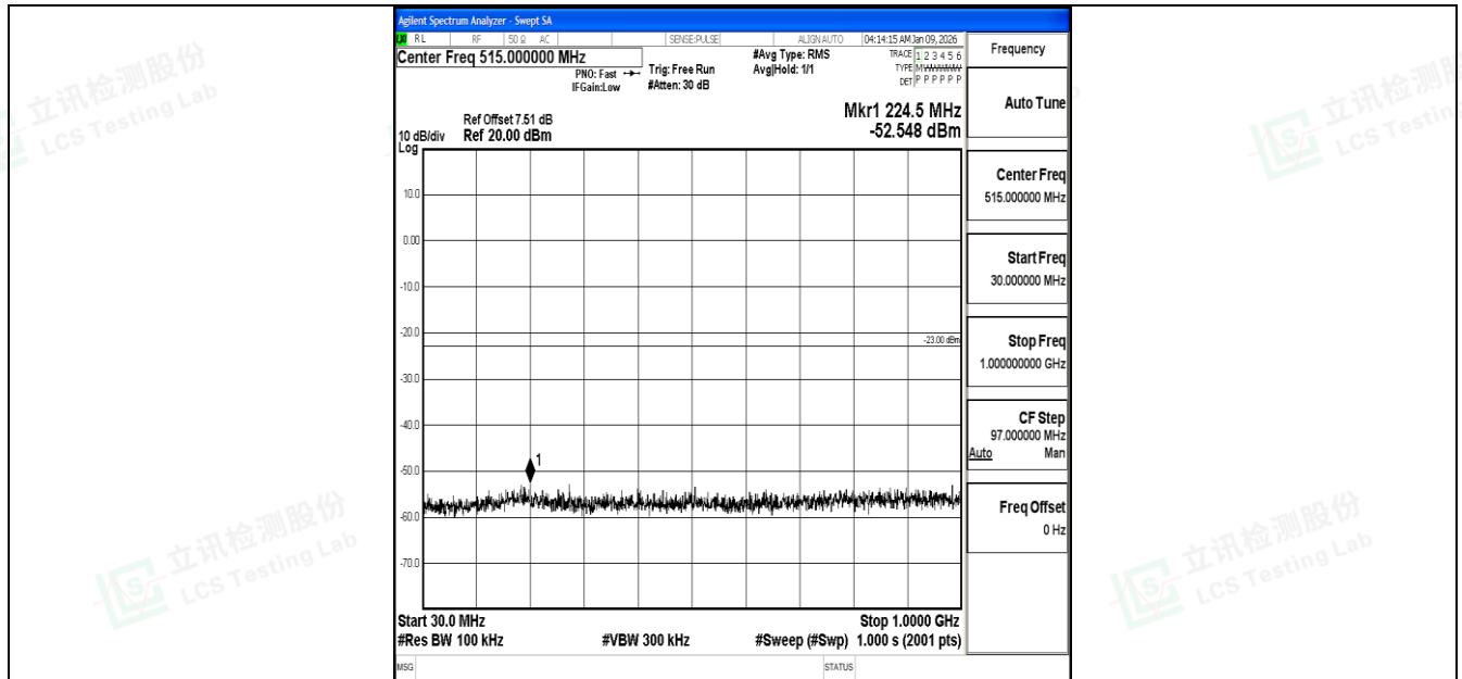
Band4_20MHz_16QAM_20175_1RB#0_30~1000_30~1000
