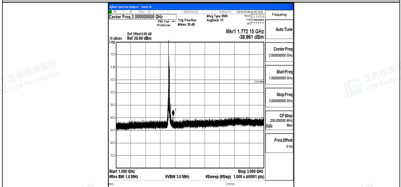
Band4_15MHz_16QAM_20025_1RB#0_1000~3000_1000~3000
