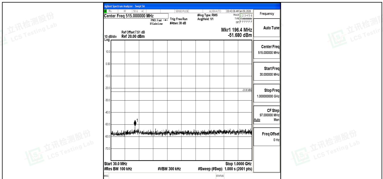
Band4_15MHz_16QAM_20025_1RB#0_30~1000_30~1000
