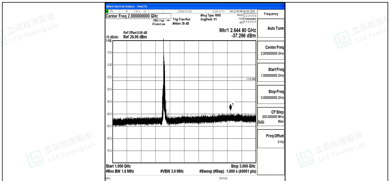
Band4_20MHz_QPSK_20050_1RB#0_1000~3000_1000~3000
