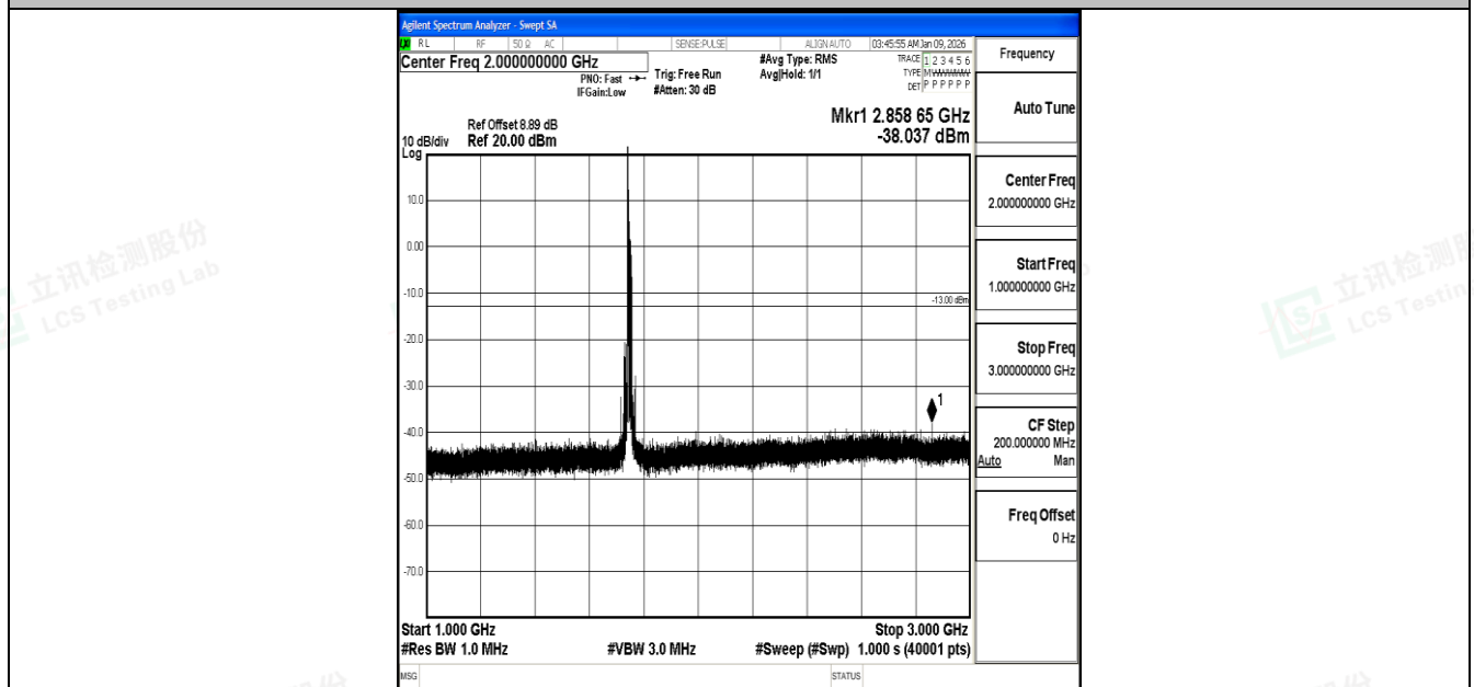
Band4_15MHz_16QAM_20325_1RB#0_1000~3000_1000~3000
