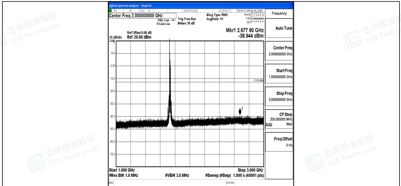
Band4_15MHz_QPSK_20175_1RB#0_1000~3000_1000~3000
