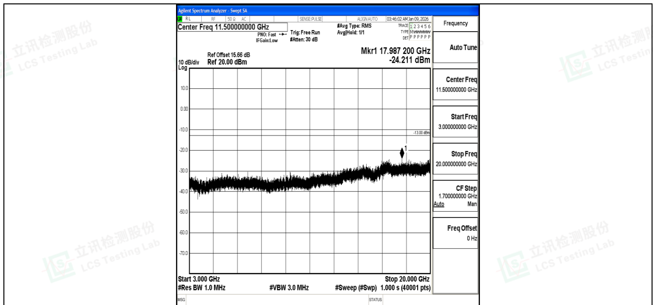
Band4_15MHz_16QAM_20325_1RB#0_3000~20000_3000~20000
