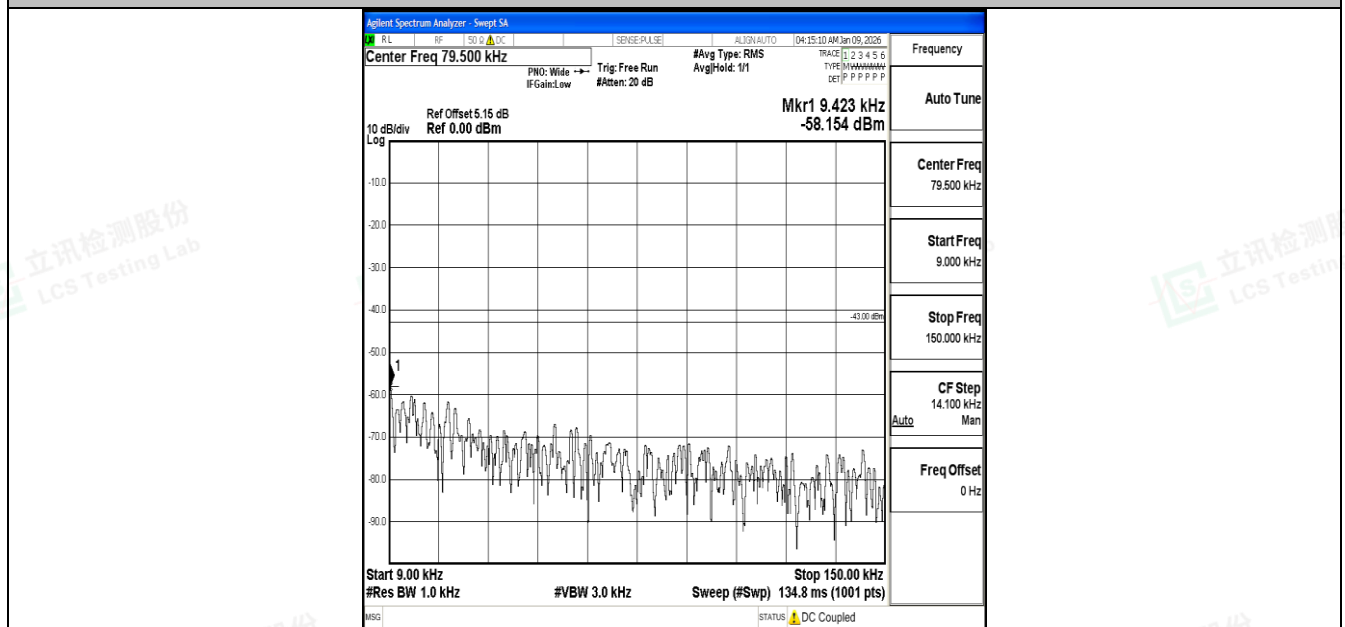
Band4_20MHz_16QAM_20300_1RB#0_0.009~0.15_0.009~0.15
