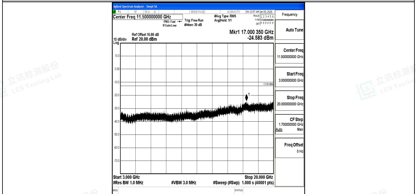
Band4_20MHz_QPSK_20175_1RB#0_3000~20000_3000~20000
