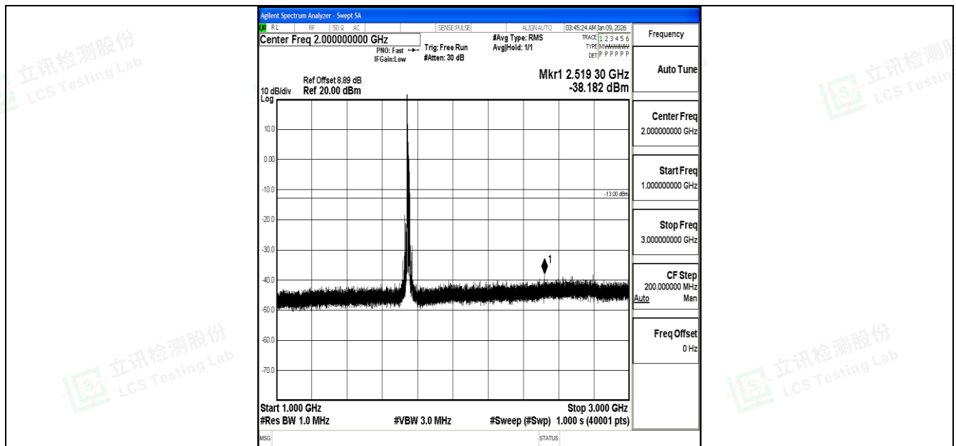
Band4_15MHz_QPSK_20325_1RB#0_1000~3000_1000~3000
