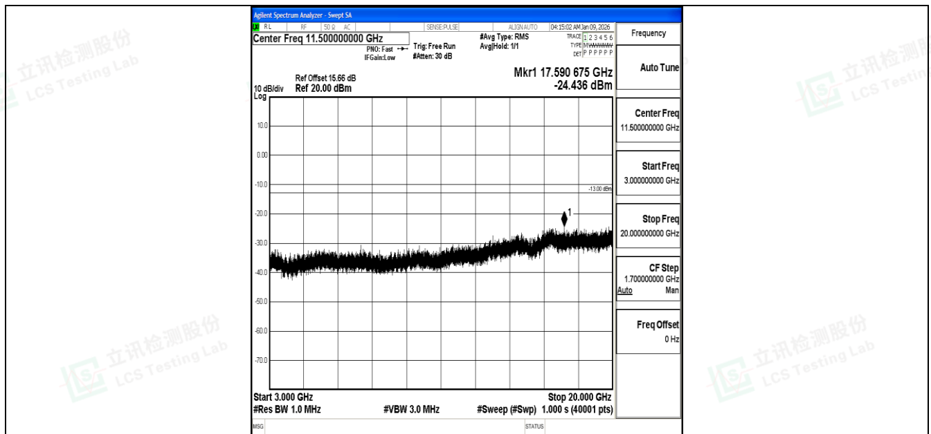
Band4_20MHz_QPSK_20300_1RB#0_3000~20000_3000~20000
