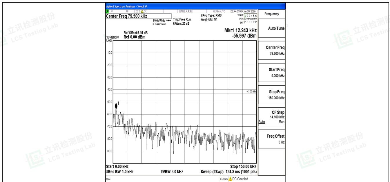
Band4_15MHz_16QAM_20175_1RB#0_0.009~0.15_0.009~0.15
