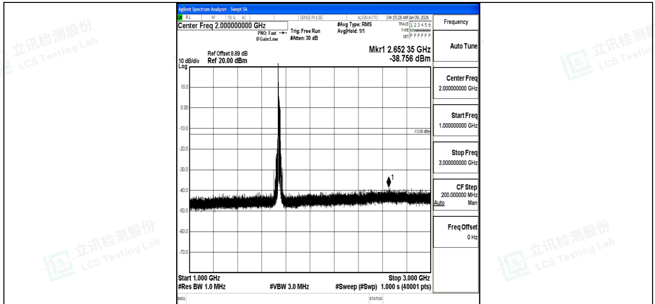
Band4_20MHz_16QAM_20300_1RB#0_1000~3000_1000~3000
