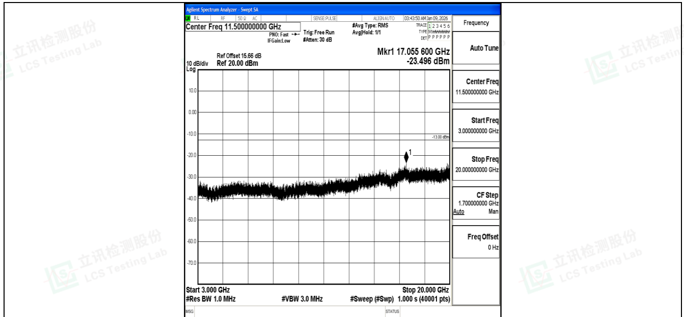
Band4_15MHz_16QAM_20025_1RB#0_3000~20000_3000~20000
