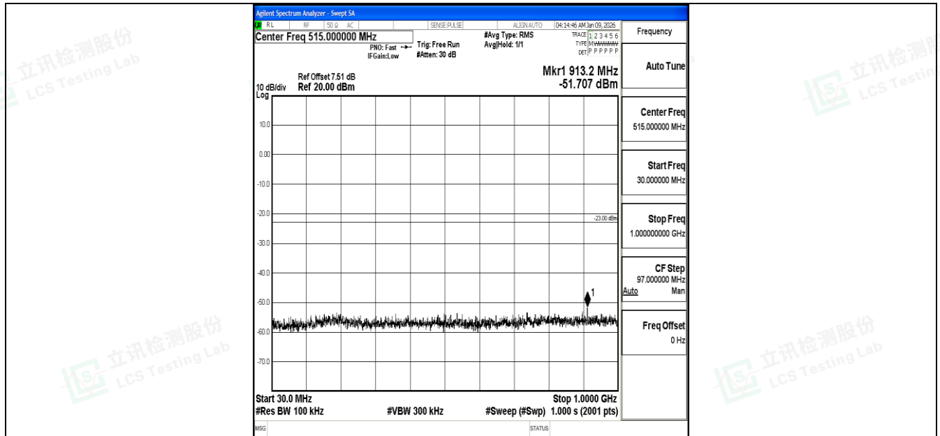
Band4_20MHz_QPSK_20300_1RB#0_30~1000_30~1000
