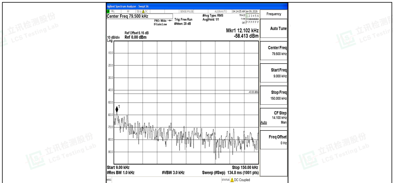
Band4_20MHz_16QAM_20175_1RB#0_0.009~0.15_0.009~0.15
