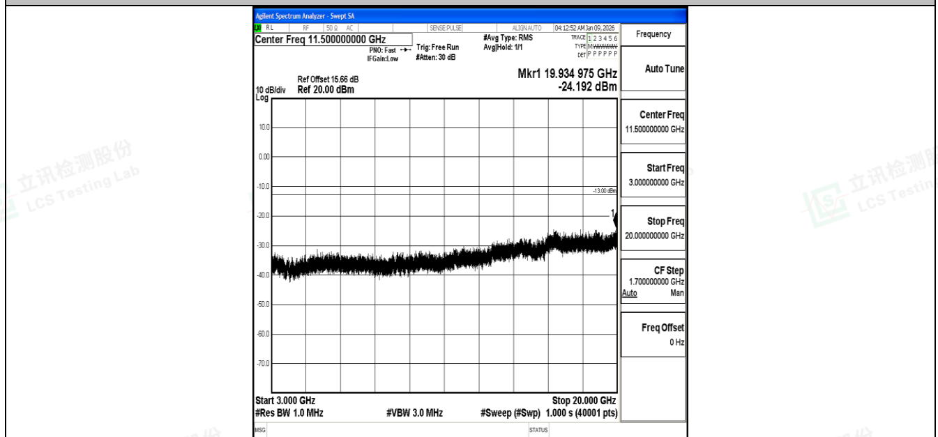
Band4_20MHz_QPSK_20050_1RB#0_3000~20000_3000~20000
