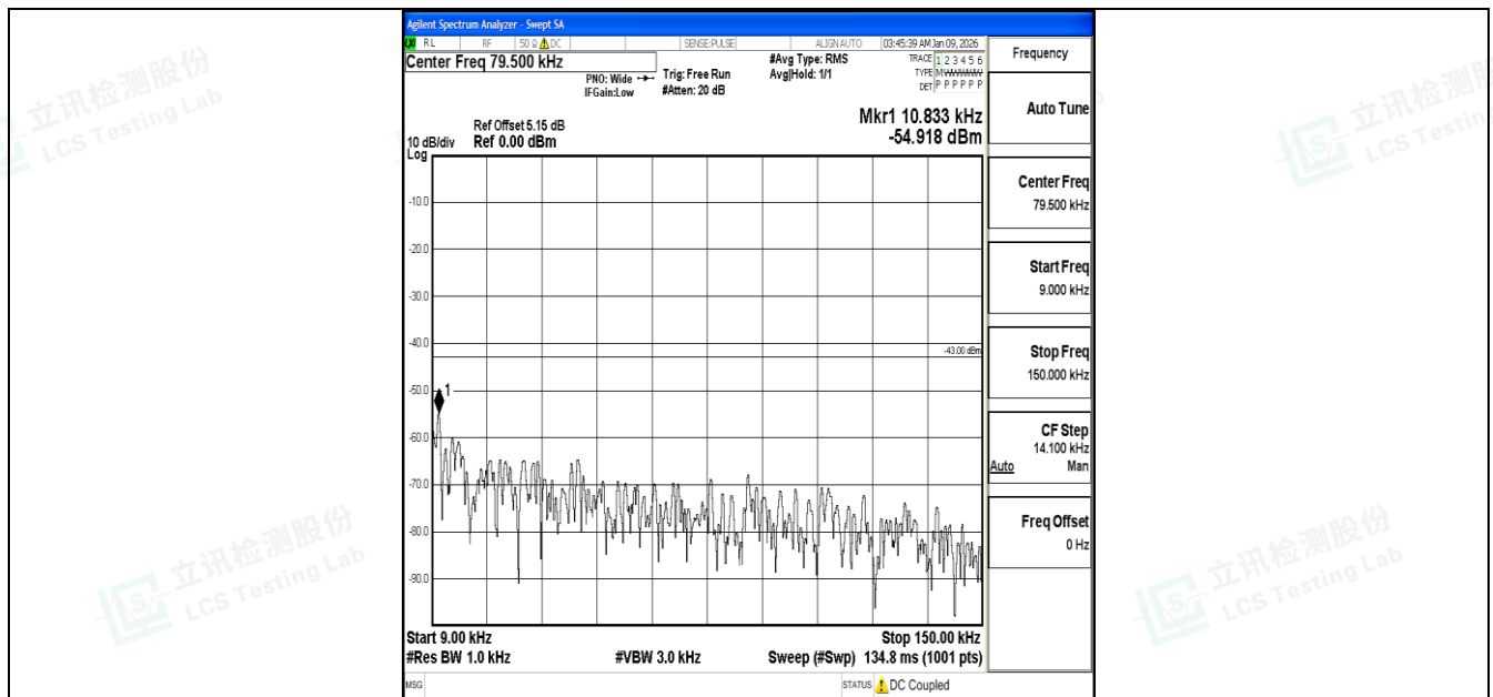
Band4_15MHz_16QAM_20325_1RB#0_0.009~0.15_0.009~0.15
