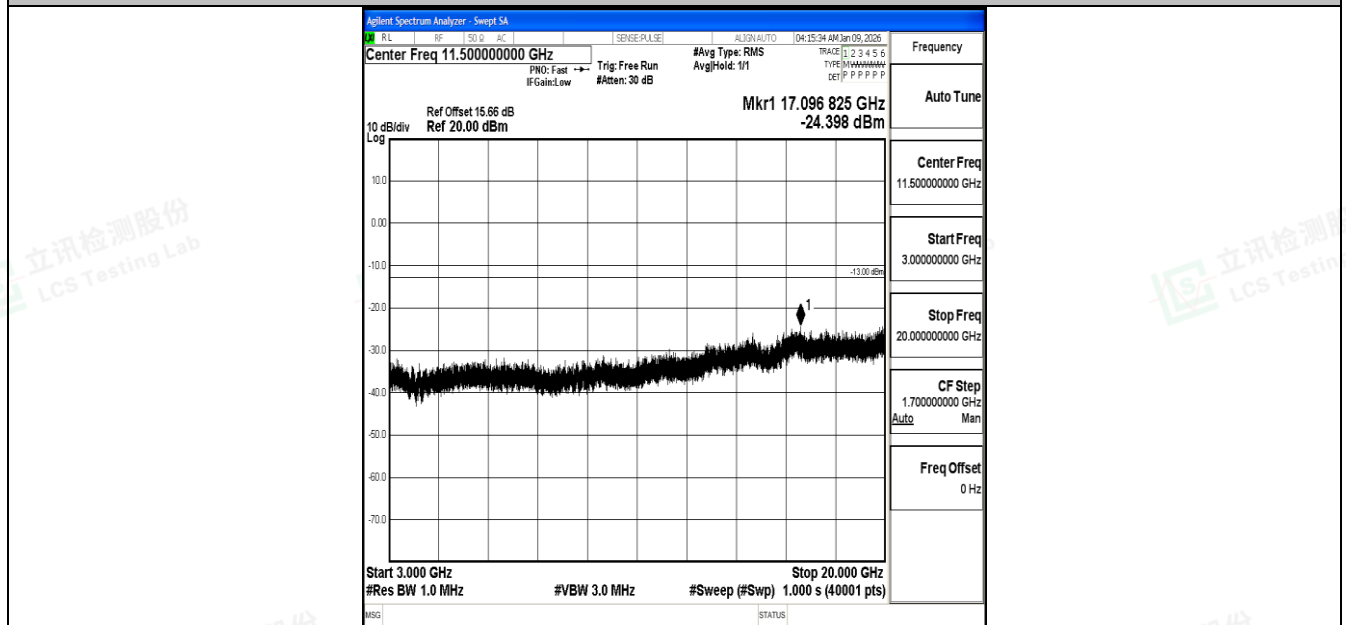
Band4_20MHz_16QAM_20300_1RB#0_3000~20000_3000~20000
