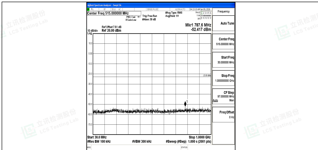
Band4_20MHz_16QAM_20050_1RB#0_30~1000_30~1000
