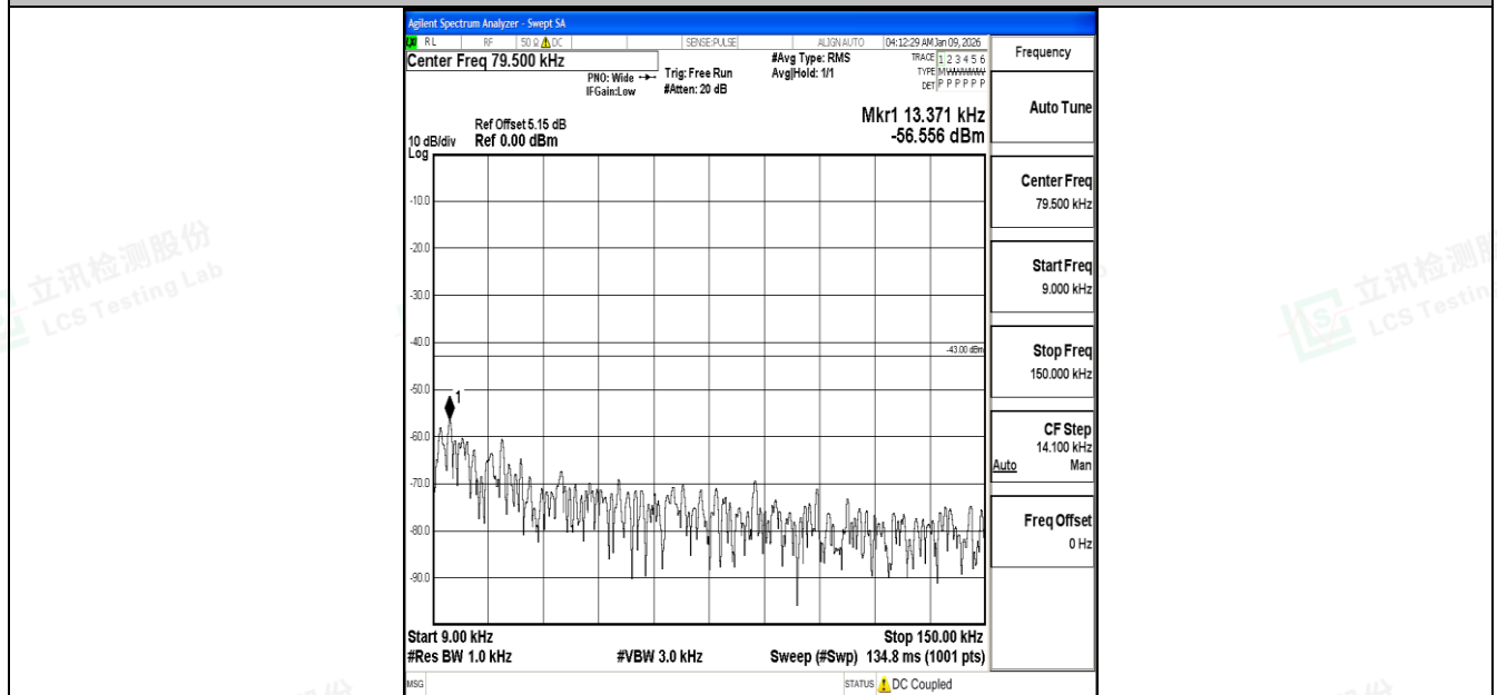
Band4_20MHz_QPSK_20050_1RB#0_0.009~0.15_0.009~0.15
