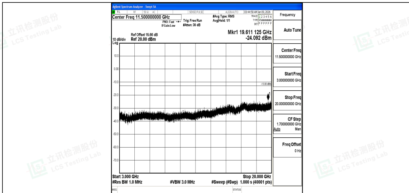
Band4_15MHz_16QAM_20175_1RB#0_3000~20000_3000~20000
