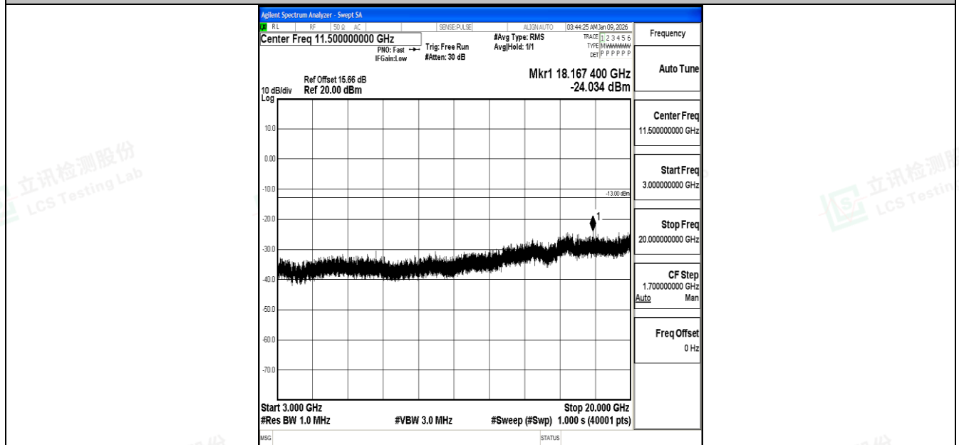
Band4_15MHz_QPSK_20175_1RB#0_3000~20000_3000~20000
