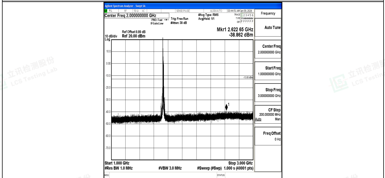
Band4_15MHz_16QAM_20175_1RB#0_1000~3000_1000~3000
