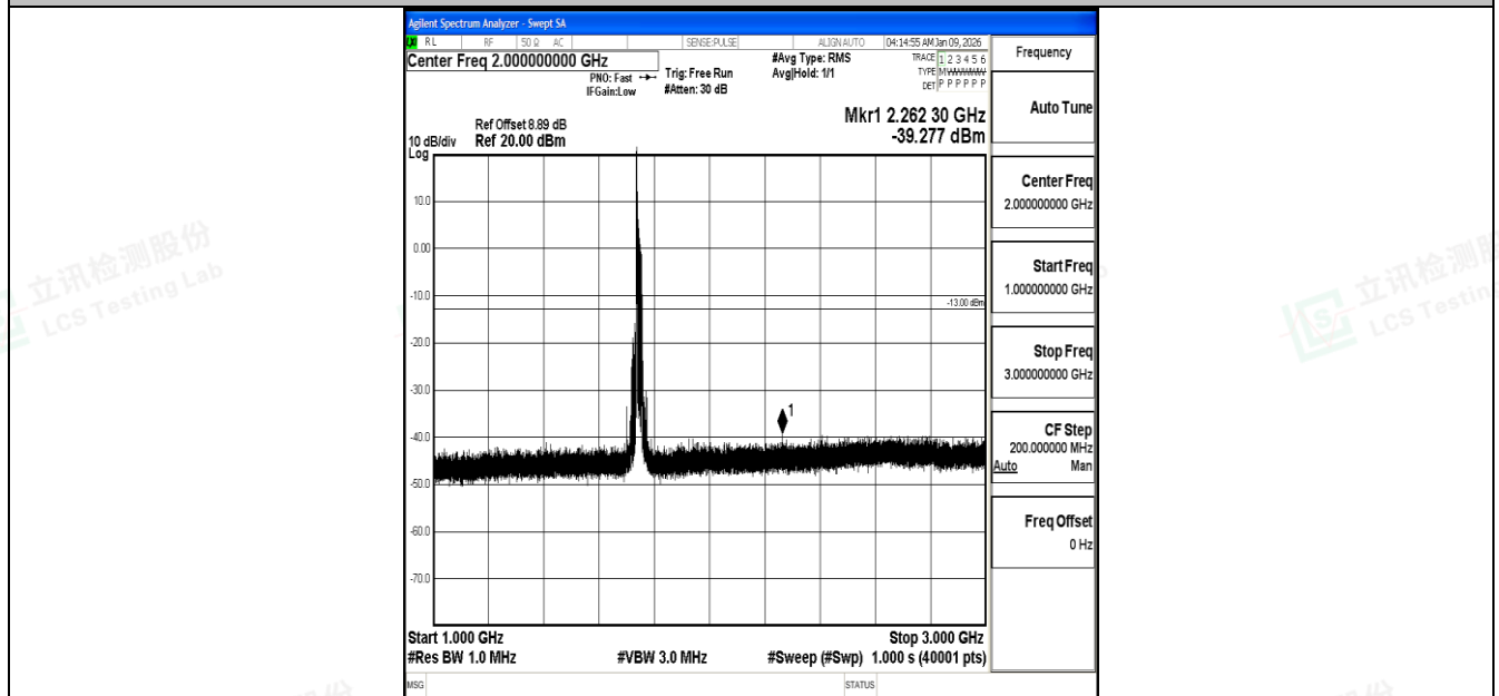
Band4_20MHz_QPSK_20300_1RB#0_1000~3000_1000~3000
