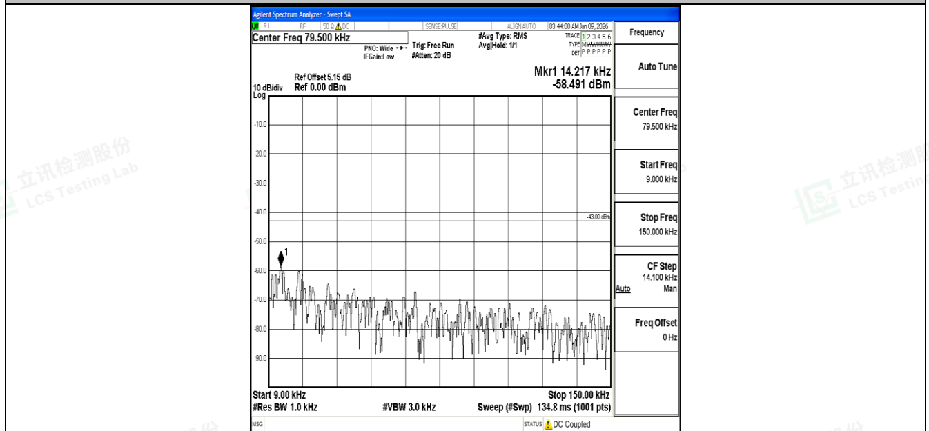
Band4_15MHz_QPSK_20175_1RB#0_0.009~0.15_0.009~0.15
