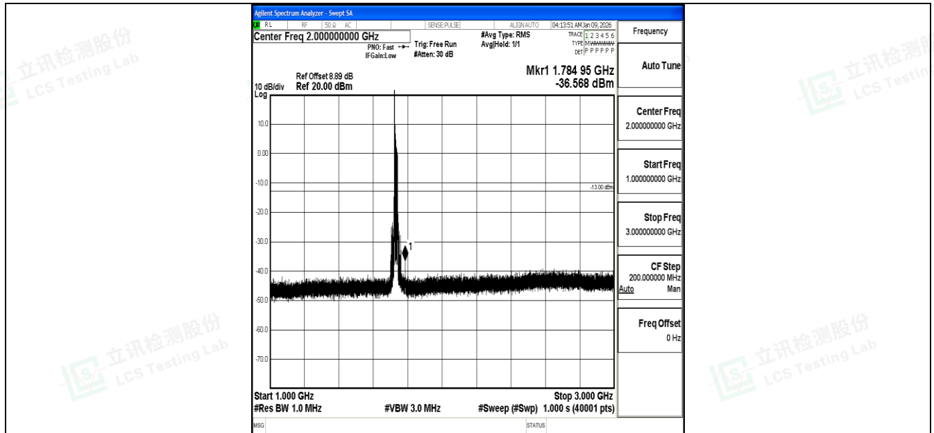
Band4_20MHz_QPSK_20175_1RB#0_1000~3000_1000~3000
