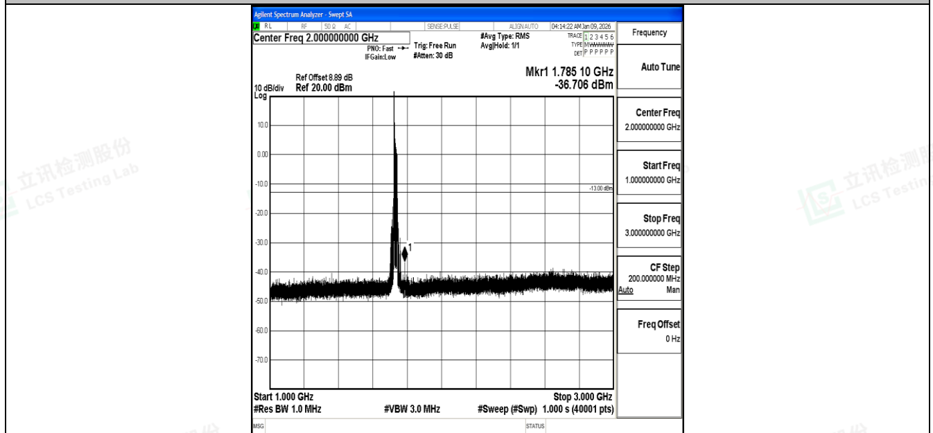
Band4_20MHz_16QAM_20175_1RB#0_1000~3000_1000~3000
