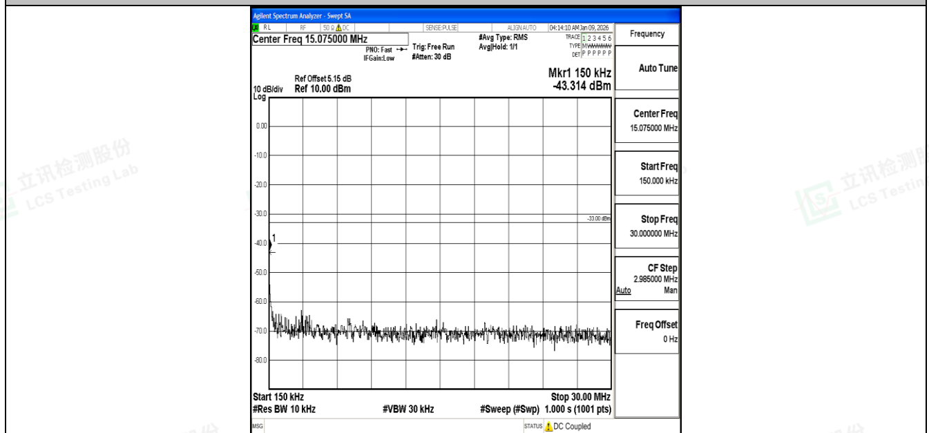
Band4_20MHz_16QAM_20175_1RB#0_0.15~30_0.15~30
