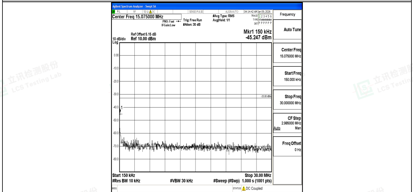
Band4_20MHz_QPSK_20300_1RB#0_0.15~30_0.15~30
