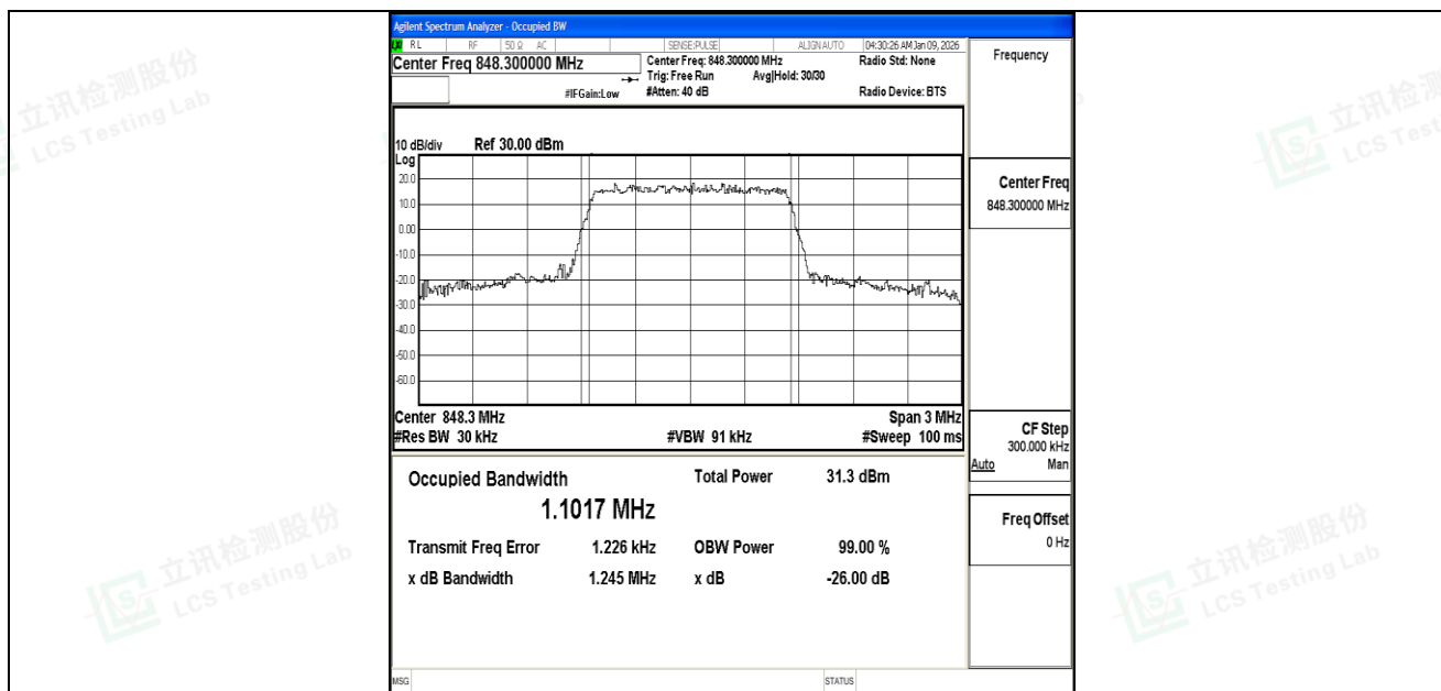
Band5-1.4MHz-QPSK-20643-6RB#0-PASS
