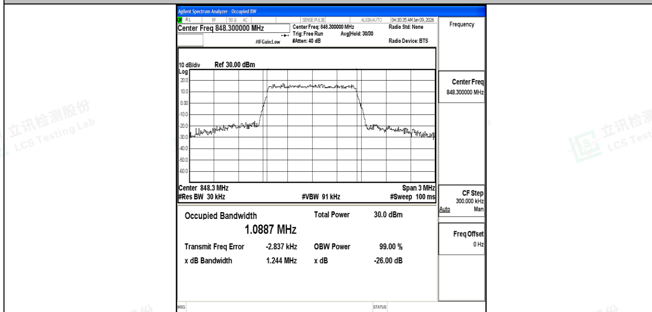
Band5-1.4MHz-16QAM-20643-6RB#0-PASS
