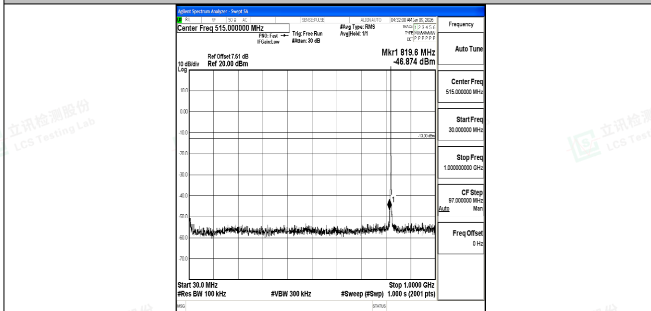
Band5_1.4MHz_16QAM_20407_1RB#0_30~1000_30~1000
