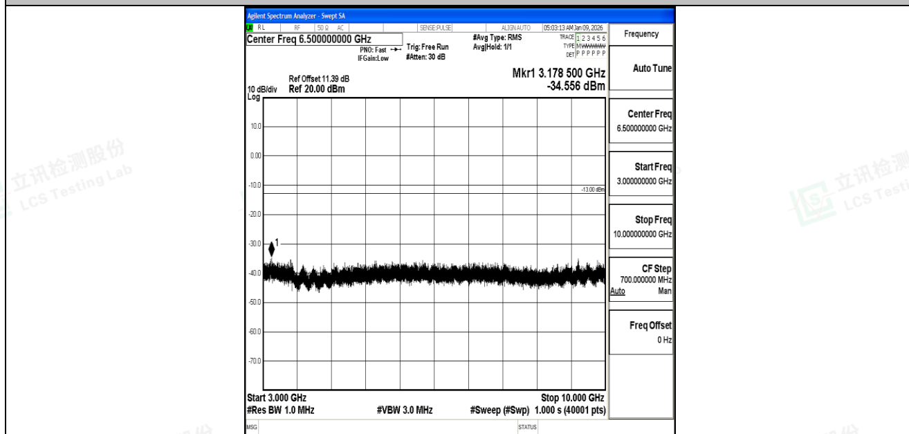
Band5_3MHz_16QAM_20525_1RB#0_3000~10000_3000~10000
