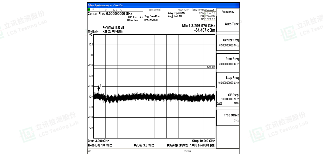
Band5_5MHz_QPSK_20425_1RB#0_3000~10000_3000~10000
