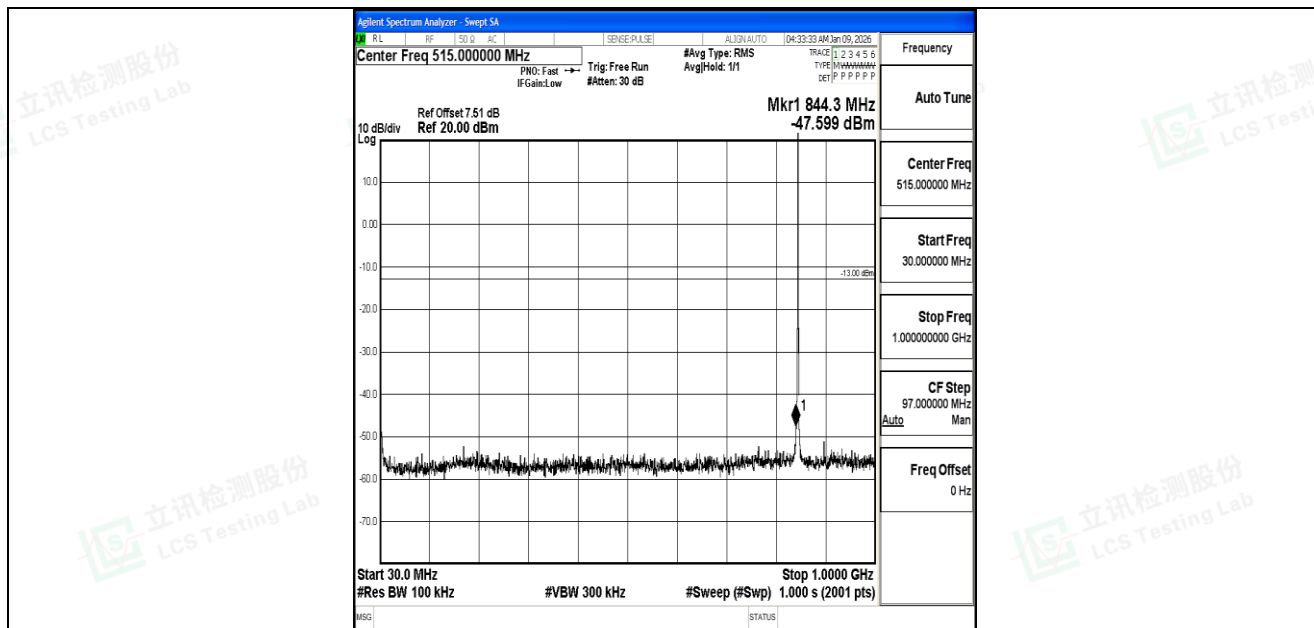
Band5_1.4MHz_QPSK_20643_1RB#0_30~1000_30~1000
