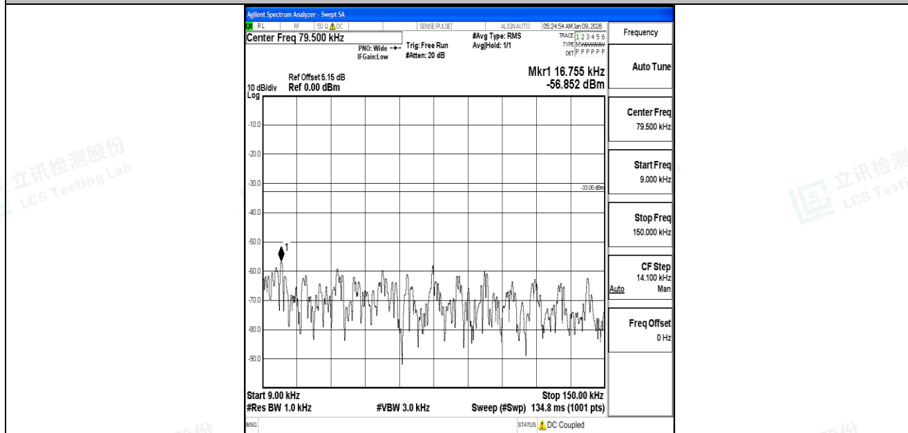
Band5_5MHz_16QAM_20425_1RB#0_0.009~0.15_0.009~0.15
