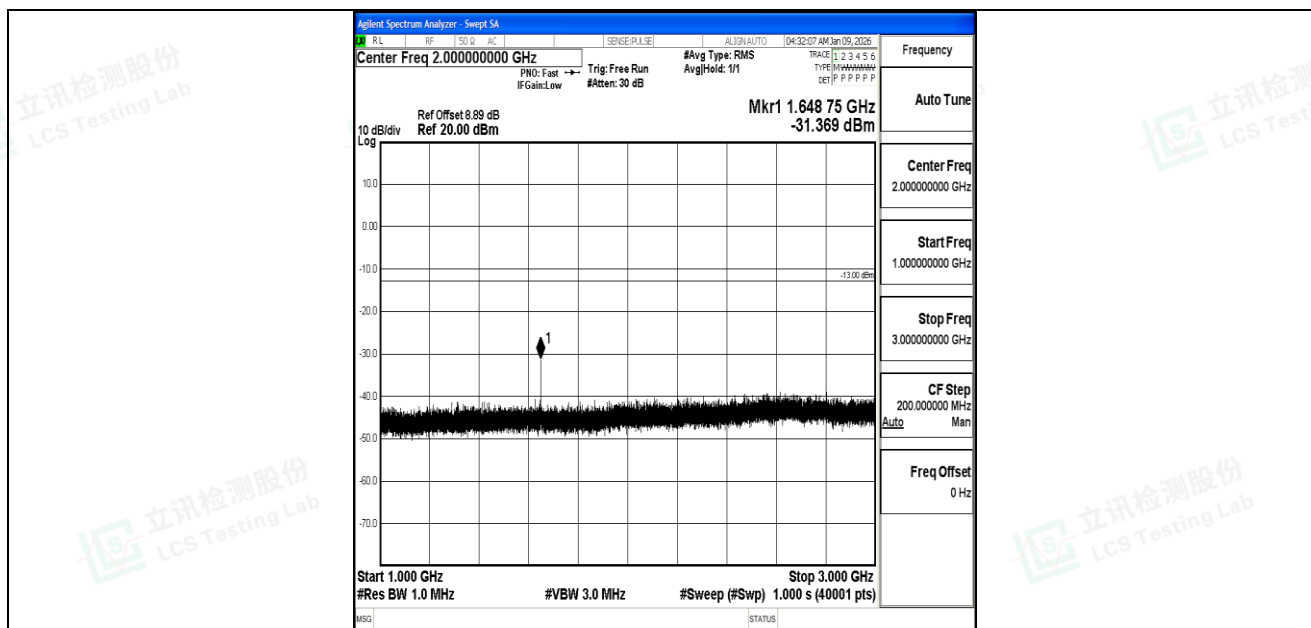
Band5_1.4MHz_16QAM_20407_1RB#0_1000~3000_1000~3000
