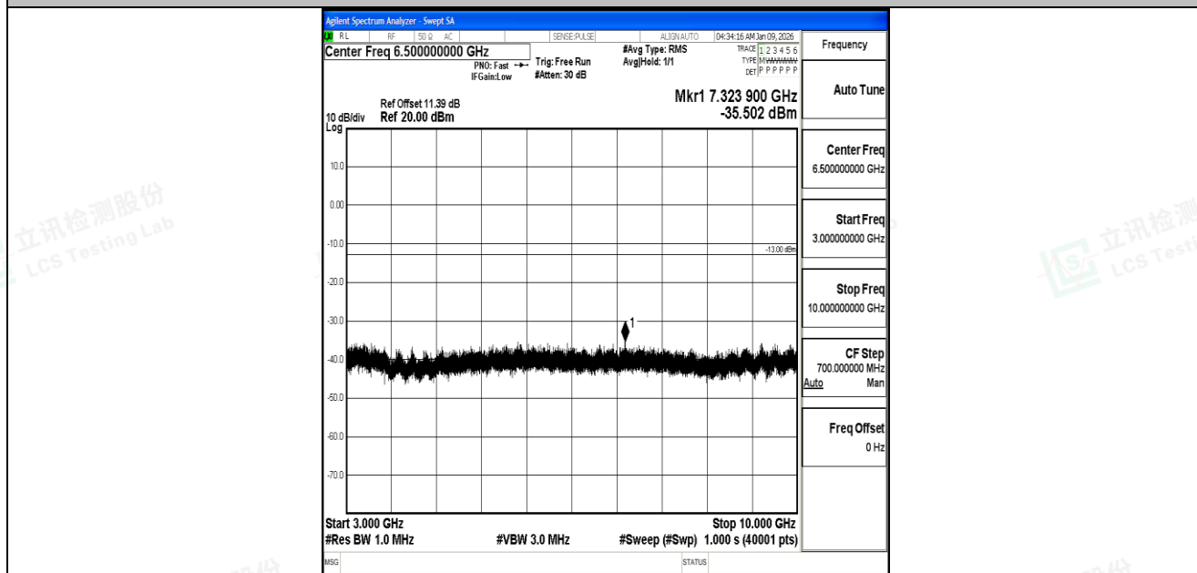
Band5_1.4MHz_16QAM_20643_1RB#0_3000~10000_3000~10000
