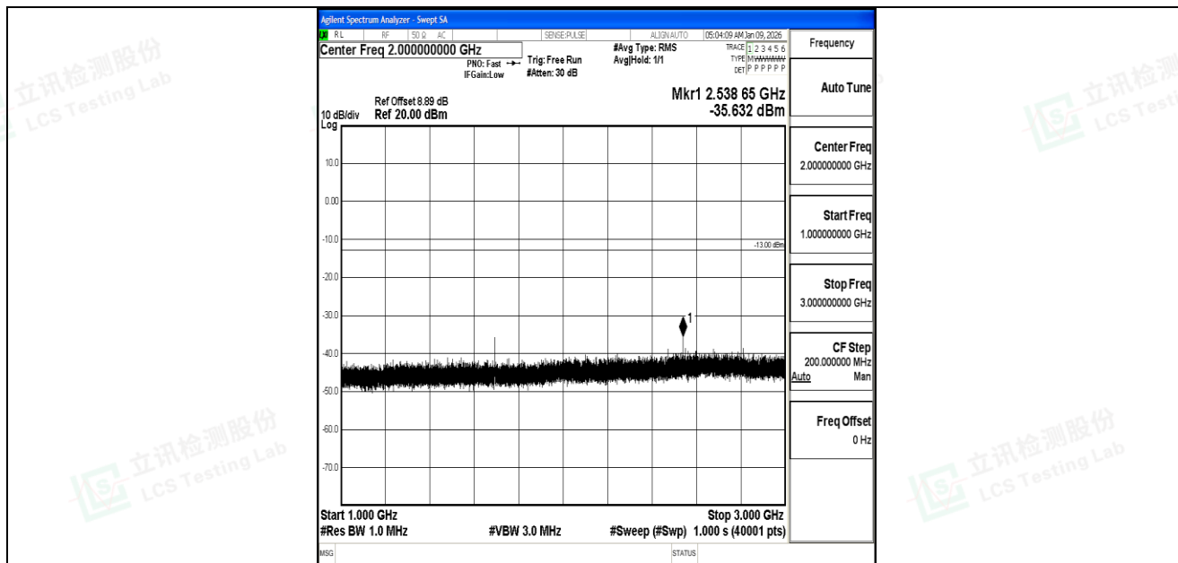
Band5_3MHz_16QAM_20635_1RB#0_1000~3000_1000~3000
