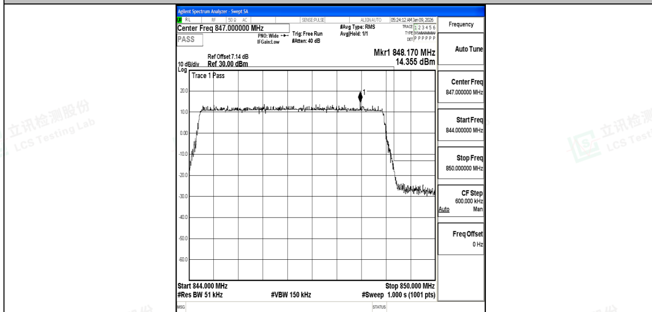
Band5_5MHz_16QAM_20625_25RB#0
