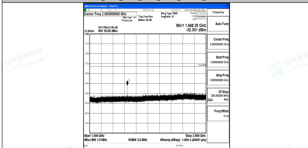
Band5_3MHz_QPSK_20415_1RB#0_1000~3000_1000~3000
