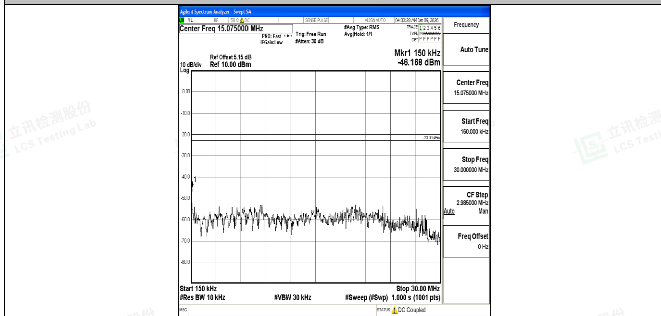
Band5_1.4MHz_QPSK_20643_1RB#0_0.15~30_0.15~30
