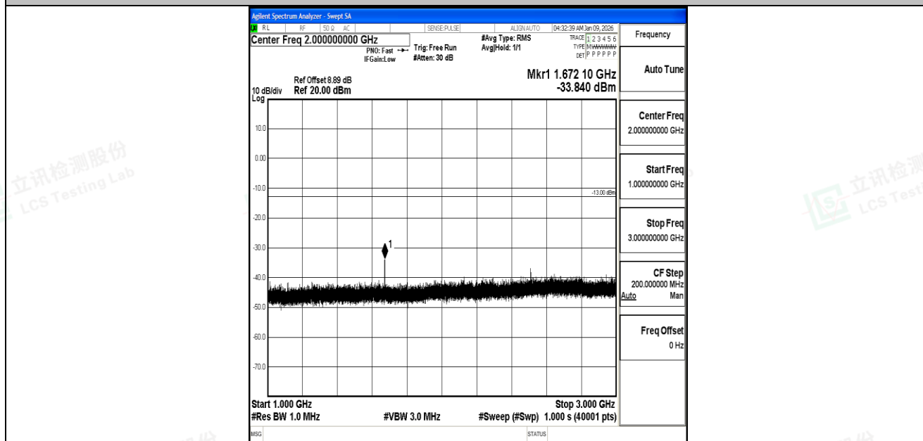
Band5_1.4MHz_QPSK_20525_1RB#0_1000~3000_1000~3000
