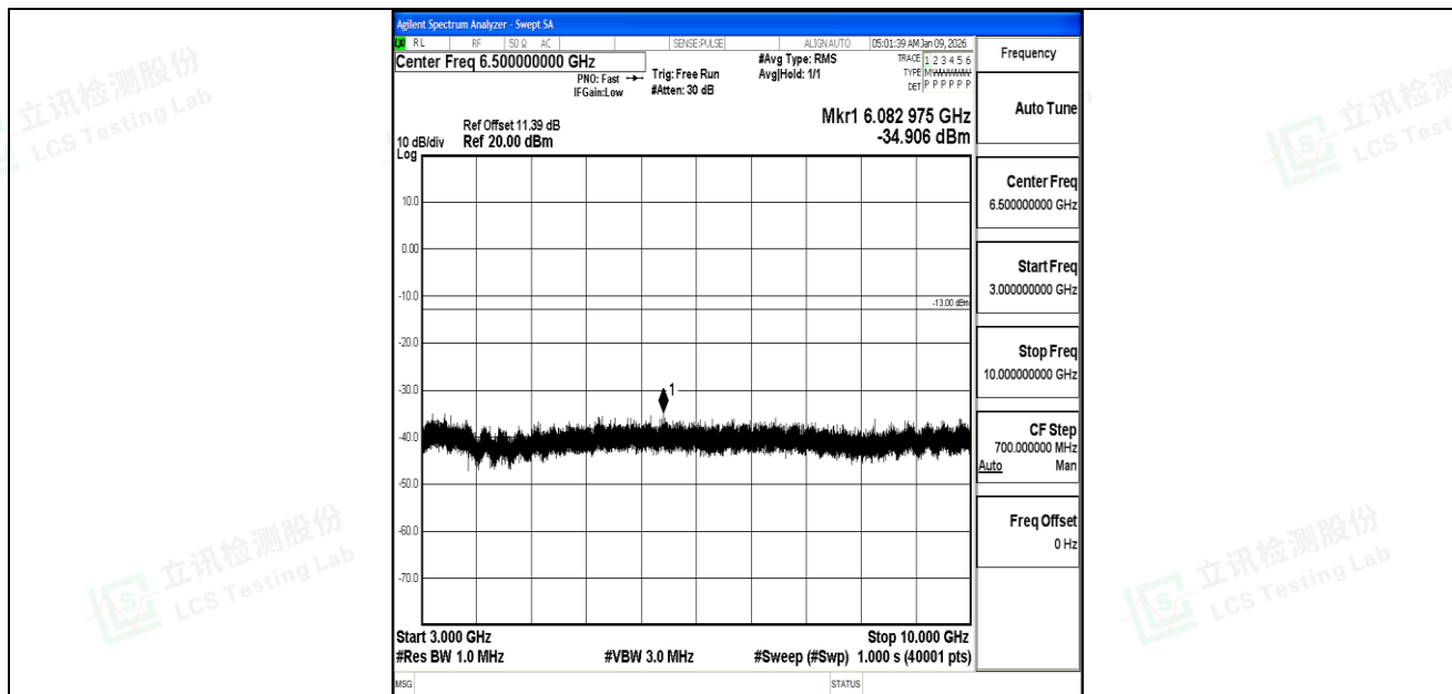
Band5_3MHz_QPSK_20415_1RB#0_3000~10000_3000~10000
