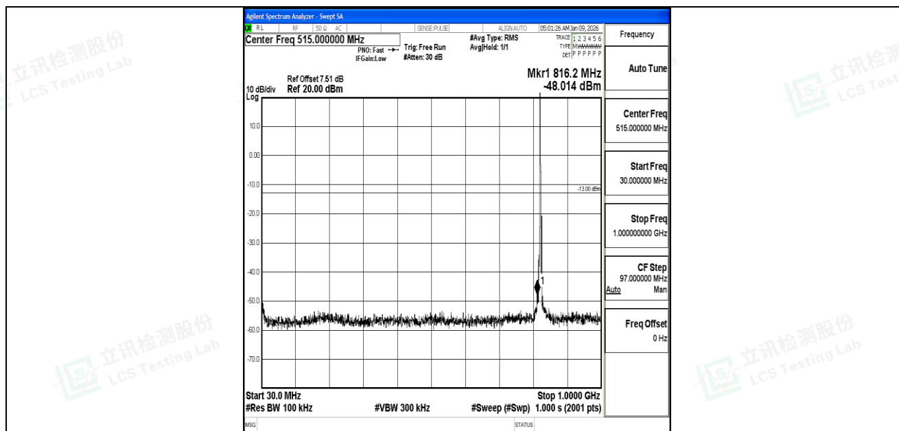
Band5_3MHz_QPSK_20415_1RB#0_30~1000_30~1000
