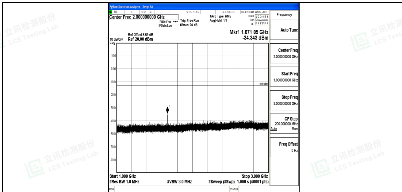
Band5_1.4MHz_16QAM_20525_1RB#0_1000~3000_1000~3000
