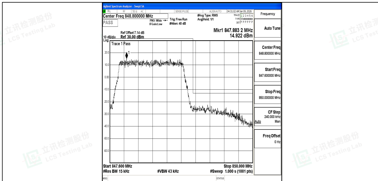
Band5_1.4MHz_QPSK_20643_6RB#0
