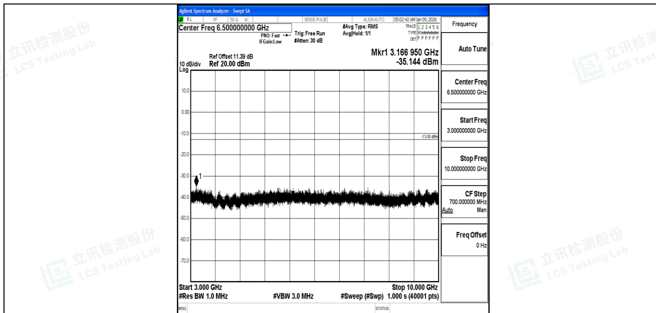
Band5_3MHz_QPSK_20525_1RB#0_3000~10000_3000~10000
