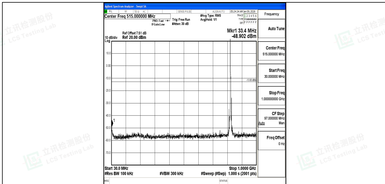
Band5_5MHz_QPSK_20425_1RB#0_30~1000_30~1000
