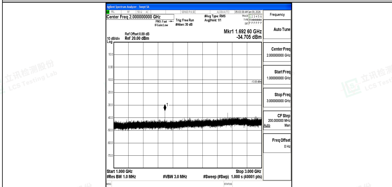
Band5_3MHz_QPSK_20635_1RB#0_1000~3000_1000~3000
