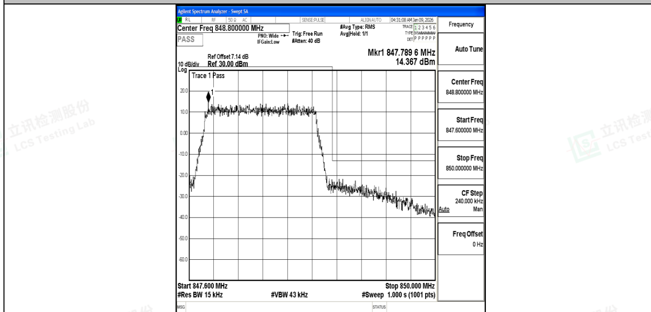
Band5_1.4MHz_16QAM_20643_6RB#0
