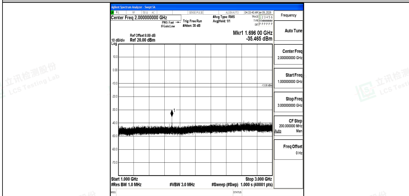
Band5_1.4MHz_QPSK_20643_1RB#0_1000~3000_1000~3000
