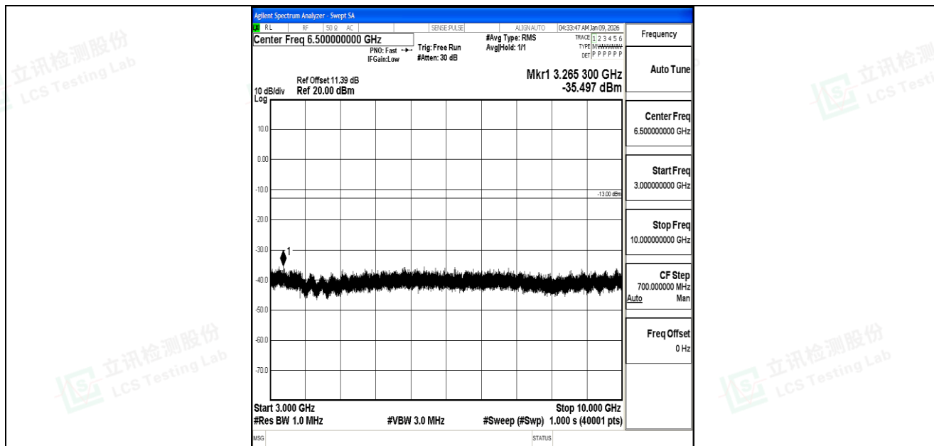
Band5_1.4MHz_QPSK_20643_1RB#0_3000~10000_3000~10000
