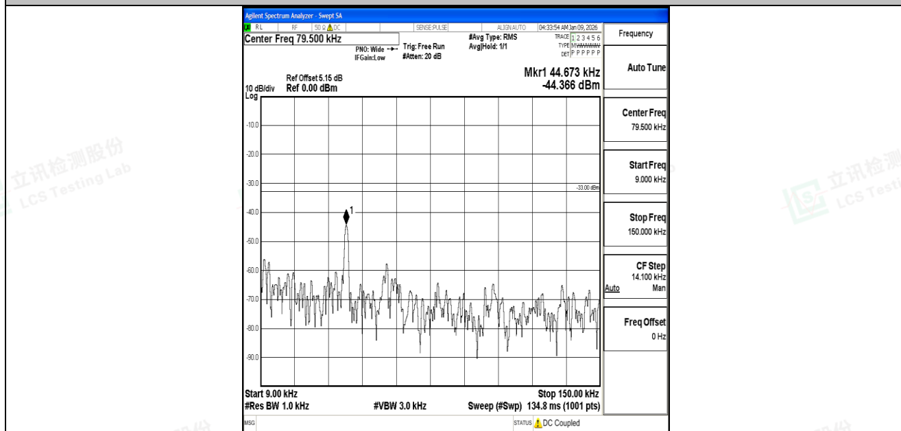
Band5_1.4MHz_16QAM_20643_1RB#0_0.009~0.15_0.009~0.15
