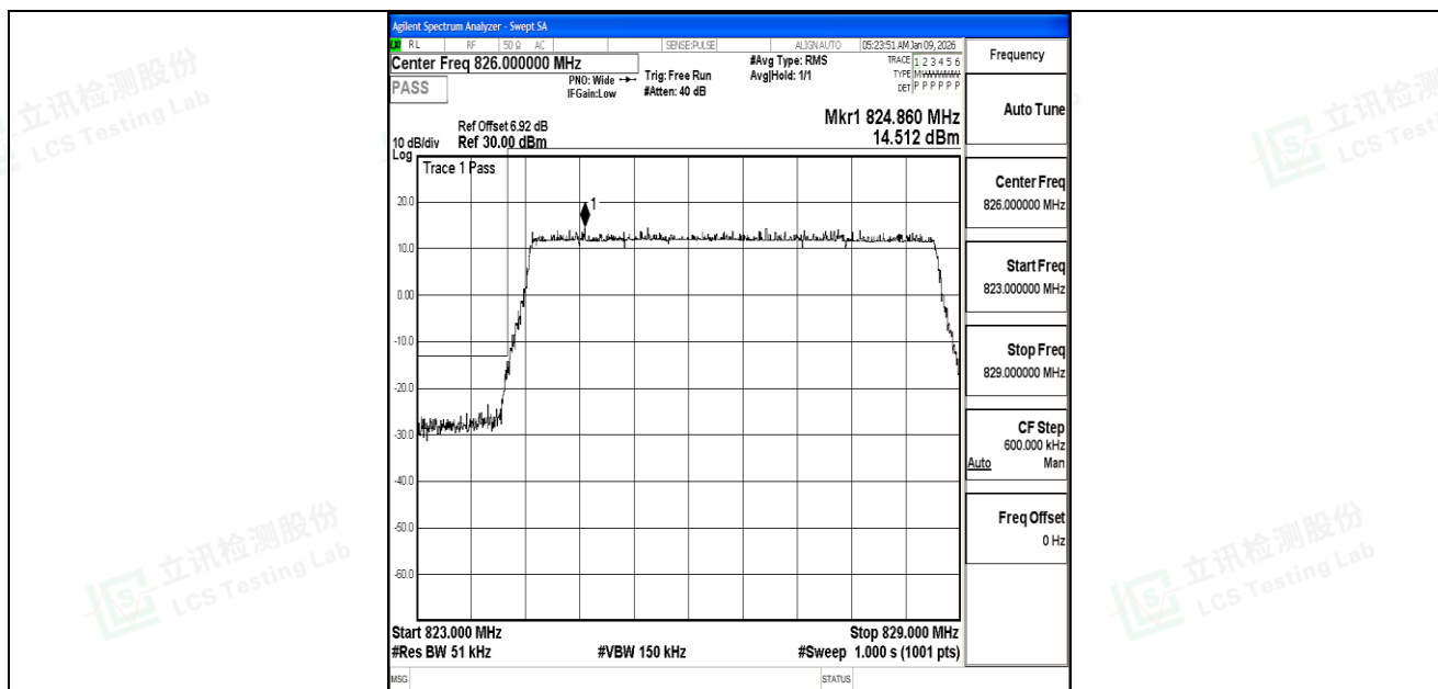
Band5_5MHz_QPSK_20425_25RB#0
