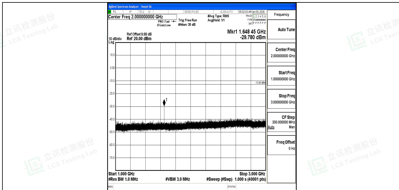
Band5_3MHz_16QAM_20415_1RB#0_1000~3000_1000~3000
