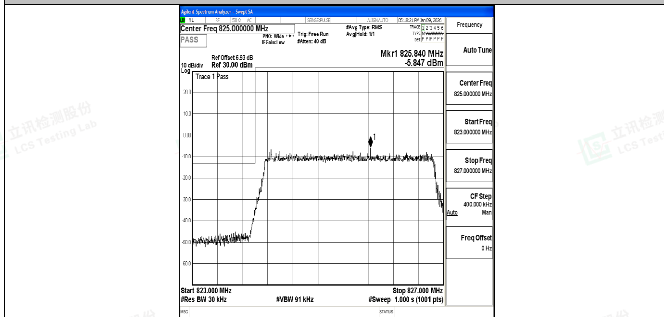
Band5_3MHz_QPSK_20415_15RB#0
