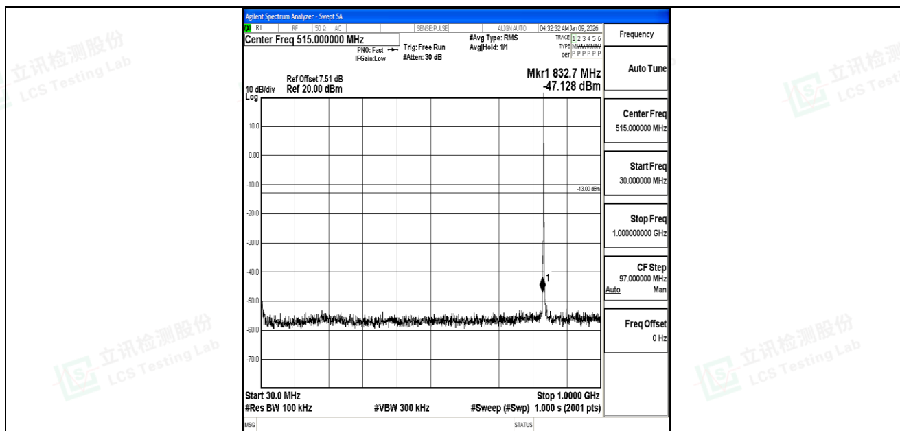
Band5_1.4MHz_QPSK_20525_1RB#0_30~1000_30~1000
