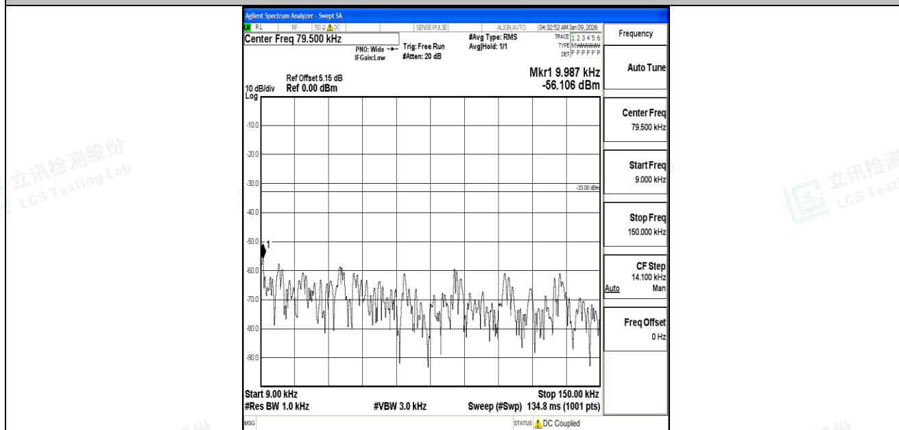
Band5_1.4MHz_16QAM_20525_1RB#0_0.009~0.15_0.009~0.15
