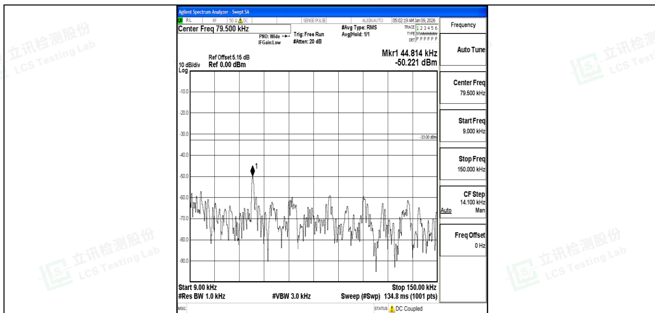
Band5_3MHz_QPSK_20525_1RB#0_0.009~0.15_0.009~0.15
