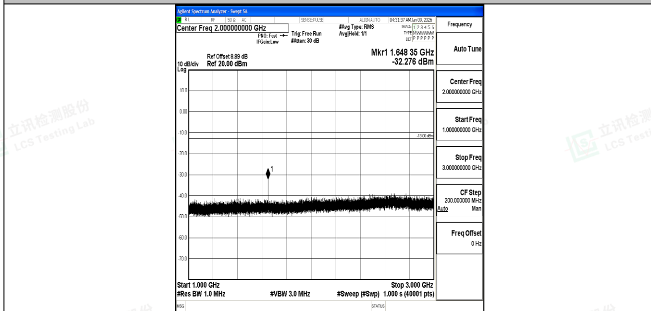
Band5_1.4MHz_QPSK_20407_1RB#0_1000~3000_1000~3000
