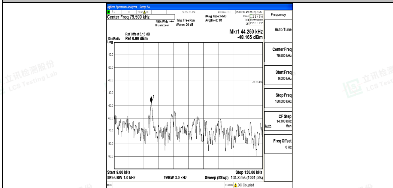
Band5_3MHz_16QAM_20415_1RB#0_0.009~0.15_0.009~0.15
