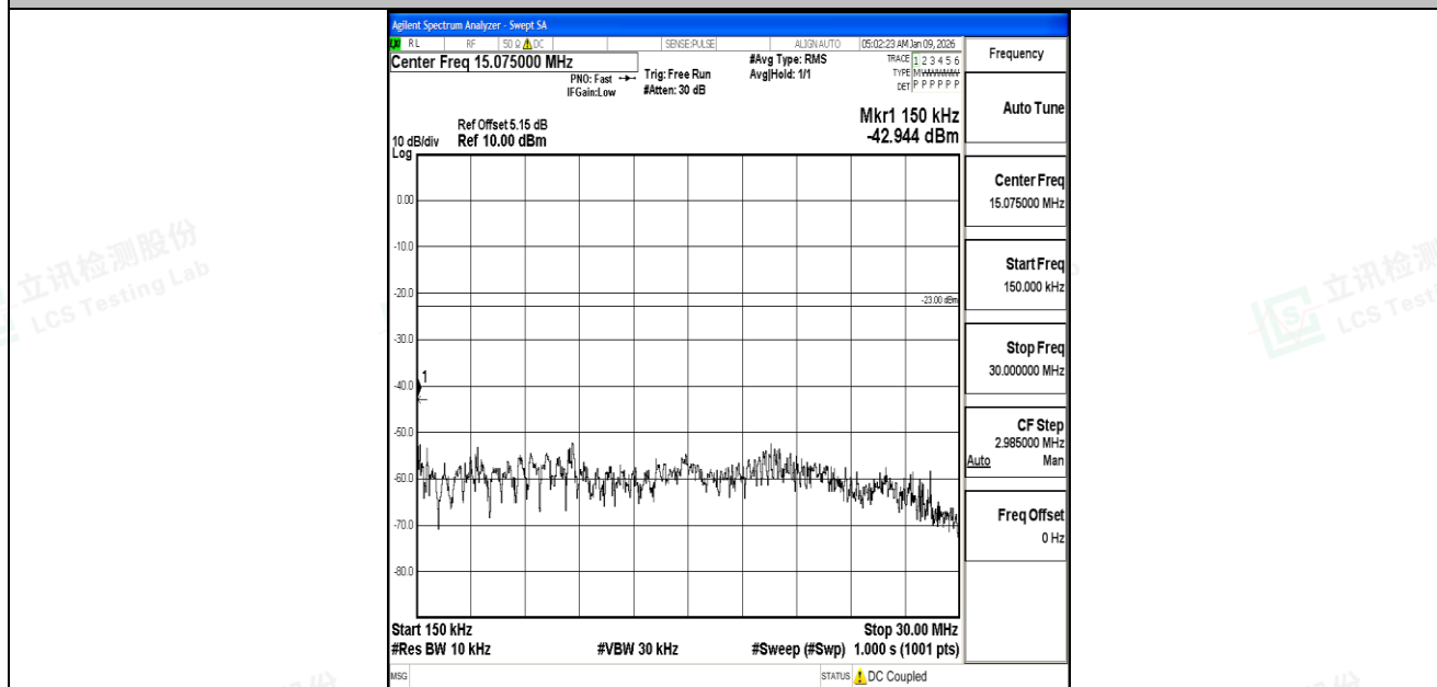
Band5_3MHz_QPSK_20525_1RB#0_0.15~30_0.15~30
