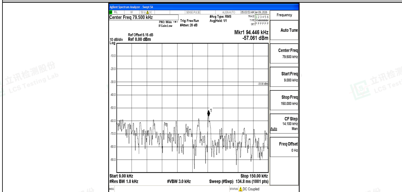
Band5_3MHz_16QAM_20635_1RB#0_0.009~0.15_0.009~0.15
