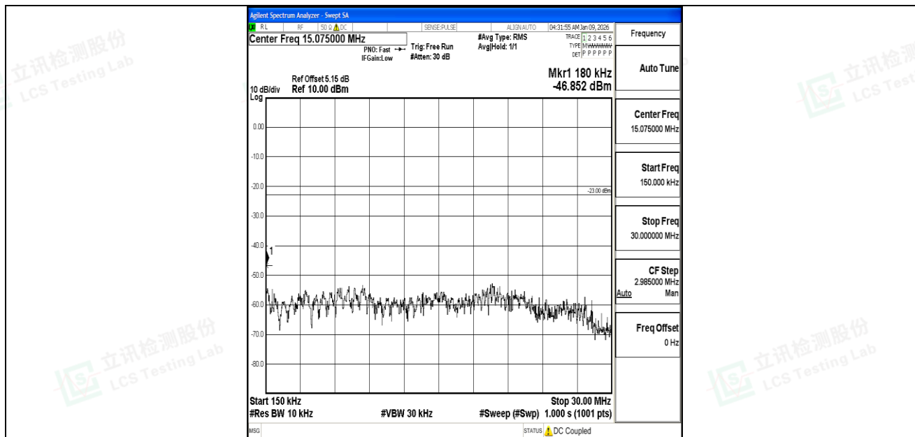
Band5_1.4MHz_16QAM_20407_1RB#0_0.15~30_0.15~30
