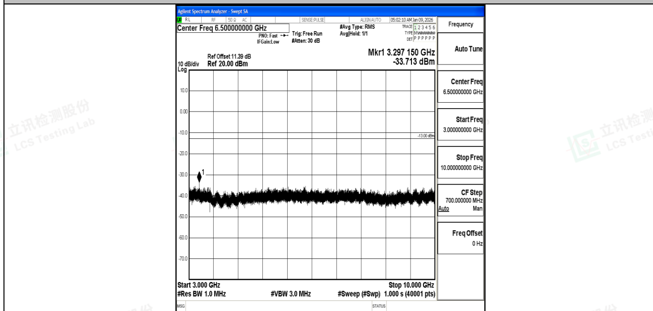
Band5_3MHz_16QAM_20415_1RB#0_3000~10000_3000~10000
