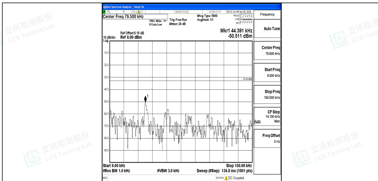
Band5_3MHz_QPSK_20415_1RB#0_0.009~0.15_0.009~0.15
