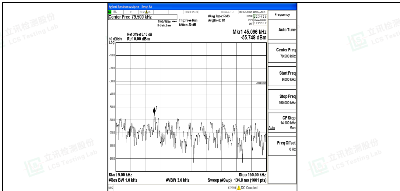
Band5_10MHz_QPSK_20525_1RB#0_0.009~0.15_0.009~0.15
