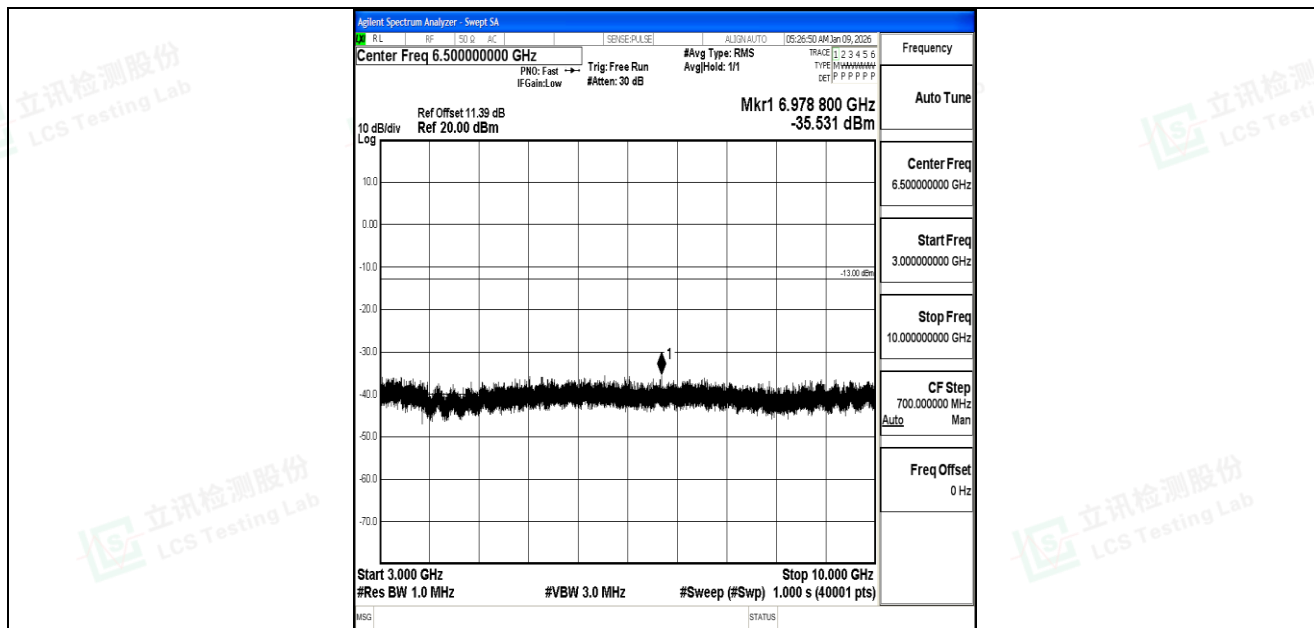
Band5_5MHz_QPSK_20625_1RB#0_3000~10000_3000~10000
