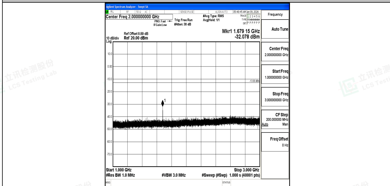
Band5_10MHz_QPSK_20600_1RB#0_1000~3000_1000~3000
