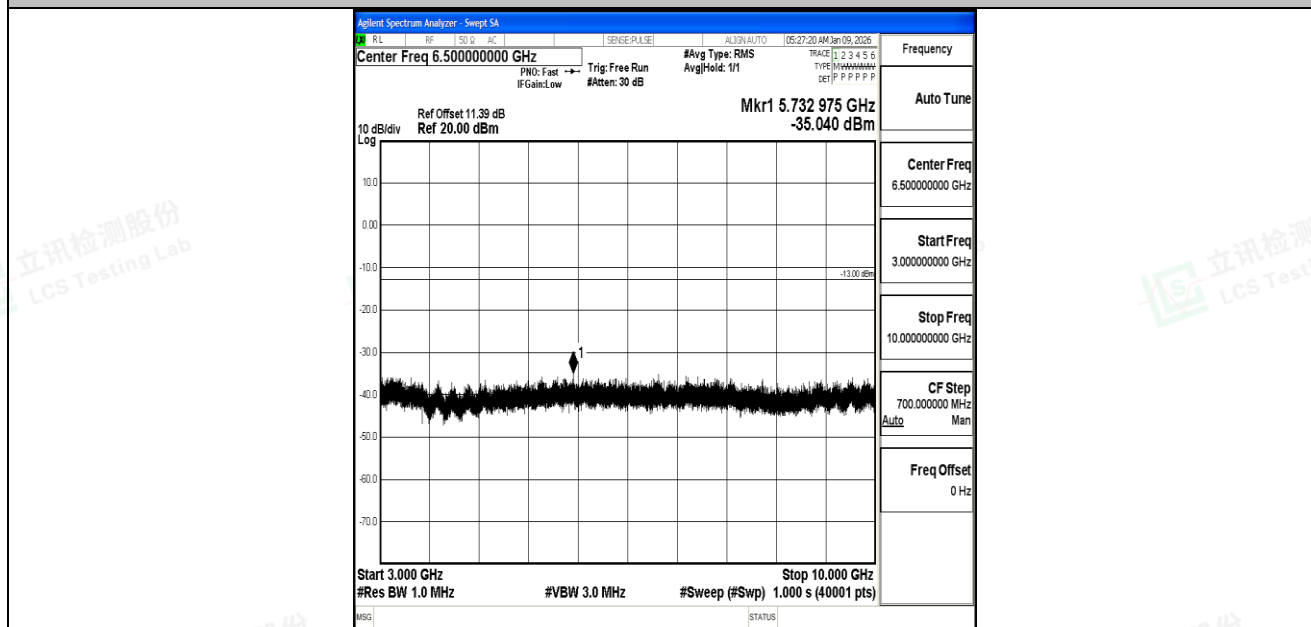
Band5_5MHz_16QAM_20625_1RB#0_3000~10000_3000~10000
