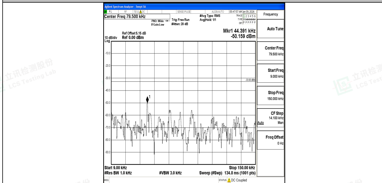
Band5_10MHz_16QAM_20525_1RB#0_0.009~0.15_0.009~0.15
