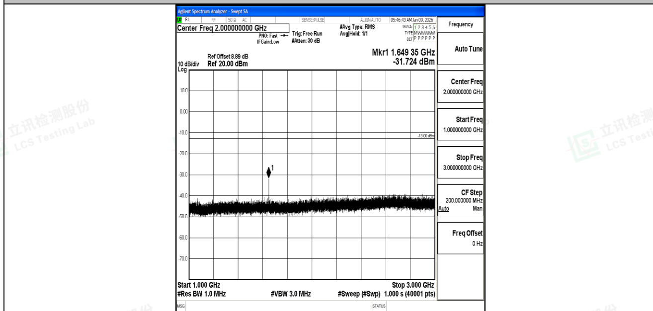
Band5_10MHz_QPSK_20450_1RB#0_1000~3000_1000~3000
