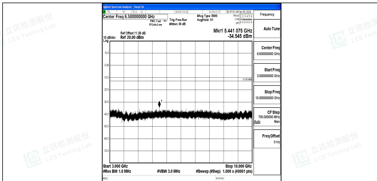
Band5_10MHz_QPSK_20525_1RB#0_3000~10000_3000~10000
