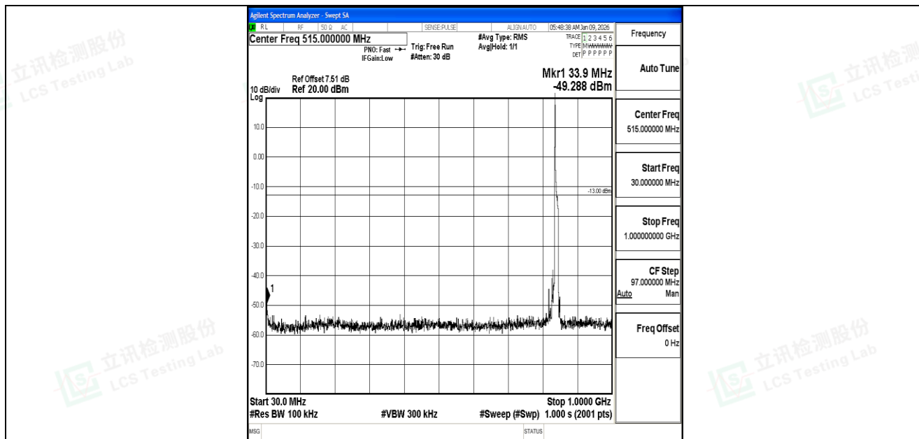
Band5_10MHz_QPSK_20600_1RB#0_30~1000_30~1000
