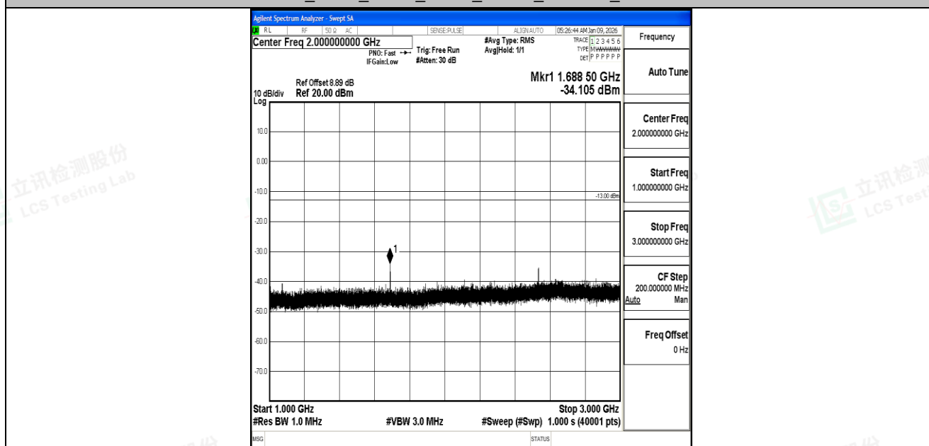
Band5_5MHz_QPSK_20625_1RB#0_1000~3000_1000~3000
