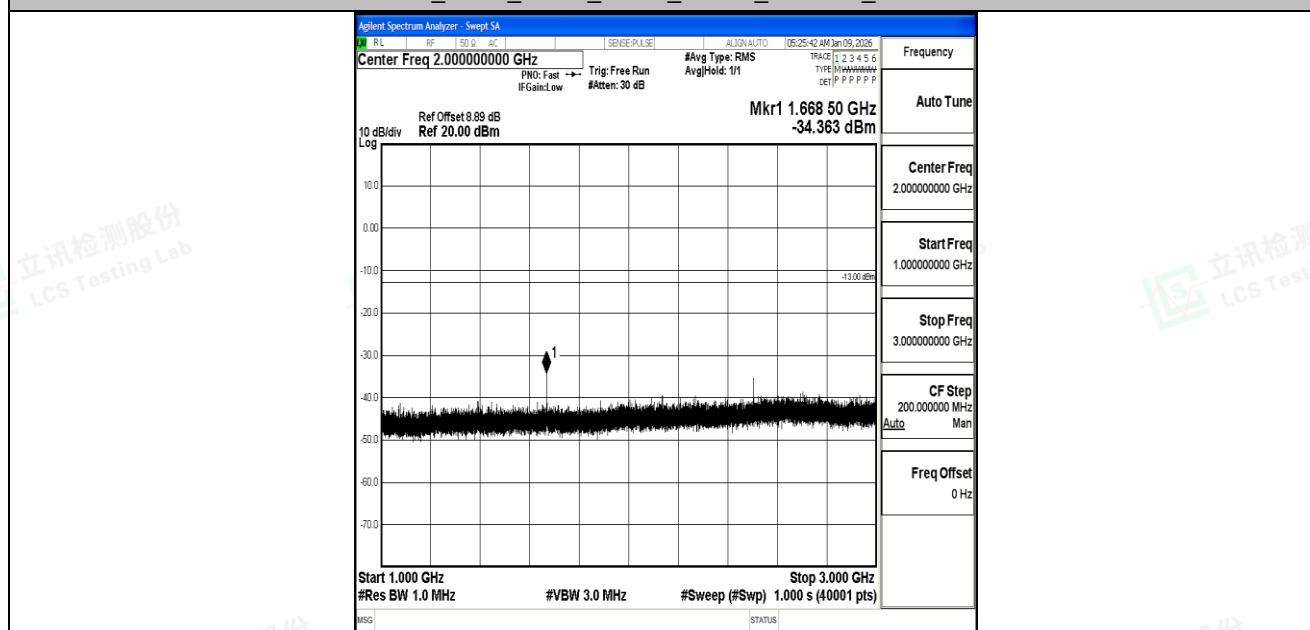
Band5_5MHz_QPSK_20525_1RB#0_1000~3000_1000~3000
