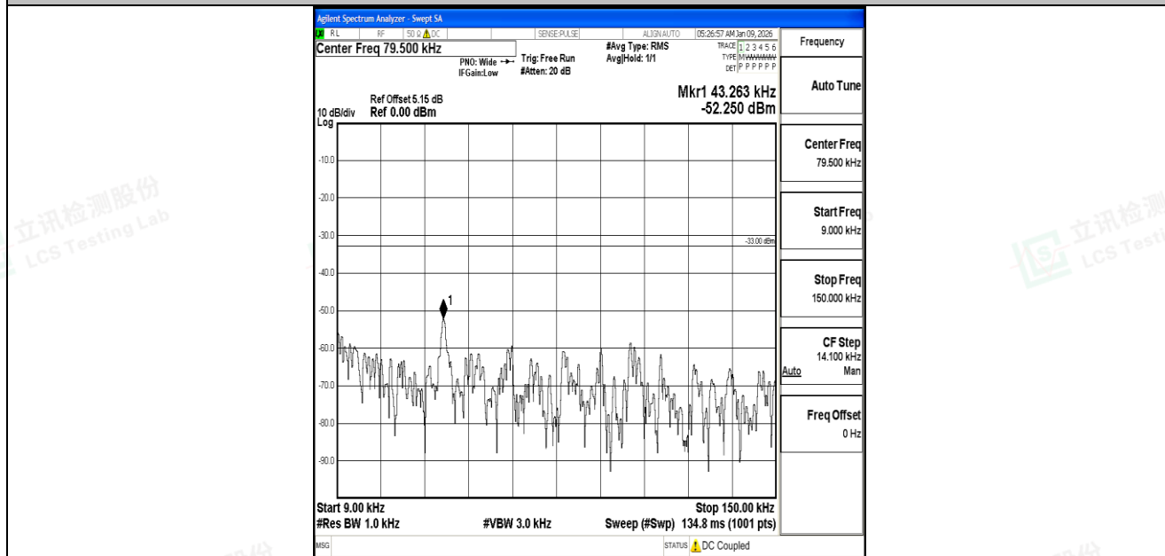
Band5_5MHz_16QAM_20625_1RB#0_0.009~0.15_0.009~0.15
