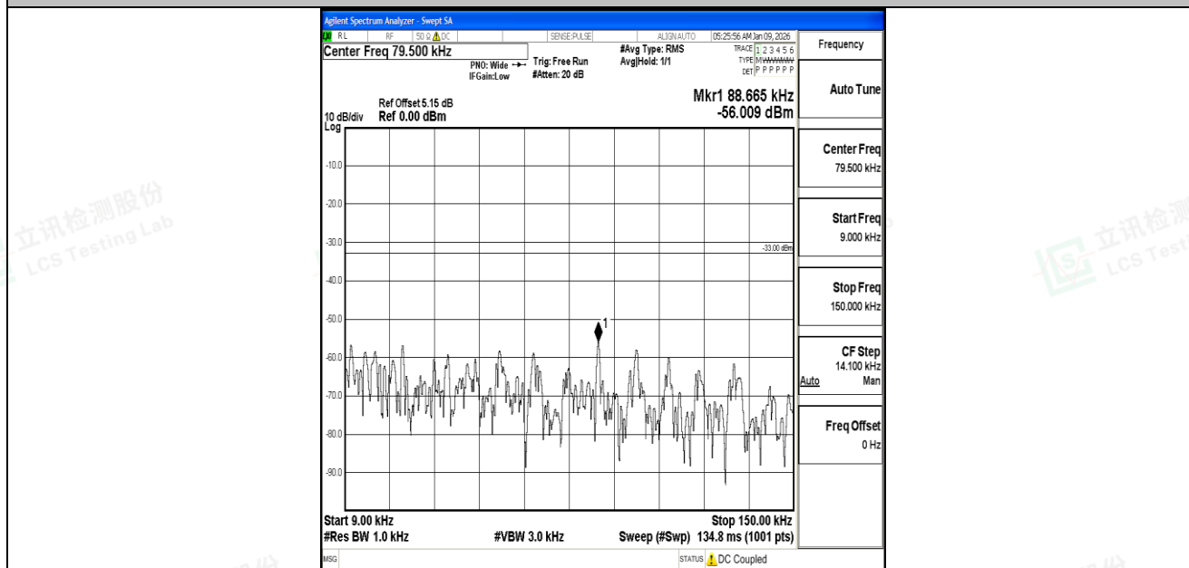
Band5_5MHz_16QAM_20525_1RB#0_0.009~0.15_0.009~0.15
