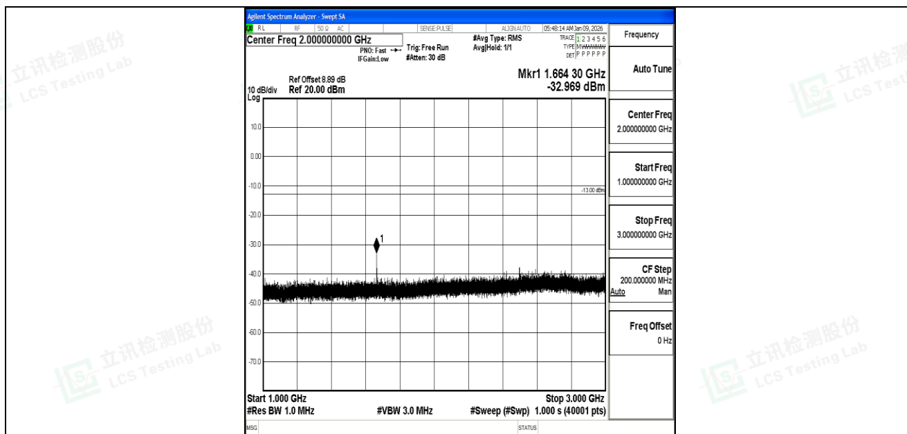
Band5_10MHz_16QAM_20525_1RB#0_1000~3000_1000~3000
