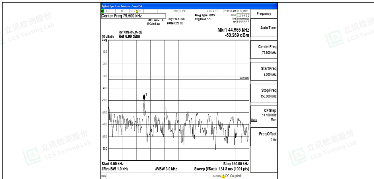
Band5_10MHz_QPSK_20450_1RB#0_0.009~0.15_0.009~0.15
