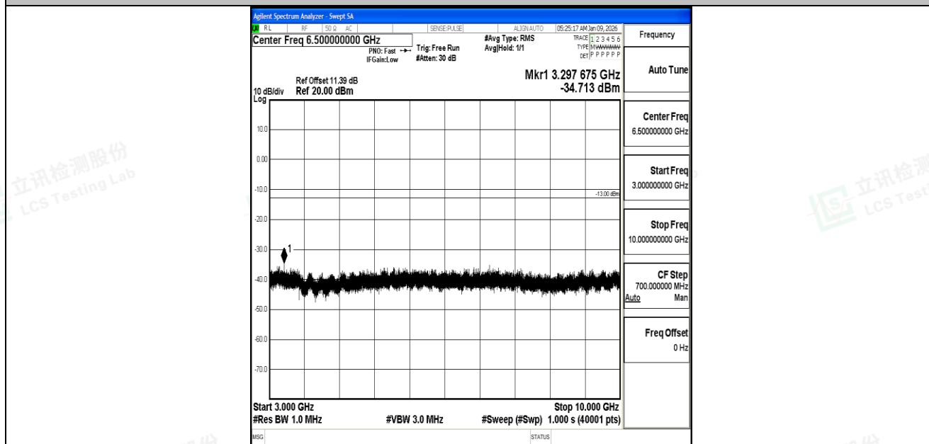
Band5_5MHz_16QAM_20425_1RB#0_3000~10000_3000~10000
