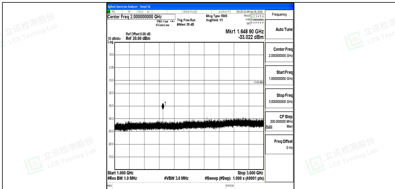
Band5_5MHz_16QAM_20425_1RB#0_1000~3000_1000~3000
