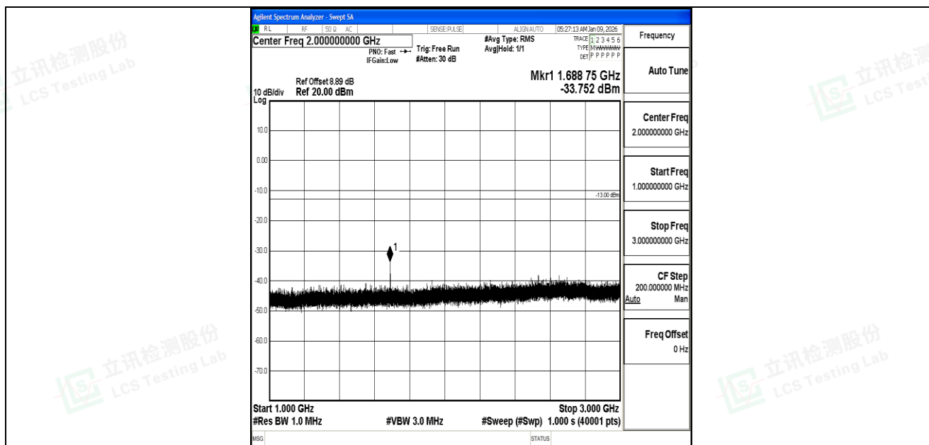
Band5_5MHz_16QAM_20625_1RB#0_1000~3000_1000~3000
