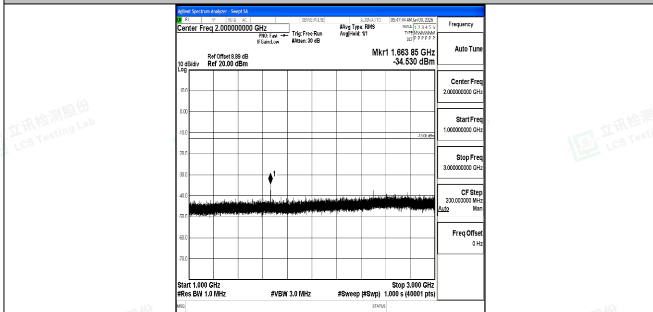
Band5_10MHz_QPSK_20525_1RB#0_1000~3000_1000~3000
