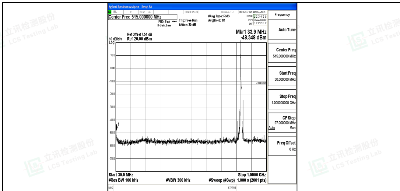
Band5_10MHz_QPSK_20525_1RB#0_30~1000_30~1000
