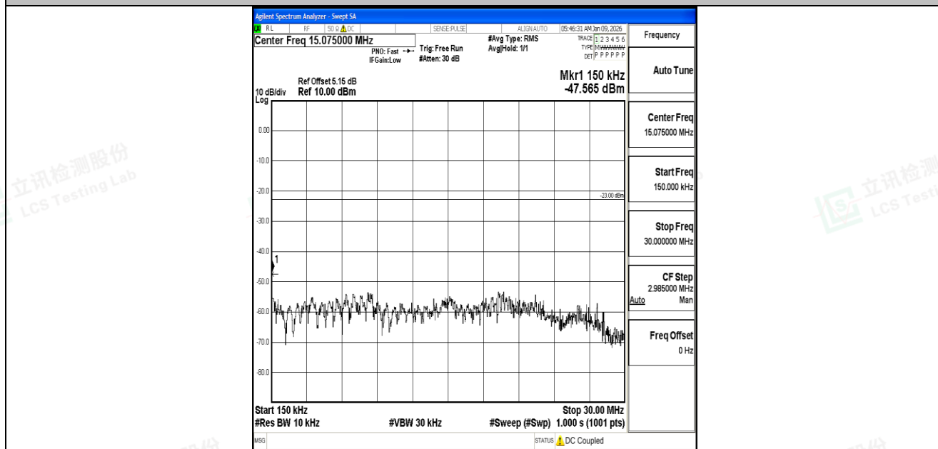
Band5_10MHz_QPSK_20450_1RB#0_0.15~30_0.15~30
