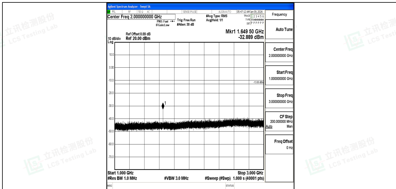
Band5_10MHz_16QAM_20450_1RB#0_1000~3000_1000~3000
