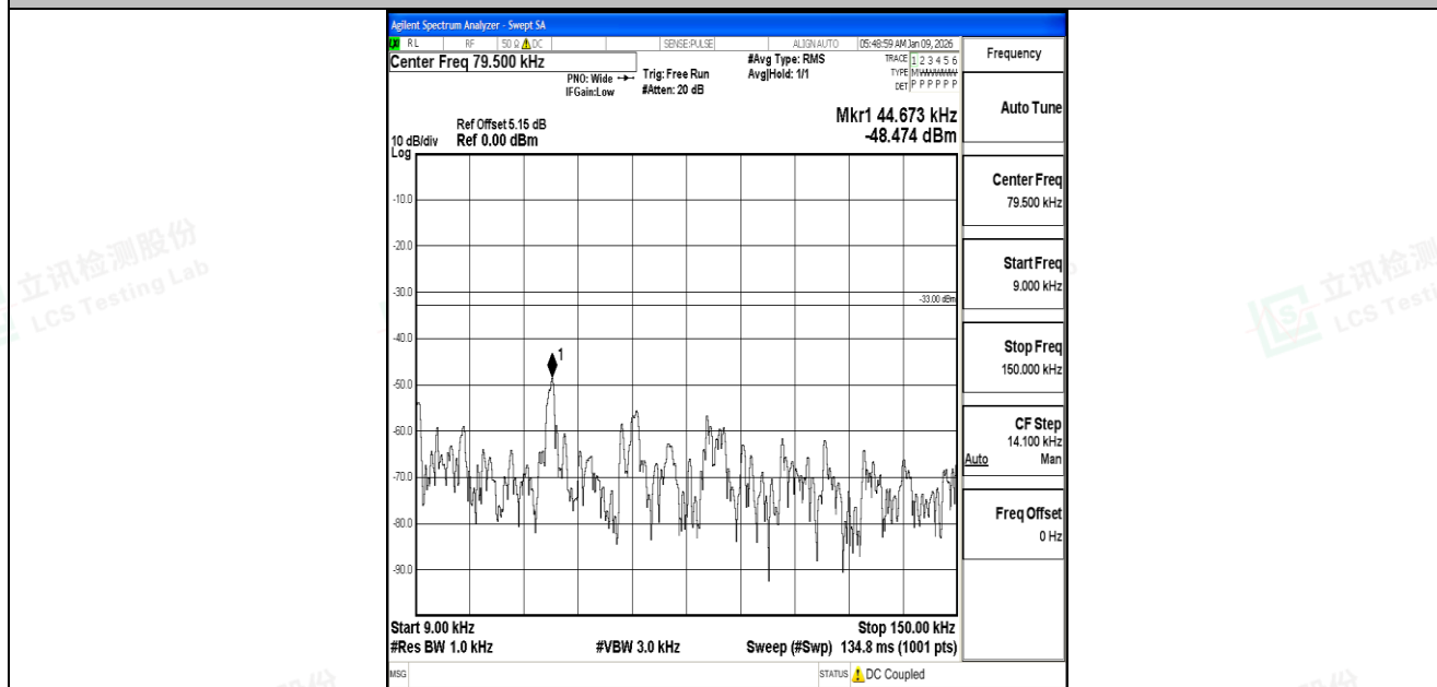
Band5_10MHz_16QAM_20600_1RB#0_0.009~0.15_0.009~0.15
