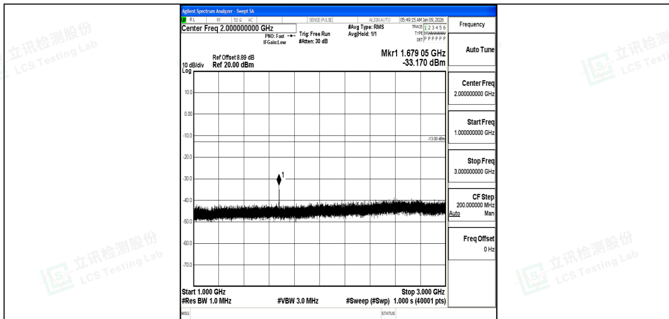
Band5_10MHz_16QAM_20600_1RB#0_1000~3000_1000~3000
