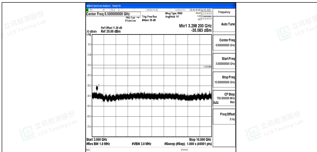
Band5_10MHz_QPSK_20450_1RB#0_3000~10000_3000~10000
