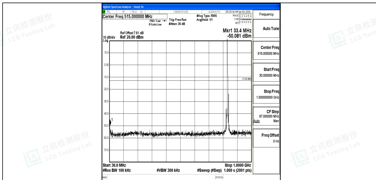
Band5_5MHz_QPSK_20525_1RB#0_30~1000_30~1000
