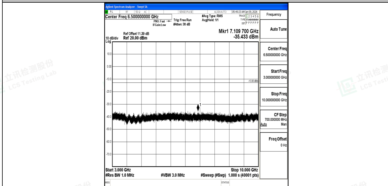
Band5_10MHz_16QAM_20600_1RB#0_3000~10000_3000~10000
