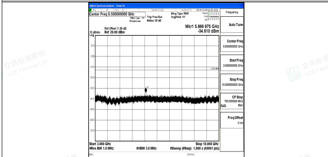
Band5_5MHz_16QAM_20525_1RB#0_3000~10000_3000~10000
