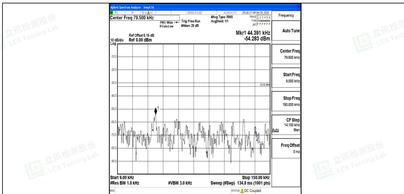
Band5_5MHz_QPSK_20625_1RB#0_0.009~0.15_0.009~0.15
