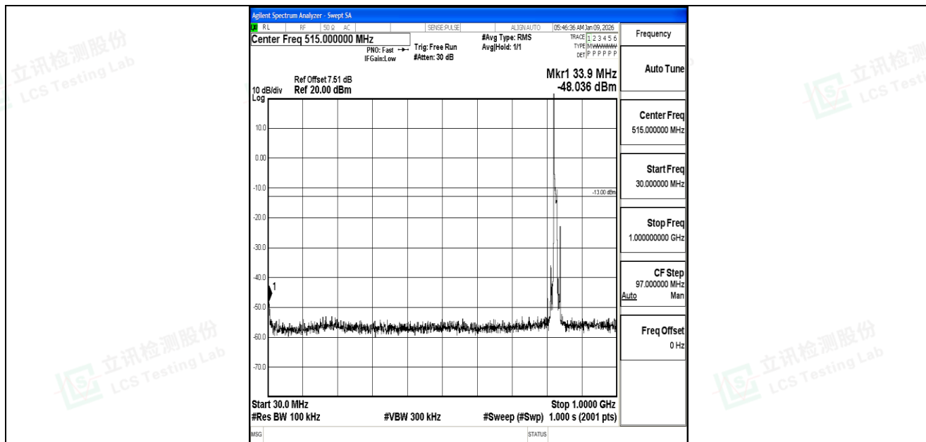
Band5_10MHz_QPSK_20450_1RB#0_30~1000_30~1000
