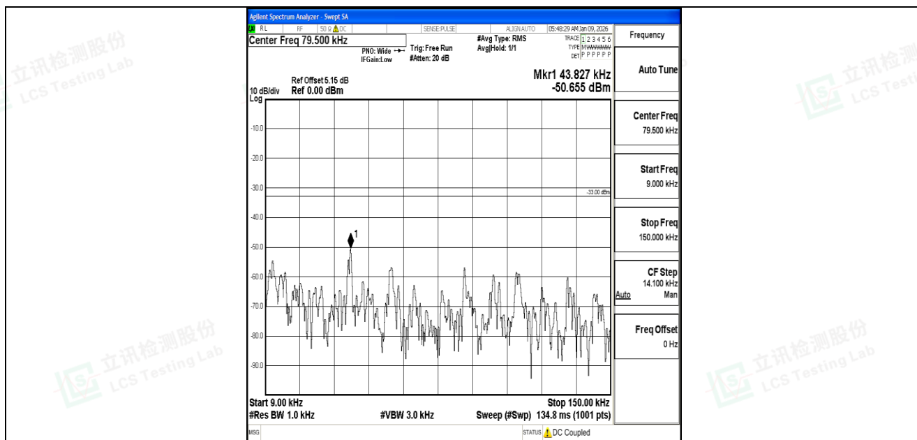
Band5_10MHz_QPSK_20600_1RB#0_0.009~0.15_0.009~0.15
