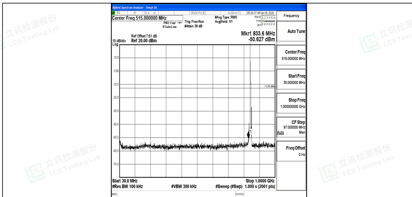
Band5_5MHz_QPSK_20625_1RB#0_30~1000_30~1000
