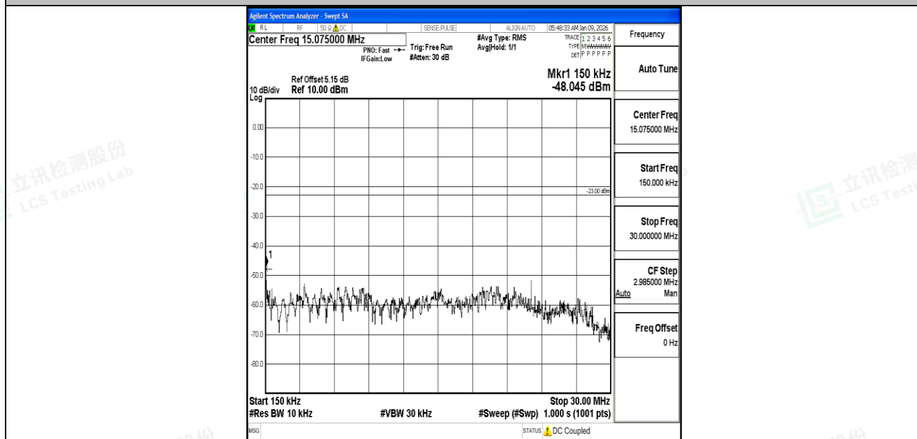
Band5_10MHz_QPSK_20600_1RB#0_0.15~30_0.15~30
