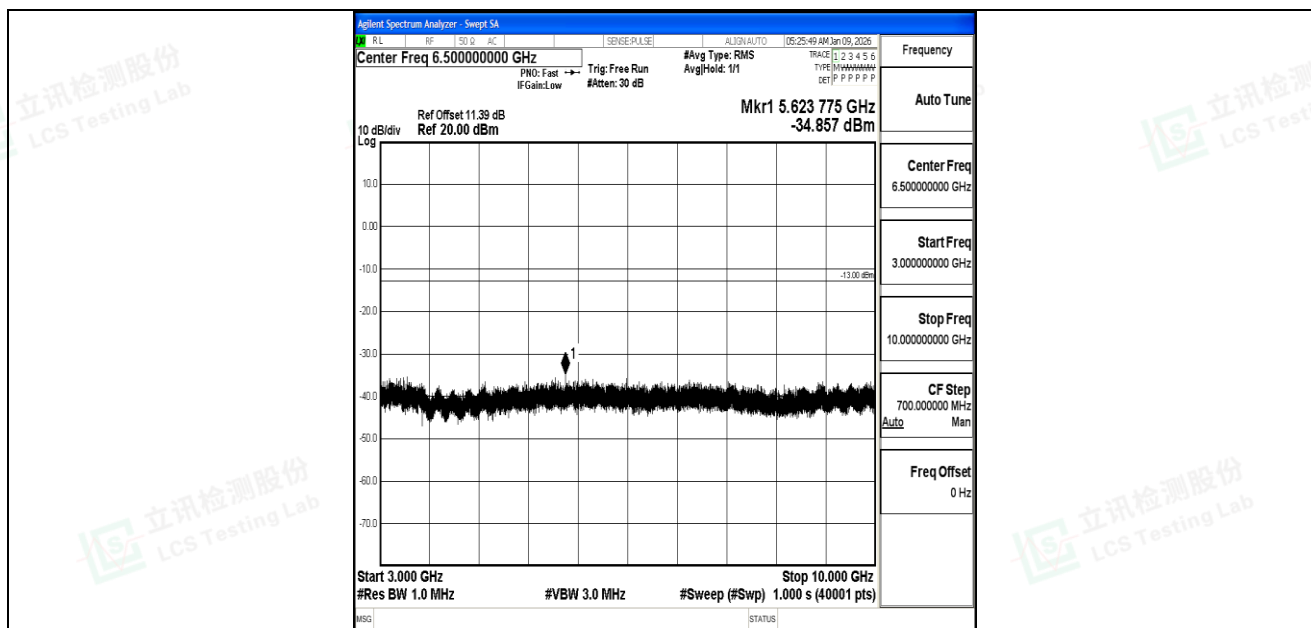
Band5_5MHz_QPSK_20525_1RB#0_3000~10000_3000~10000
