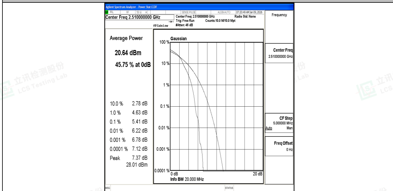
Band7-20MHz-16QAM-20850-1RB#0-PASS
