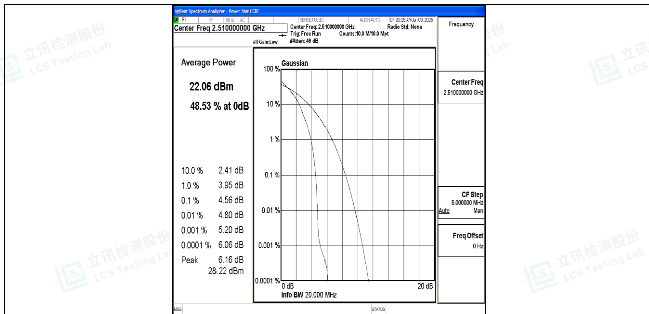
Band7-20MHz-QPSK-20850-1RB#0-PASS
