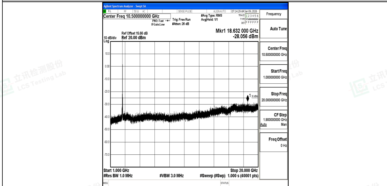
Band7_20MHz_QPSK_21350_1RB#0_1000~20000_1000~20000
