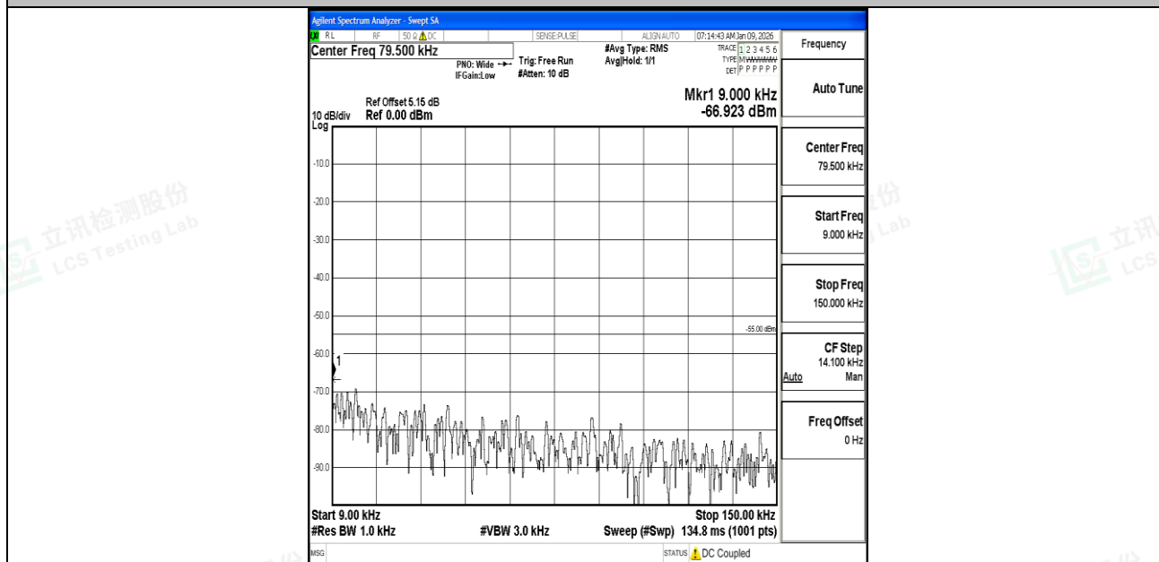
Band7_20MHz_16QAM_21350_1RB#0_0.009~0.15_0.009~0.15
