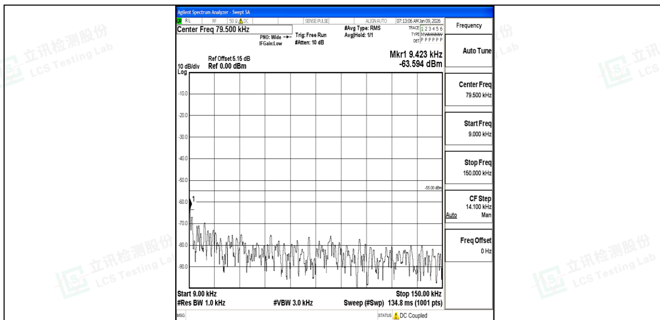
Band7_20MHz_QPSK_21100_1RB#0_0.009~0.15_0.009~0.15
