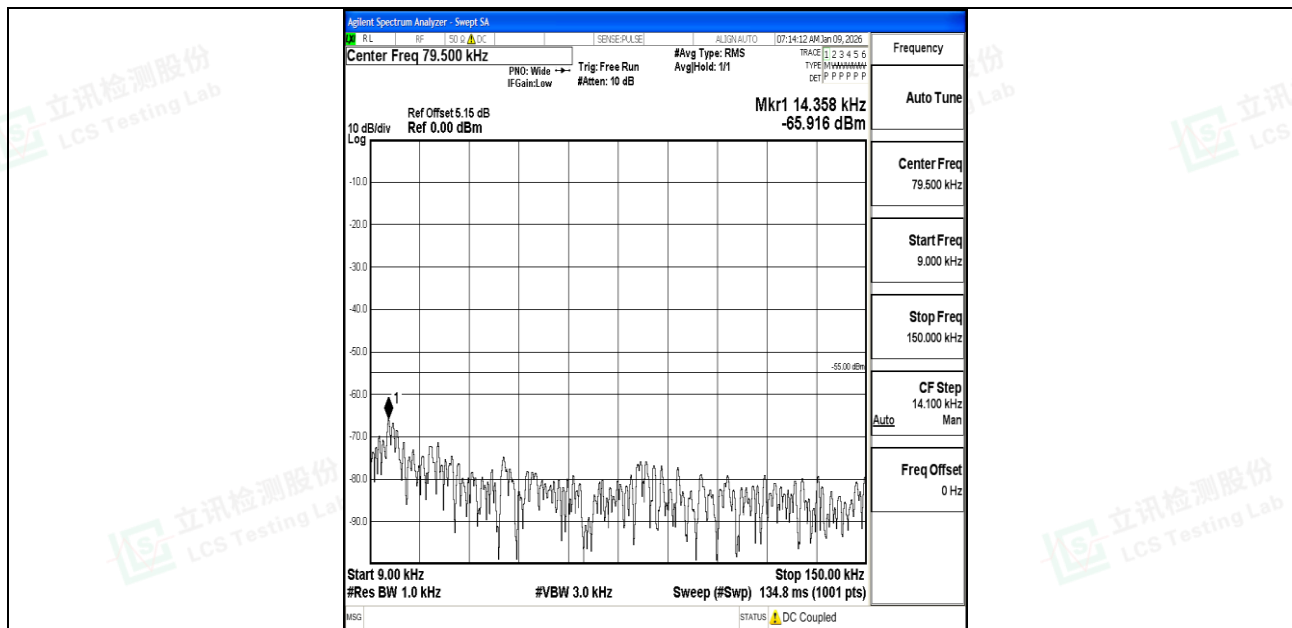
Band7_20MHz_QPSK_21350_1RB#0_0.009~0.15_0.009~0.15
