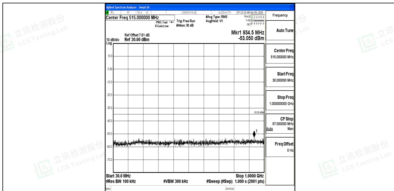
Band7_20MHz_QPSK_21100_1RB#0_30~1000_30~1000
