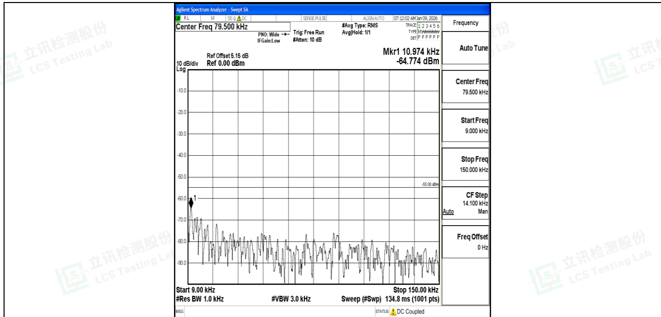
Band7_20MHz_QPSK_20850_1RB#0_0.009~0.15_0.009~0.15
