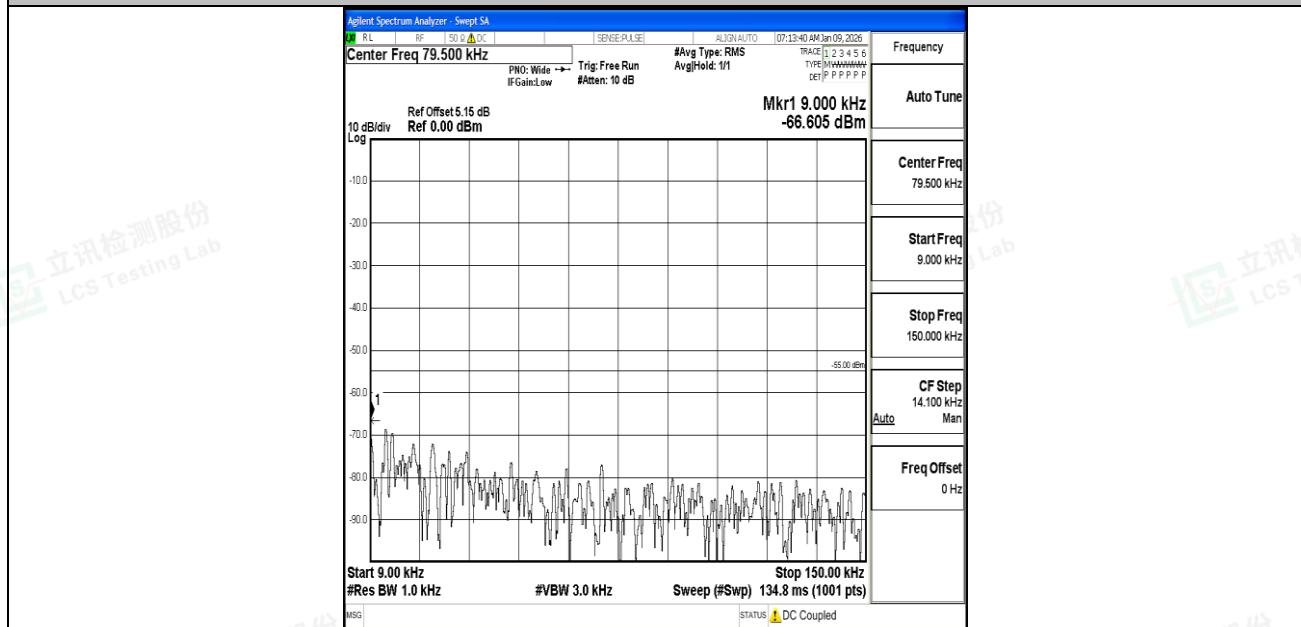
Band7_20MHz_16QAM_21100_1RB#0_0.009~0.15_0.009~0.15
