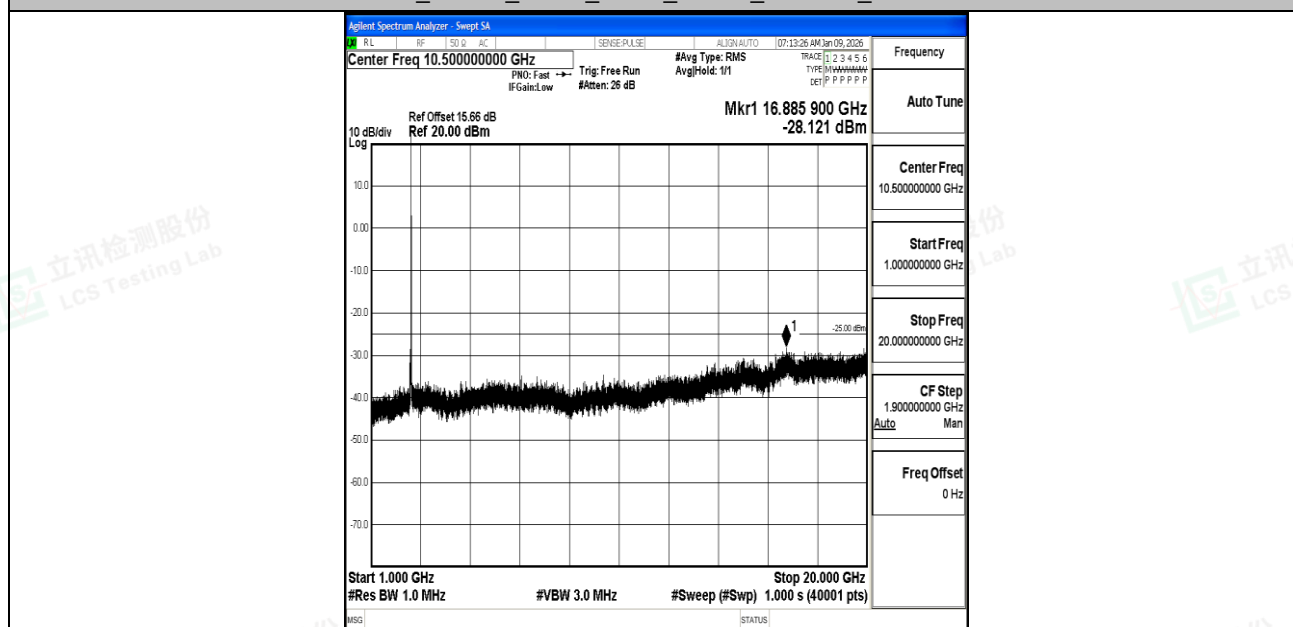
Band7_20MHz_QPSK_21100_1RB#0_1000~20000_1000~20000
