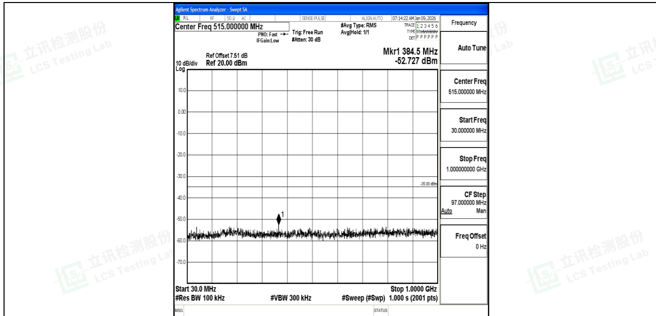
Band7_20MHz_QPSK_21350_1RB#0_30~1000_30~1000
