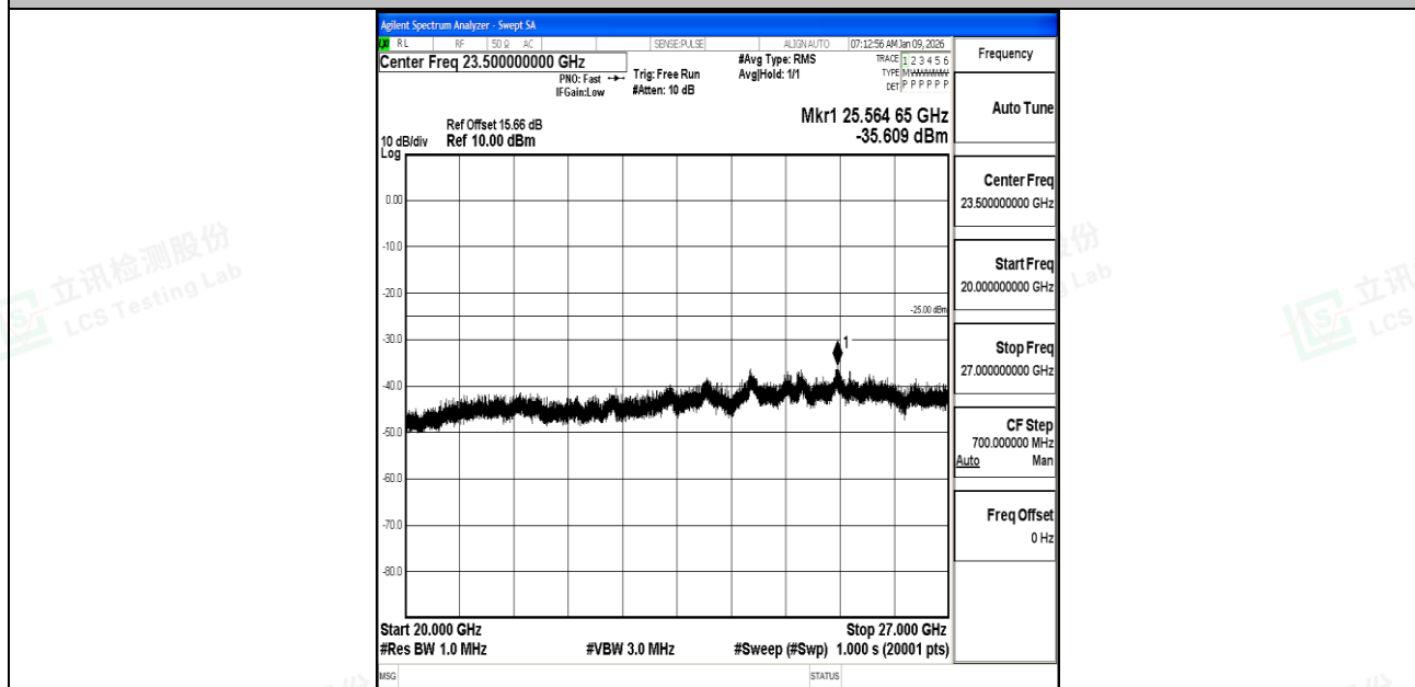
Band7_20MHz_16QAM_20850_1RB#0_20000~27000_20000~27000
