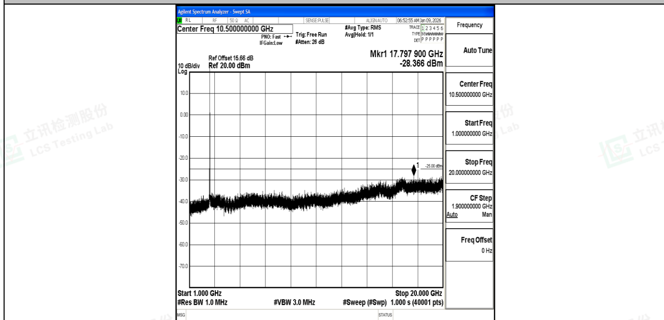
Band7_15MHz_QPSK_21100_1RB#0_1000~20000_1000~20000
