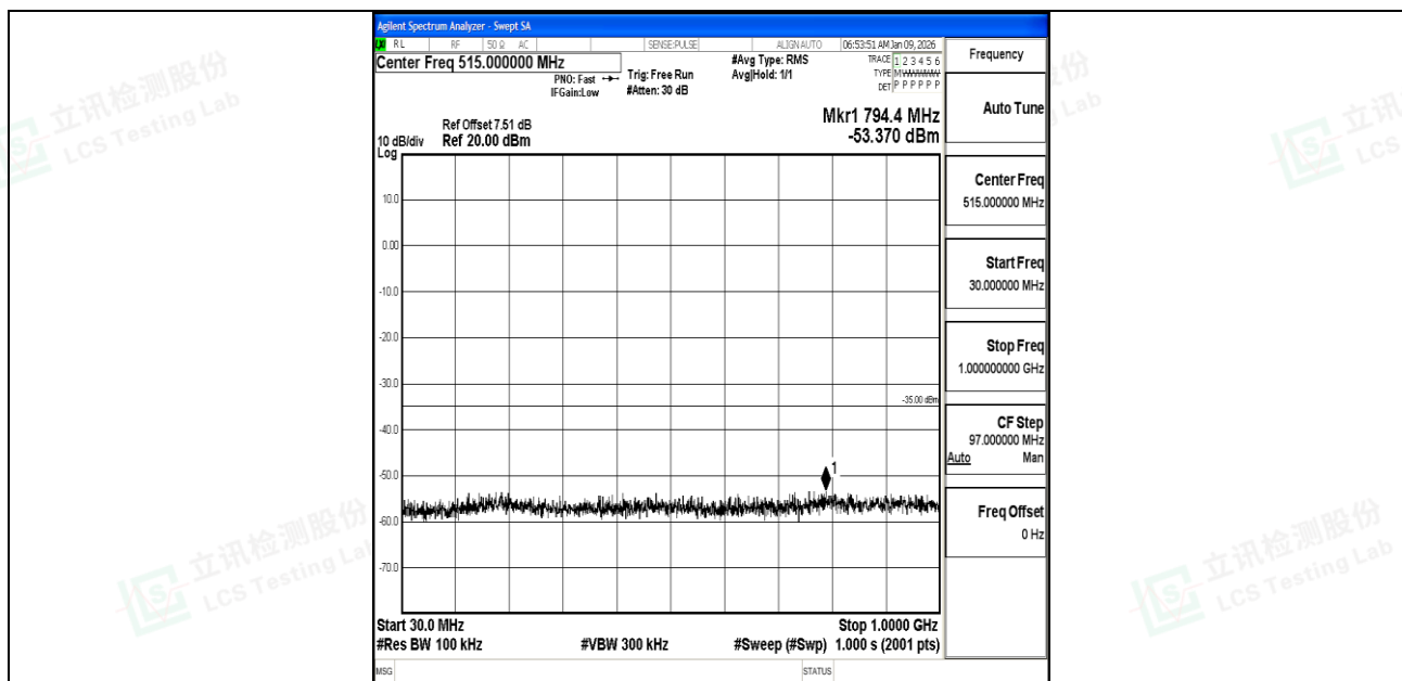
Band7_15MHz_QPSK_21375_1RB#0_30~1000_30~1000
