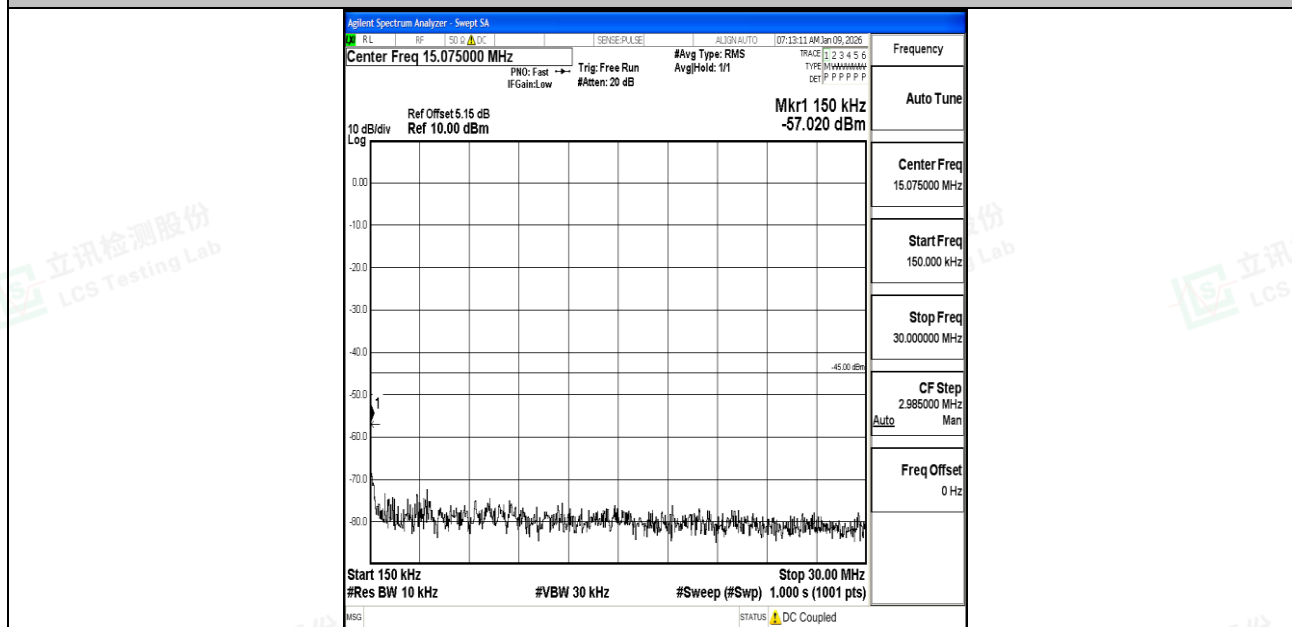
Band7_20MHz_QPSK_21100_1RB#0_0.15~30_0.15~30
