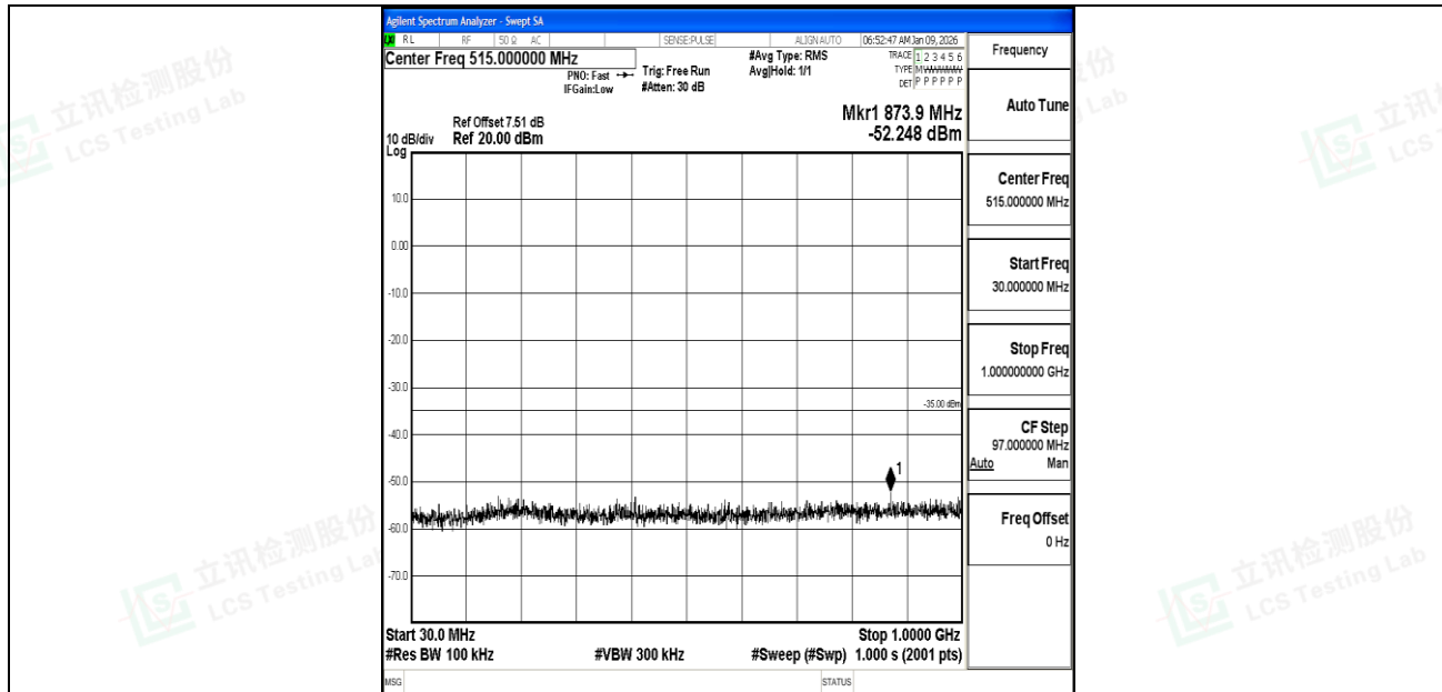
Band7_15MHz_QPSK_21100_1RB#0_30~1000_30~1000
