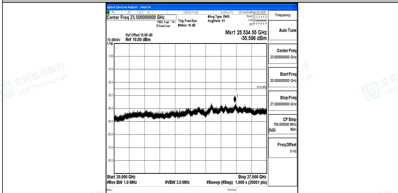
Band7_20MHz_16QAM_21100_1RB#0_20000~27000_20000~27000
