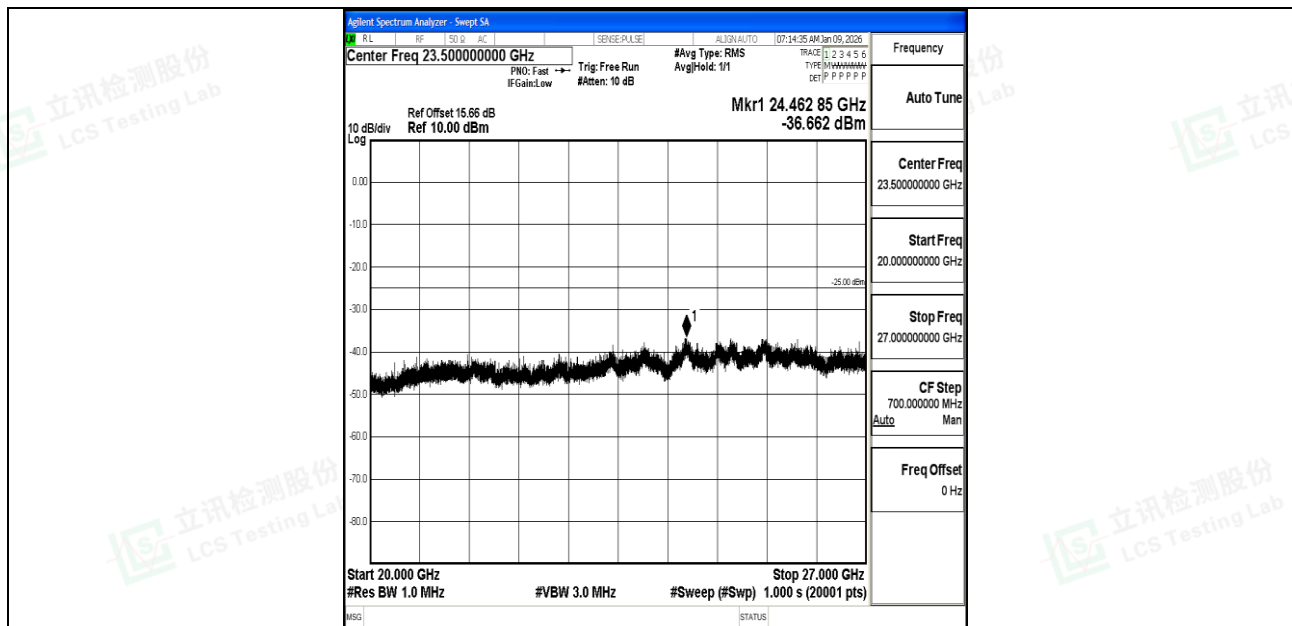
Band7_20MHz_QPSK_21350_1RB#0_20000~27000_20000~27000
