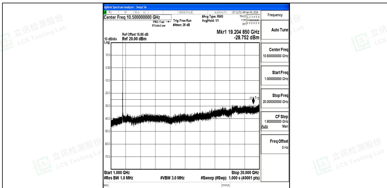
Band7_20MHz_16QAM_20850_1RB#0_1000~20000_1000~20000
