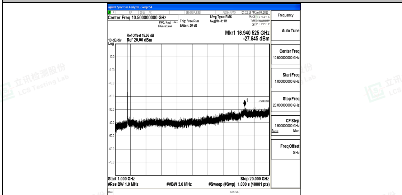
Band7_20MHz_QPSK_20850_1RB#0_1000~20000_1000~20000
