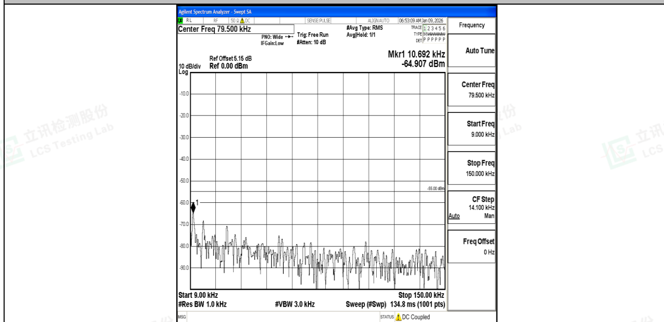
Band7_15MHz_16QAM_21100_1RB#0_0.009~0.15_0.009~0.15
