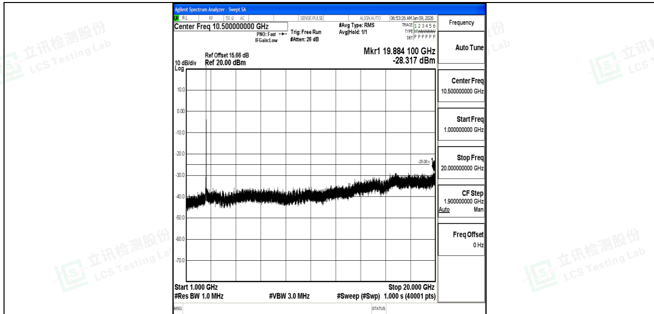
Band7_15MHz_16QAM_21100_1RB#0_1000~20000_1000~20000
