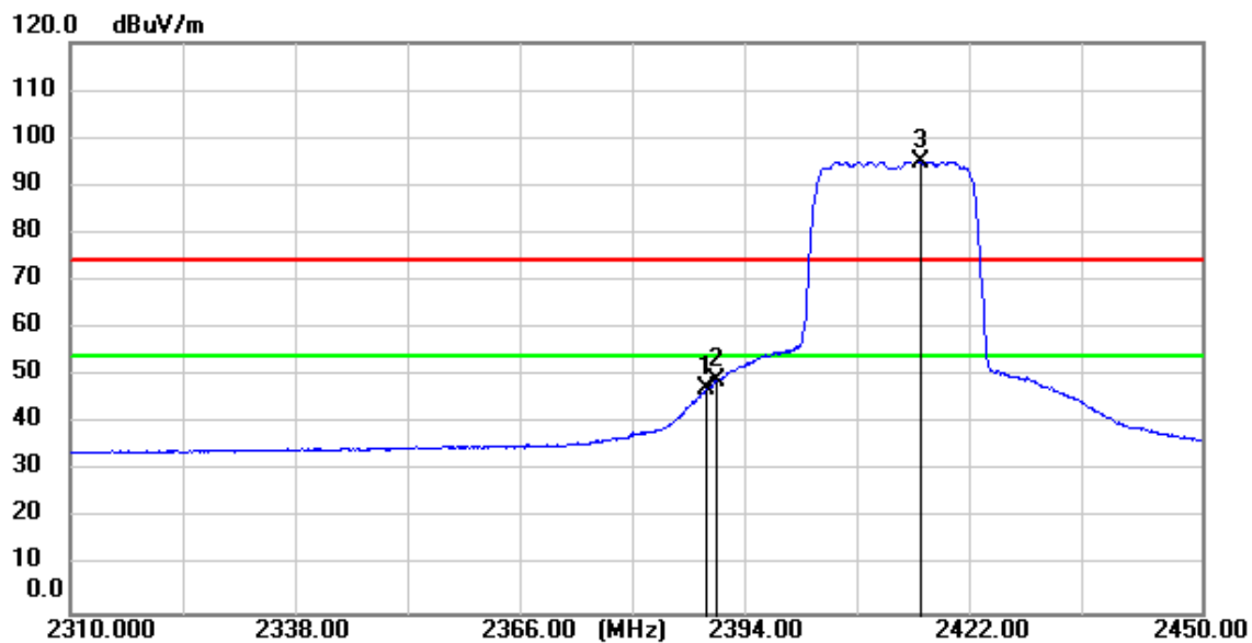
11(HE20)_TX_CH_01_Vertical_Average
