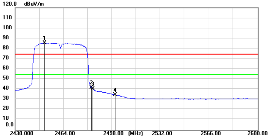
11n(HT40)_TX_CH_09_Vertical_Average
