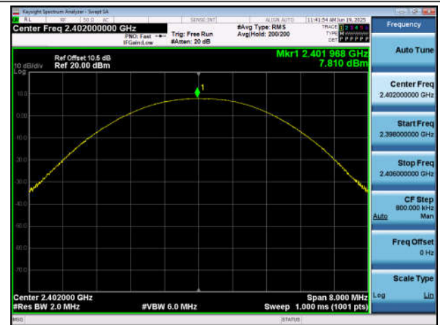
Peak Output Power \pi/4 DQPSK_Channel 0
