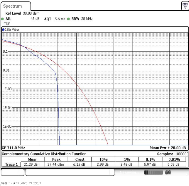
Band12-10MHz-16QAM-23130-1RB#0
