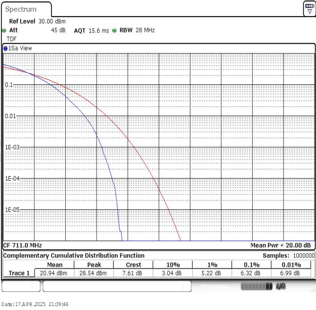
Band12-10MHz-16QAM-23130-50RB#0
