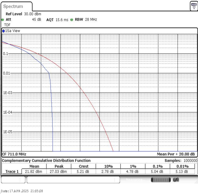
Band12-10MHz-QPSK-23130-1RB#0
