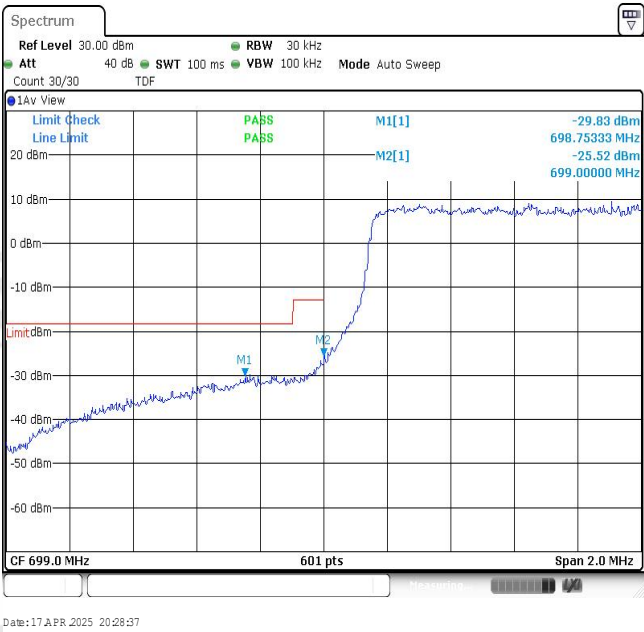
Band12-1.4MHz-QPSK-23017-6RB#0
