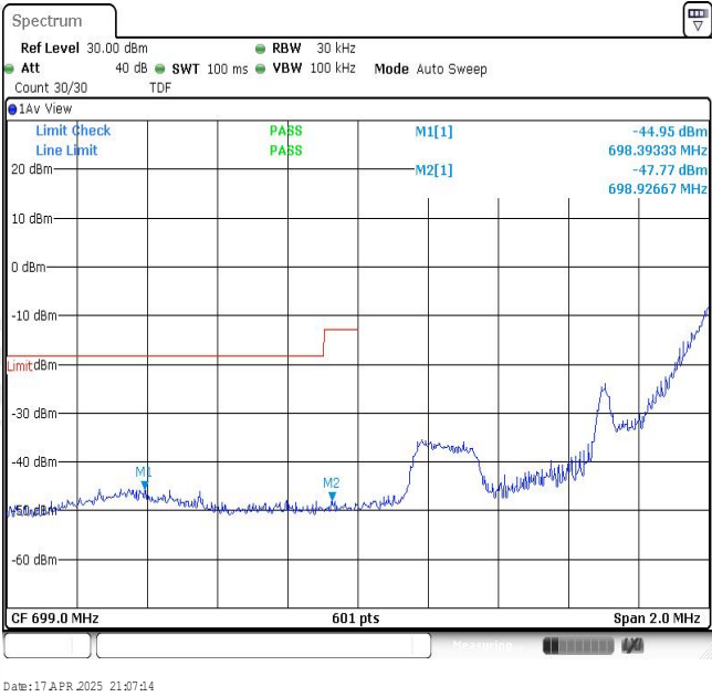
Band12-1.4MHz-16QAM-23017-1RB#5
