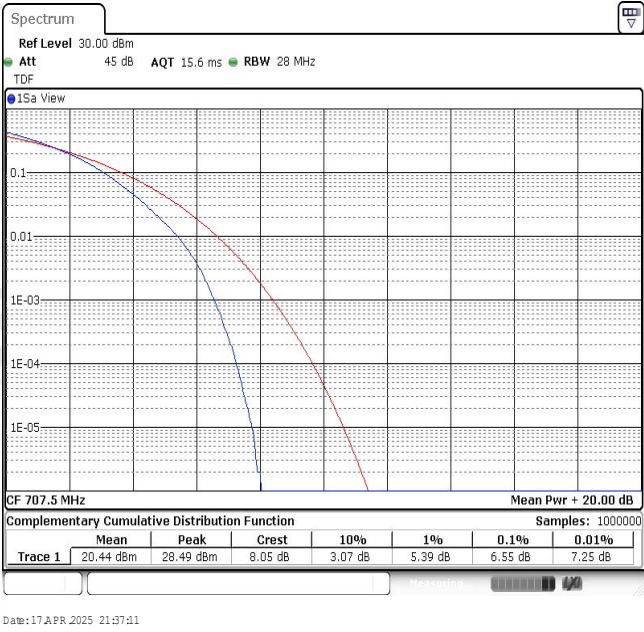
Band12-10MHz-16QAM-23095-50RB#0
