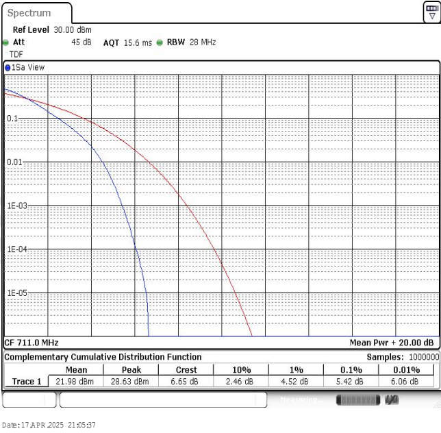
Band12-10MHz-QPSK-23130-50RB#0
