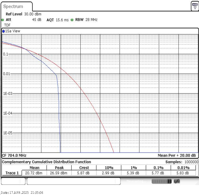
Band12-10MHz-16QAM-23060-1RB#0
