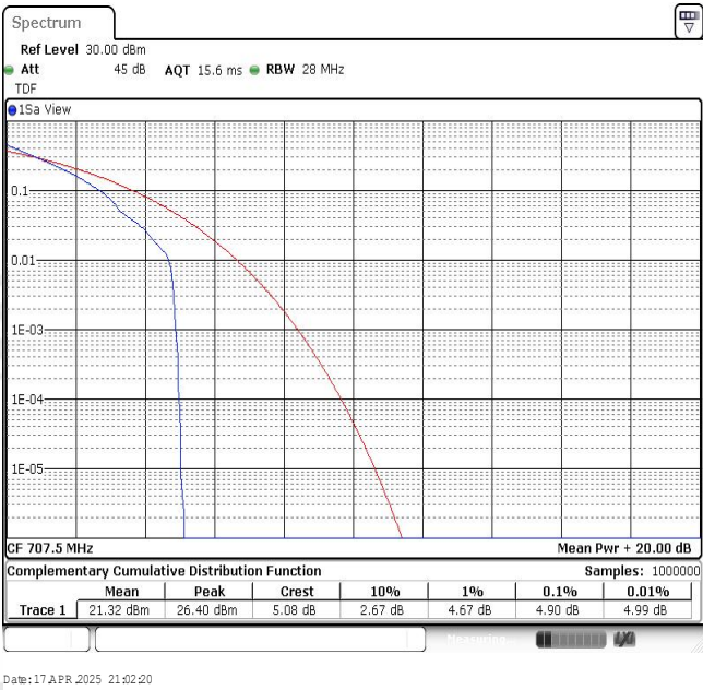
Band12-10MHz-QPSK-23095-1RB#0
