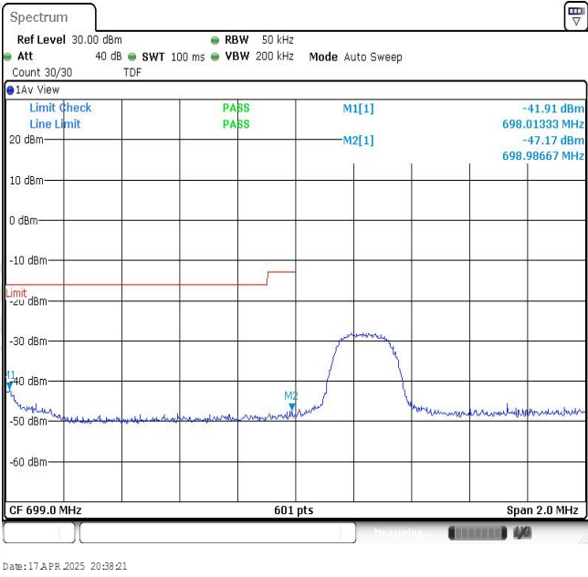
Band12-3MHz-QPSK-23025-1RB#14
