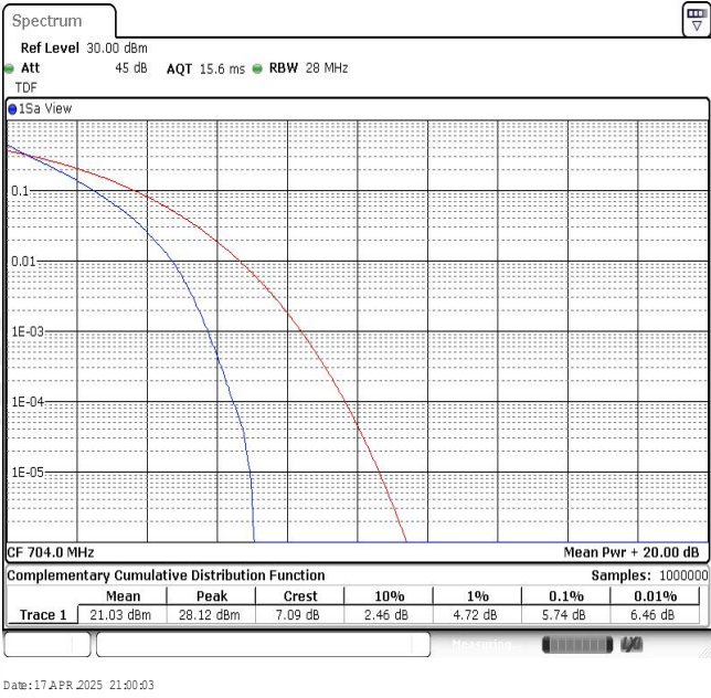
Band12-10MHz-QPSK-23060-50RB#0
