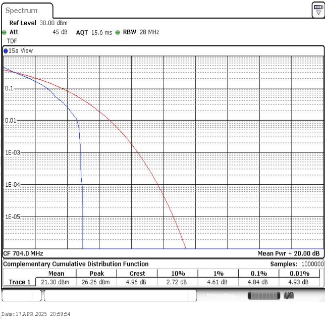
Band12-10MHz-QPSK-23060-1RB#0
