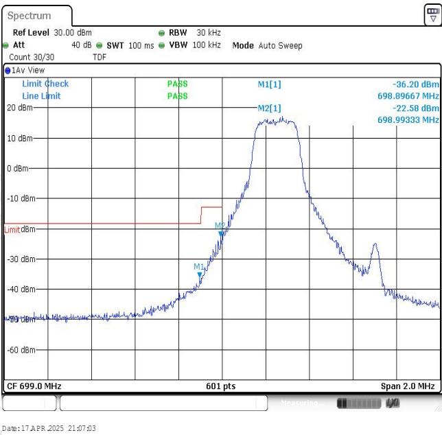
Band12-1.4MHz-16QAM-23017-1RB#0
