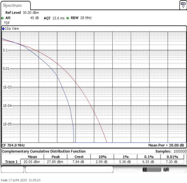
Band12-10MHz-16QAM-23060-50RB#0
