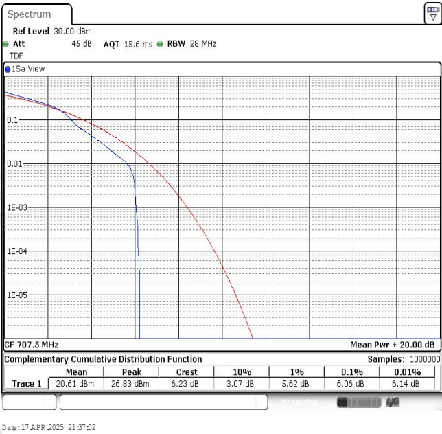
Band12-10MHz-16QAM-23095-1RB#0
