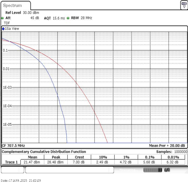
Band12-10MHz-QPSK-23095-50RB#0
