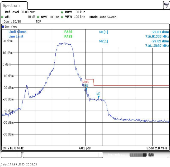
Band12-1.4MHz-QPSK-23173-1RB#5
