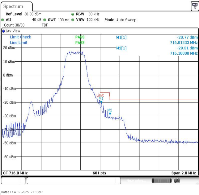
Band12-1.4MHz-16QAM-23173-1RB#5
