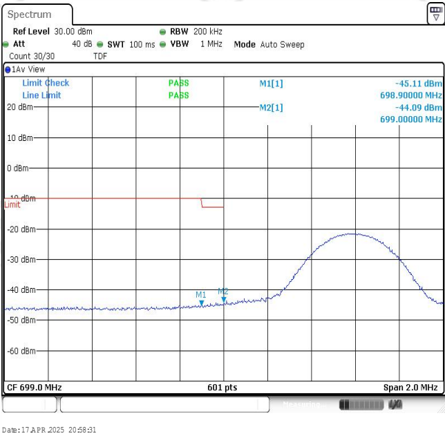
Band12-10MHz-QPSK-23060-1RB#49
