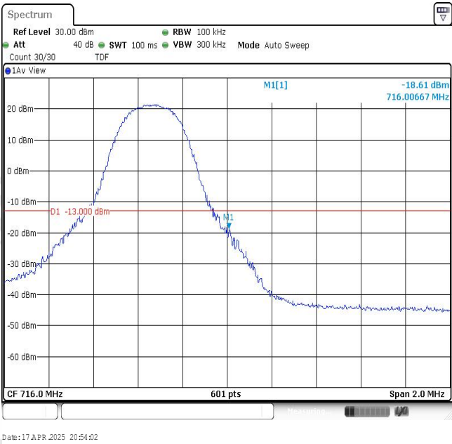
Band12-5MHz-QPSK-23155-1RB#24
