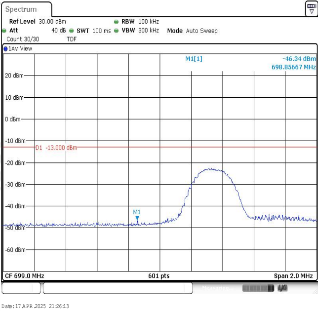
Band12-5MHz-16QAM-23035-1RB#24
