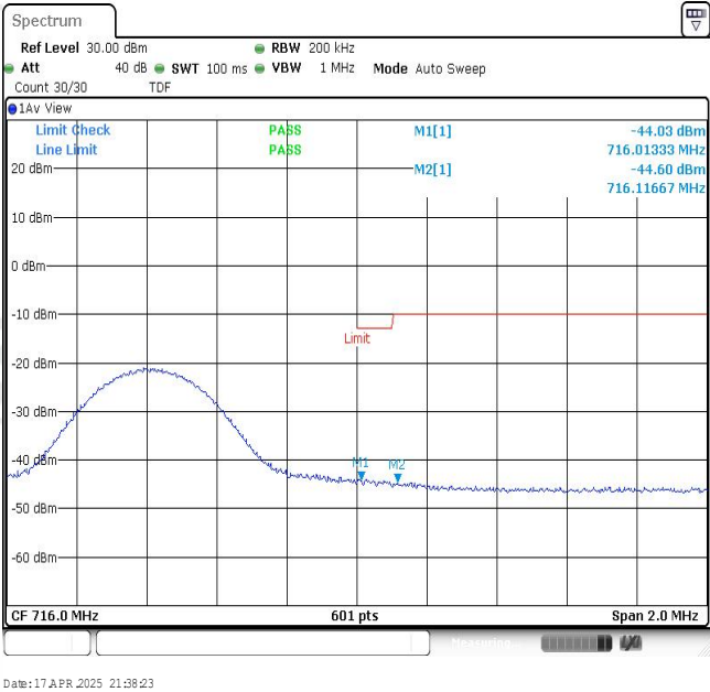
Band12-10MHz-16QAM-23130-1RB#0
