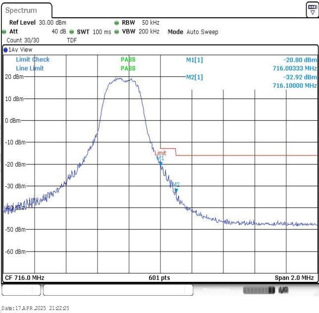
Band12-3MHz-16QAM-23165-1RB#14
