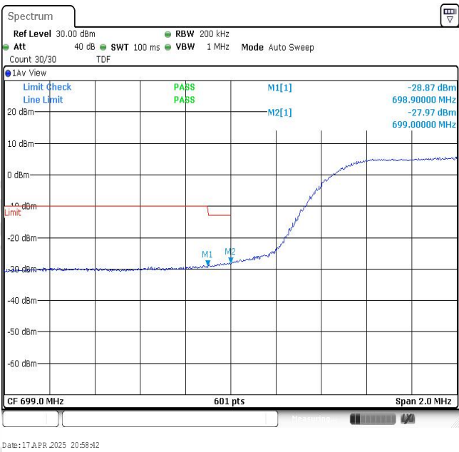
Band12-10MHz-QPSK-23060-50RB#0
