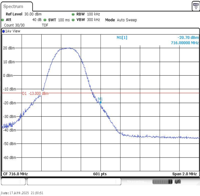
Band12-5MHz-16QAM-23155-1RB#24
