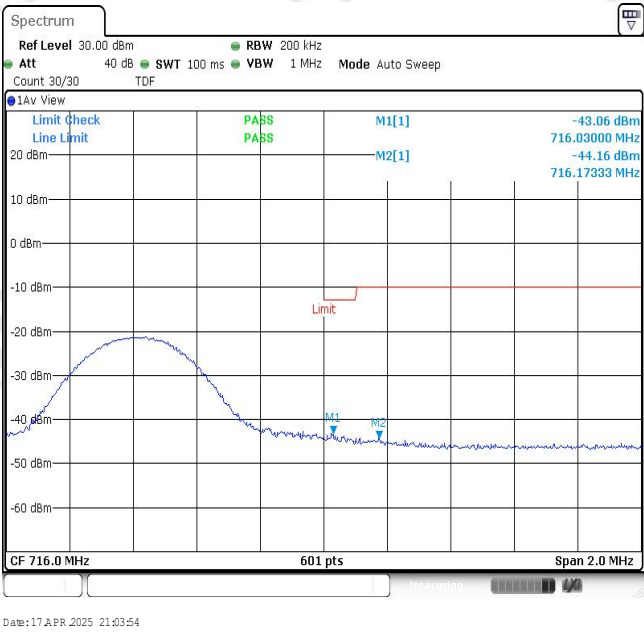
Band12-10MHz-QPSK-23130-1RB#0
