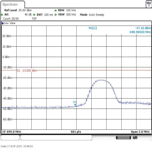
Band12-5MHz-QPSK-23035-1RB#24
