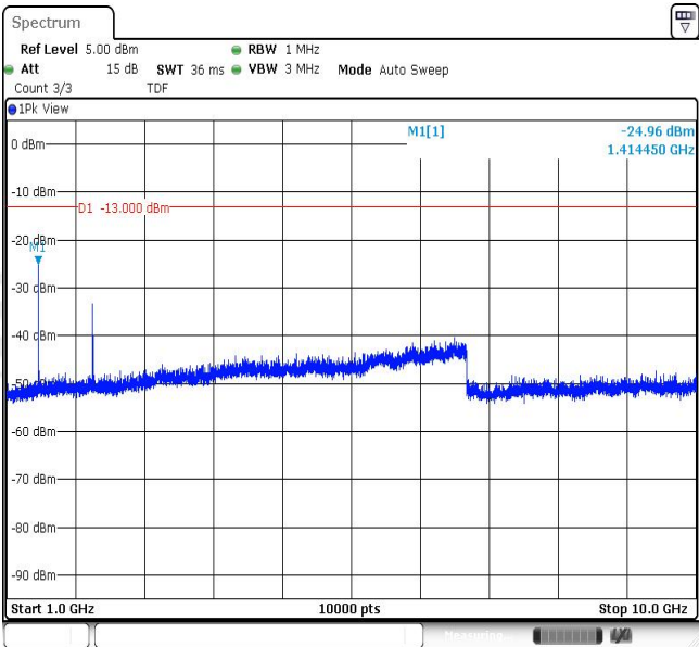
Band12-1.4MHz-QPSK-23095-1RB#0-Range2:1000~10000MHz
