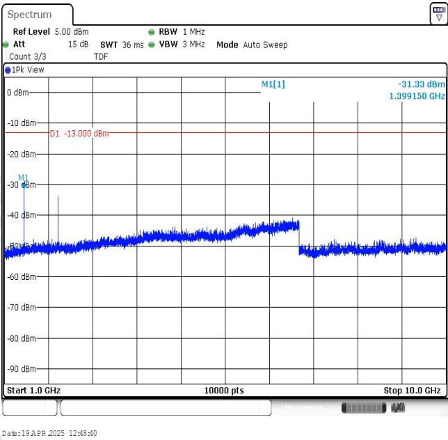
Band12-5MHz-QPSK-23035-1RB#0-Range2:1000~10000MHz
