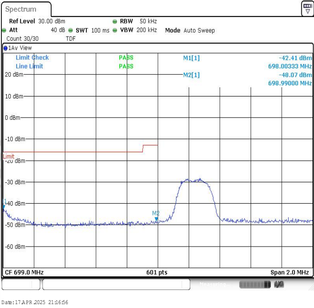
Band12-3MHz-16QAM-23025-1RB#14
