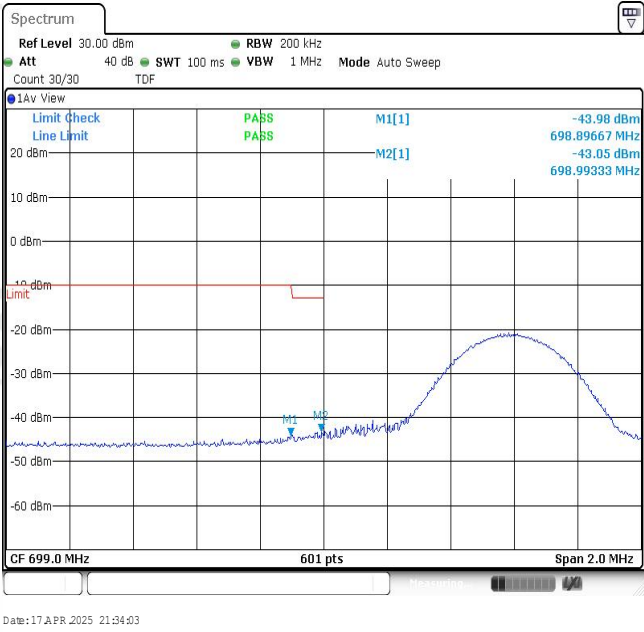
Band12-10MHz-16QAM-23060-1RB#49
