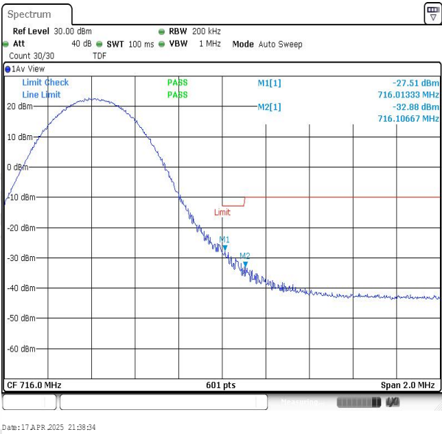
Band12-10MHz-16QAM-23130-1RB#49
