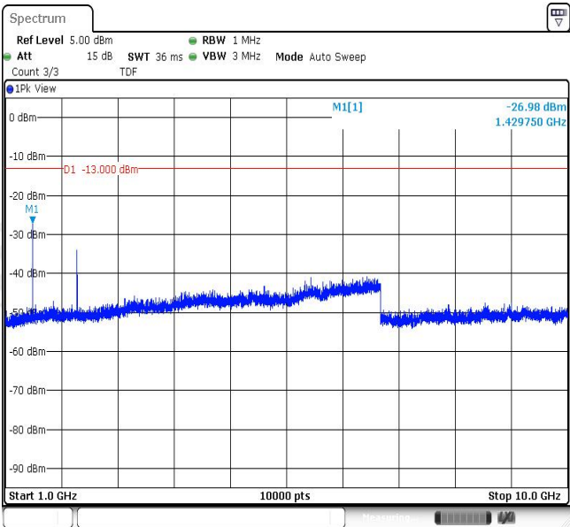
Band12-1.4MHz-QPSK-23173-1RB#0-Range2:1000~10000MHz
