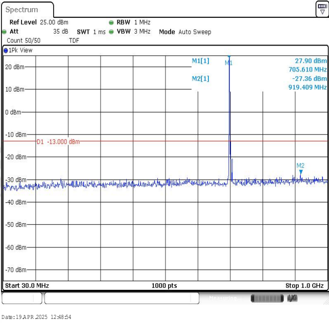
Band12-5MHz-QPSK-23095-1RB#0-Range1:30~1000MHz
