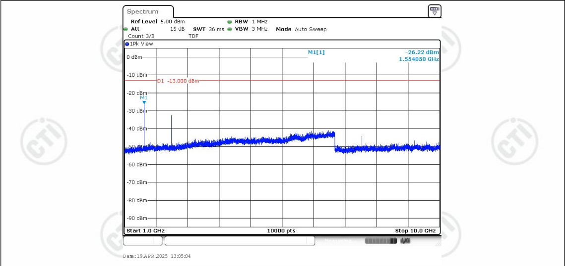
Band13-5MHz-16QAM-23205-1RB#0-Range2:1000~10000MHz
