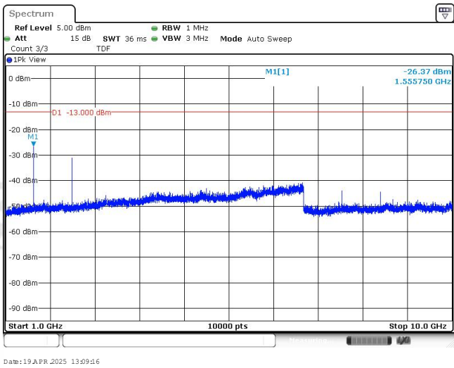
Band13-10MHz-16QAM-23230-1RB#0-Range2:1000~10000MHz
