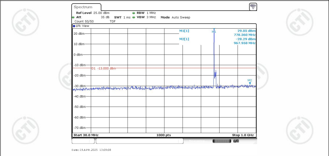
Band13-10MHz-16QAM-23230-1RB#0-Range1:30~1000MHz
