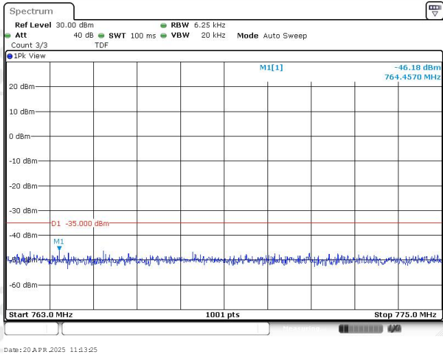
Band13-5MHz-QPSK-23205-1RB#0-Range1:763~775MHz
