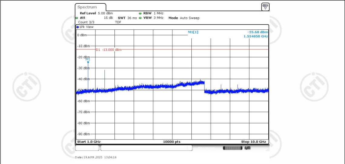
Band13-10MHz-QPSK-23230-1RB#0-Range2:1000~10000MHz
