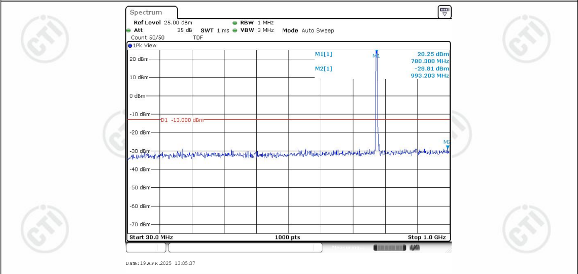
Band13-5MHz-16QAM-23230-1RB#0-Range1:30~1000MHz
