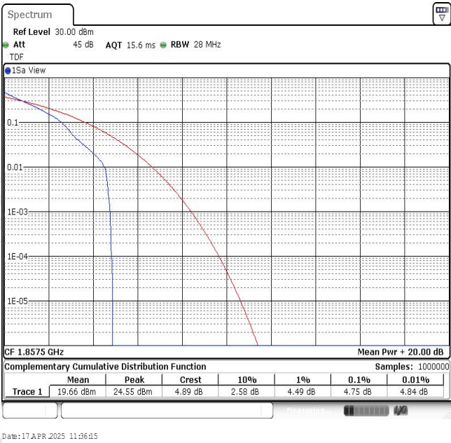
Band2-15MHz-QPSK-18675-1RB#0
