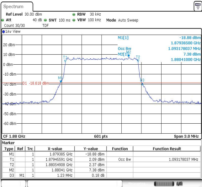
Band2-1.4MHz-16QAM-18900-6RB#0-1.093
