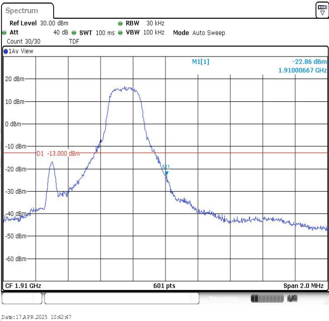
Band2-1.4MHz-QPSK-19193-1RB#5
