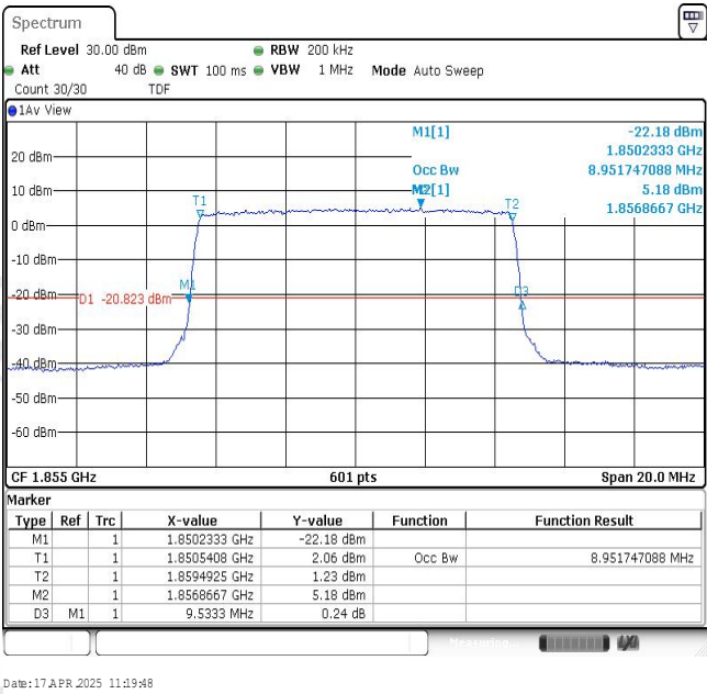
Band2-10MHz-QPSK-18650-50RB#0-8.952
