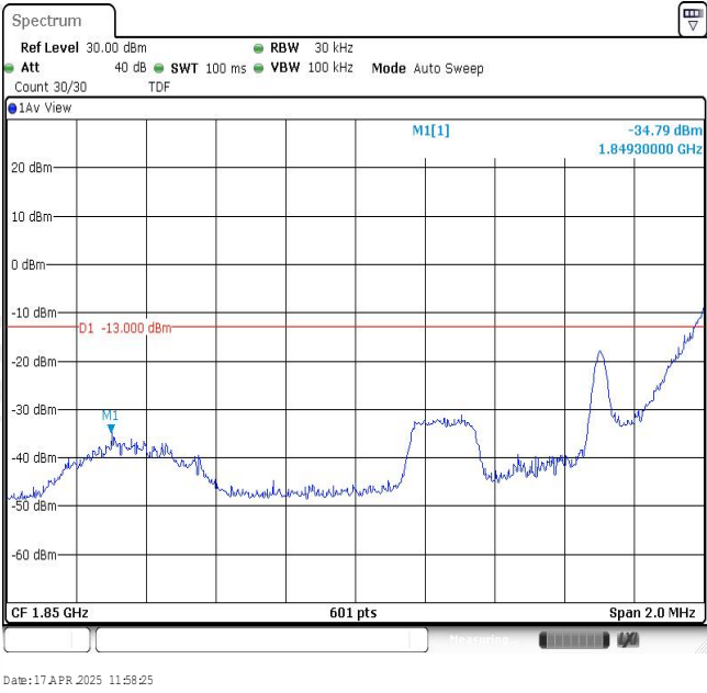
Band2-1.4MHz-16QAM-18607-1RB#5
