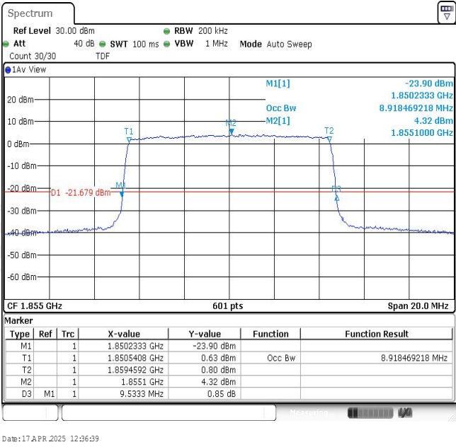
Band2-10MHz-16QAM-18650-50RB#0-8.918
