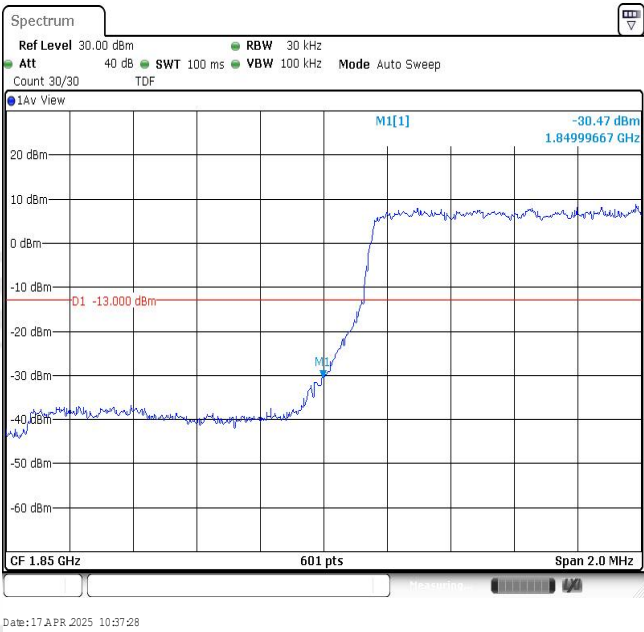
Band2-1.4MHz-QPSK-18607-6RB#0
