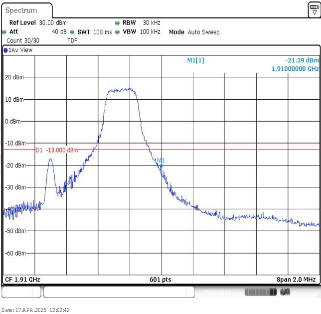
Band2-1.4MHz-16QAM-19193-1RB#5
