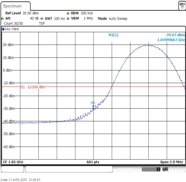
Band2-10MHz-16QAM-18650-1RB#0
