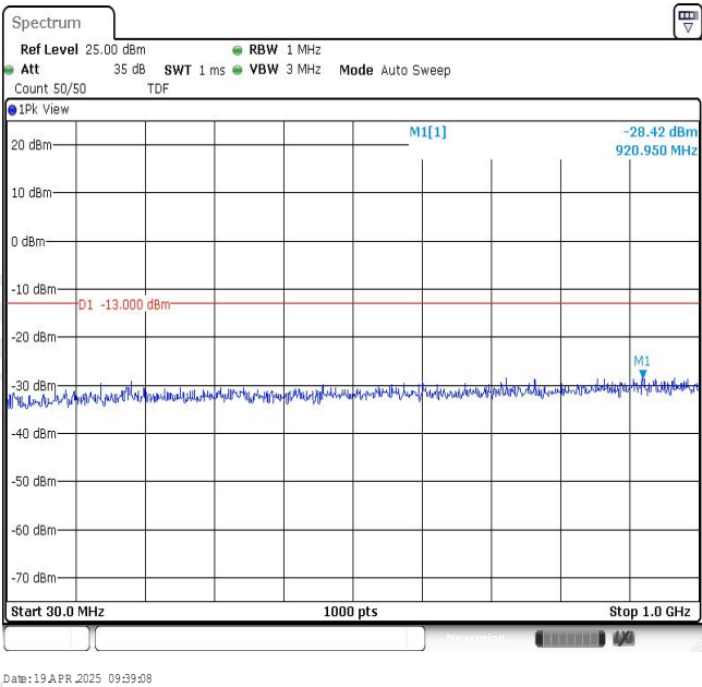
Band2-1.4MHz-16QAM-18607-1RB#0-Range1:30~1000MHz
