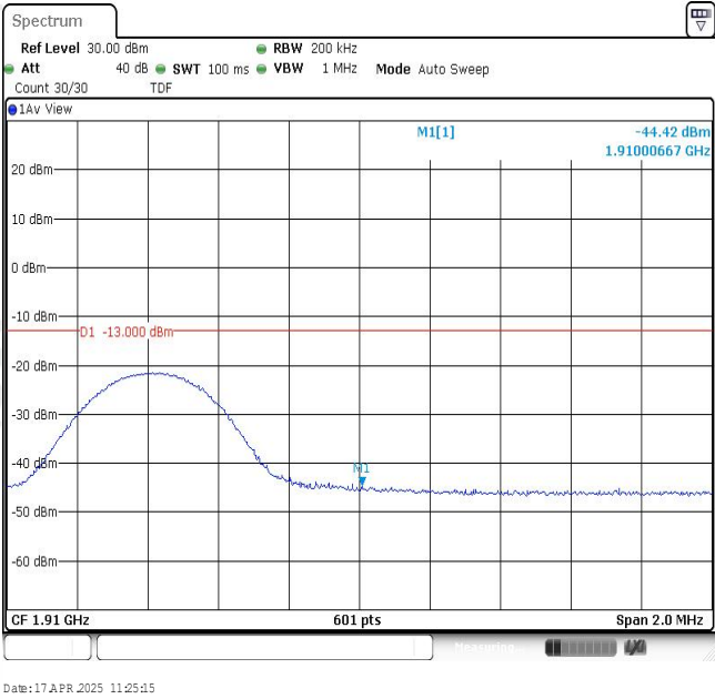
Band2-10MHz-QPSK-19150-1RB#0
