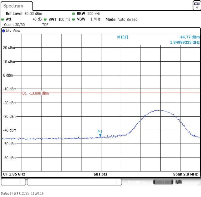
Band2-10MHz-QPSK-18650-1RB#49
