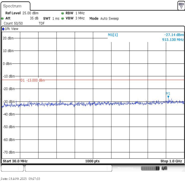
Band2-1.4MHz-QPSK-18900-1RB#0-Range1:30~1000MHz
