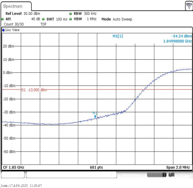
Band2-15MHz-QPSK-18675-75RB#0
