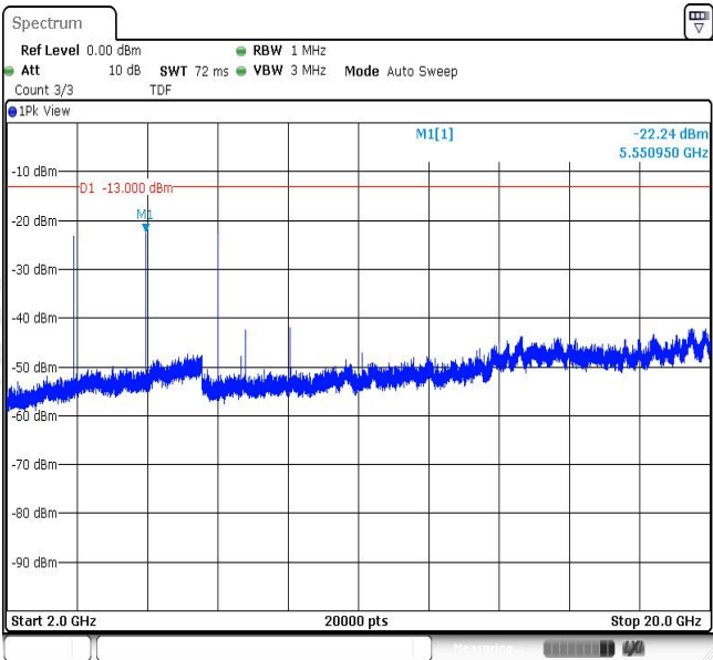
Band2-1.4MHz-16QAM-18607-1RB#0-Range3:2000~20000MHz
