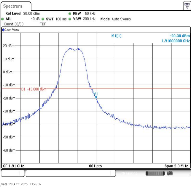
Band2-3MHz-16QAM-19185-1RB#14
