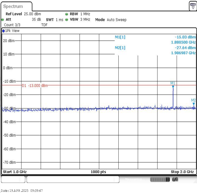
Band2-1.4MHz-16QAM-18900-1RB#0-Range2:1000~2000MHz
