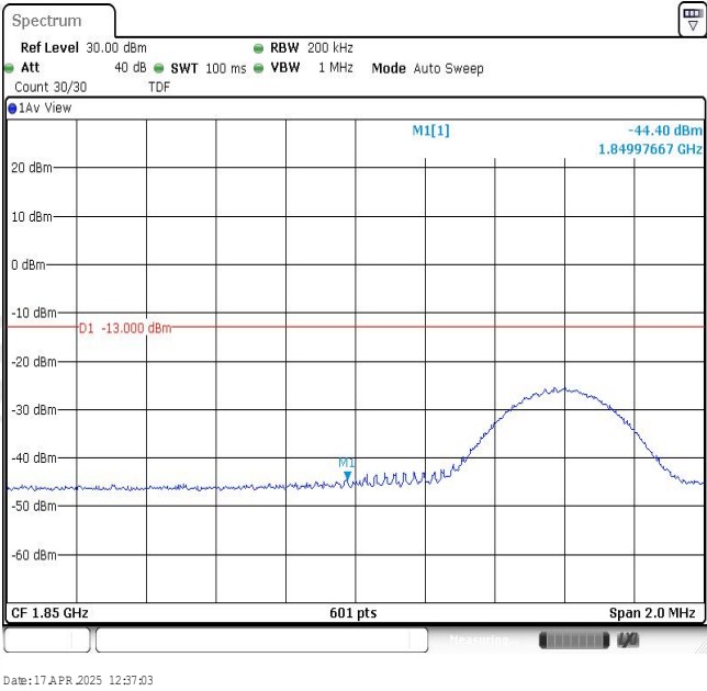
Band2-10MHz-16QAM-18650-1RB#49
