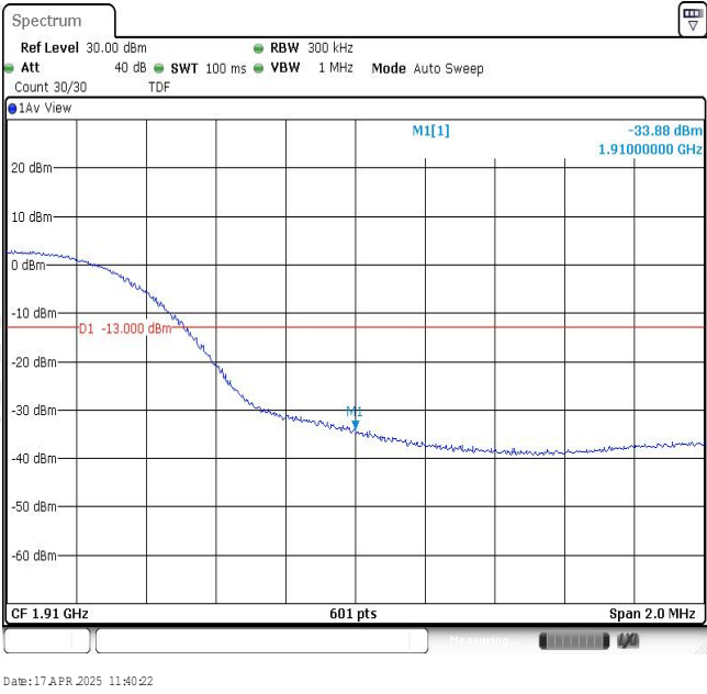
Band2-15MHz-QPSK-19125-75RB#0
