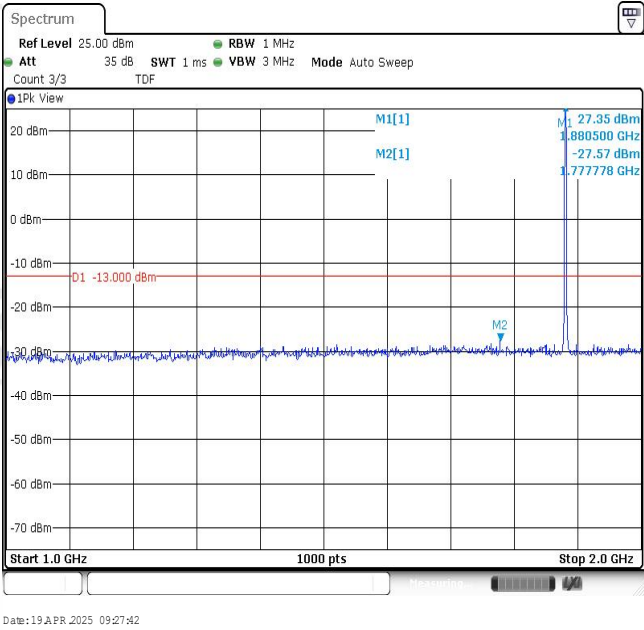
Band2-1.4MHz-QPSK-18900-1RB#0-Range2:1000~2000MHz
