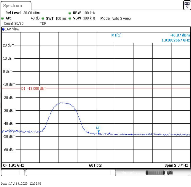
Band2-5MHz-16QAM-19175-1RB#0
