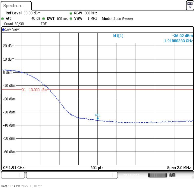
Band2-15MHz-16QAM-19125-75RB#0
