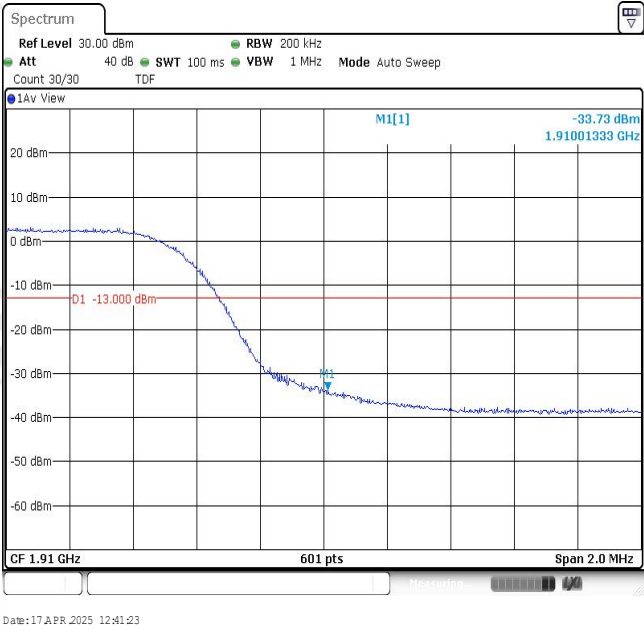
Band2-10MHz-16QAM-19150-50RB#0
