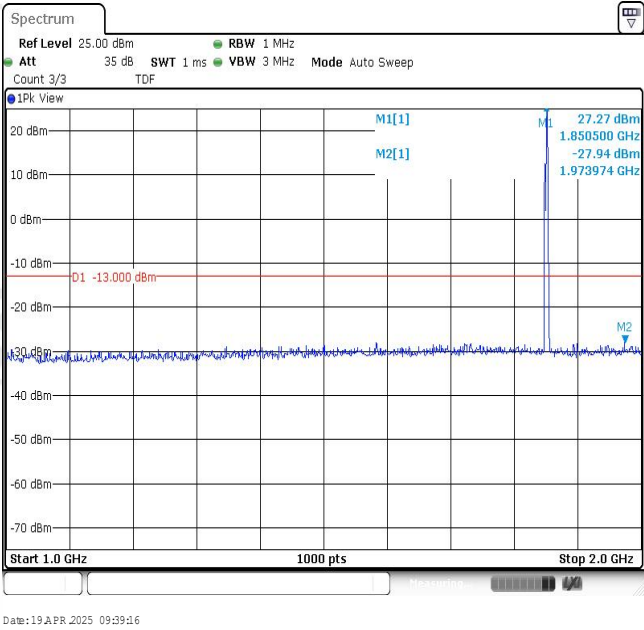
Band2-1.4MHz-16QAM-18607-1RB#0-Range2:1000~2000MHz
