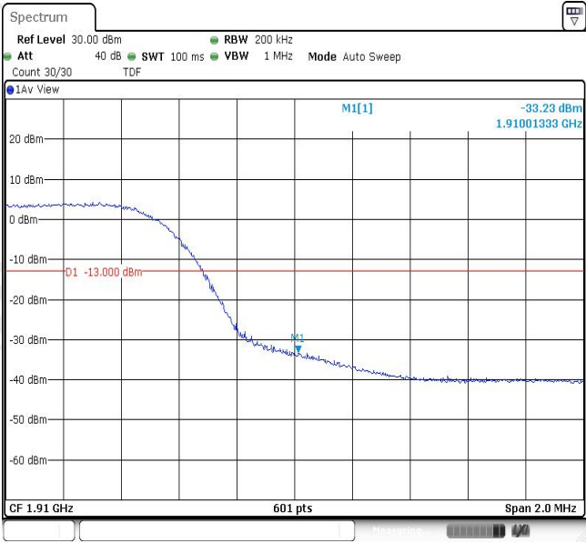
Band2-10MHz-QPSK-19150-1RB#49
