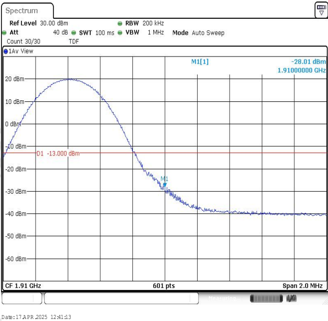
Band2-10MHz-16QAM-19150-1RB#49
