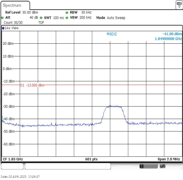
Band2-3MHz-16QAM-18615-1RB#14
