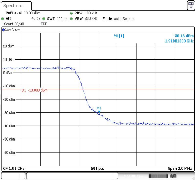
Band2-5MHz-16QAM-19175-1RB#24
