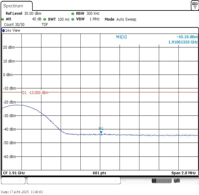
Band2-15MHz-QPSK-19125-1RB#0
