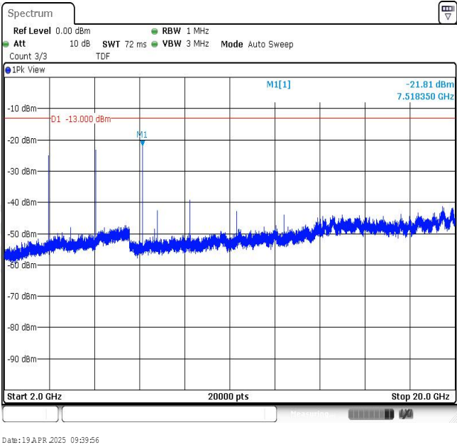
Band2-1.4MHz-16QAM-18900-1RB#0-Range3:2000~20000MHz
