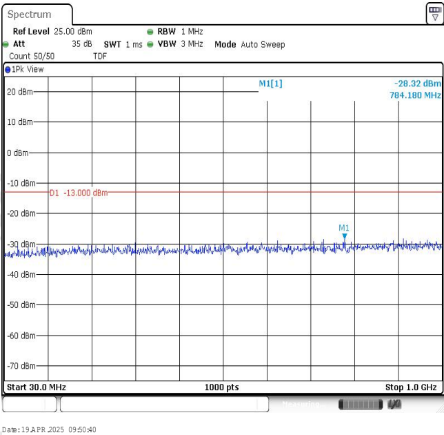
Band2-20MHz-16QAM-19100-1RB#0-Range1:30~1000MHz
