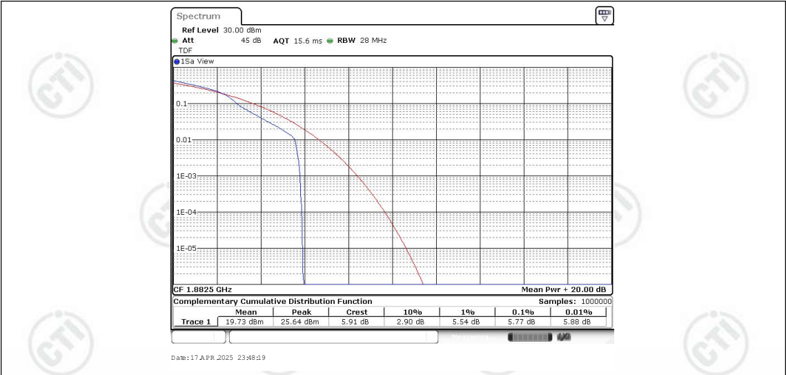
Band25-15MHz-16QAM-26365-1RB#0
