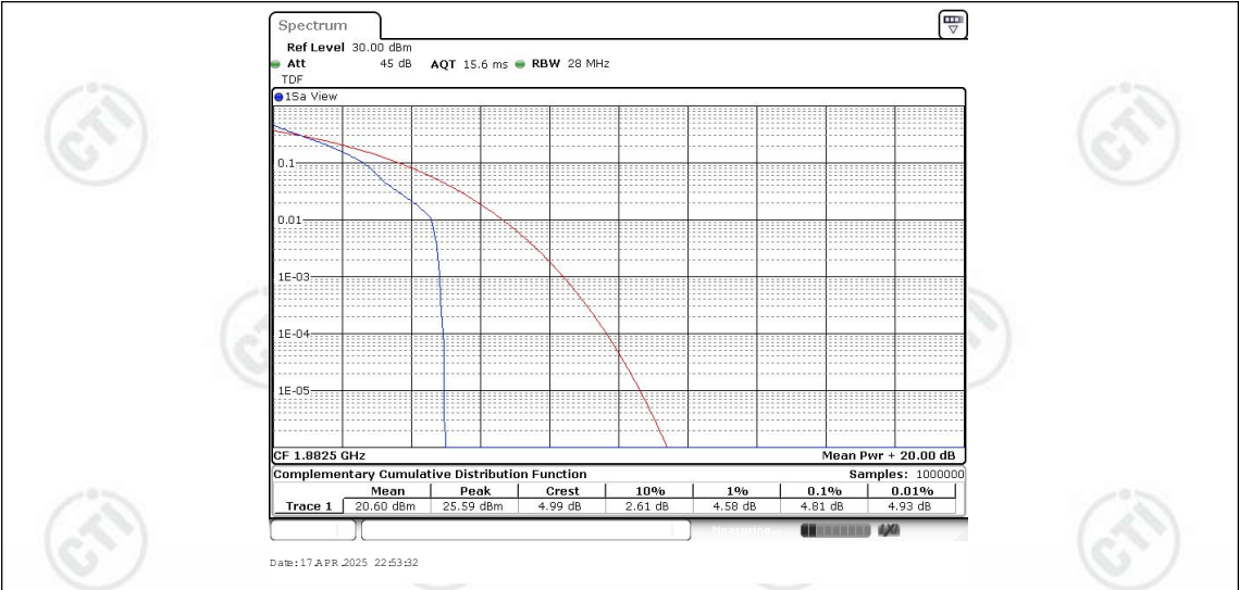
Band25-15MHz-QPSK-26365-1RB#0
