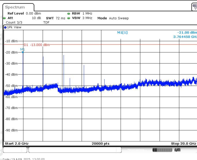
Band25-1.4MHz-16QAM-26365-1RB#0-Range3:2000~20000MHz
