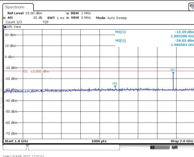
Band25-1.4MHz-16QAM-26365-1RB#0-Range2:1000~2000MHz
