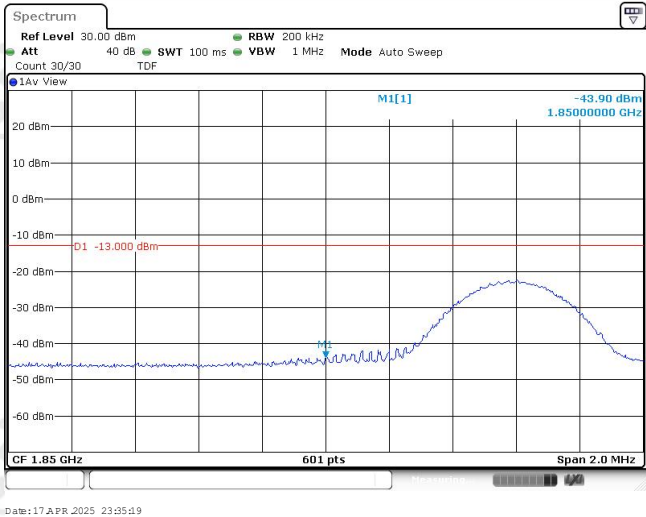
Band25-10MHz-16QAM-26090-1RB#49
