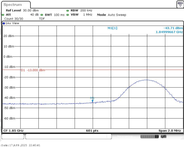
Band25-10MHz-QPSK-26090-1RB#49
