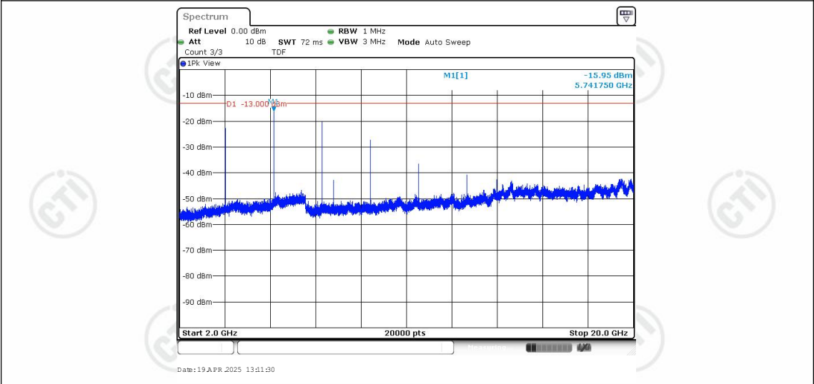
Band25-1.4MHz-QPSK-26683-1RB#0-Range3:2000~20000MHz
