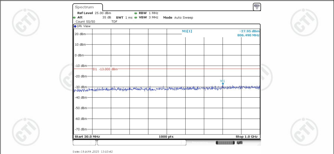
Band25-1.4MHz-QPSK-26365-1RB#0-Range1:30~1000MHz
