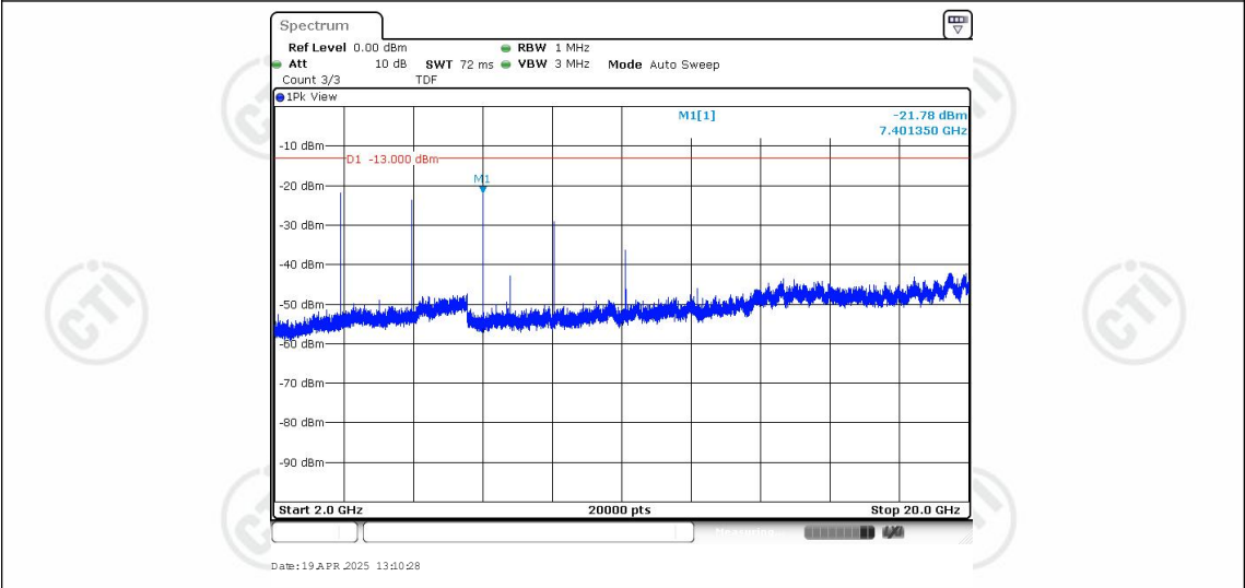
Band25-1.4MHz-QPSK-26047-1RB#0-Range3:2000~20000MHz
