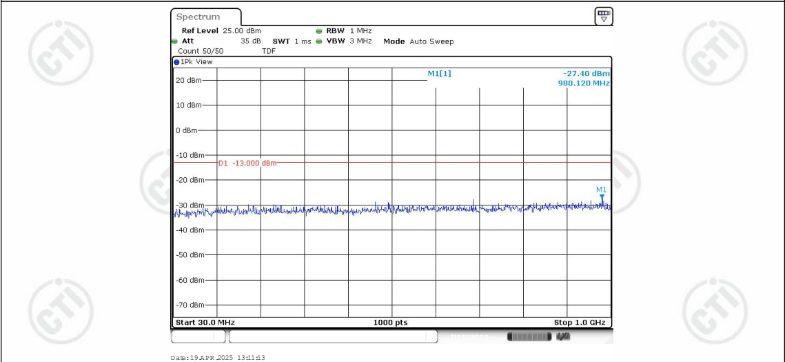
Band25-1.4MHz-QPSK-26683-1RB#0-Range1:30~1000MHz
