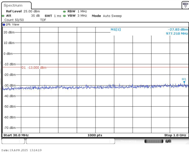
Band25-3MHz-QPSK-26055-1RB#0-Range1:30~1000MHz
