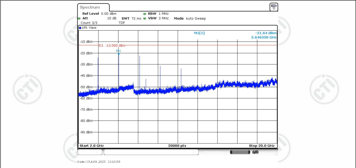
Band25-1.4MHz-QPSK-26365-1RB#0-Range3:2000~20000MHz
