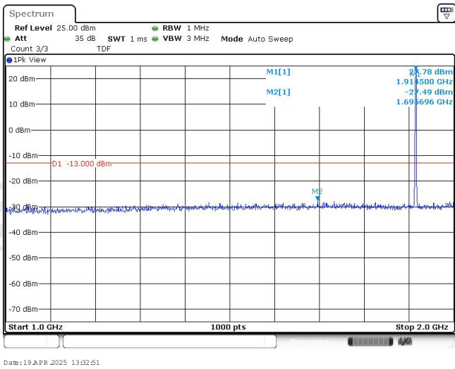
Band25-1.4MHz-16QAM-26683-1RB#0-Range2:1000~2000MHz
