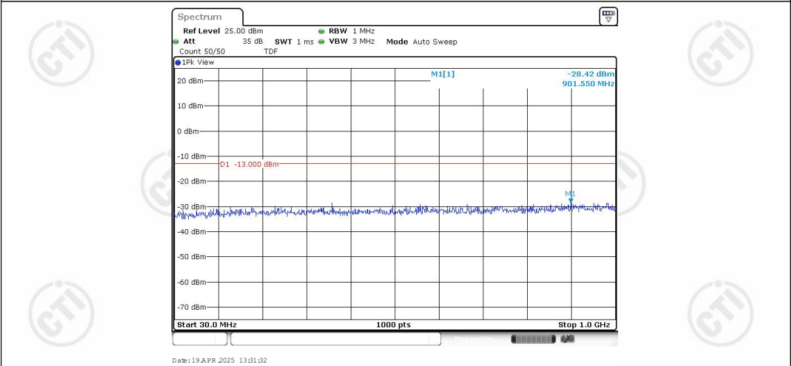
Band25-1.4MHz-16QAM-26047-1RB#0-Range1:30~1000MHz
