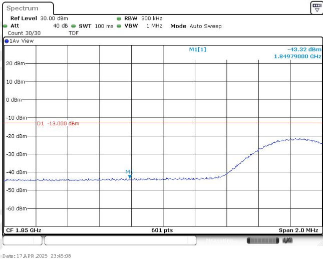
Band25-15MHz-16QAM-26115-1RB#74
