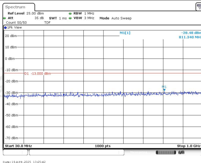
Band25-15MHz-QPSK-26115-1RB#0-Range1:30~1000MHz
