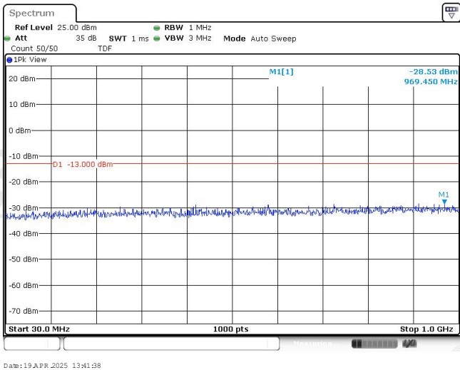
Band25-10MHz-16QAM-26090-1RB#0-Range1:30~1000MHz
