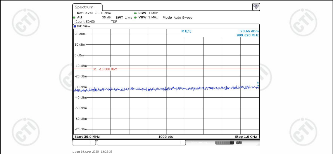
Band25-10MHz-QPSK-26640-1RB#0-Range1:30~1000MHz
