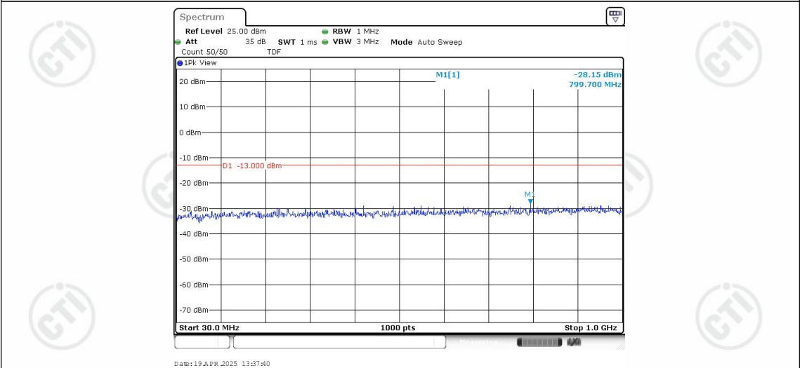
Band25-5MHz-16QAM-26065-1RB#0-Range1:30~1000MHz
