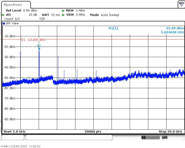
Band25-10MHz-16QAM-26365-1RB#0-Range3:2000~20000MHz
