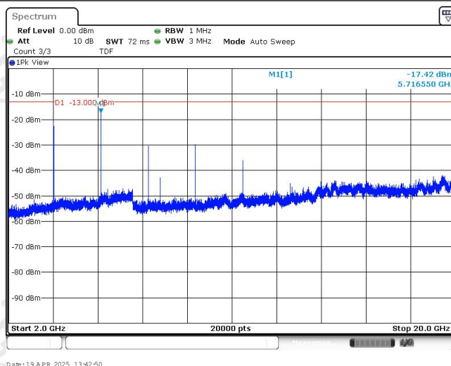
Band25-10MHz-16QAM-26640-1RB#0-Range3:2000~20000MHz
