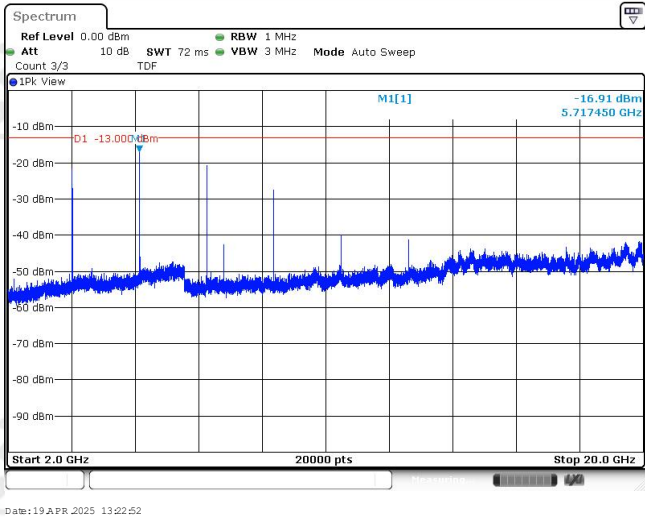
Band25-10MHz-QPSK-26640-1RB#0-Range3:2000~20000MHz
