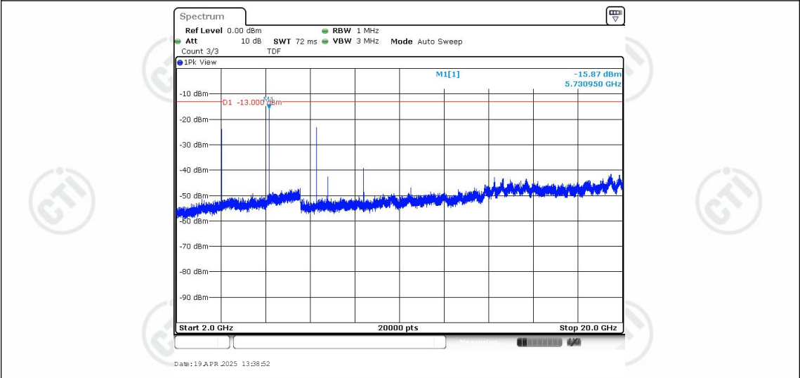
Band25-5MHz-16QAM-26665-1RB#0-Range3:2000~20000MHz
