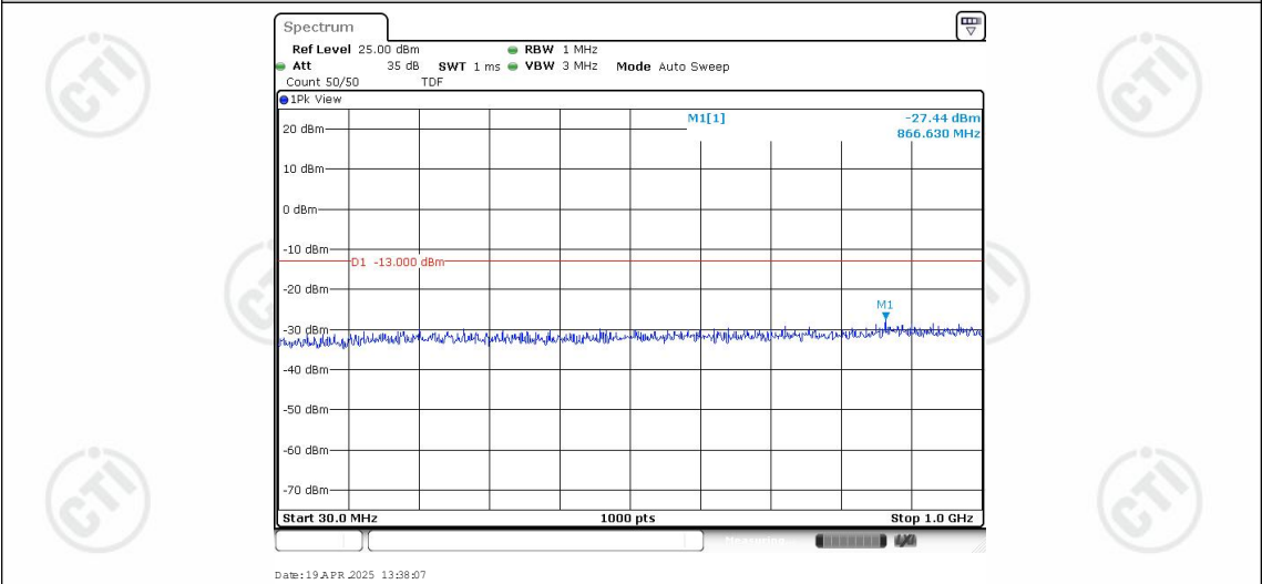
Band25-5MHz-16QAM-26365-1RB#0-Range1:30~1000MHz
