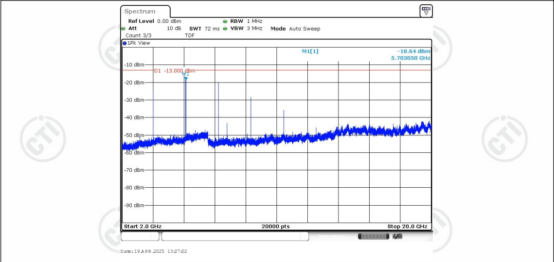
Band25-15MHz-QPSK-26615-1RB#0-Range3:2000~20000MHz
