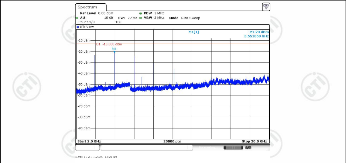
Band25-10MHz-QPSK-26090-1RB#0-Range3:2000~20000MHz
