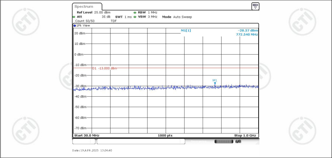
Band25-3MHz-16QAM-26055-1RB#0-Range1:30~1000MHz
