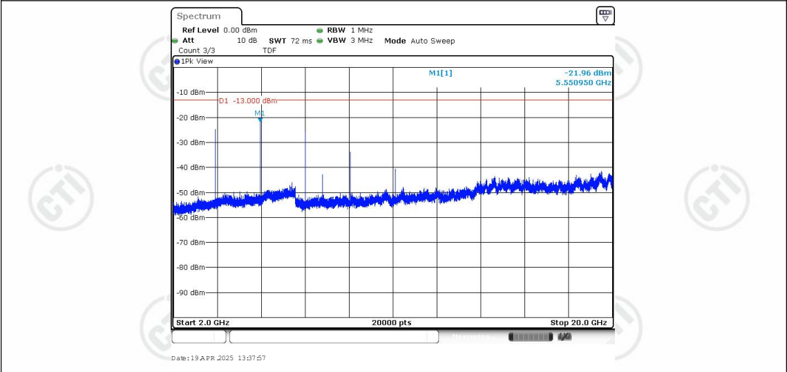
Band25-5MHz-16QAM-26065-1RB#0-Range3:2000~20000MHz
