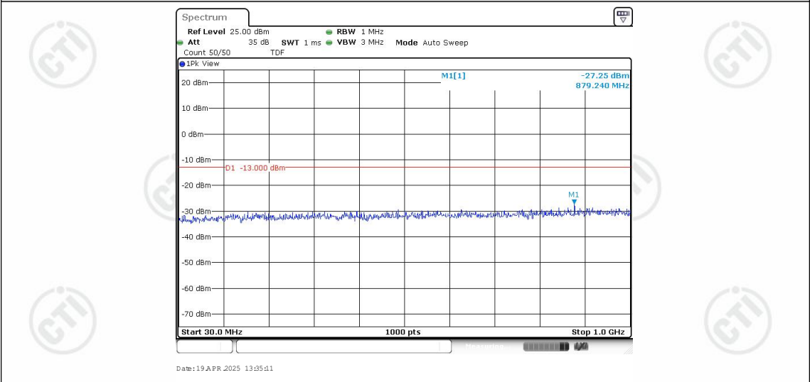
Band25-3MHz-16QAM-26365-1RB#0-Range1:30~1000MHz
