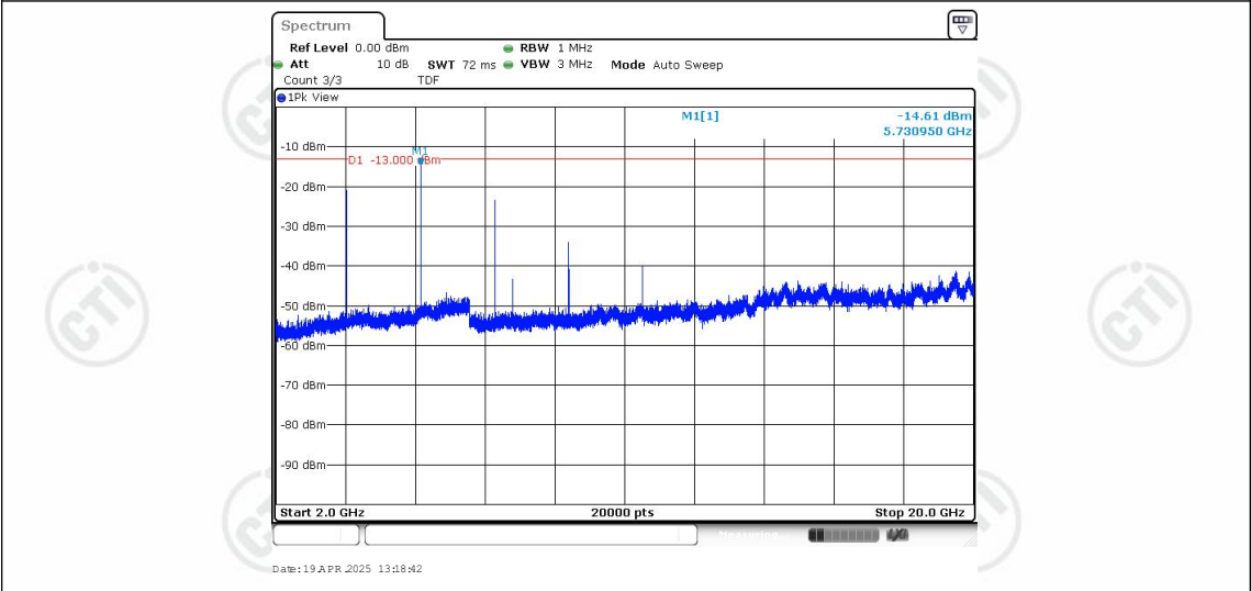
Band25-5MHz-QPSK-26665-1RB#0-Range3:2000~20000MHz
