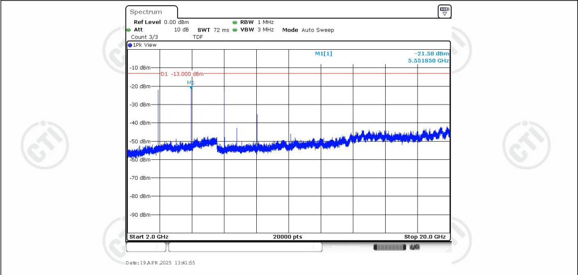
Band25-10MHz-16QAM-26090-1RB#0-Range3:2000~20000MHz
