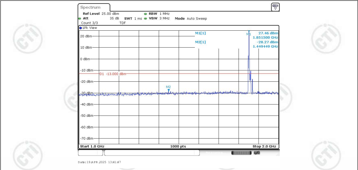
Band25-10MHz-16QAM-26090-1RB#0-Range2:1000~2000MHz
