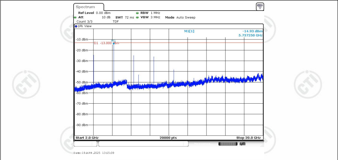
Band25-3MHz-QPSK-26675-1RB#0-Range3:2000~20000MHz
