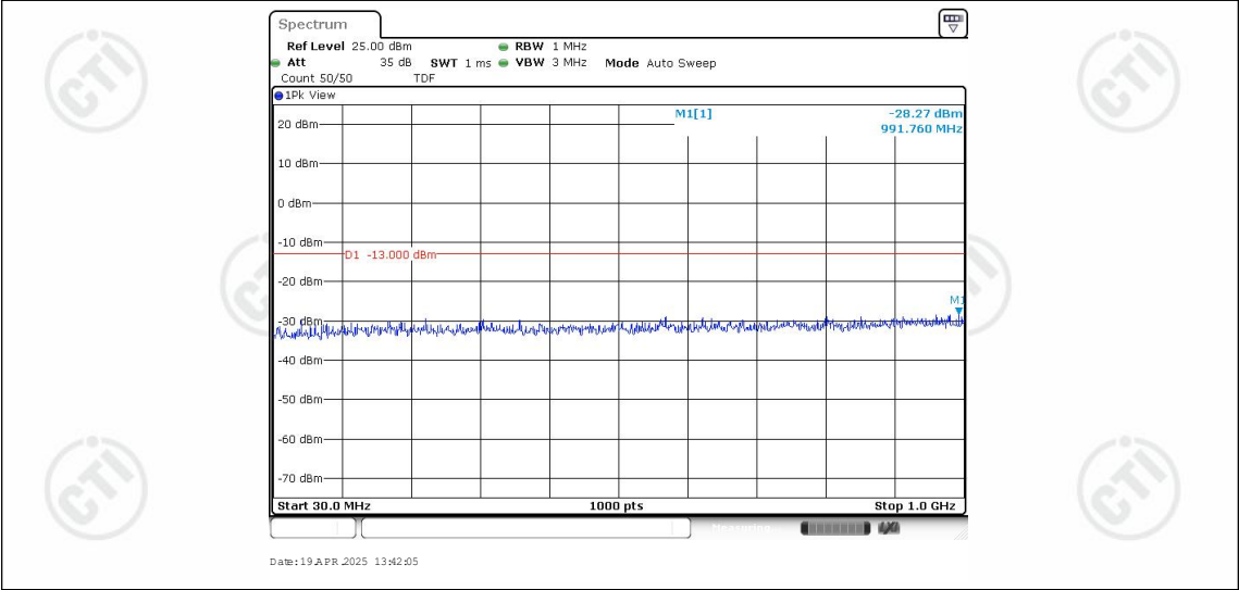
Band25-10MHz-16QAM-26365-1RB#0-Range1:30~1000MHz
