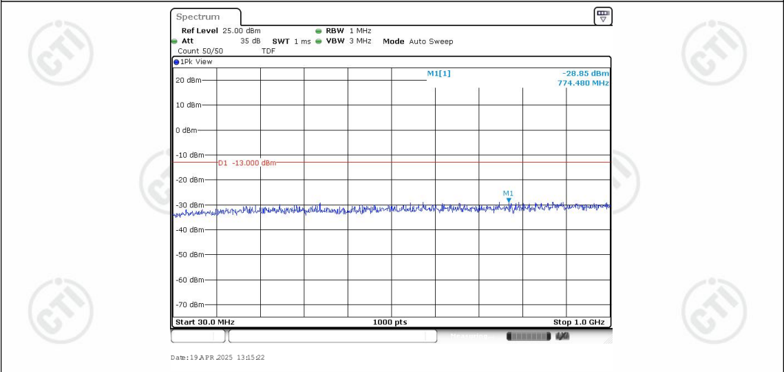
Band25-3MHz-QPSK-26675-1RB#0-Range1:30~1000MHz
