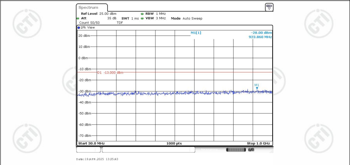
Band25-3MHz-16QAM-26675-1RB#0-Range1:30~1000MHz
