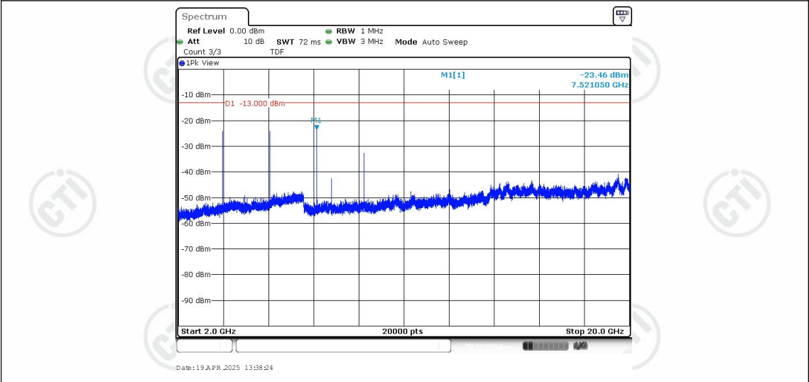
Band25-5MHz-16QAM-26365-1RB#0-Range3:2000~20000MHz
