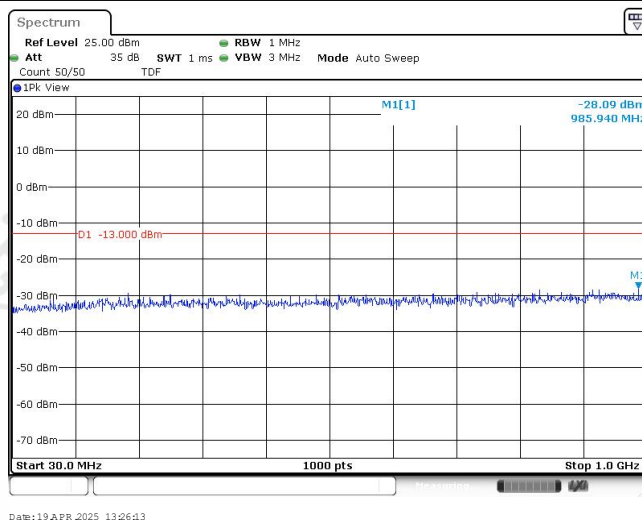
Band25-15MHz-QPSK-26365-1RB#0-Range1:30~1000MHz
