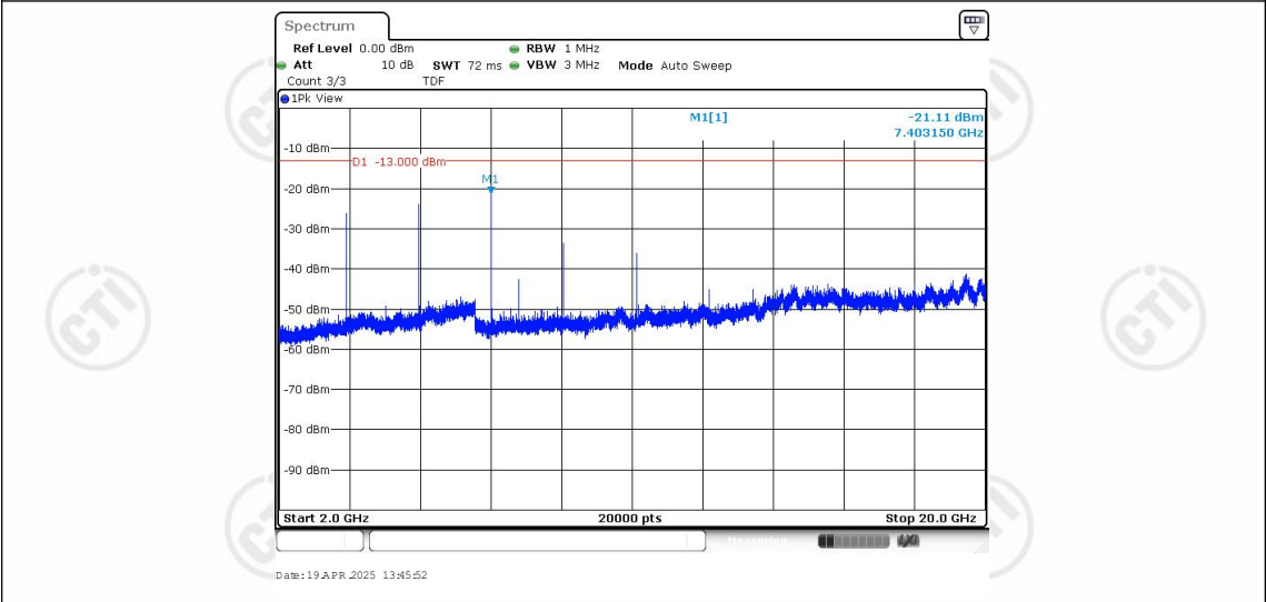
Band25-15MHz-16QAM-26115-1RB#0-Range3:2000~20000MHz
