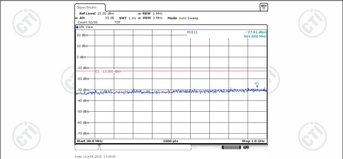
Band25-5MHz-16QAM-26665-1RB#0-Range1:30~1000MHz
