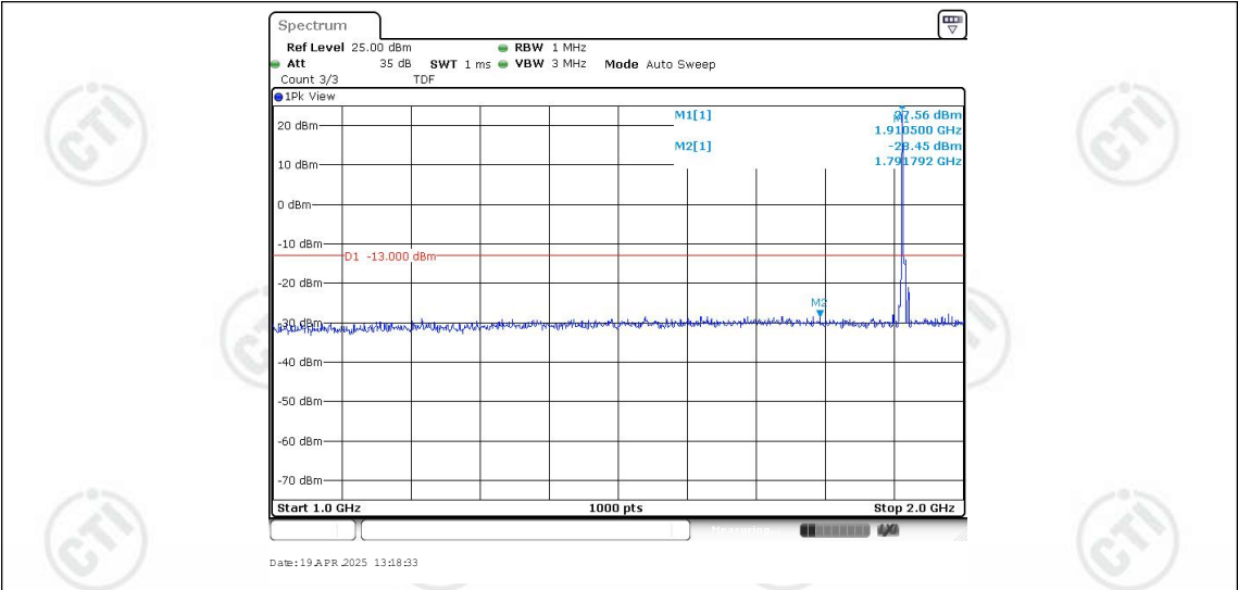
Band25-5MHz-QPSK-26665-1RB#0-Range2:1000~2000MHz
