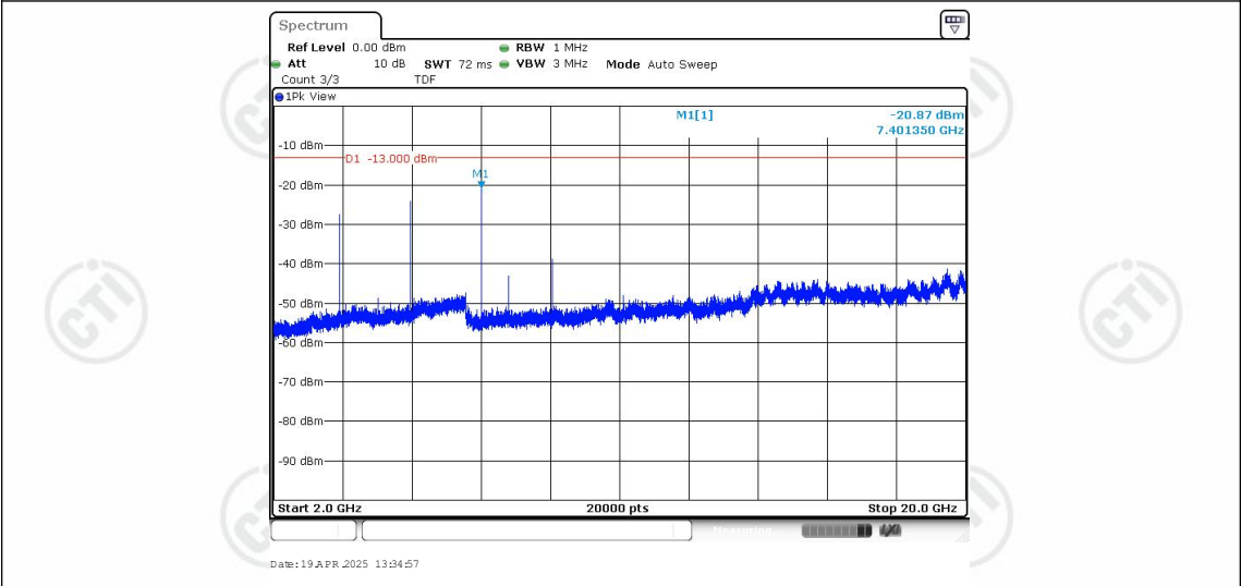
Band25-3MHz-16QAM-26055-1RB#0-Range3:2000~20000MHz
