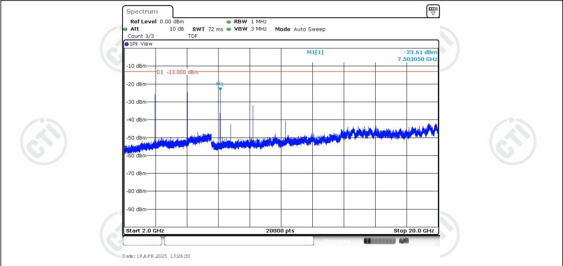
Band25-15MHz-QPSK-26365-1RB#0-Range3:2000~20000MHz
