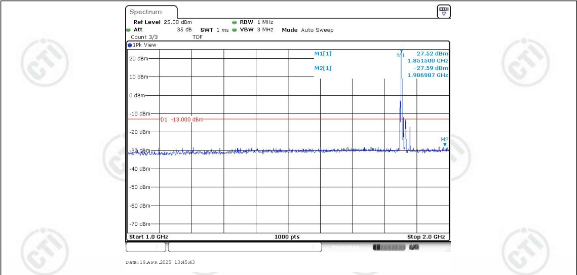
Band25-15MHz-16QAM-26115-1RB#0-Range2:1000~2000MHz
