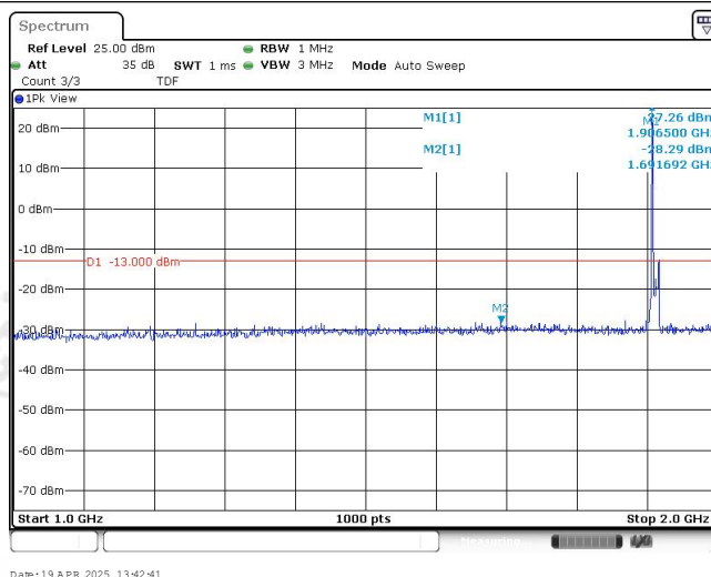
Band25-10MHz-16QAM-26640-1RB#0-Range2:1000~2000MHz
