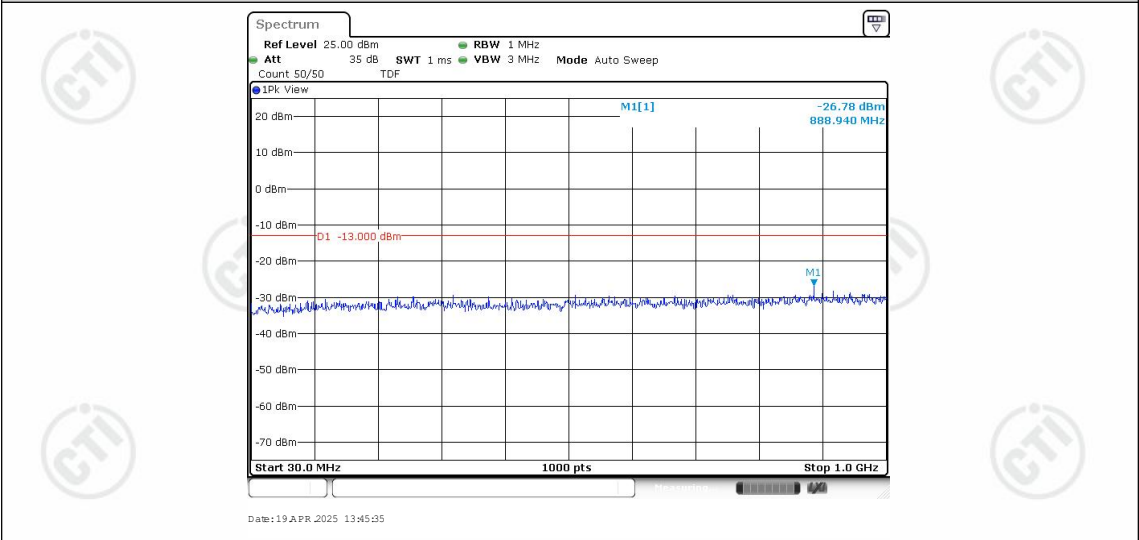
Band25-15MHz-16QAM-26115-1RB#0-Range1:30~1000MHz
