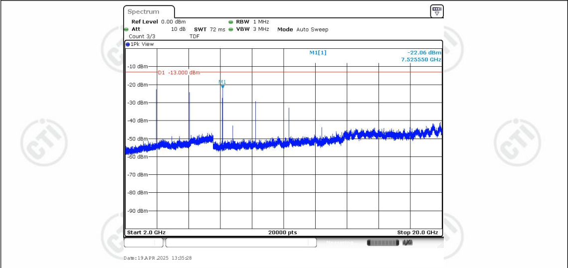
Band25-3MHz-16QAM-26365-1RB#0-Range3:2000~20000MHz
