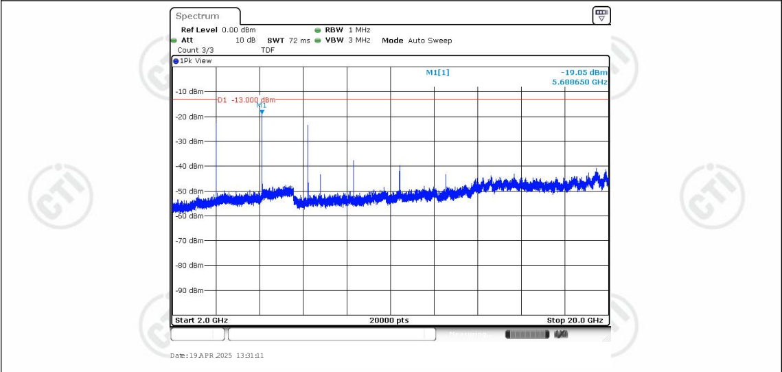
Band25-20MHz-QPSK-26590-1RB#0-Range3:2000~20000MHz
