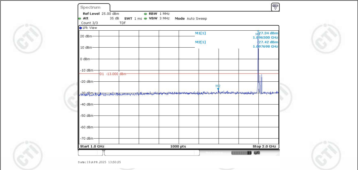
Band25-20MHz-16QAM-26590-1RB#0-Range2:1000~2000MHz
