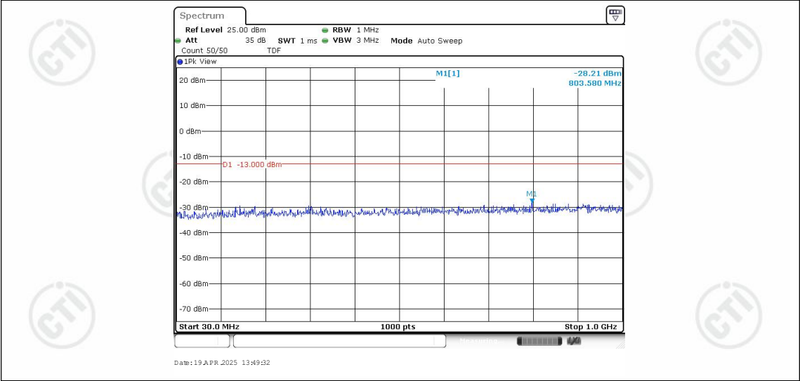
Band25-20MHz-16QAM-26140-1RB#0-Range1:30~1000MHz
