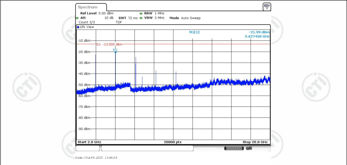
Band25-15MHz-16QAM-26365-1RB#0-Range3:2000~20000MHz
