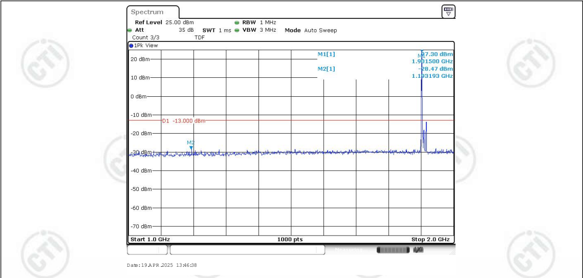
Band25-15MHz-16QAM-26615-1RB#0-Range2:1000~2000MHz
