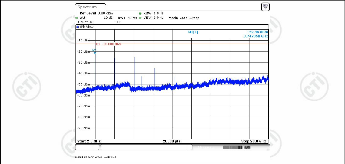
Band25-20MHz-16QAM-26365-1RB#0-Range3:2000~20000MHz
