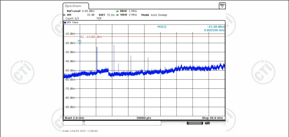
Band25-15MHz-16QAM-26615-1RB#0-Range3:2000~20000MHz
