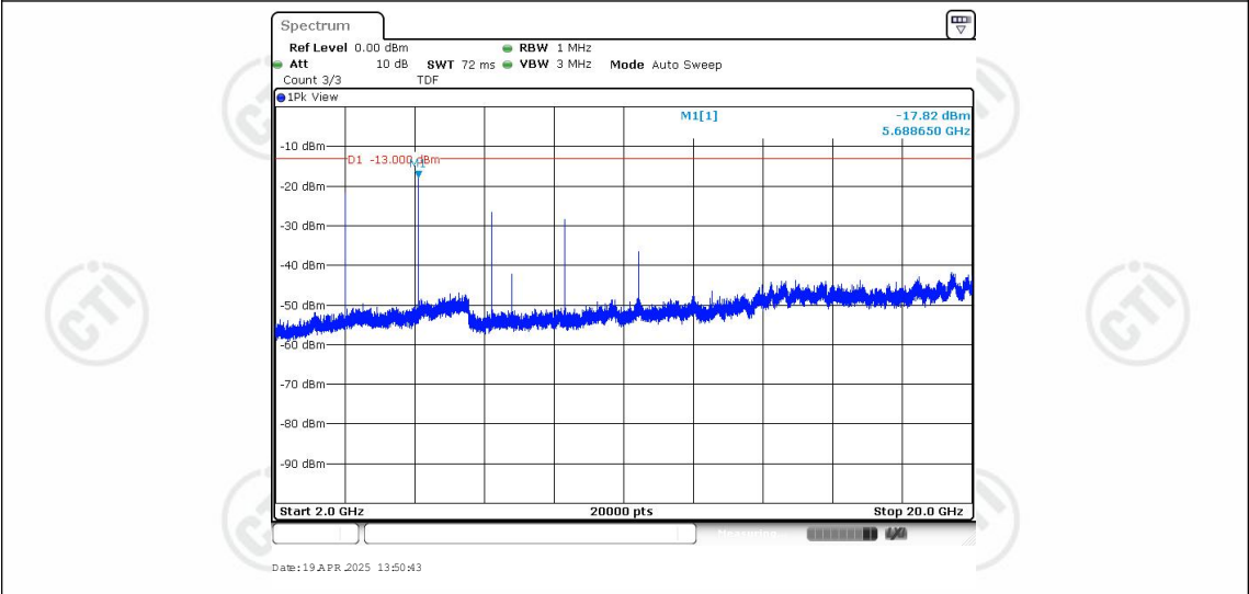
Band25-20MHz-16QAM-26590-1RB#0-Range3:2000~20000MHz
