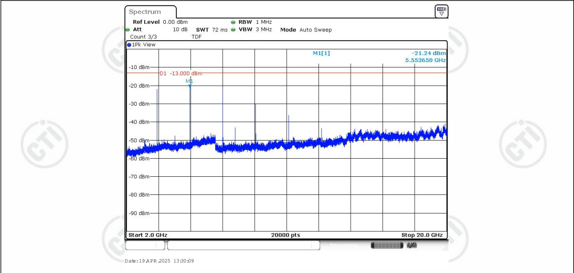
Band25-20MHz-QPSK-26140-1RB#0-Range3:2000~20000MHz
