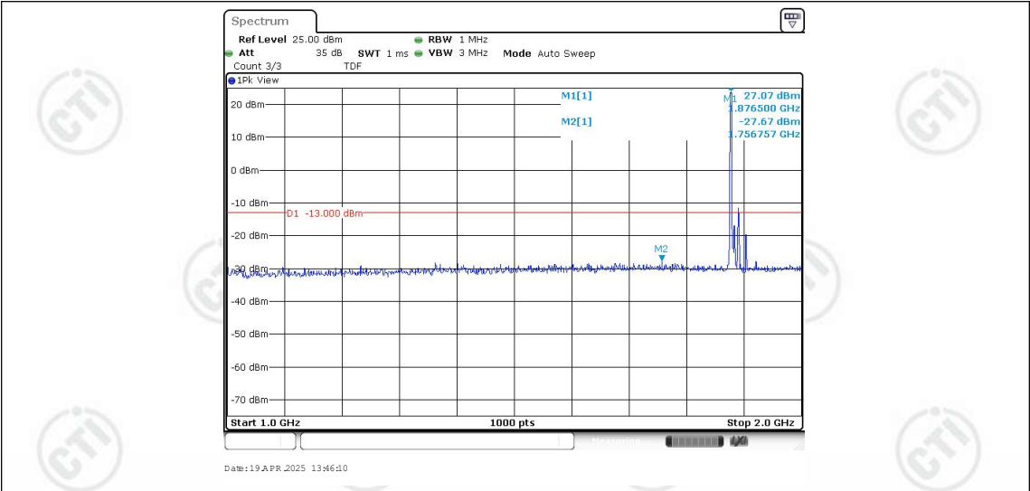
Band25-15MHz-16QAM-26365-1RB#0-Range2:1000~2000MHz
