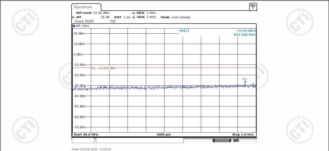
Band25-20MHz-QPSK-26590-1RB#0-Range1:30~1000MHz
