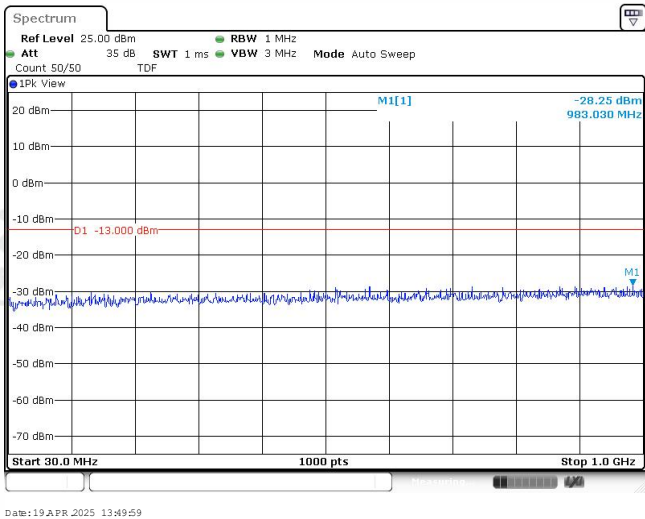
Band25-20MHz-16QAM-26365-1RB#0-Range1:30~1000MHz
