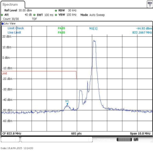
Band26-1.4MHz-16QAM-26785-1RB#5
