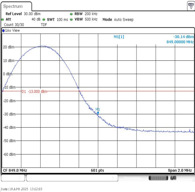
Band26-10MHz-16QAM-26990-1RB#49
