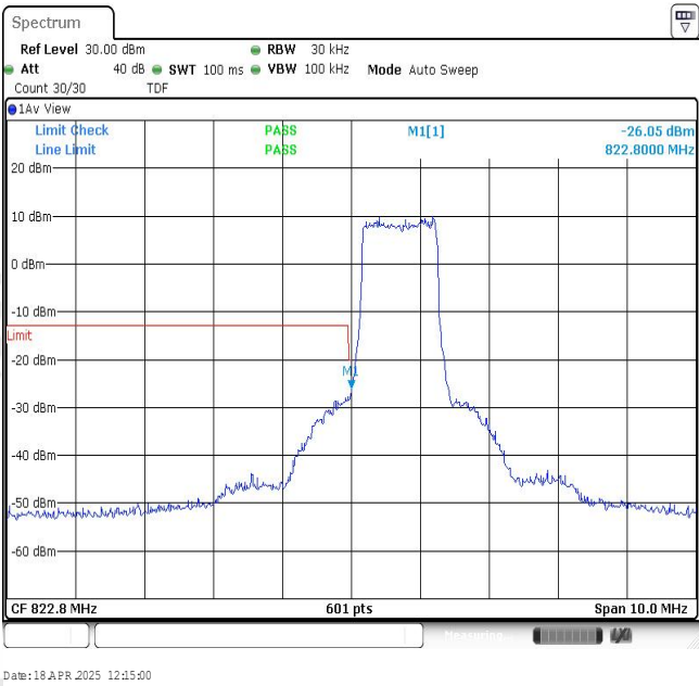
Band26-1.4MHz-QPSK-26785-6RB#0
