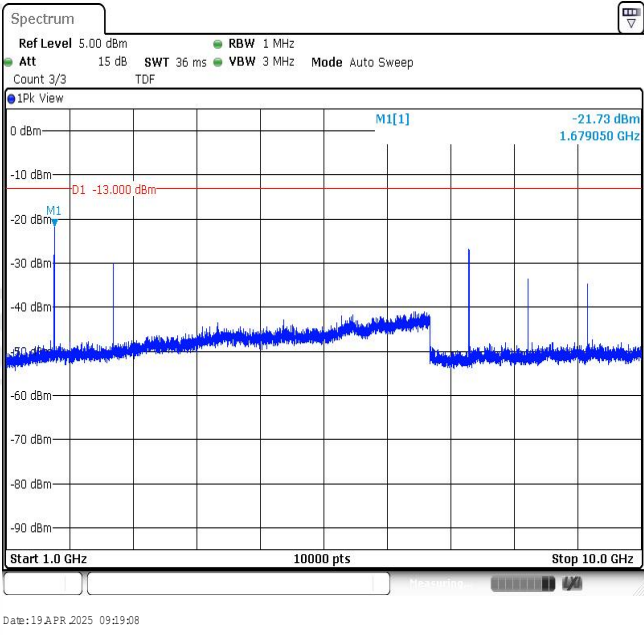
Band26-10MHz-16QAM-26990-1RB#0-Range2:1000~10000MHz
