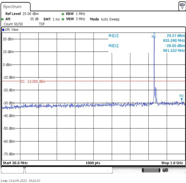
Band26-15MHz-QPSK-26965-1RB#0-Range1:30~1000MHz
