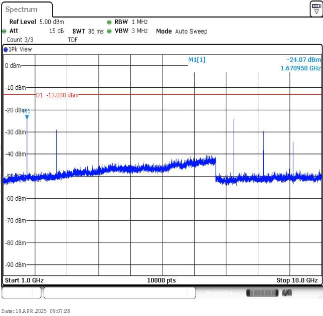
Band26-1.4MHz-16QAM-26909-1RB#0-Range2:1000~10000MHz
