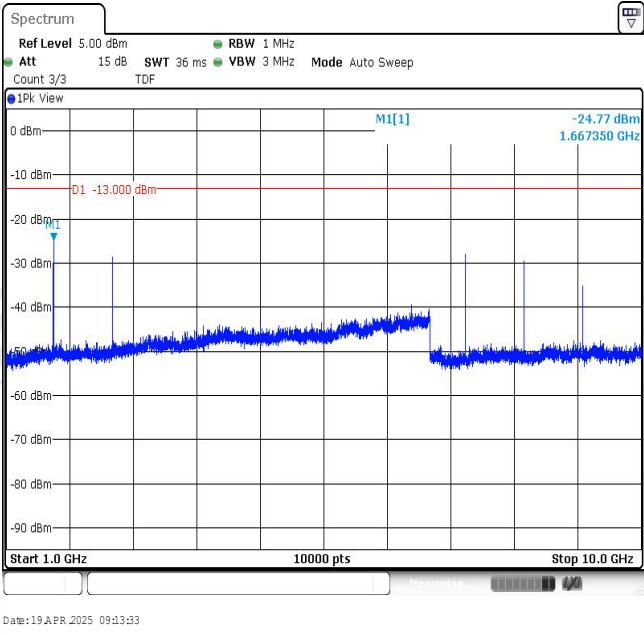
Band26-5MHz-QPSK-26909-1RB#0-Range2:1000~10000MHz
