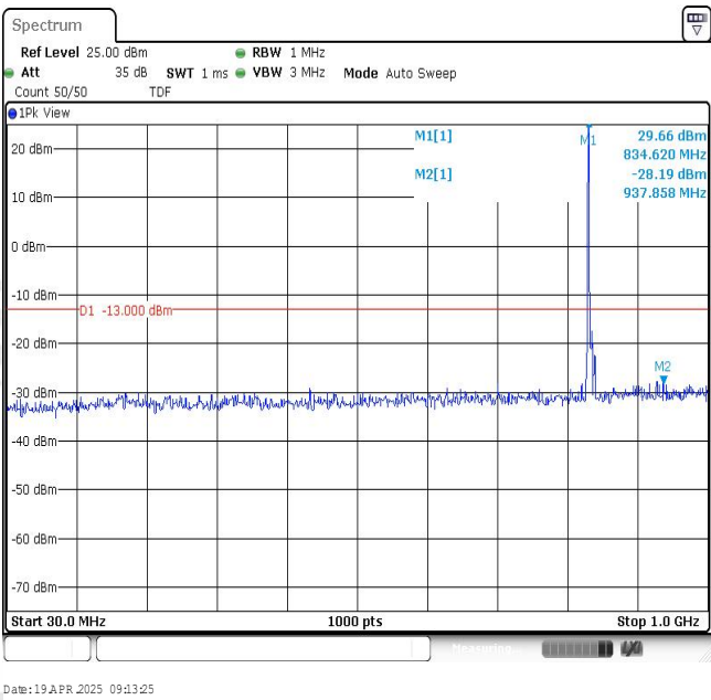
Band26-5MHz-QPSK-26909-1RB#0-Range1:30~1000MHz
