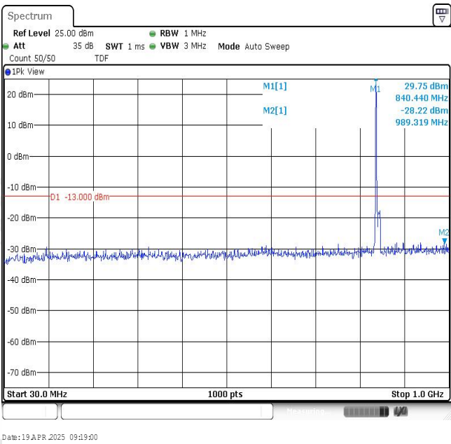
Band26-10MHz-16QAM-26990-1RB#0-Range1:30~1000MHz
