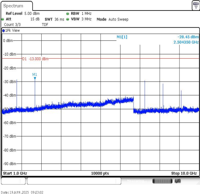
Band26-15MHz-QPSK-26965-1RB#0-Range2:1000~10000MHz
