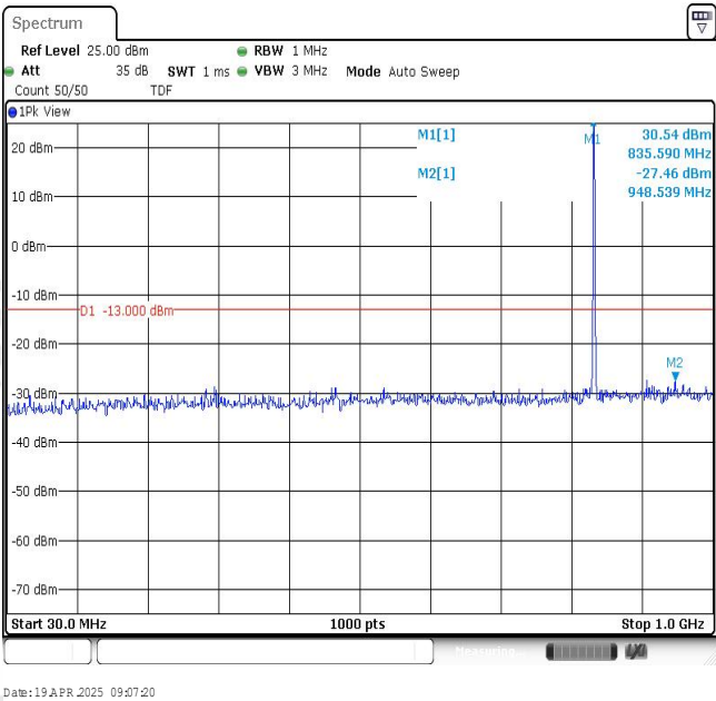
Band26-1.4MHz-16QAM-26909-1RB#0-Range1:30~1000MHz
