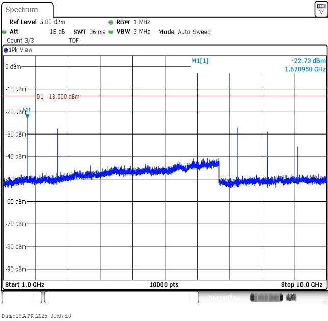
Band26-1.4MHz-QPSK-26909-1RB#0-Range2:1000~10000MHz
