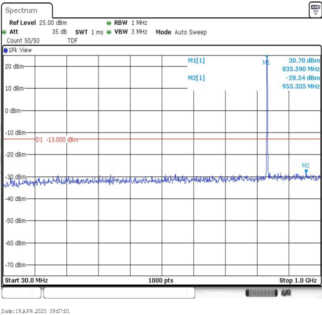
Band26-1.4MHz-QPSK-26909-1RB#0-Range1:30~1000MHz
