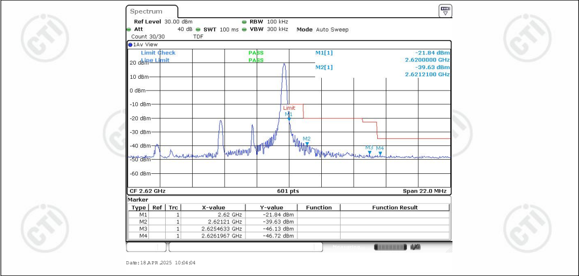
Band38-5MHz-16QAM-38225-1RB#24
