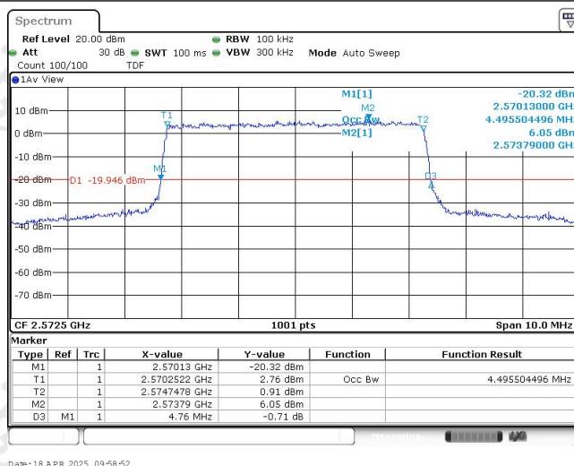
Band38-5MHz-16QAM-37775-25RB#0-4.496
