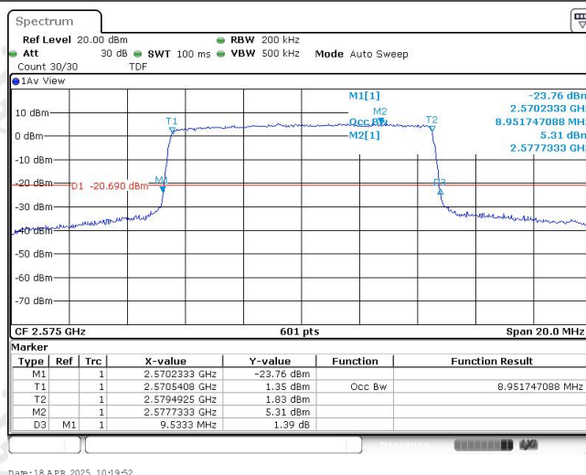
Band38-10MHz-QPSK-37800-50RB#0-8.952
