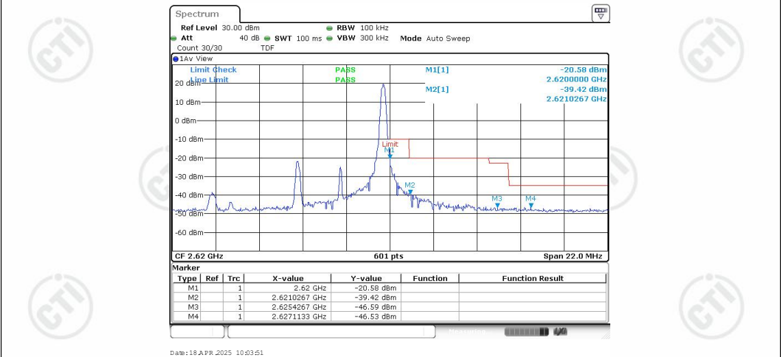
Band38-5MHz-QPSK-38225-1RB#24
