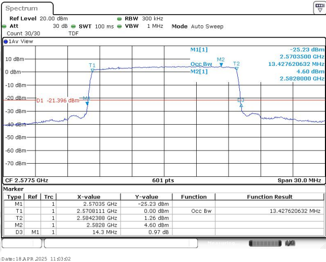
Band38-15MHz-QPSK-37825-75RB#0-13.428
