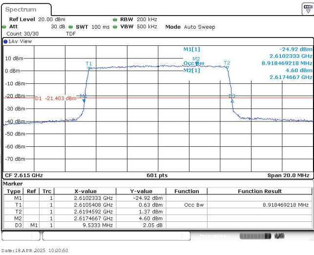
Band38-10MHz-16QAM-38200-50RB#0-8.918
