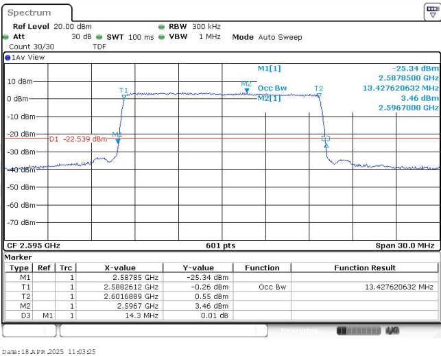
Band38-15MHz-QPSK-38000-75RB#0-13.428
