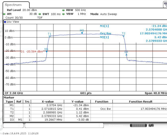
Band38-20MHz-16QAM-37850-100RB#0-17.903
