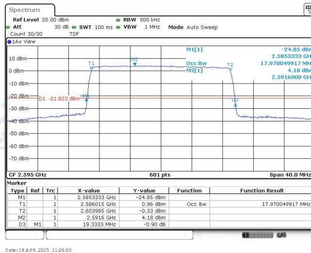
Band38-20MHz-16QAM-38000-100RB#0-17.97
