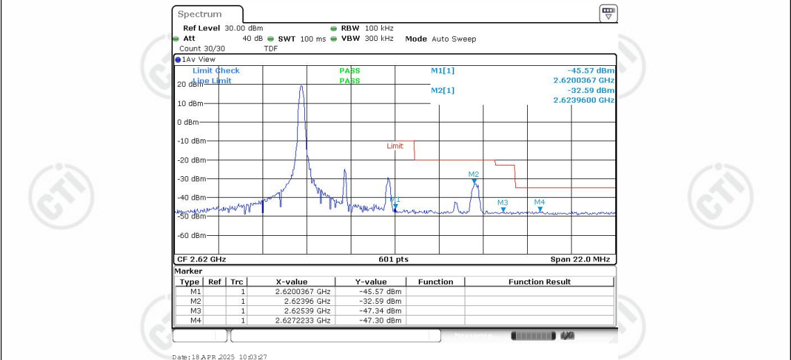
Band38-5MHz-QPSK-38225-1RB#0
