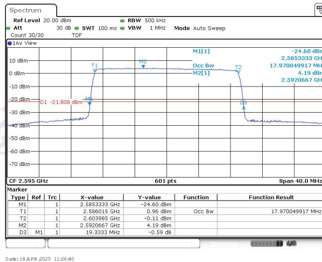
Band38-20MHz-QPSK-38000-100RB#0-17.97
