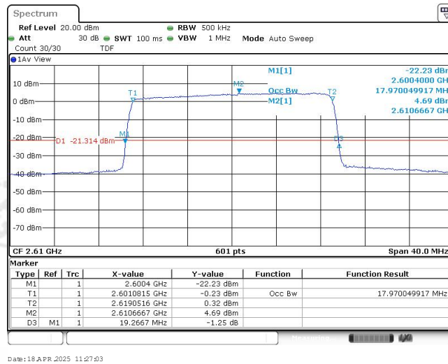
Band38-20MHz-QPSK-38150-100RB#0-17.97
