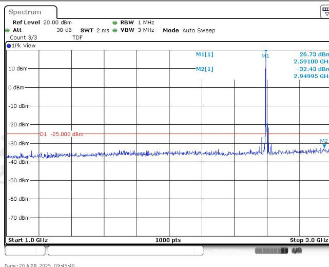
Band38-10MHz-QPSK-38000-1RB#0-Range2:1000~3000MHz
