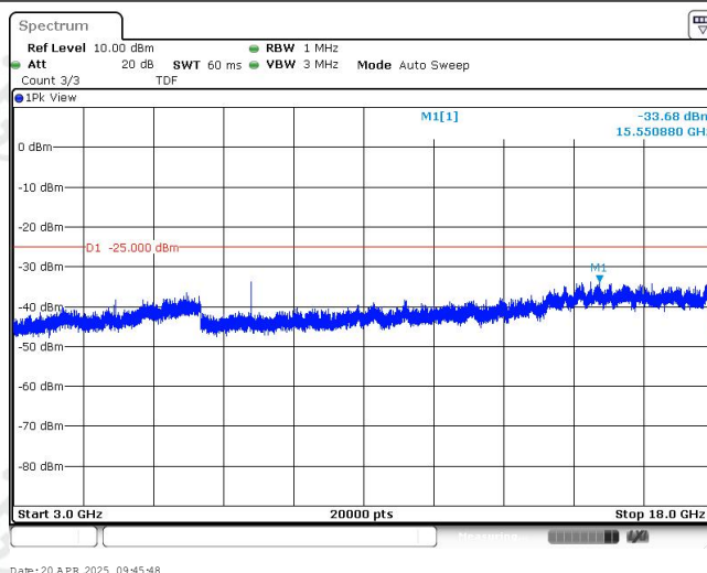
Band38-10MHz-QPSK-38000-1RB#0-Range3:3000~18000MHz
