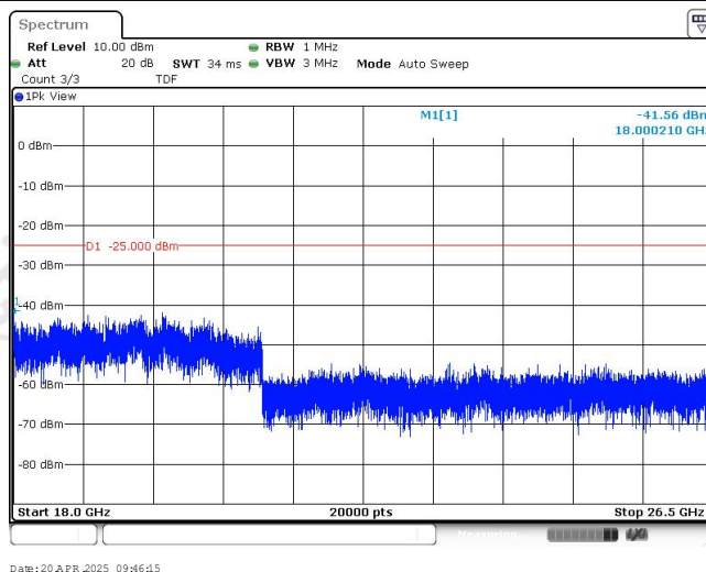
Band38-10MHz-QPSK-38000-1RB#0-Range4:18000~26500MHz
