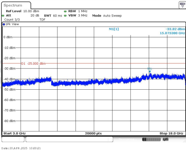
Band38-20MHz-QPSK-38150-1RB#0-Range3:3000~18000MHz
