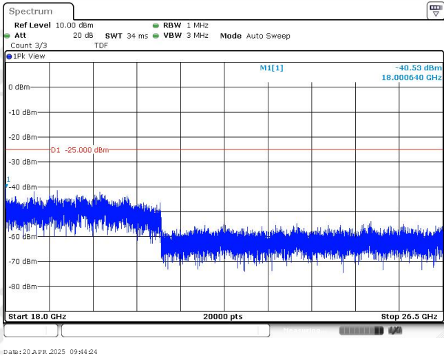
Band38-10MHz-QPSK-37800-1RB#0-Range4:18000~26500MHz
