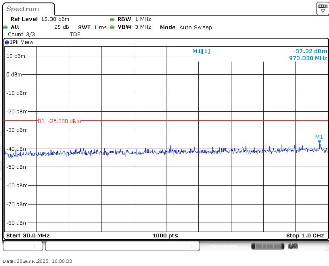
Band38-20MHz-QPSK-38150-1RB#0-Range1:30~1000MHz
