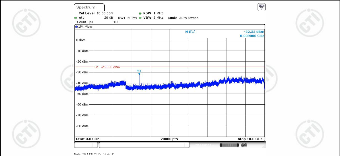
Band38-10MHz-QPSK-38200-1RB#0-Range3:3000~18000MHz
