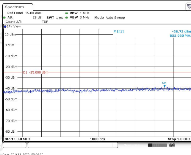
Band38-20MHz-QPSK-37850-1RB#0-Range1:30~1000MHz
