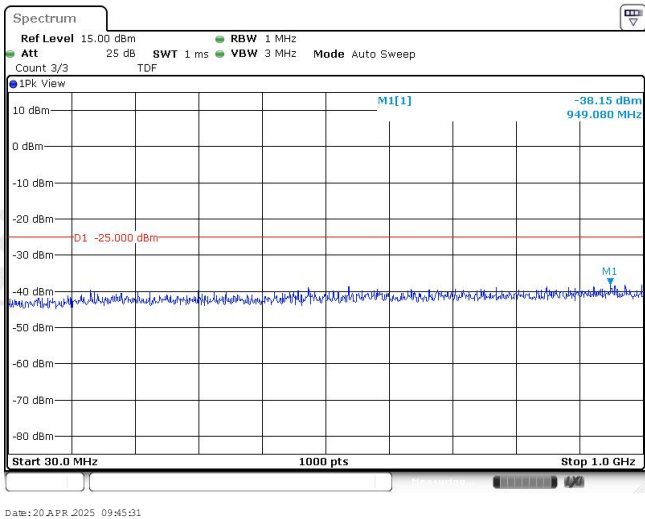
Band38-10MHz-QPSK-38000-1RB#0-Range1:30~1000MHz
