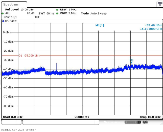
Band38-10MHz-QPSK-37800-1RB#0-Range3:3000~18000MHz
