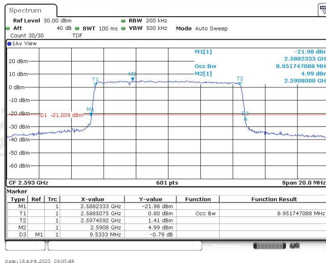
Band41-10MHz-QPSK-40620-50RB#0-8.952
