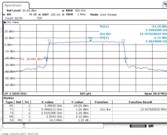
Band41-15MHz-QPSK-39725-75RB#0-13.428
