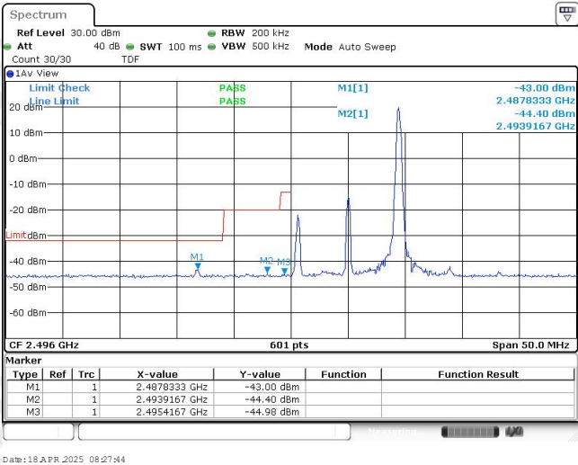
Band41-10MHz-16QAM-39700-1RB#49
