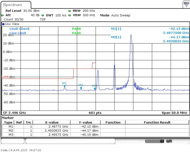
Band41-10MHz-QPSK-39700-1RB#49
