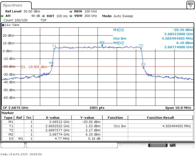
Band41-5MHz-QPSK-41565-25RB#0-4.505
