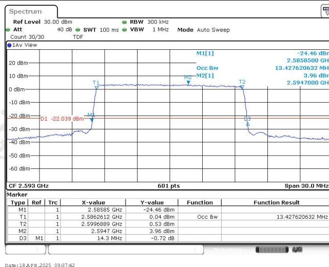
Band41-15MHz-QPSK-40620-75RB#0-13.428
