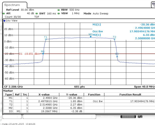
Band41-20MHz-QPSK-39750-100RB#0-17.903
