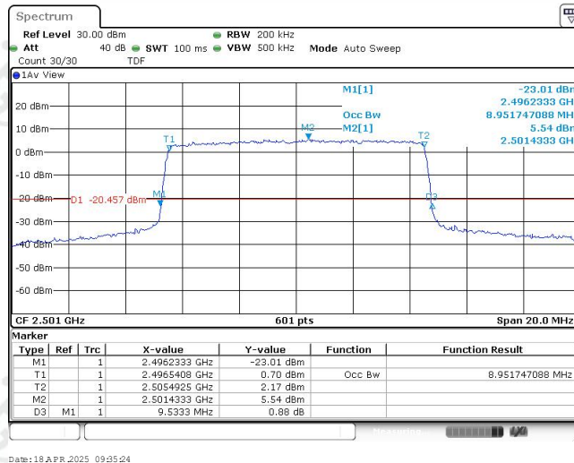
Band41-10MHz-QPSK-39700-50RB#0-8.952
