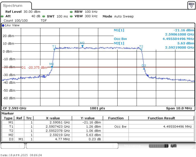
Band41-5MHz-16QAM-40620-25RB#0-4.496
