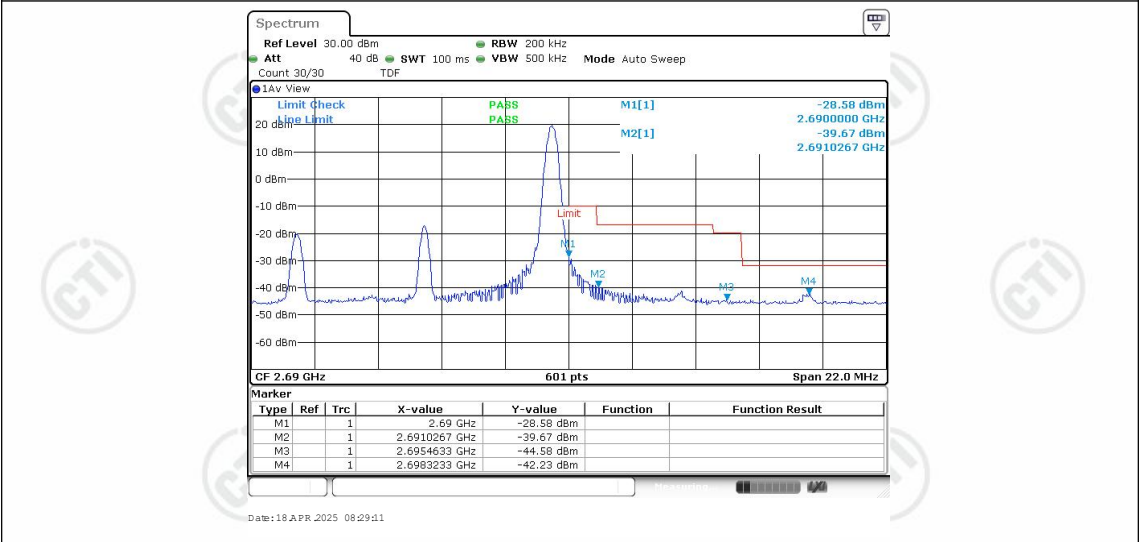
Band41-10MHz-16QAM-41540-1RB#49
