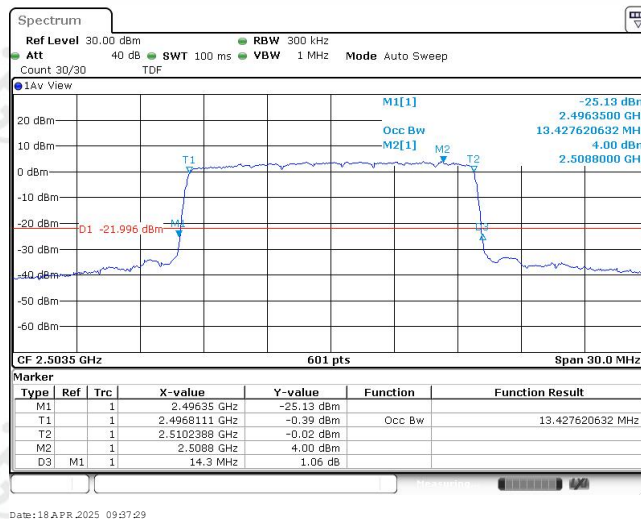
Band41-15MHz-16QAM-39725-75RB#0-13.428
