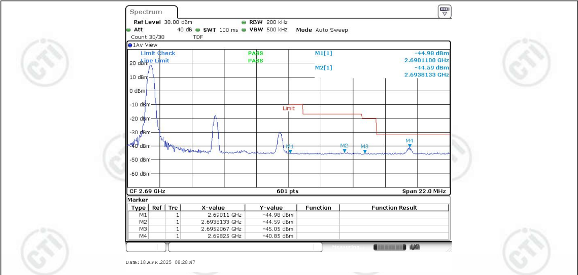
Band41-10MHz-16QAM-41540-1RB#0
