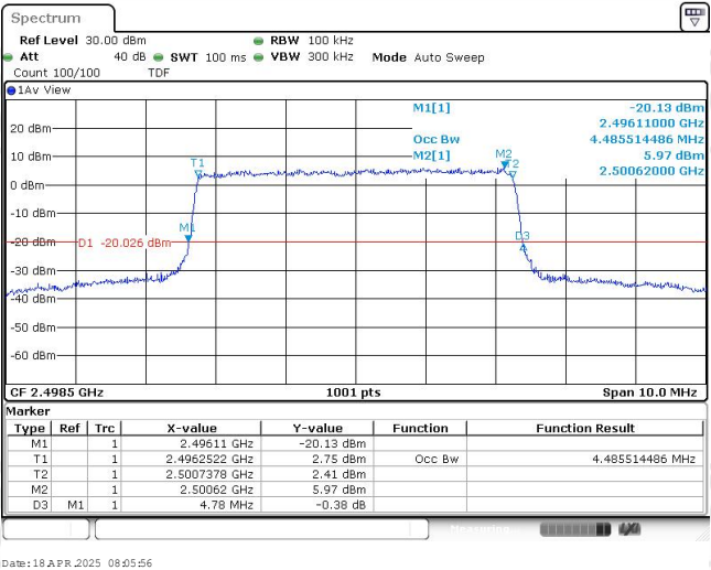
Band41-5MHz-16QAM-39675-25RB#0-4.486
