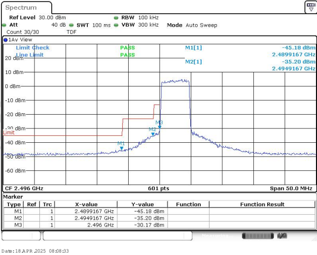
Band41-5MHz-16QAM-39675-25RB#0
