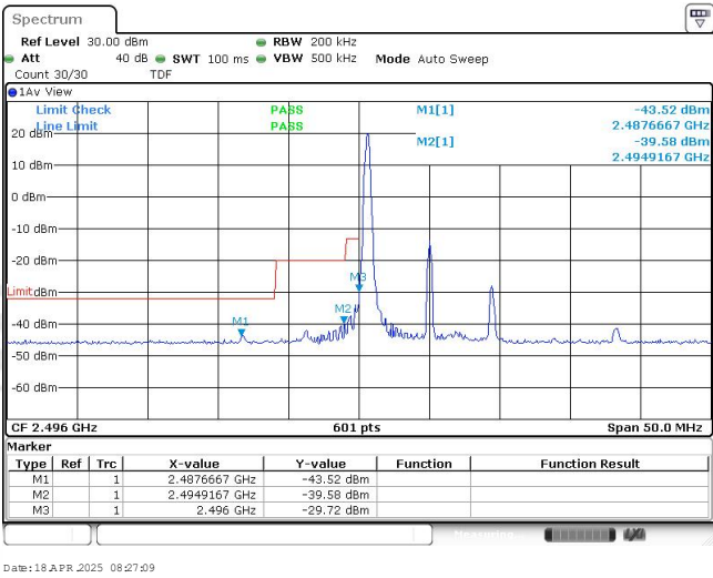
Band41-10MHz-QPSK-39700-1RB#0
