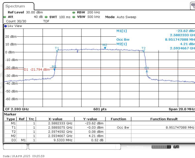
Band41-10MHz-16QAM-40620-50RB#0-8.952
