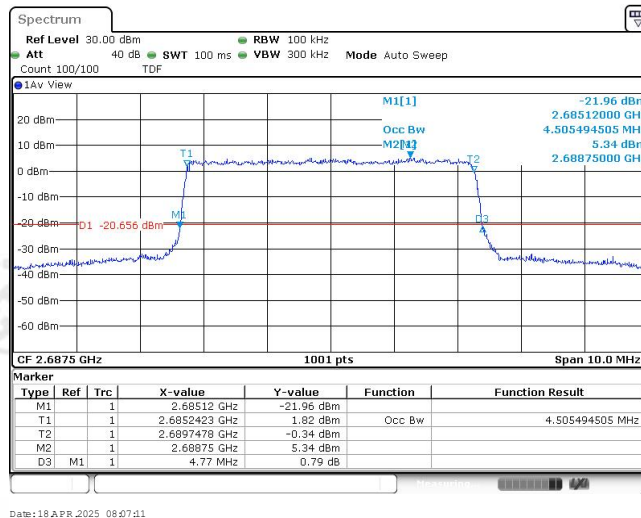
Band41-5MHz-16QAM-41565-25RB#0-4.505
