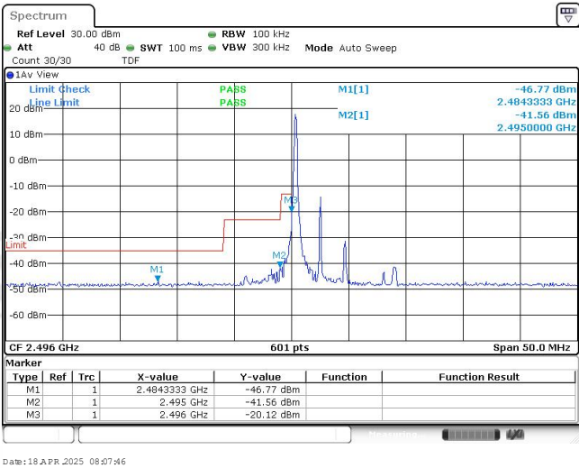
Band41-5MHz-16QAM-39675-1RB#0
