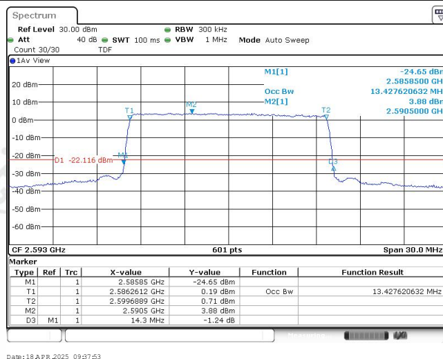
Band41-15MHz-16QAM-40620-75RB#0-13.428
