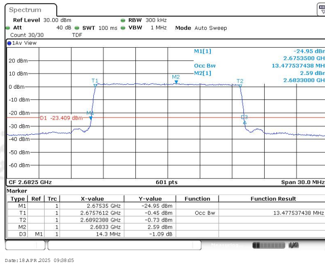
Band41-15MHz-QPSK-41515-75RB#0-13.478
