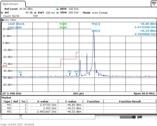
Band41-5MHz-16QAM-39675-1RB#24
