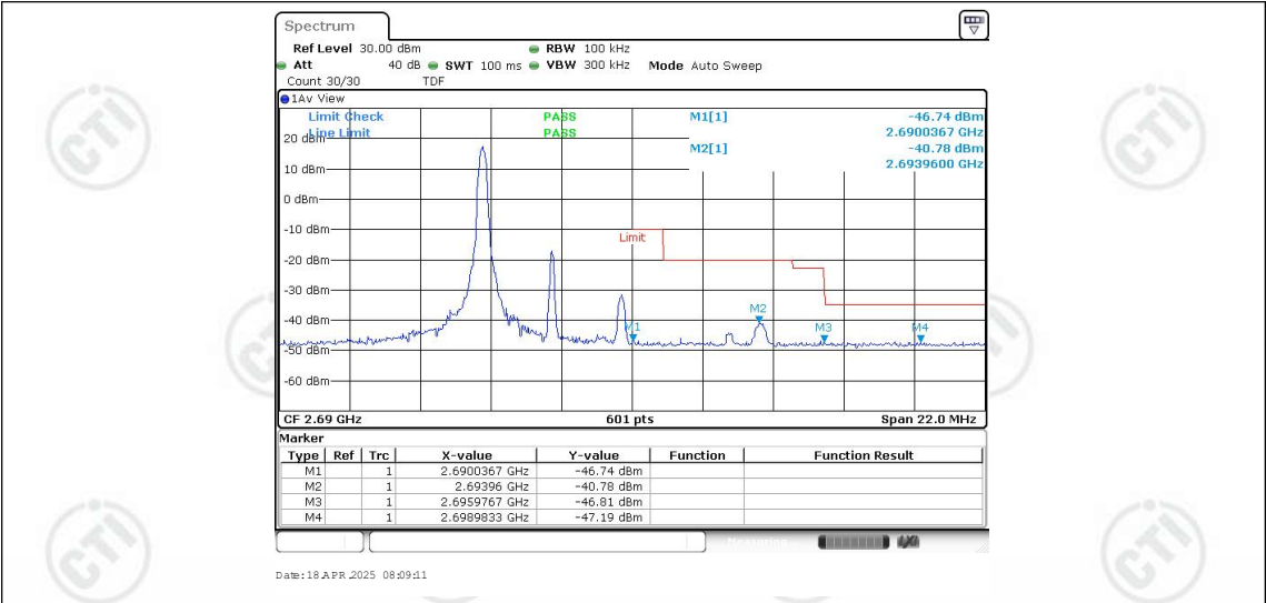
Band41-5MHz-16QAM-41565-1RB#0
