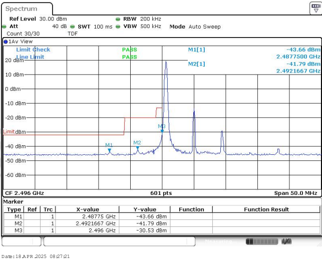
Band41-10MHz-16QAM-39700-1RB#0
