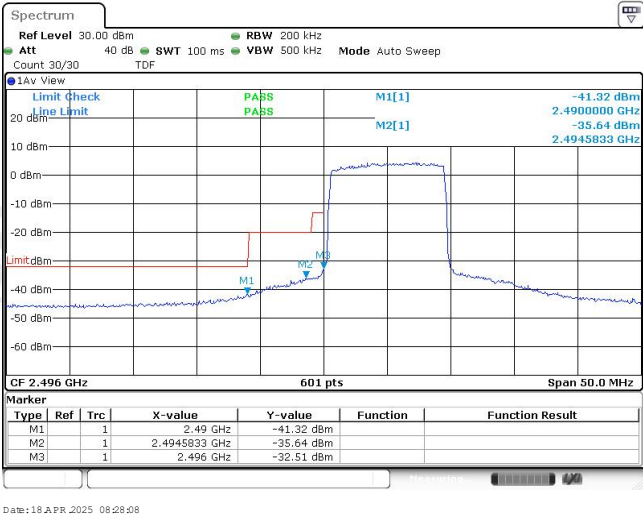
Band41-10MHz-16QAM-39700-50RB#0
