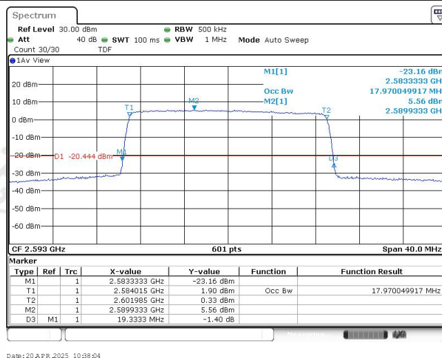
Band41-20MHz-QPSK-40620-100RB#0-17.97
