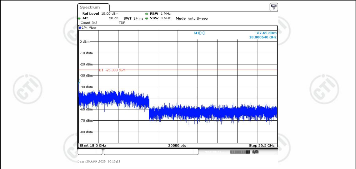
Band41-10MHz-QPSK-40620-1RB#0-Range4:18000~26500MHz
