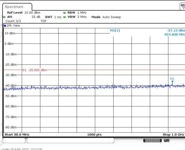
Band41-10MHz-QPSK-40620-1RB#0-Range1:30~1000MHz
