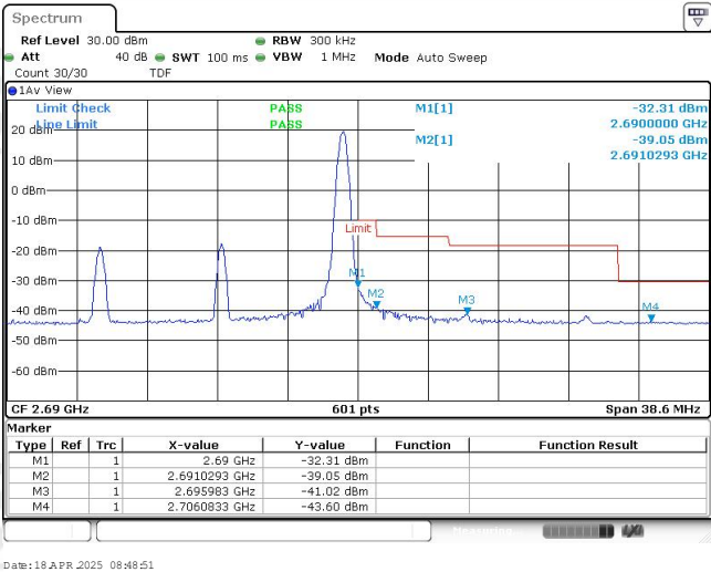
Band41-15MHz-16QAM-41515-1RB#74
