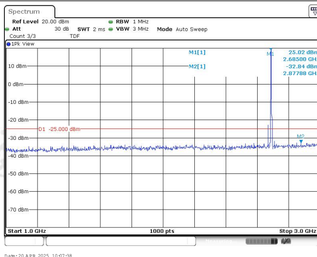
Band41-5MHz-16QAM-41565-1RB#0-Range2:1000~3000MHz
