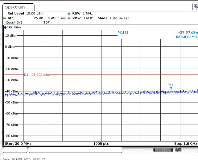
Band41-5MHz-16QAM-40620-1RB#0-Range1:30~1000MHz
