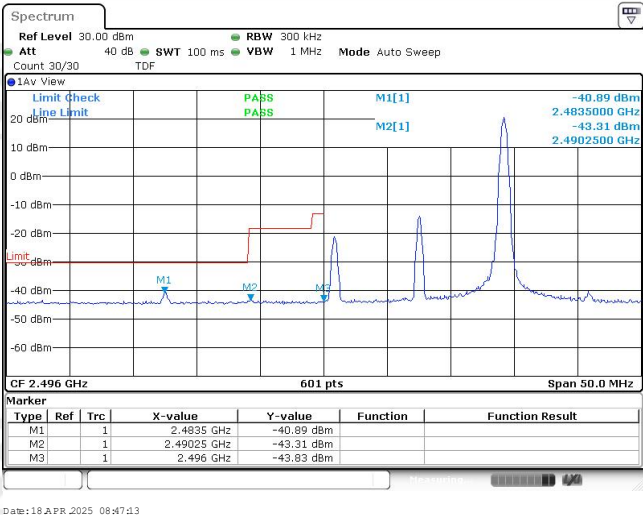
Band41-15MHz-QPSK-39725-1RB#74
