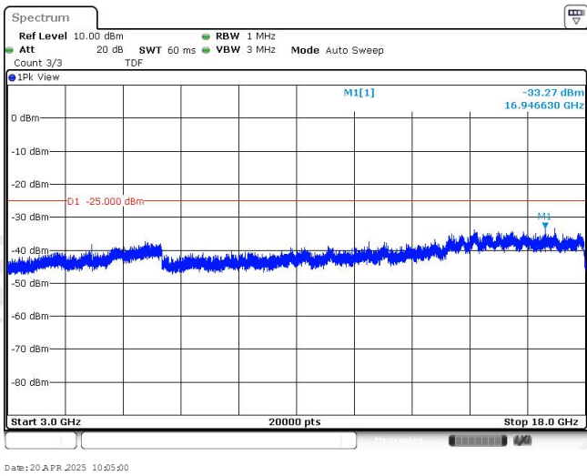
Band41-5MHz-QPSK-40620-1RB#0-Range3:3000~18000MHz
