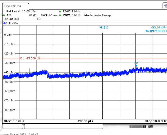
Band41-5MHz-16QAM-41565-1RB#0-Range3:3000~18000MHz
