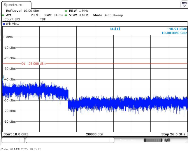
Band41-5MHz-QPSK-40620-1RB#0-Range4:18000~26500MHz
