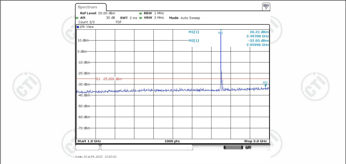
Band41-5MHz-16QAM-39675-1RB#0-Range2:1000~3000MHz
