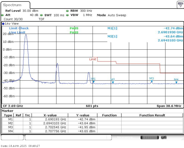
Band41-15MHz-16QAM-41515-1RB#0
