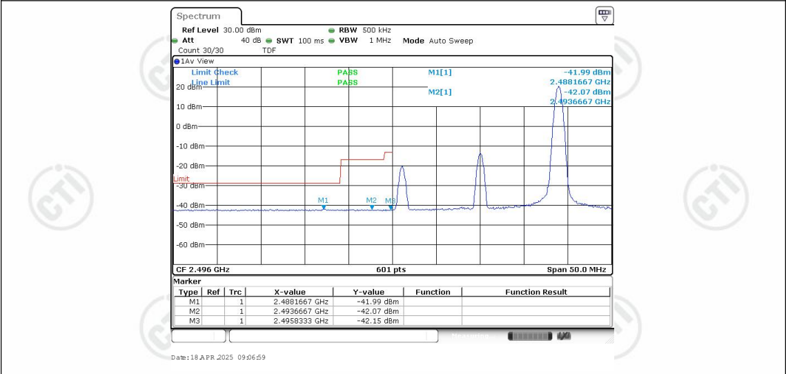
Band41-20MHz-16QAM-39750-1RB#99
