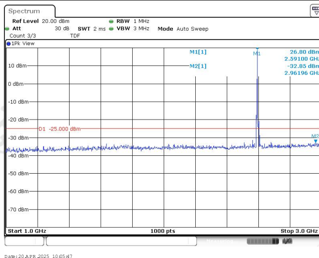
Band41-5MHz-16QAM-40620-1RB#0-Range2:1000~3000MHz
