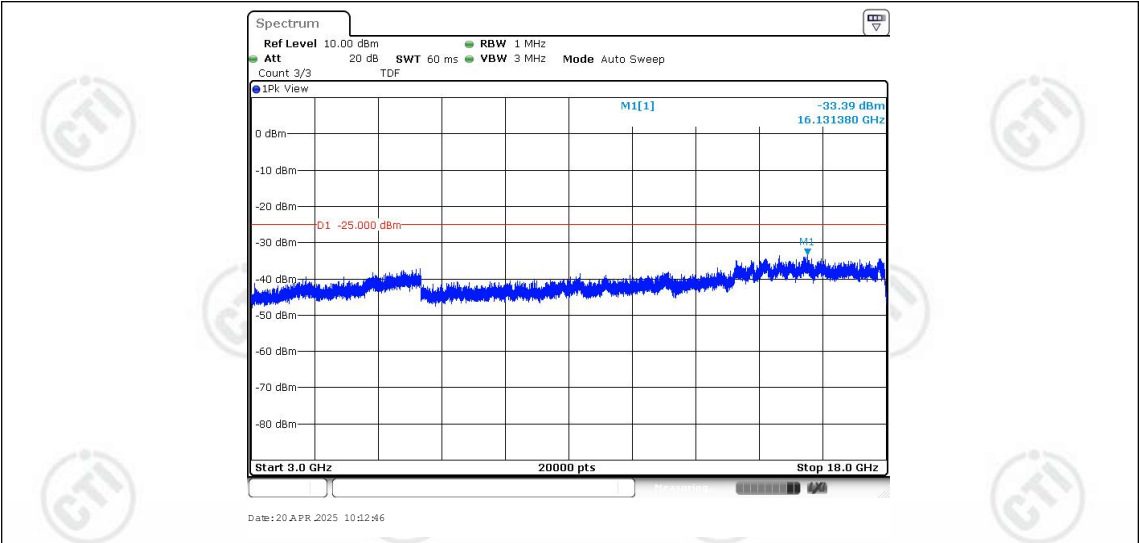
Band41-10MHz-QPSK-40620-1RB#0-Range3:3000~18000MHz
