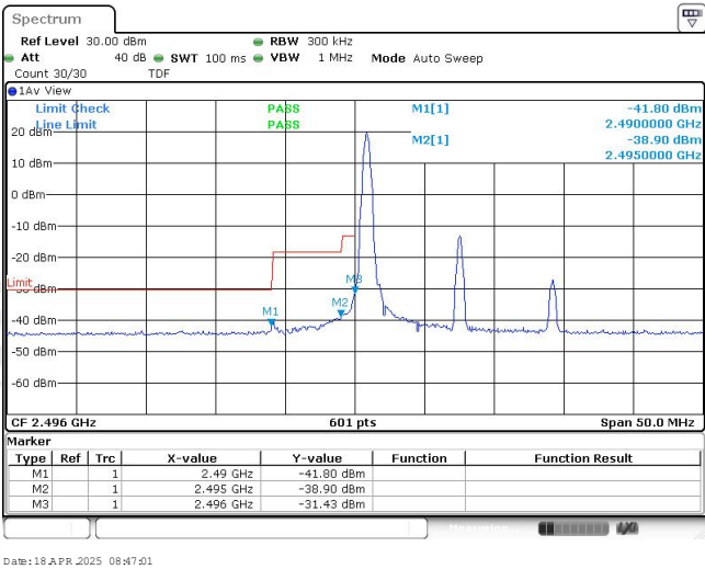
Band41-15MHz-16QAM-39725-1RB#0
