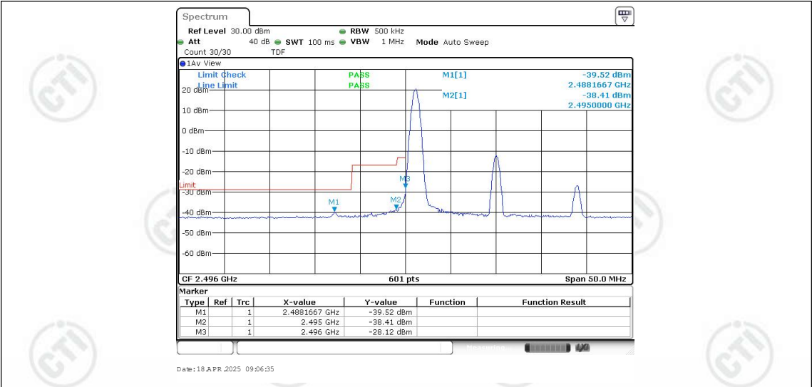
Band41-20MHz-16QAM-39750-1RB#0
