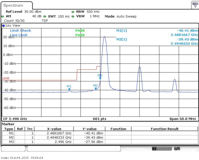
Band41-20MHz-QPSK-39750-1RB#0
