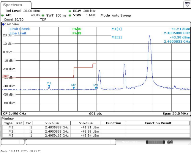
Band41-15MHz-16QAM-39725-1RB#74
