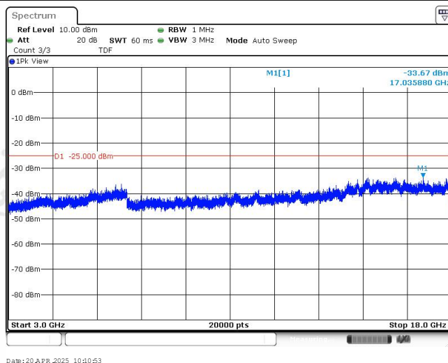
Band41-10MHz-QPSK-39700-1RB#0-Range3:3000~18000MHz
