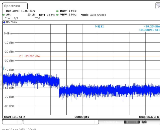
Band41-5MHz-16QAM-39675-1RB#0-Range4:18000~26500MHz
