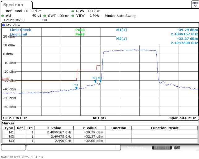
Band41-15MHz-QPSK-39725-75RB#0
