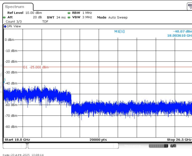
Band41-5MHz-16QAM-41565-1RB#0-Range4:18000~26500MHz
