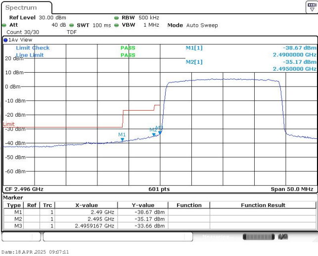
Band41-20MHz-QPSK-39750-100RB#0
