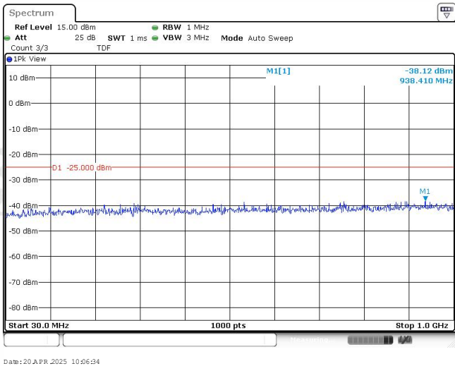
Band41-5MHz-QPSK-41565-1RB#0-Range1:30~1000MHz
