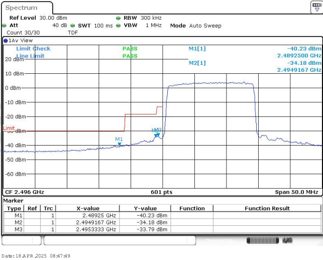
Band41-15MHz-16QAM-39725-75RB#0
