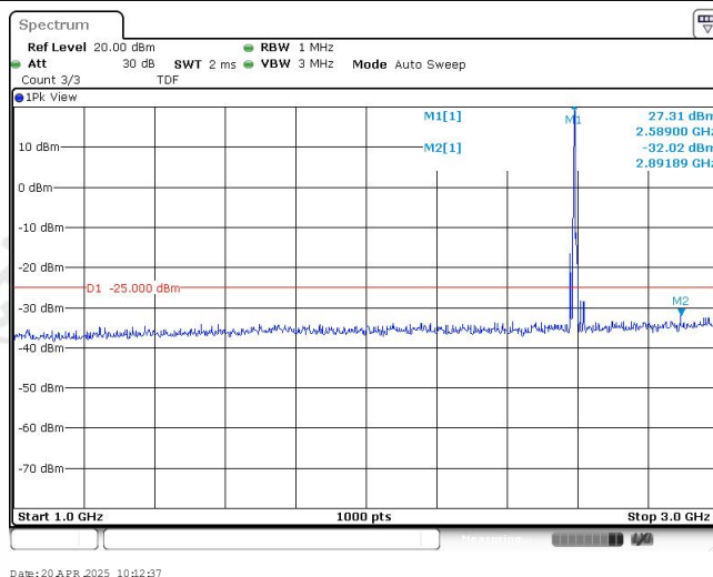
Band41-10MHz-QPSK-40620-1RB#0-Range2:1000~3000MHz
