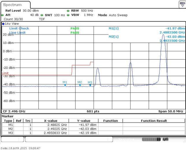
Band41-20MHz-QPSK-39750-1RB#99
