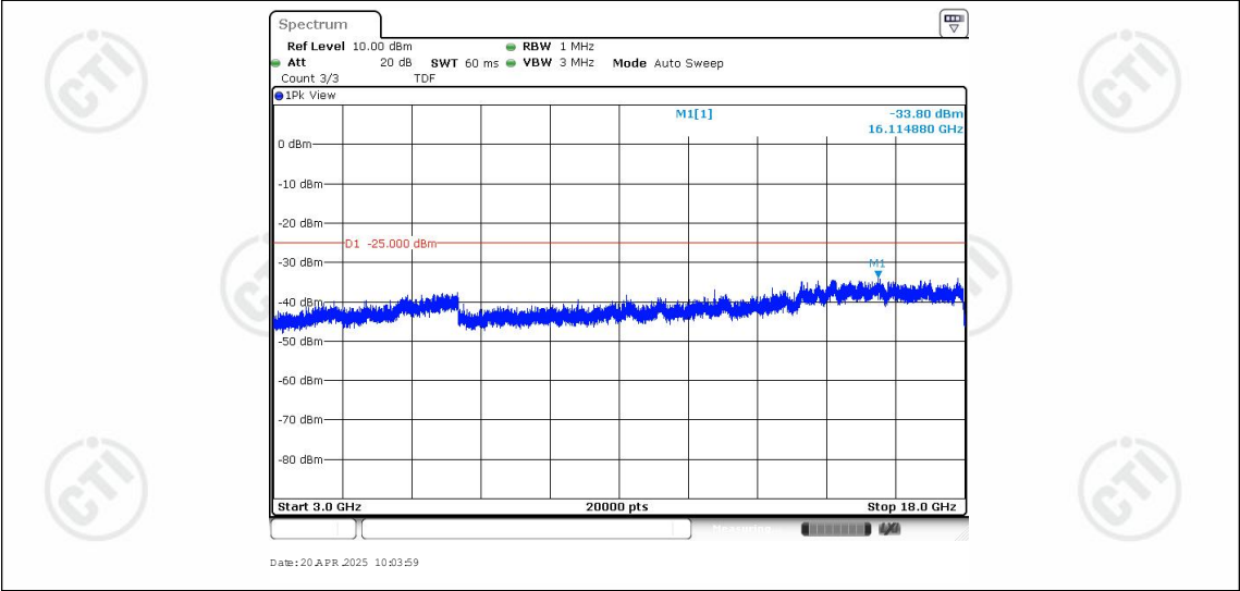
Band41-5MHz-16QAM-39675-1RB#0-Range3:3000~18000MHz
