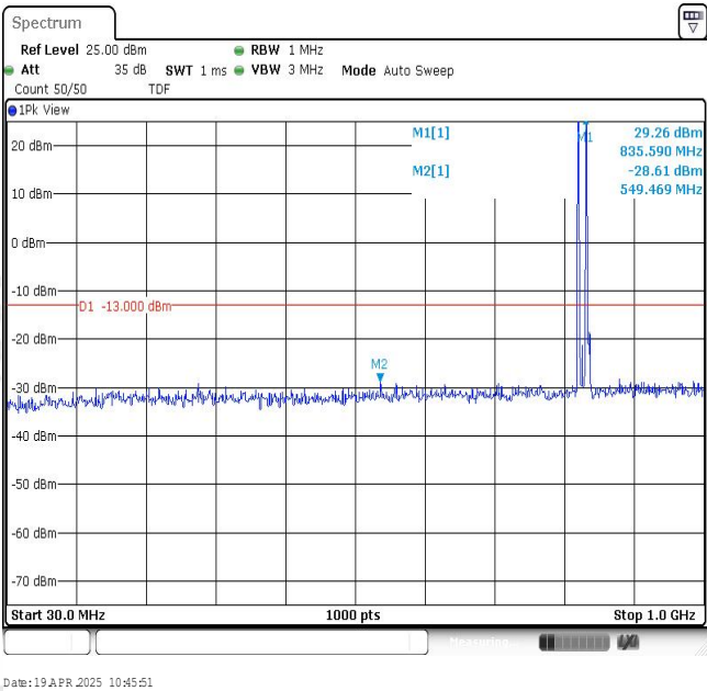
Band5-3MHz-16QAM-20525-1RB#0-Range1:30~1000MHz
