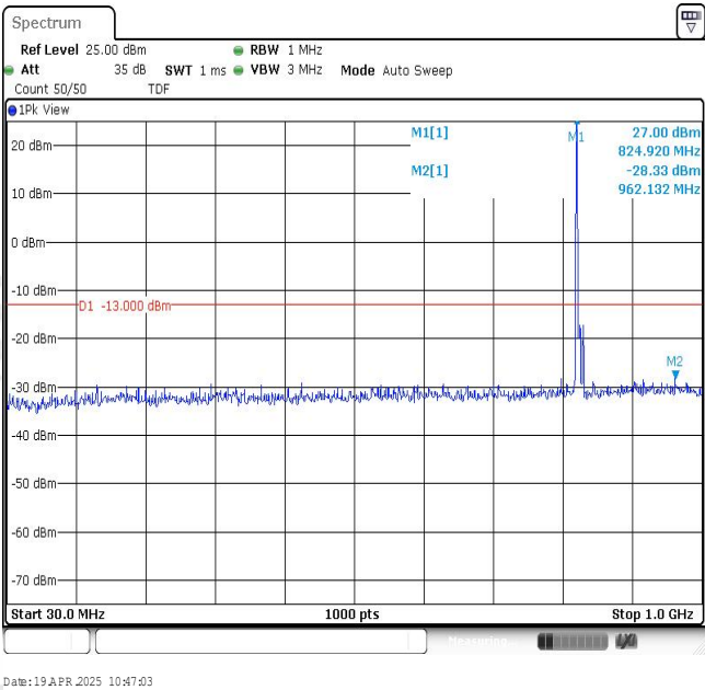
Band5-5MHz-16QAM-20425-1RB#0-Range1:30~1000MHz
