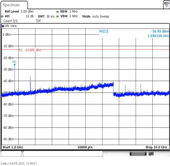
Band5-1.4MHz-QPSK-20643-1RB#0-Range2:1000~10000MHz
