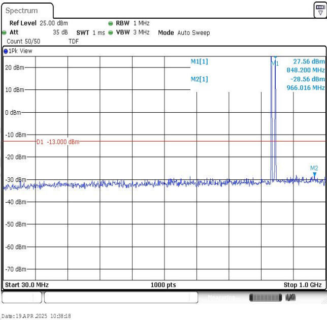
Band5-1.4MHz-QPSK-20643-1RB#0-Range1:30~1000MHz
