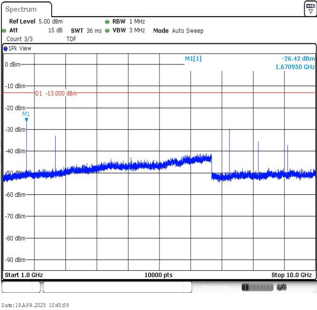
Band5-3MHz-16QAM-20525-1RB#0-Range2:1000~10000MHz
