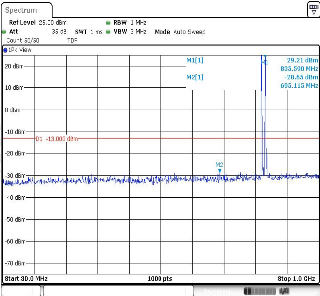
Band5-3MHz-QPSK-20525-1RB#0-Range1:30~1000MHz
