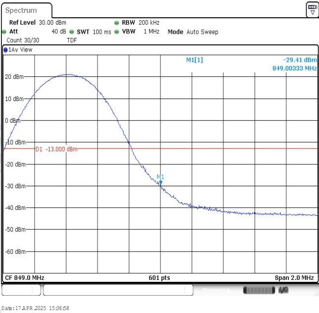
Band5-10MHz-QPSK-20600-1RB#49
