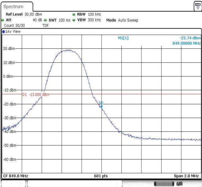
Band5-5MHz-16QAM-20625-1RB#24
