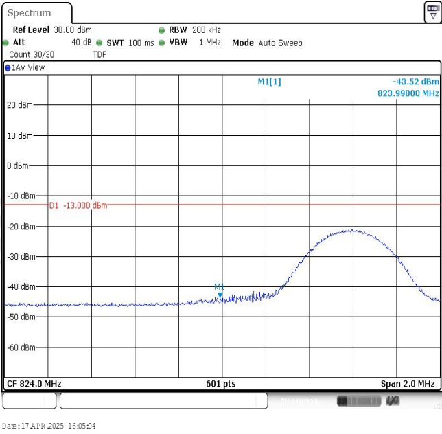
Band5-10MHz-16QAM-20450-1RB#49
