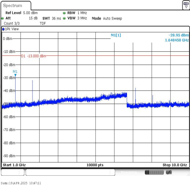
Band5-5MHz-16QAM-20425-1RB#0-Range2:1000~10000MHz
