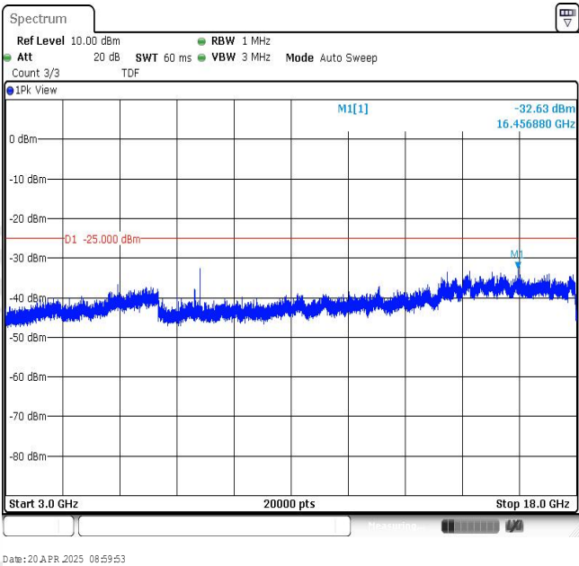
Band7-5MHz-16QAM-20775-1RB#0-Range3:3000~18000MHz
