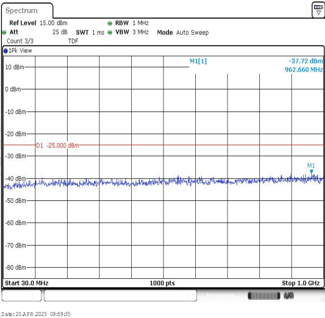
Band7-5MHz-16QAM-20775-1RB#0-Range1:30~1000MHz
