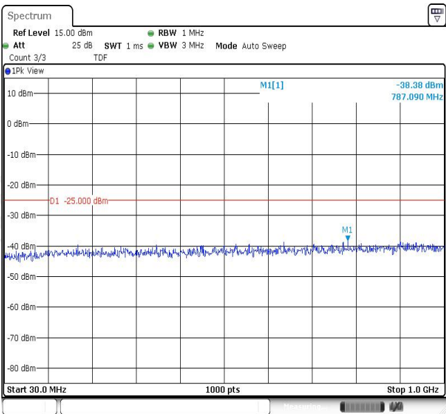
Band7-5MHz-16QAM-21100-1RB#0-Range1:30~1000MHz
