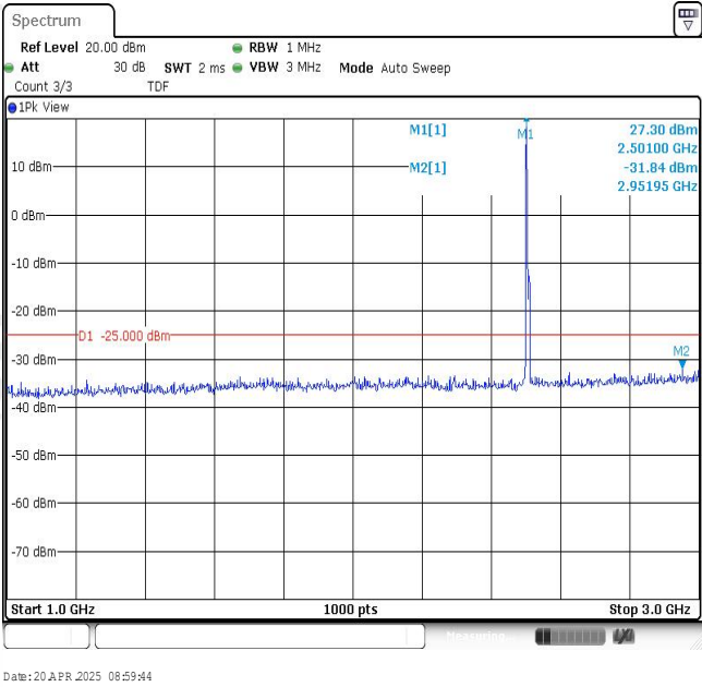
Band7-5MHz-16QAM-20775-1RB#0-Range2:1000~3000MHz
