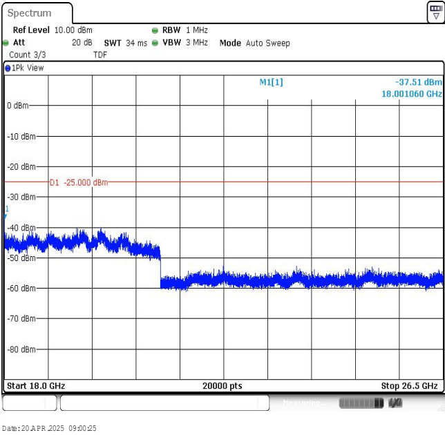
Band7-5MHz-16QAM-20775-1RB#0-Range4:18000~26500MHz
