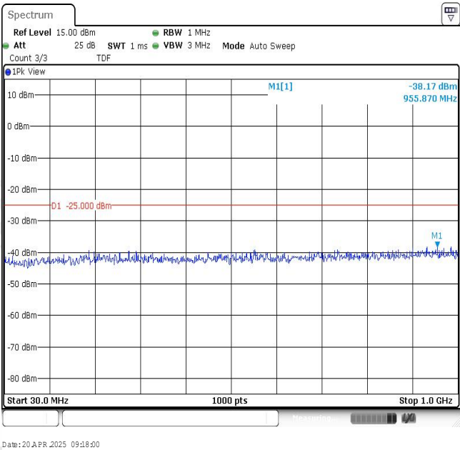
Band7-15MHz-16QAM-21100-1RB#0-Range1:30~1000MHz
