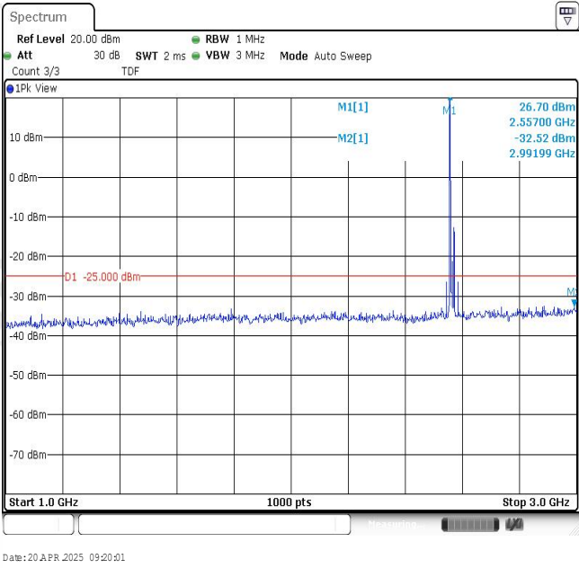
Band7-15MHz-16QAM-21375-1RB#0-Range2:1000~3000MHz
