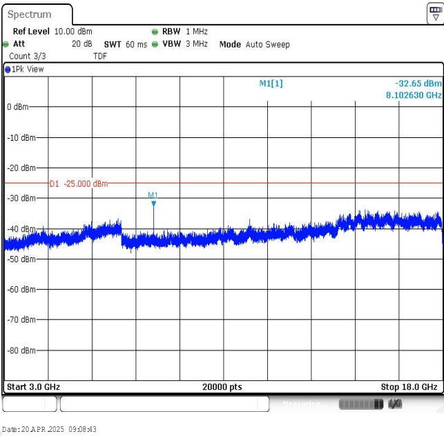
Band7-10MHz-16QAM-20800-1RB#0-Range3:3000~18000MHz
