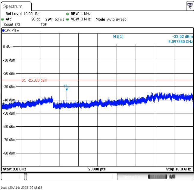
Band7-15MHz-16QAM-21100-1RB#0-Range3:3000~18000MHz
