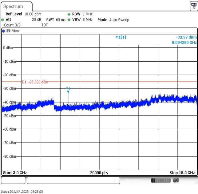
Band7-20MHz-QPSK-21350-1RB#0-Range3:3000~18000MHz
