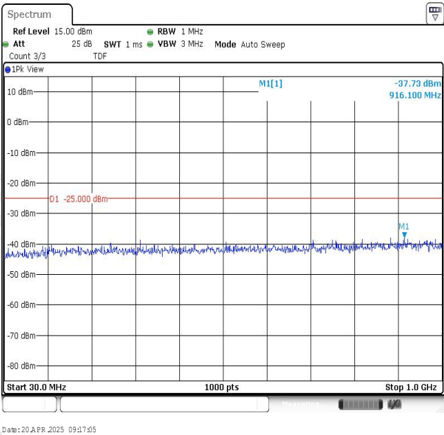
Band7-15MHz-QPSK-21100-1RB#0-Range1:30~1000MHz
