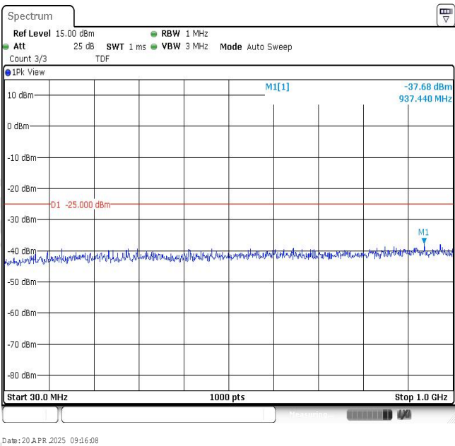
Band7-15MHz-16QAM-20825-1RB#0-Range1:30~1000MHz
