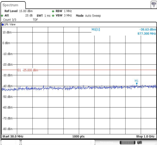
Band7-10MHz-16QAM-21400-1RB#0-Range1:30~1000MHz
