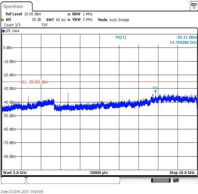
Band7-20MHz-QPSK-21100-1RB#0-Range3:3000~18000MHz
