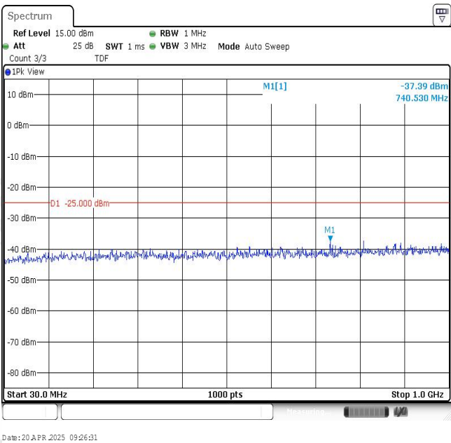
Band7-20MHz-QPSK-21350-1RB#0-Range1:30~1000MHz
