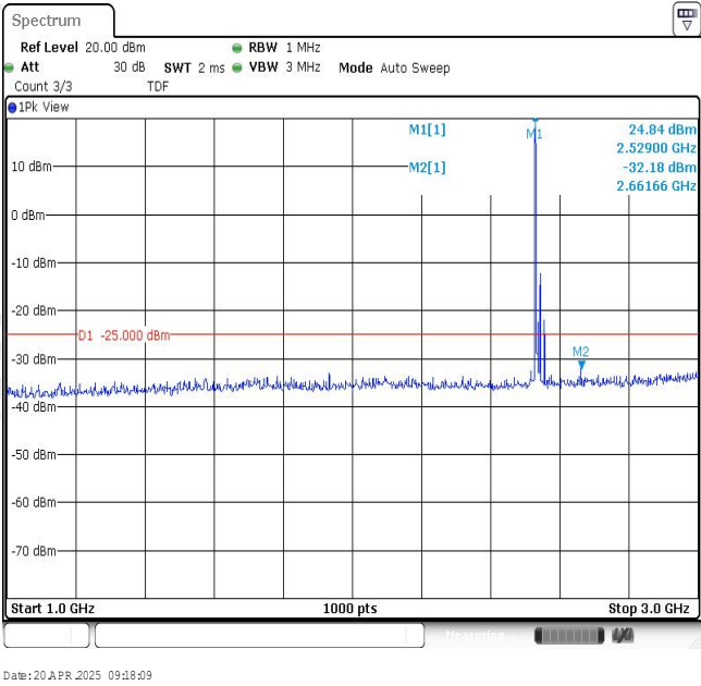
Band7-15MHz-16QAM-21100-1RB#0-Range2:1000~3000MHz
