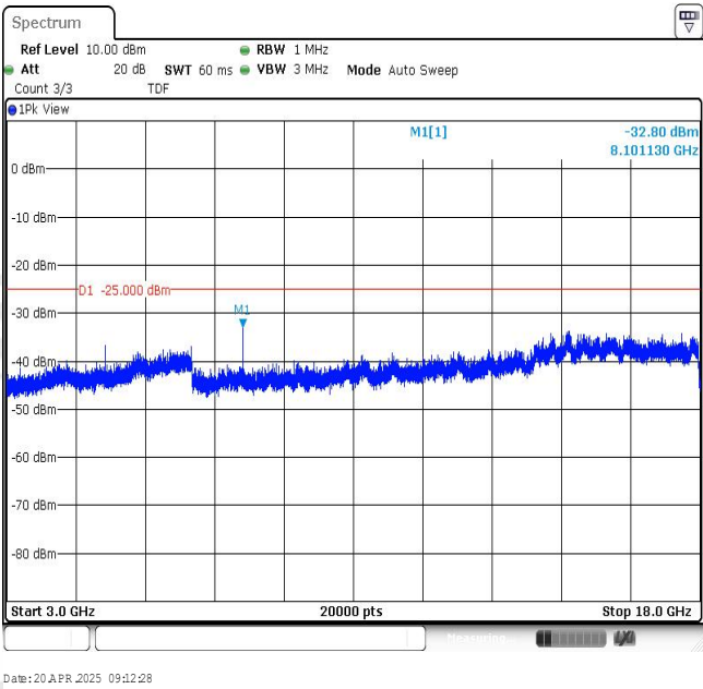
Band7-10MHz-16QAM-21400-1RB#0-Range3:3000~18000MHz
