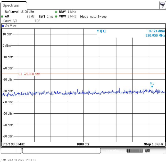
Band7-10MHz-QPSK-21400-1RB#0-Range1:30~1000MHz
