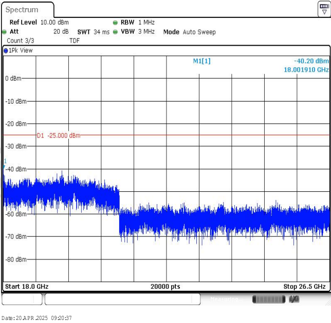
Band7-15MHz-16QAM-21375-1RB#0-Range4:18000~26500MHz
