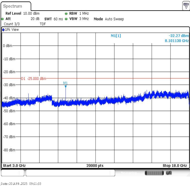
Band7-10MHz-QPSK-21400-1RB#0-Range3:3000~18000MHz
