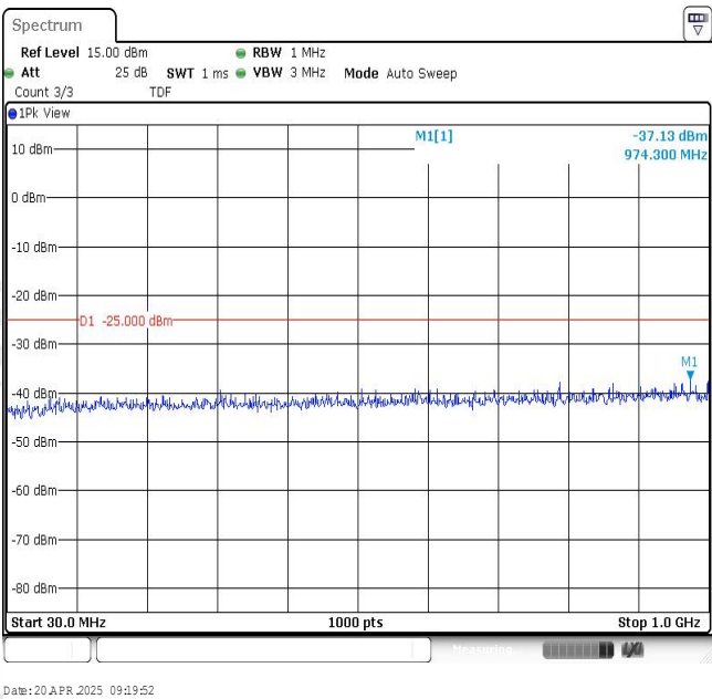
Band7-15MHz-16QAM-21375-1RB#0-Range1:30~1000MHz
