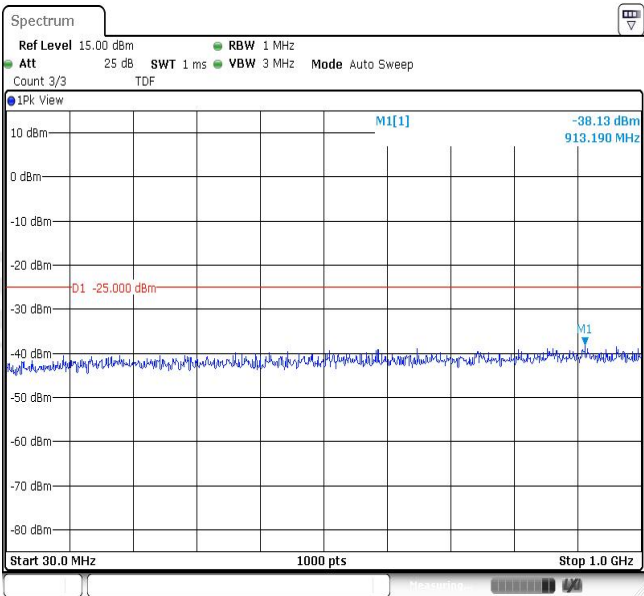
Band7-10MHz-16QAM-21100-1RB#0-Range1:30~1000MHz
