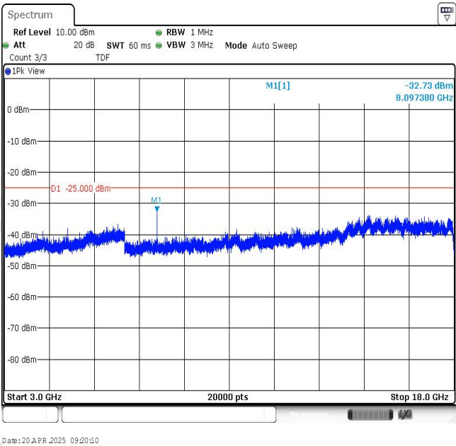
Band7-15MHz-16QAM-21375-1RB#0-Range3:3000~18000MHz
