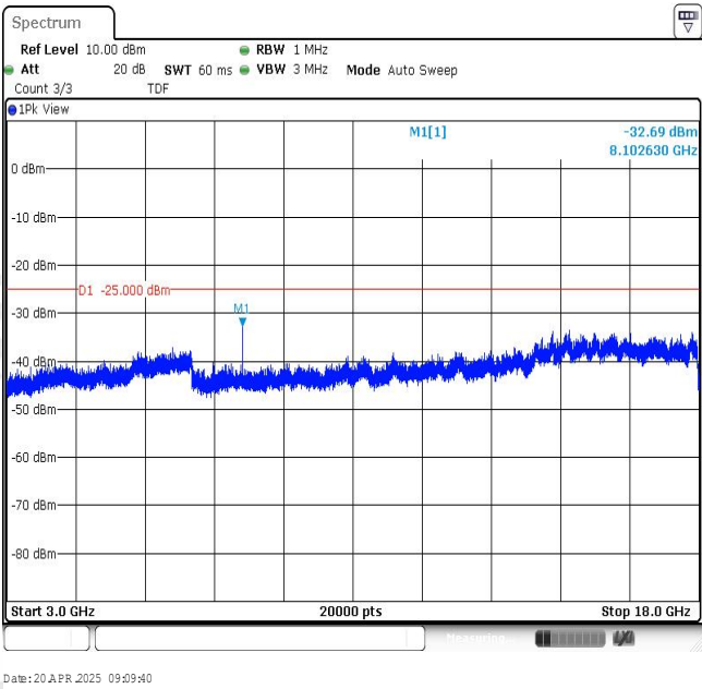
Band7-10MHz-QPSK-21100-1RB#0-Range3:3000~18000MHz
