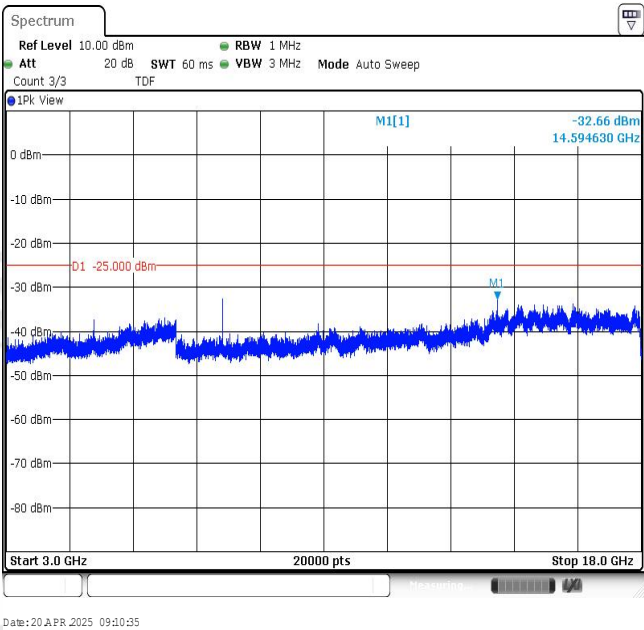
Band7-10MHz-16QAM-21100-1RB#0-Range3:3000~18000MHz
