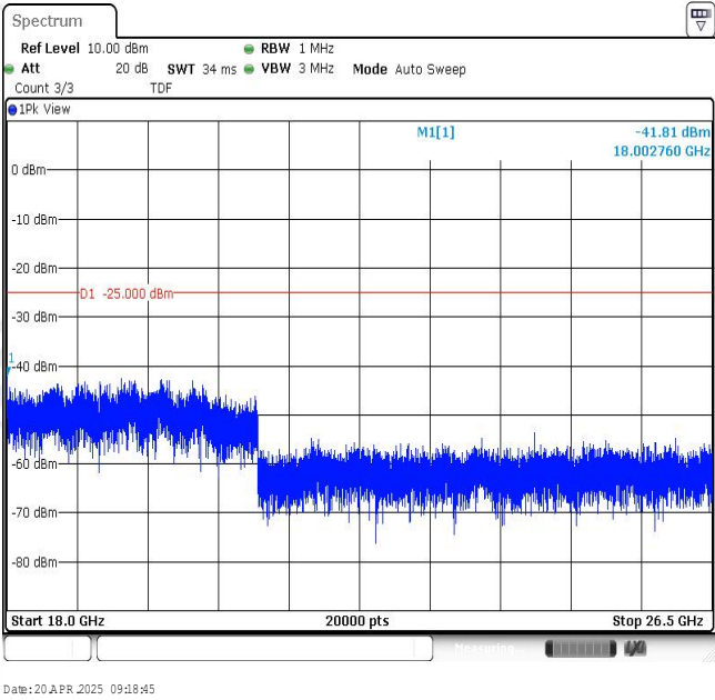
Band7-15MHz-16QAM-21100-1RB#0-Range4:18000~26500MHz
