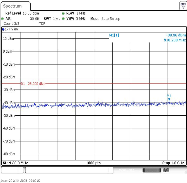
Band7-10MHz-QPSK-21100-1RB#0-Range1:30~1000MHz
