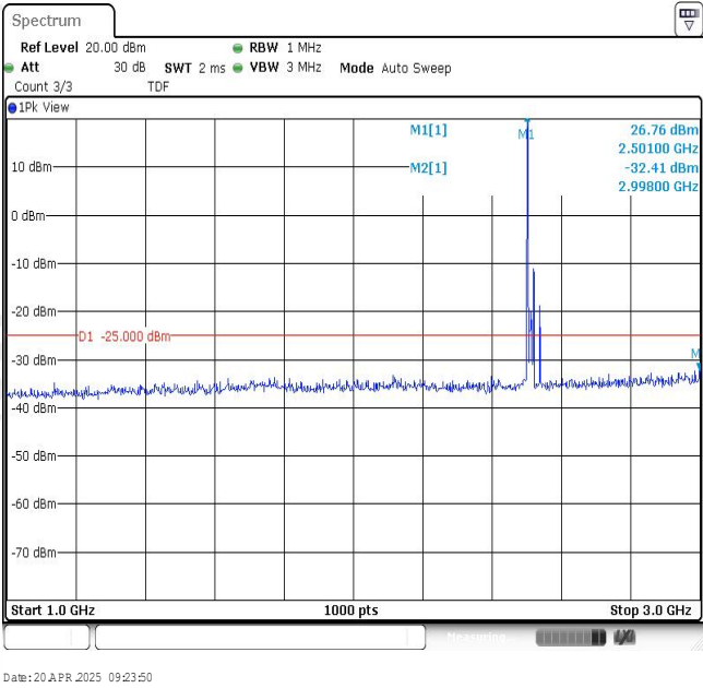
Band7-20MHz-16QAM-20850-1RB#0-Range2:1000~3000MHz
