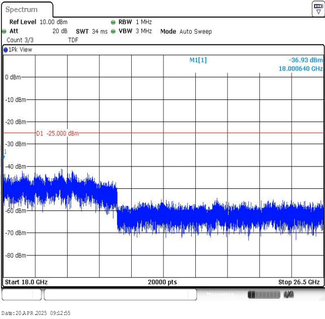
Band7-10MHz-16QAM-21400-1RB#0-Range4:18000~26500MHz
