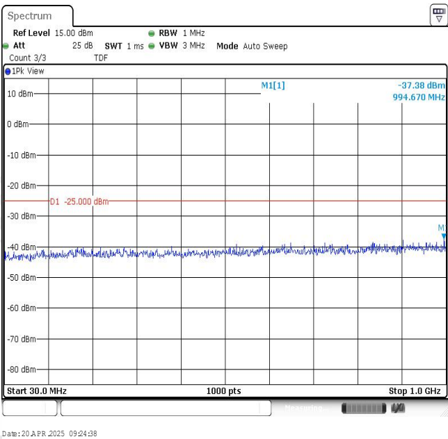
Band7-20MHz-QPSK-21100-1RB#0-Range1:30~1000MHz
