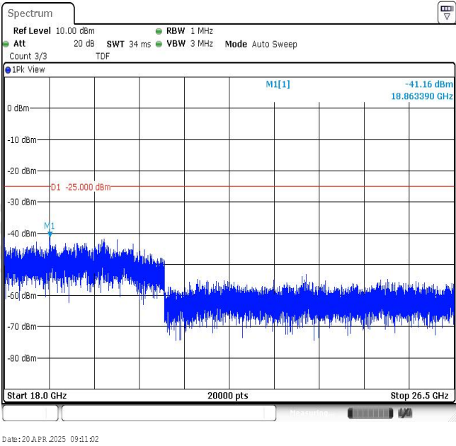
Band7-10MHz-16QAM-21100-1RB#0-Range4:18000~26500MHz
