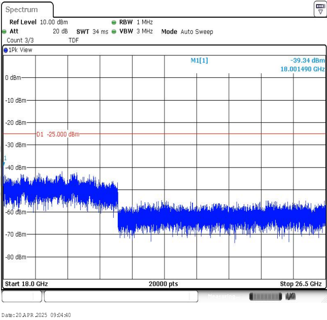
Band7-5MHz-16QAM-21425-1RB#0-Range4:18000~26500MHz
