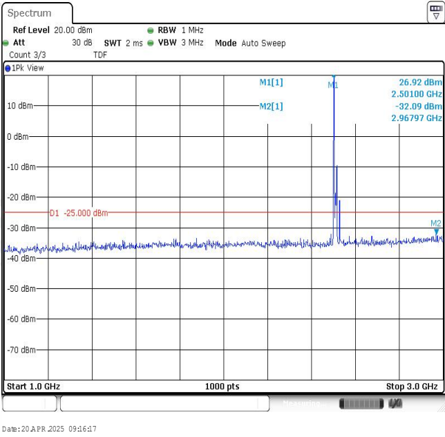
Band7-15MHz-16QAM-20825-1RB#0-Range2:1000~3000MHz
