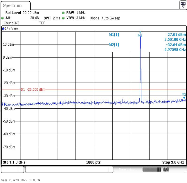
Band7-10MHz-16QAM-20800-1RB#0-Range2:1000~3000MHz
