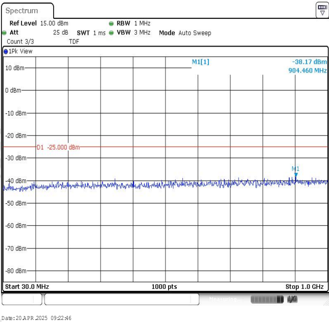
Band7-20MHz-QPSK-20850-1RB#0-Range1:30~1000MHz
