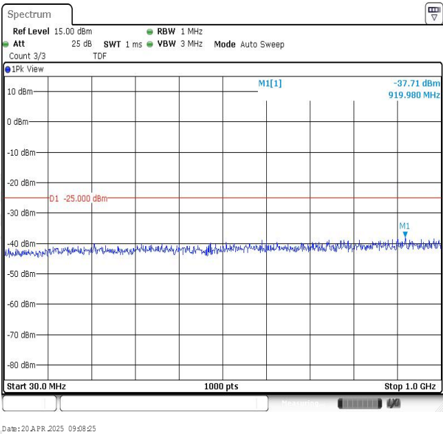
Band7-10MHz-16QAM-20800-1RB#0-Range1:30~1000MHz
