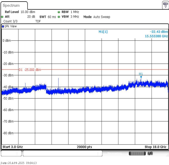
Band7-5MHz-16QAM-21425-1RB#0-Range3:3000~18000MHz
