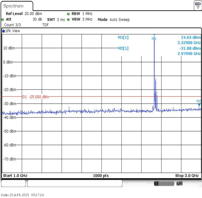
Band7-15MHz-QPSK-21100-1RB#0-Range2:1000~3000MHz
