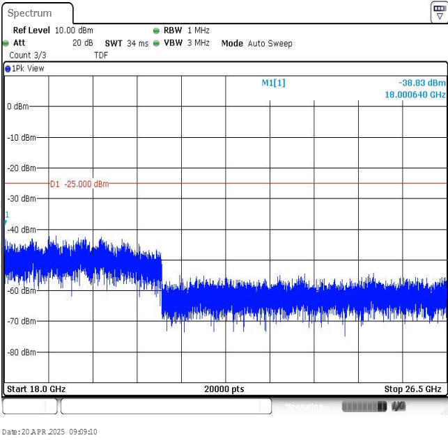
Band7-10MHz-16QAM-20800-1RB#0-Range4:18000~26500MHz
