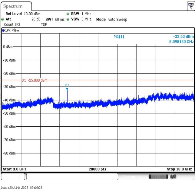
Band7-15MHz-16QAM-20825-1RB#0-Range3:3000~18000MHz
