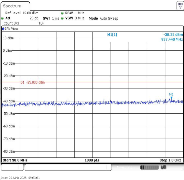
Band7-20MHz-16QAM-20850-1RB#0-Range1:30~1000MHz
