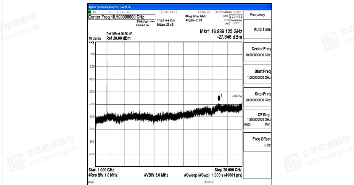
Band7_20MHz_16QAM_20850_1RB#0_1000~20000_1000~20000
