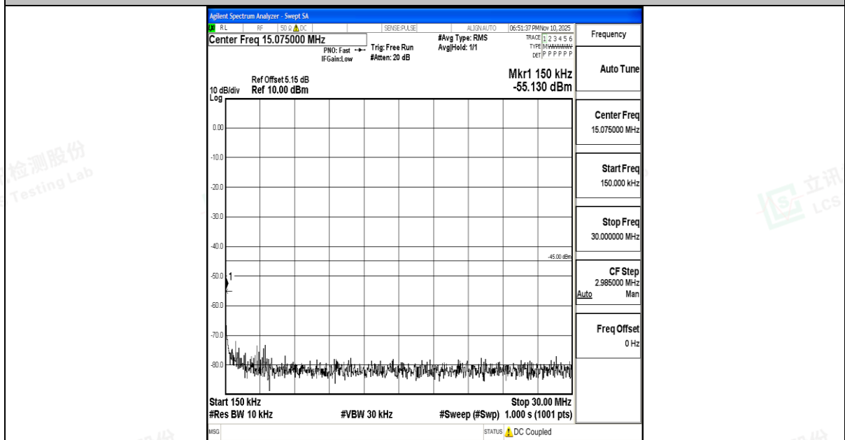
Band7_5MHz_16QAM_21425_1RB#0_0.15~30_0.15~30
