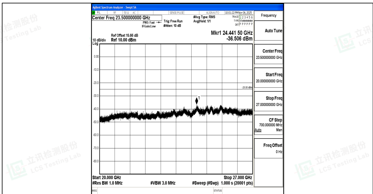
Band7_10MHz_QPSK_21400_1RB#0_20000~27000_20000~27000
