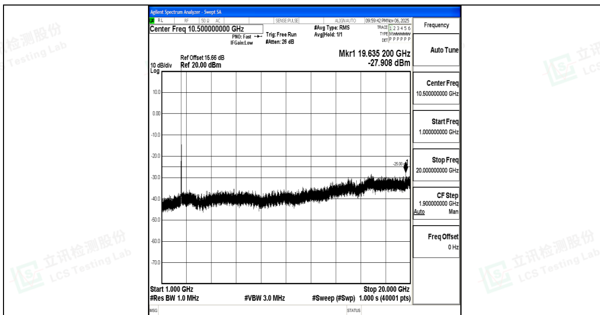
Band7_10MHz_16QAM_20800_1RB#0_1000~20000_1000~20000
