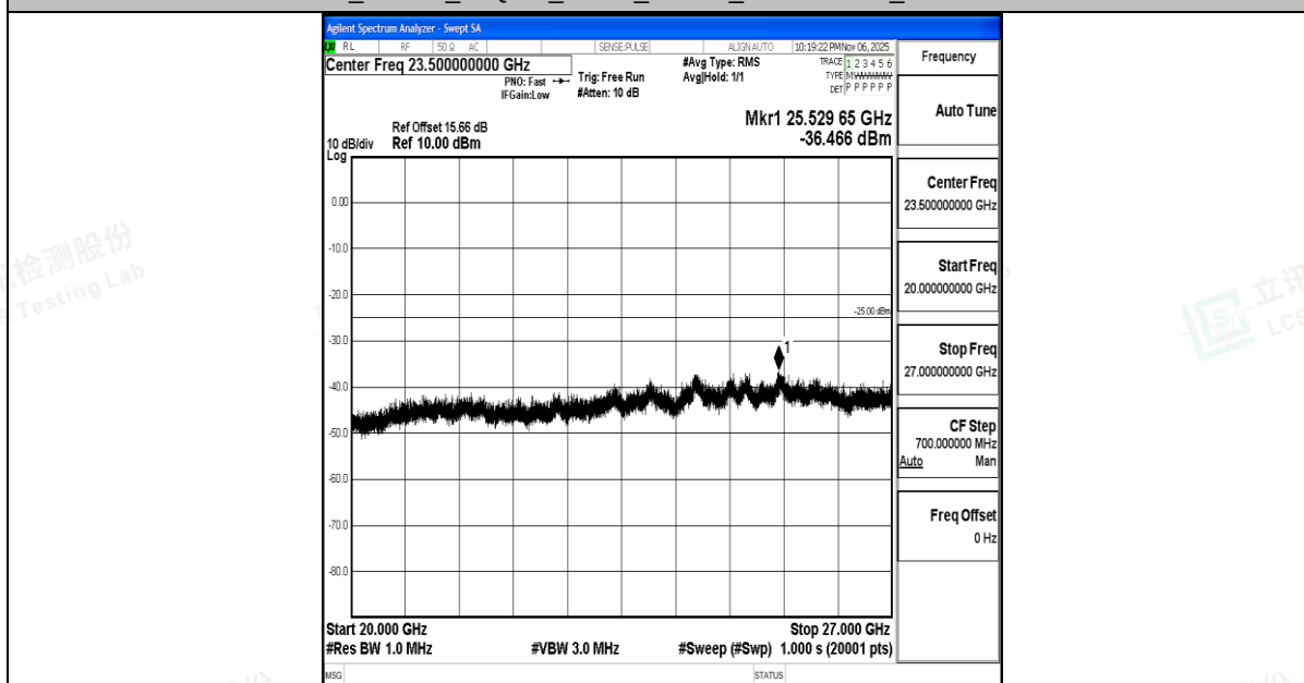
Band7_15MHz_16QAM_21100_1RB#0_20000~27000_20000~27000
