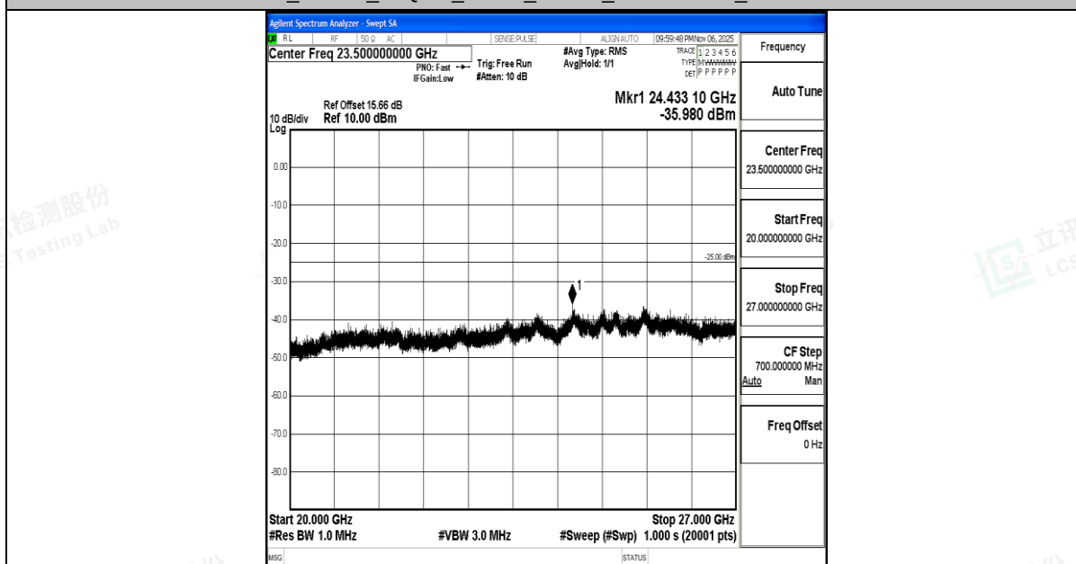
Band7_10MHz_16QAM_20800_1RB#0_20000~27000_20000~27000
