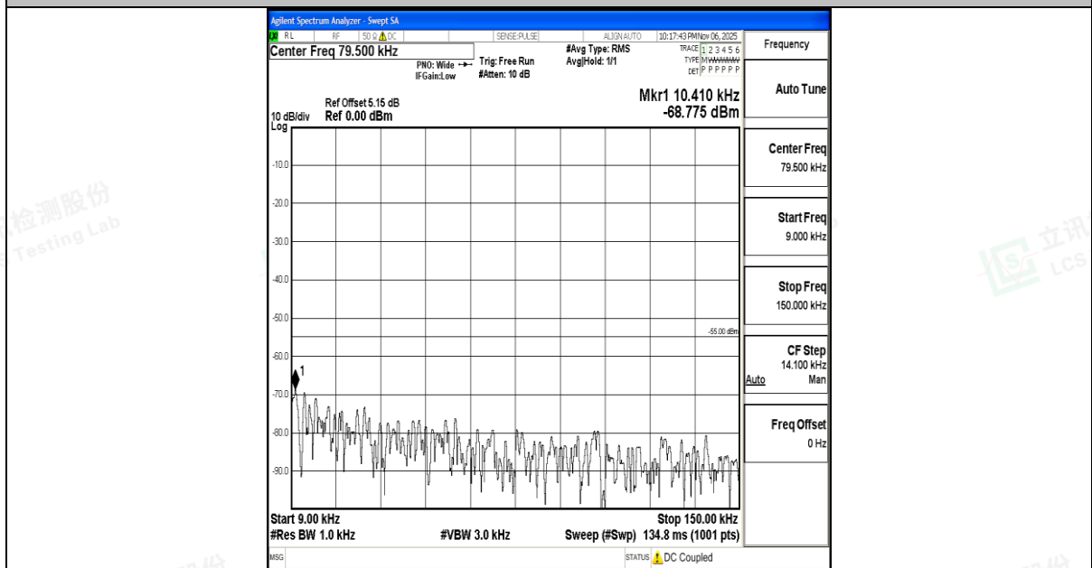
Band7_15MHz_16QAM_20825_1RB#0_0.009~0.15_0.009~0.15
