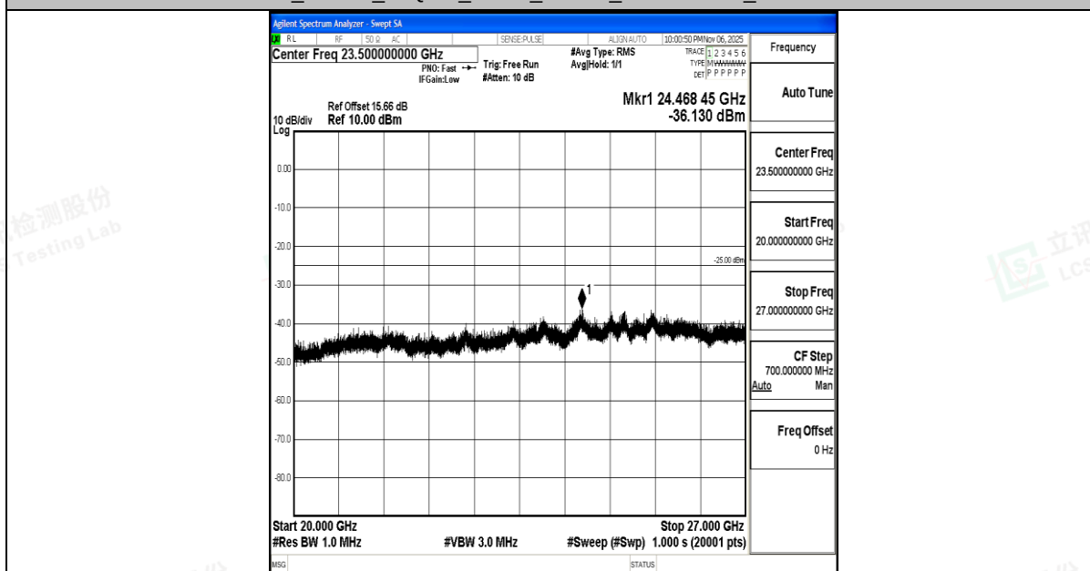
Band7_10MHz_16QAM_21100_1RB#0_20000~27000_20000~27000
