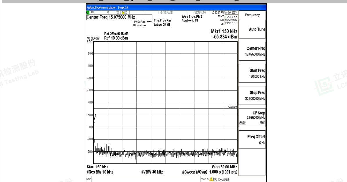
Band7_20MHz_QPSK_21100_1RB#0_0.15~30_0.15~30
