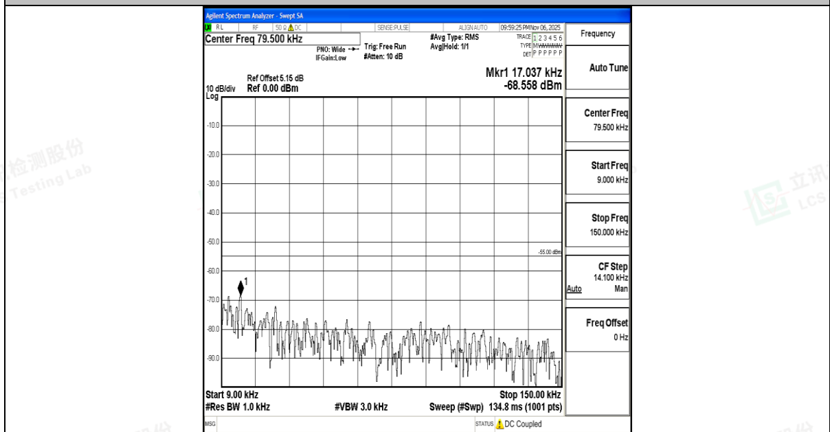
Band7_10MHz_16QAM_20800_1RB#0_0.009~0.15_0.009~0.15
