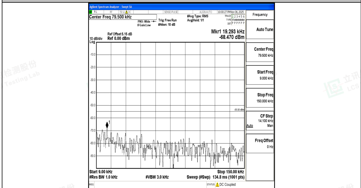
Band7_10MHz_16QAM_21100_1RB#0_0.009~0.15_0.009~0.15
