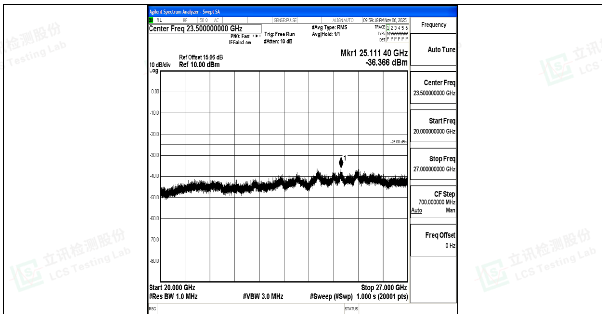
Band7_10MHz_QPSK_20800_1RB#0_20000~27000_20000~27000
