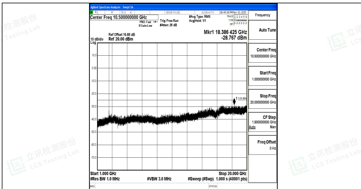
Band7_5MHz_16QAM_20775_1RB#0_1000~20000_1000~20000
