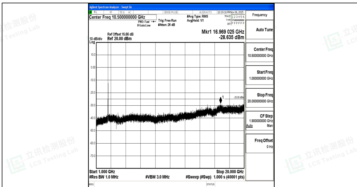
Band7_15MHz_16QAM_21100_1RB#0_1000~20000_1000~20000
