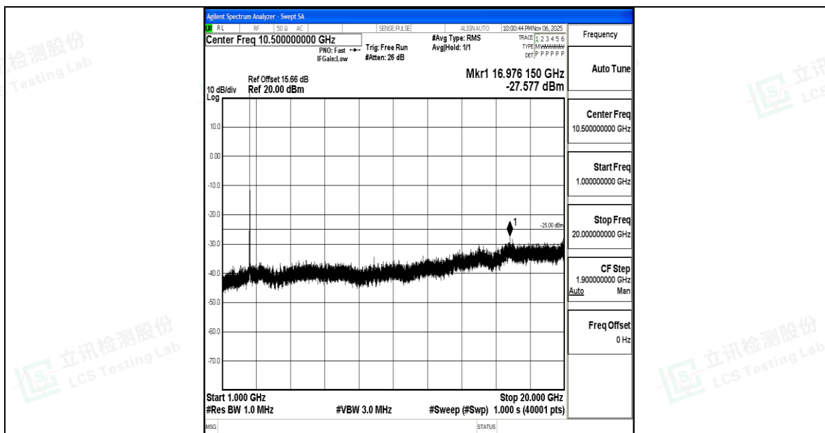
Band7_10MHz_16QAM_21100_1RB#0_1000~20000_1000~20000
