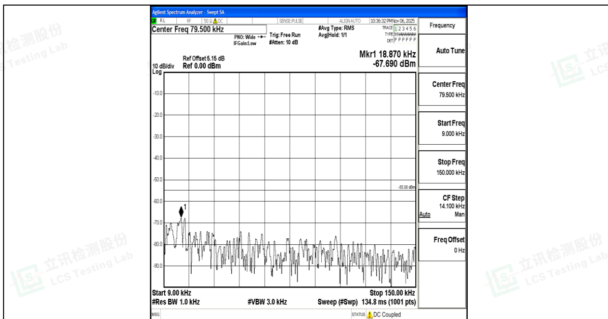
Band7_20MHz_QPSK_21100_1RB#0_0.009~0.15_0.009~0.15
