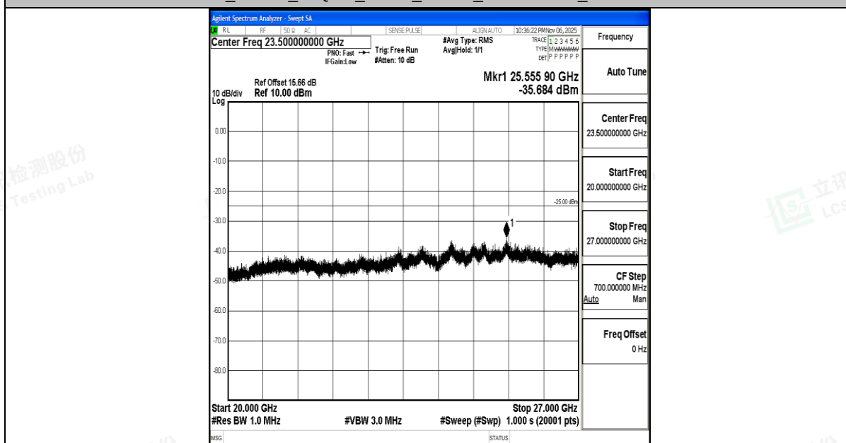
Band7_20MHz_16QAM_20850_1RB#0_20000~27000_20000~27000
