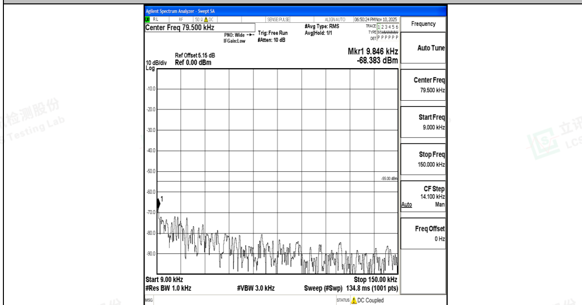
Band7_5MHz_16QAM_21100_1RB#0_0.009~0.15_0.009~0.15
