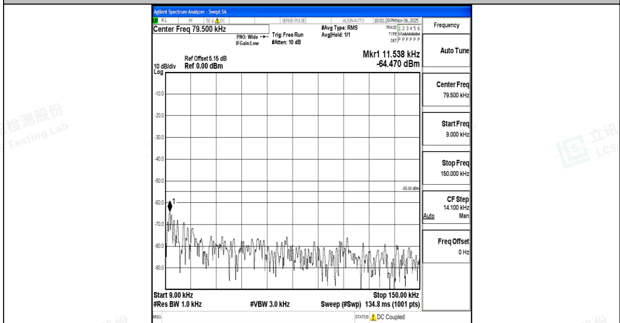
Band7_10MHz_16QAM_21400_1RB#0_0.009~0.15_0.009~0.15
