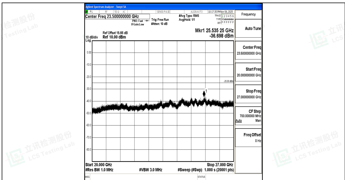
Band7_15MHz_QPSK_20825_1RB#0_20000~27000_20000~27000
