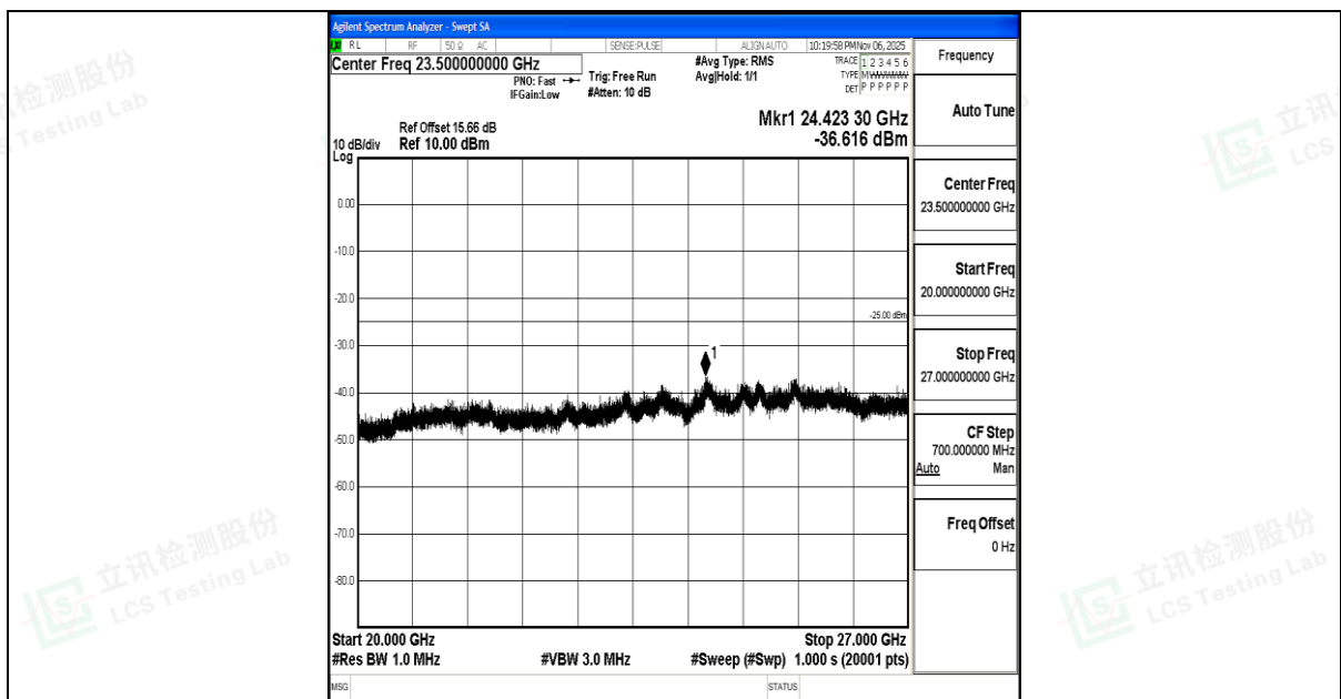
Band7_15MHz_QPSK_21375_1RB#0_20000~27000_20000~27000
