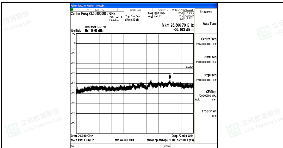
Band7_5MHz_QPSK_21100_1RB#0_20000~27000_20000~27000
