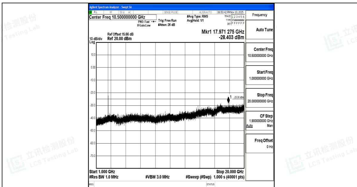
Band7_5MHz_16QAM_21100_1RB#0_1000~20000_1000~20000
