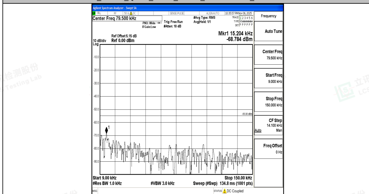
Band7_20MHz_16QAM_20850_1RB#0_0.009~0.15_0.009~0.15
