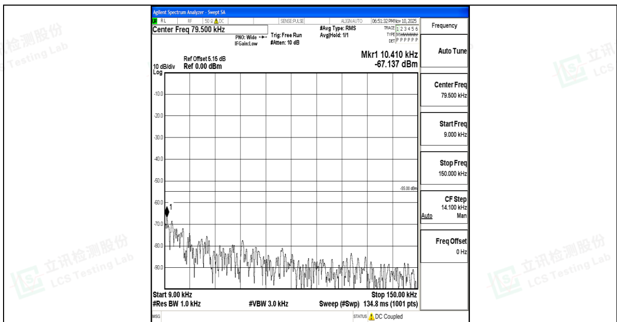
Band7_5MHz_16QAM_21425_1RB#0_0.009~0.15_0.009~0.15
