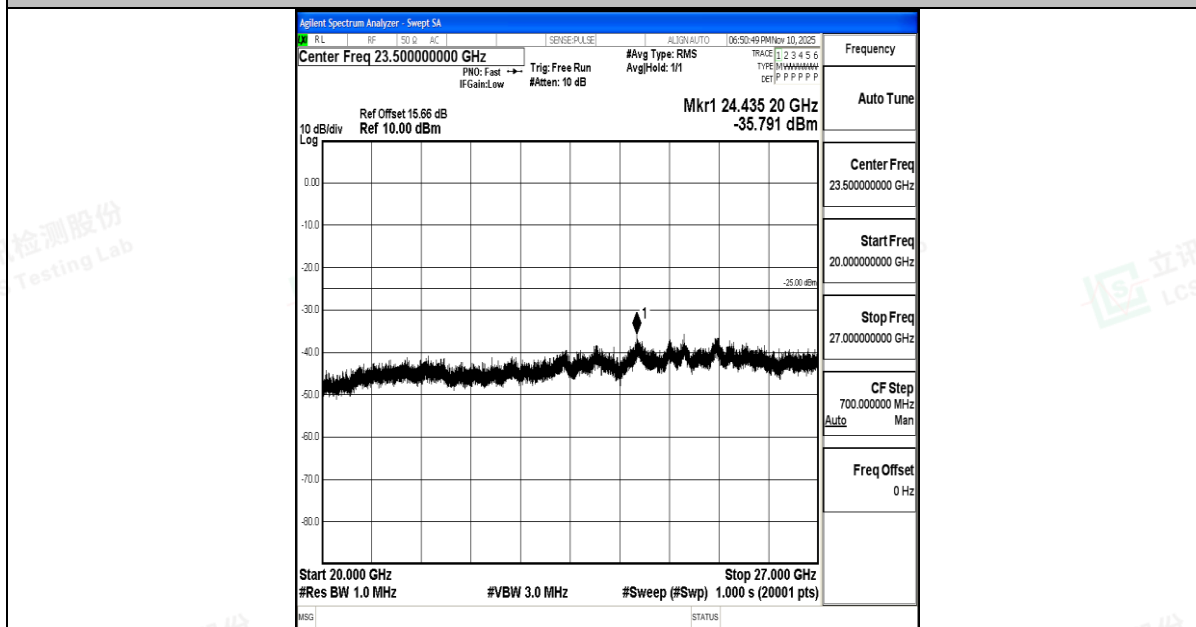
Band7_5MHz_16QAM_21100_1RB#0_20000~27000_20000~27000
