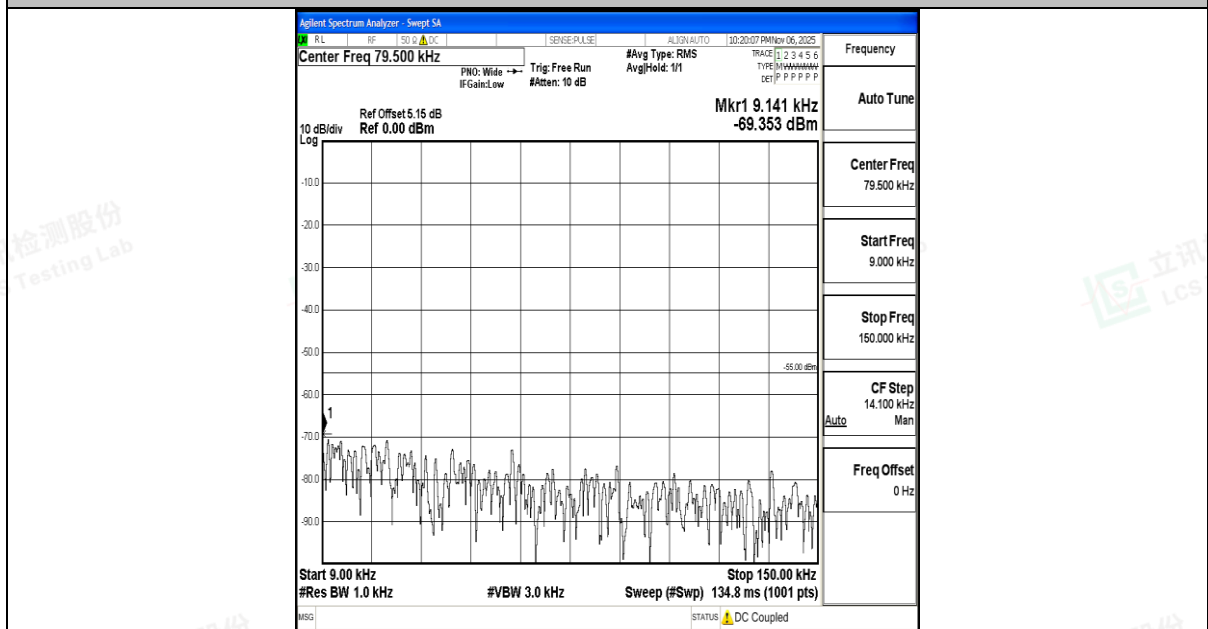
Band7_15MHz_16QAM_21375_1RB#0_0.009~0.15_0.009~0.15
