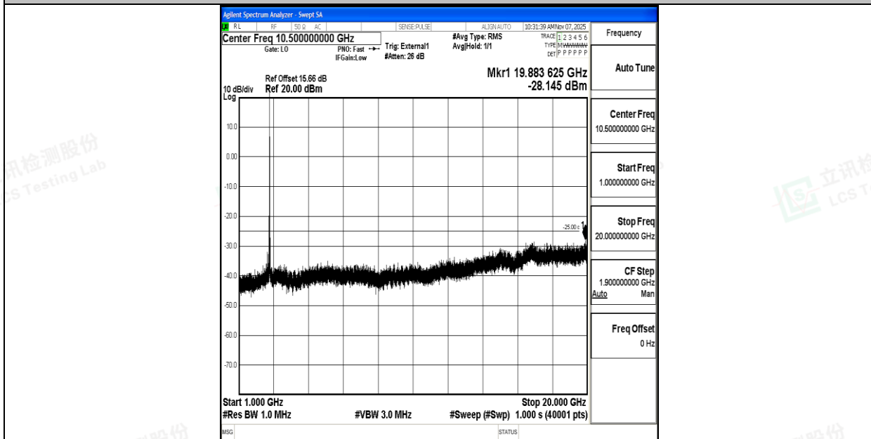
Band41_20MHz_QPSK_41490_1RB#0_1000~20000_1000~20000
