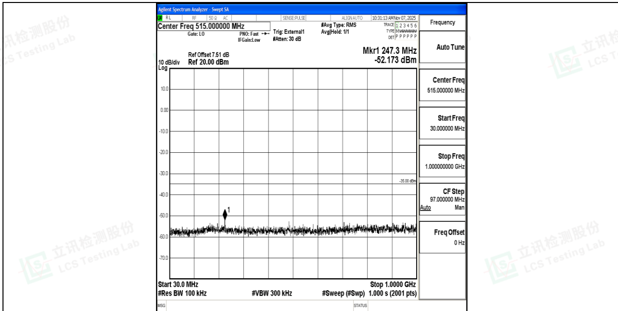
Band41_20MHz_QPSK_41490_1RB#0_30~1000_30~1000
