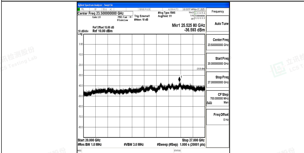
Band41_20MHz_16QAM_41490_1RB#0_20000~27000_20000~27000
