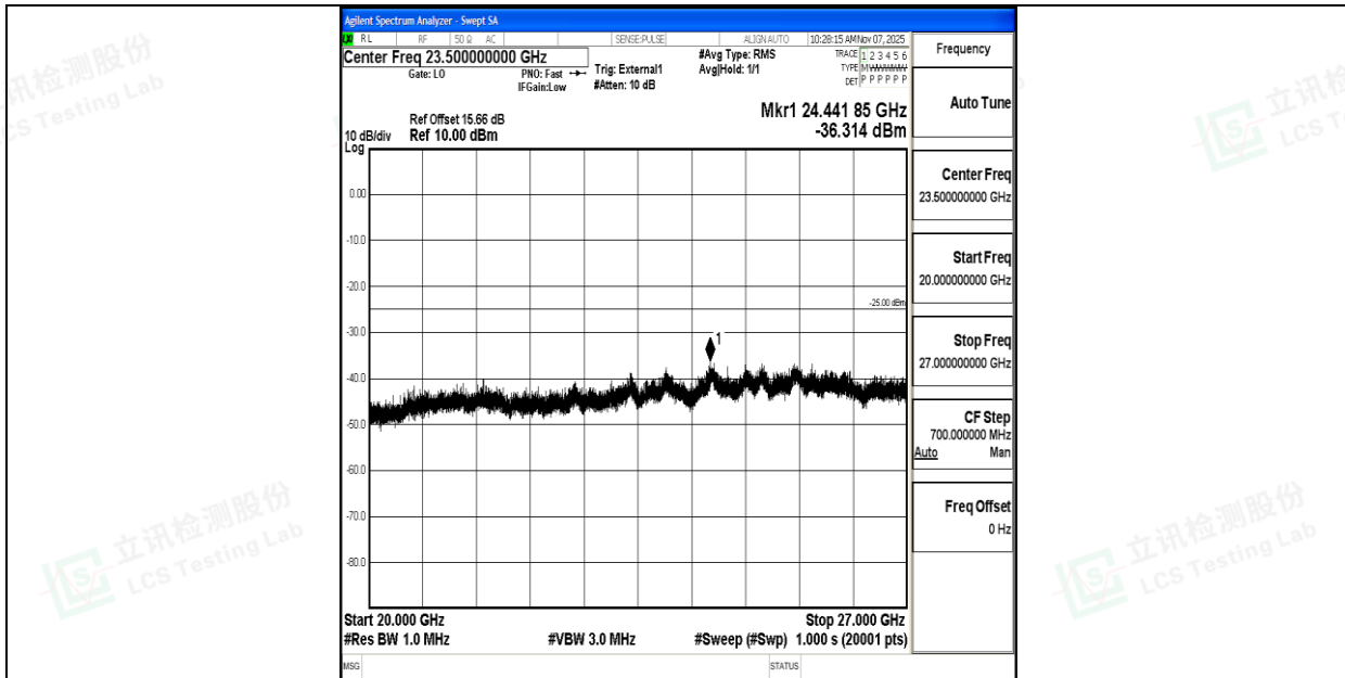
Band41_20MHz_QPSK_40620_1RB#0_20000~27000_20000~27000
