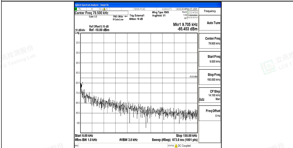
Band41_20MHz_16QAM_41490_1RB#0_0.009~0.15_0.009~0.15
