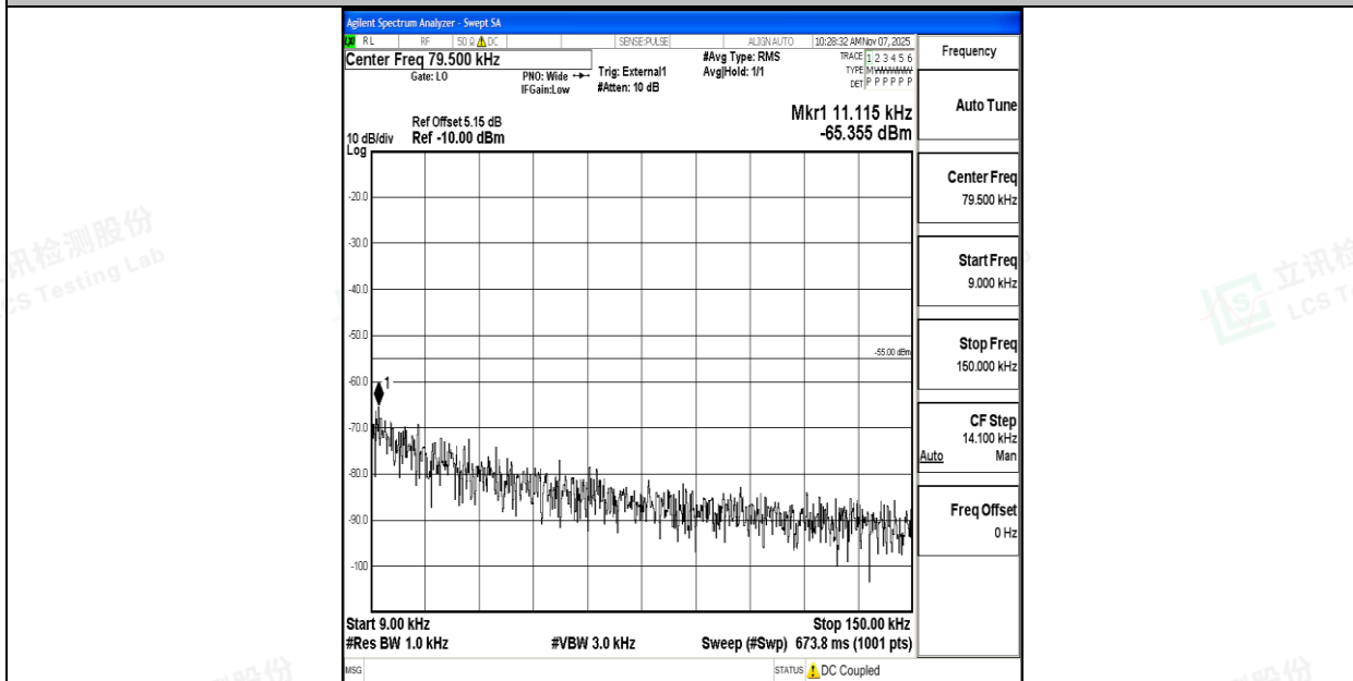
Band41_20MHz_16QAM_40620_1RB#0_0.009~0.15_0.009~0.15
