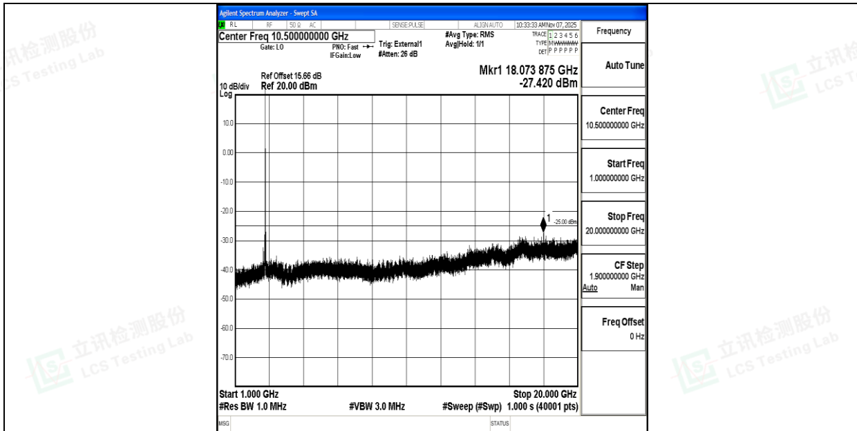
Band41_20MHz_16QAM_41490_1RB#0_1000~20000_1000~20000
