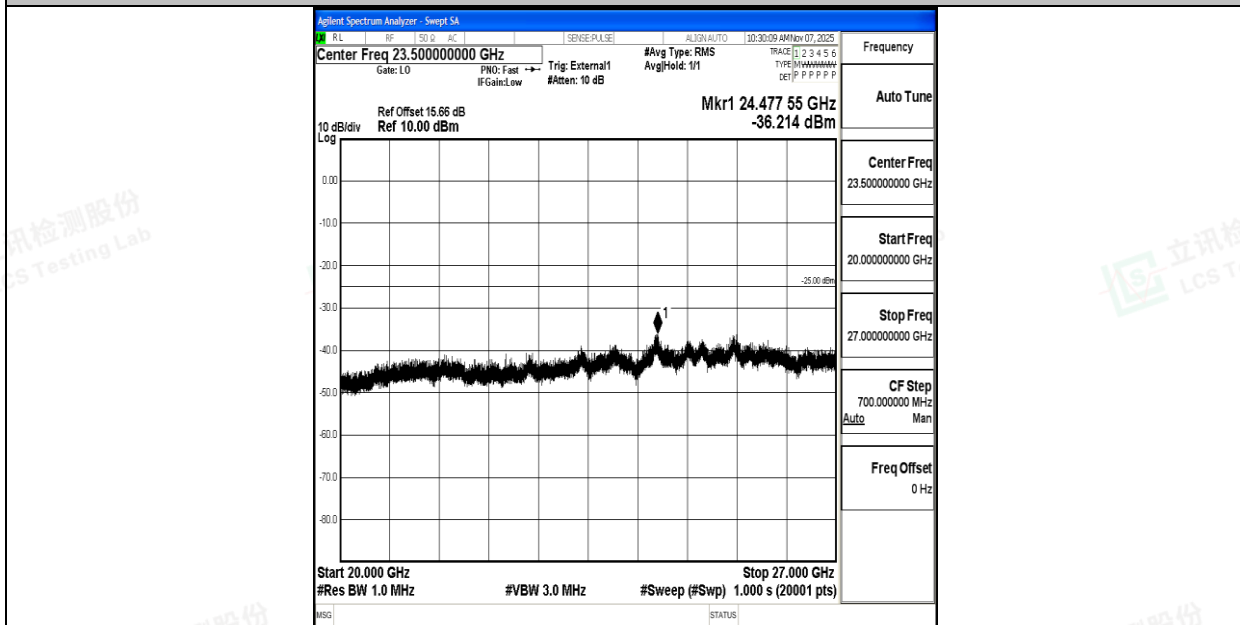
Band41_20MHz_16QAM_40620_1RB#0_20000~27000_20000~27000
