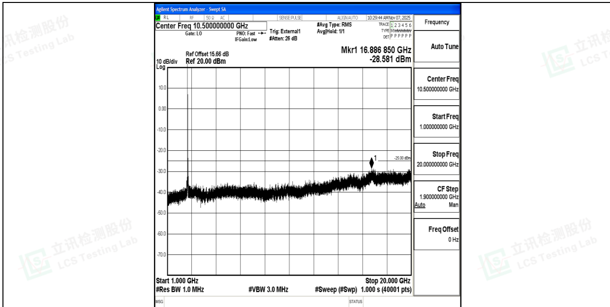
Band41_20MHz_16QAM_40620_1RB#0_1000~20000_1000~20000
