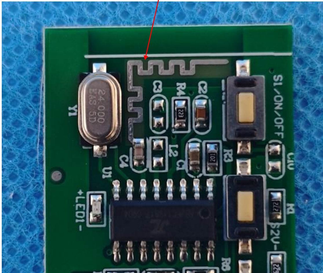
View of wireless antenna
