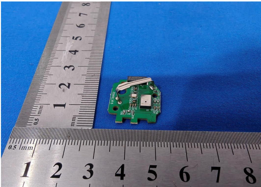
Photo 4: Internal View for PCB
