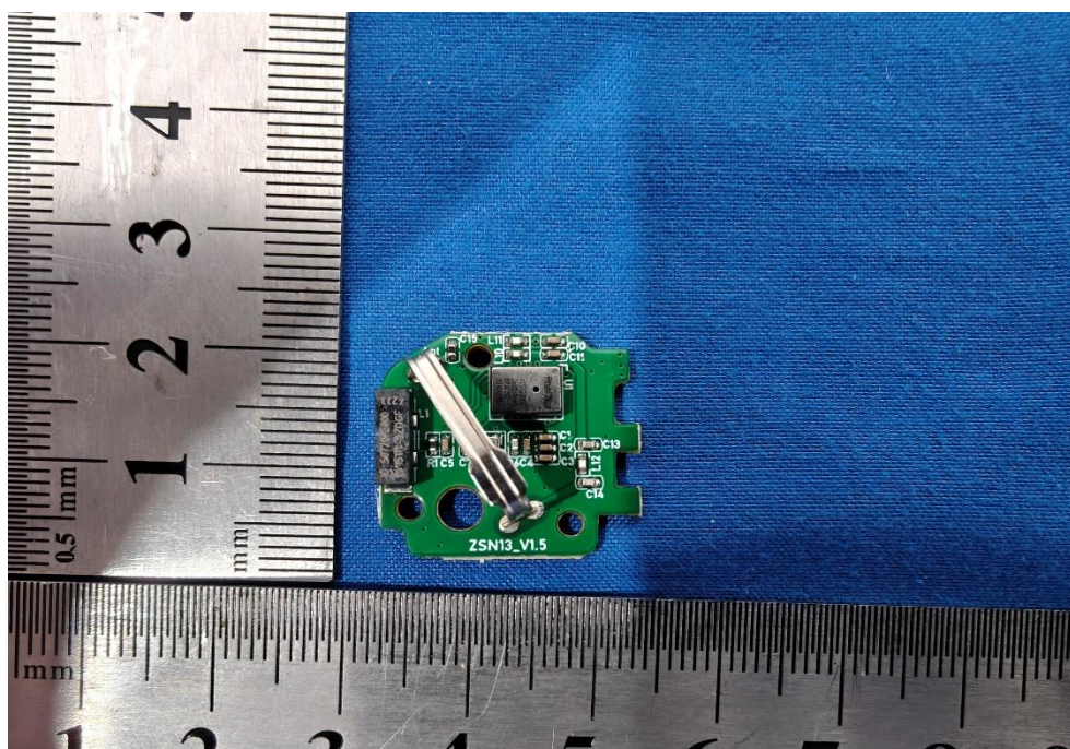
Photo 2: Internal View for PCB
