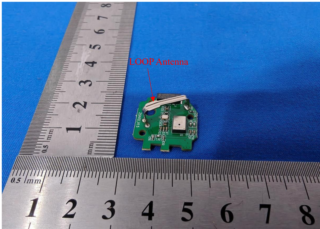
Photo 5: Antenna
