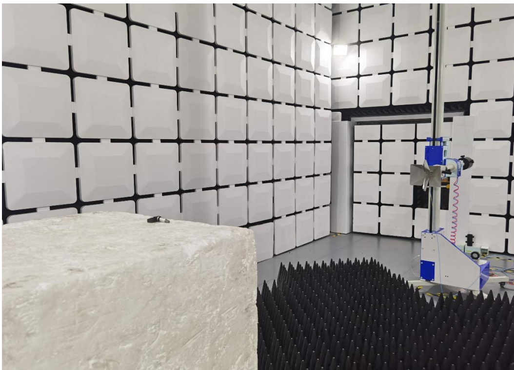
Description: RF Radiated Emission Test Setup for 1GHz ~ 18GHz
