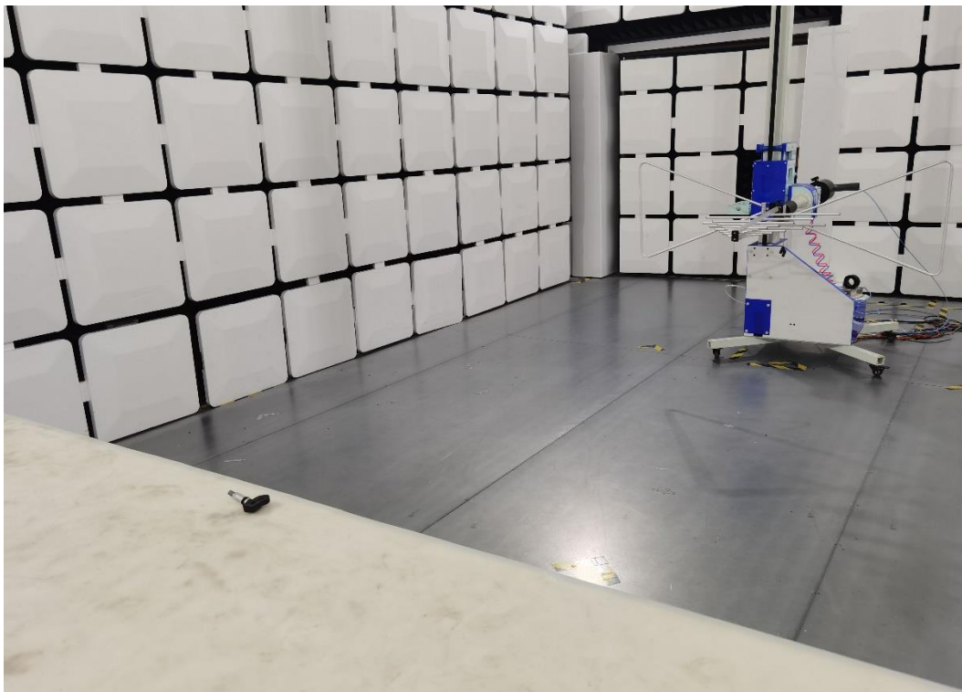
Description: RF Radiated Emission Test Setup for 30MHz ~ 1GHz
