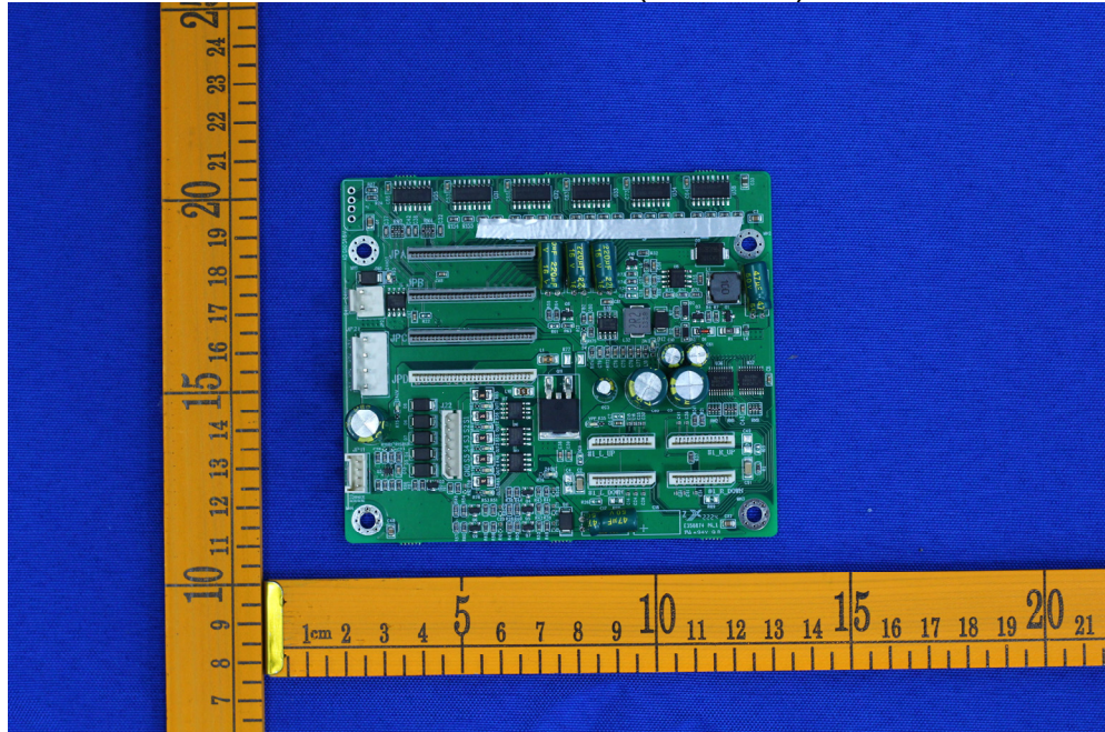
Printer mainboard 3 (back side)
