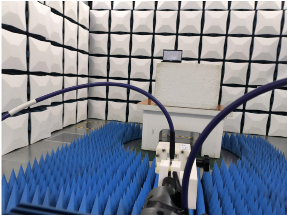
Test Set-up: Radiated spurious emission 18GHz to 26GHz
