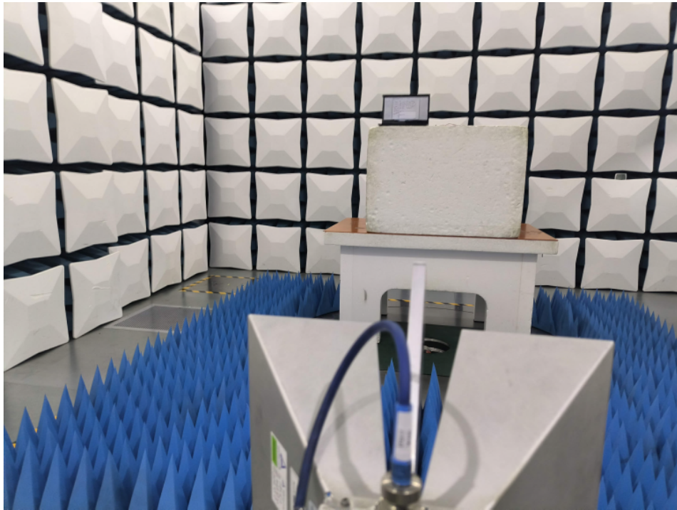
Test Set-up: Radiated spurious emission 1GHz to 18GHz
