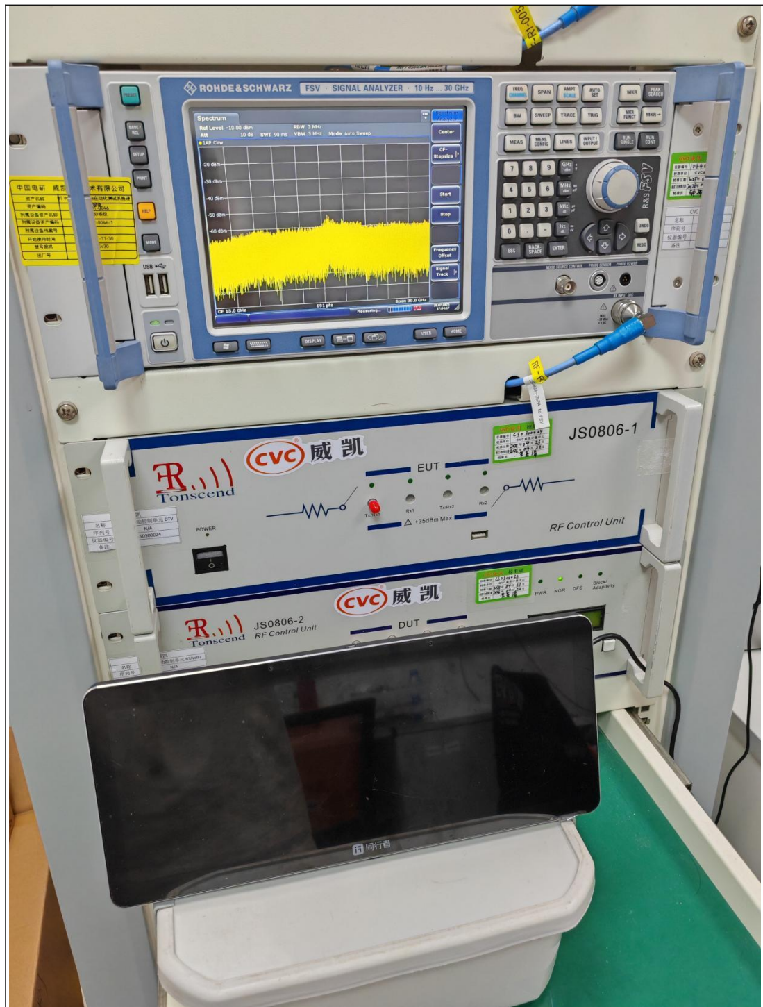
ANTENNA PORT CONDUCTED TEST (WiFi 5G)
