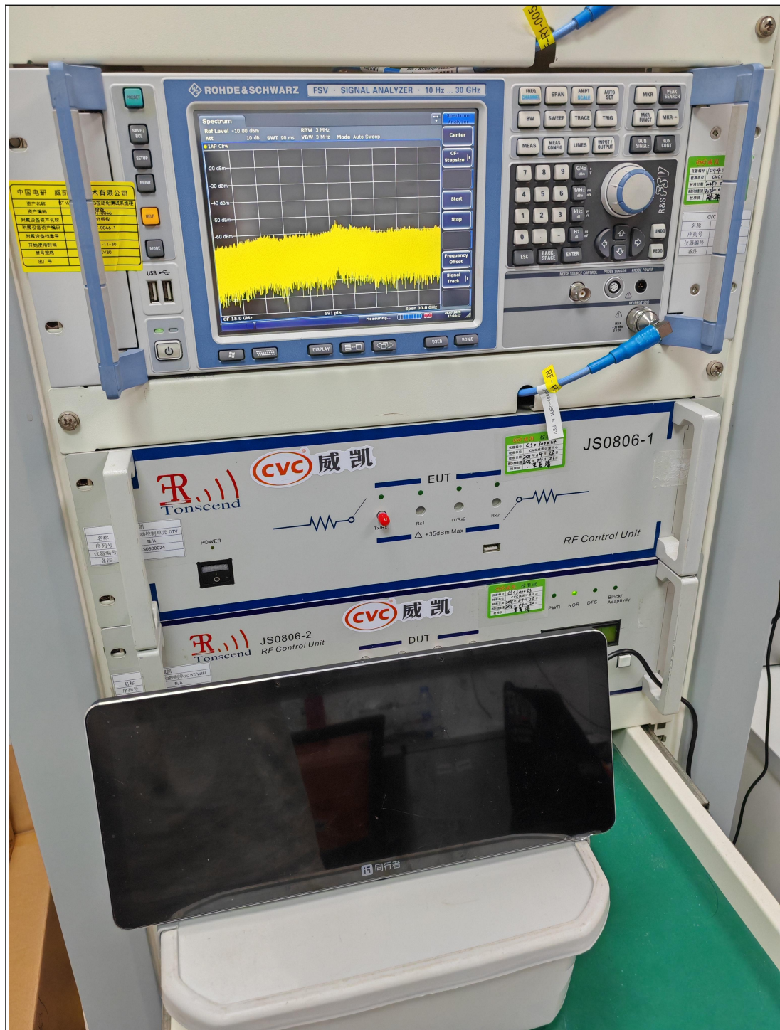
ANTENNA PORT CONDUCTED TEST (BT/BLE)
