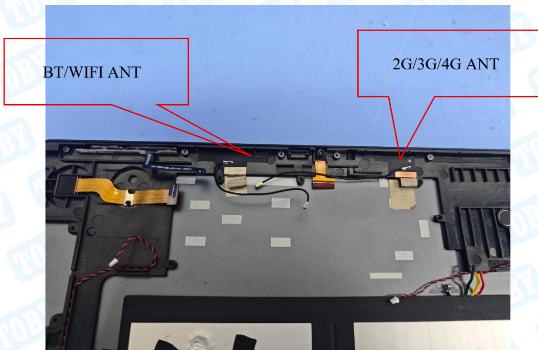
Photo 10 Internal of EUT
