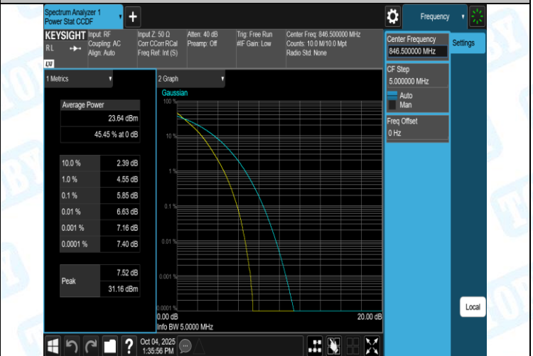
Band26(824-849)-5MHz-16QAM-26815-25RB#0-PASS
