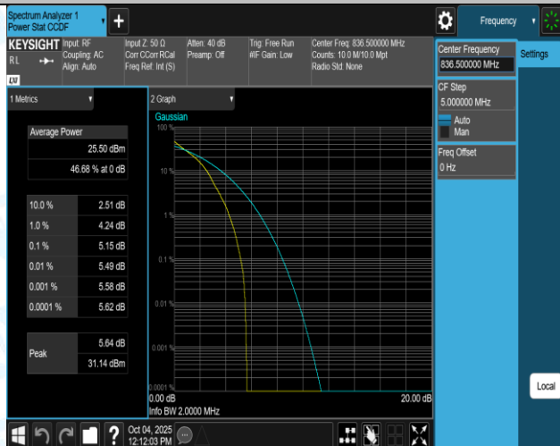
Band26(824-849)-1.4MHz-QPSK-27033-1RB#0-PASS
