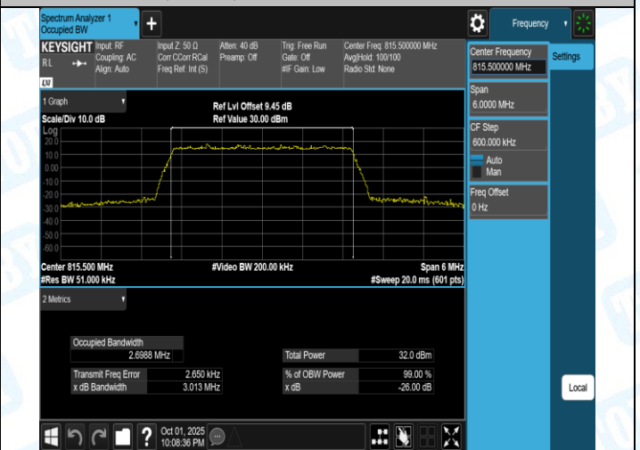
Band26(814-824)-3MHz-16QAM-26775-15RB#0-PASS
