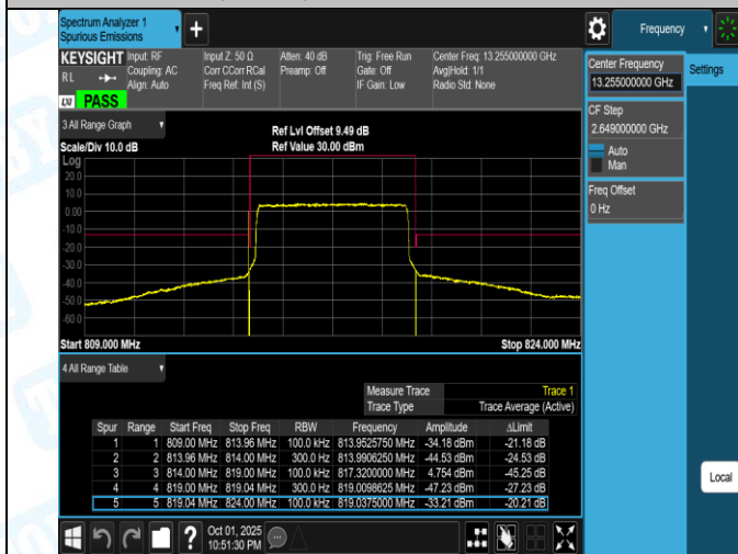
Band26(814-824)-5MHz-QPSK-26765-1RB#24-PASS
