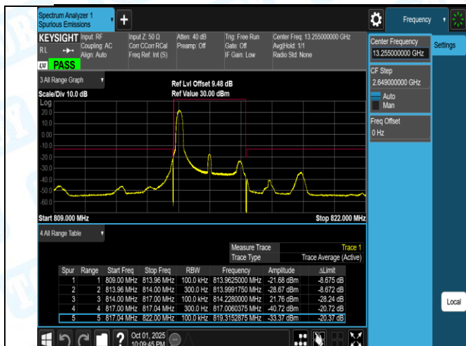
Band26(814-824)-3MHz-QPSK-26705-15RB#0-PASS
