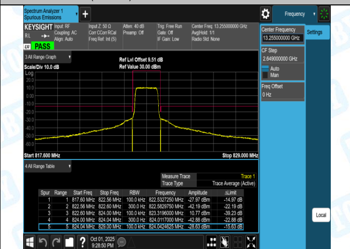
Band26(814-824)-3MHz-QPSK-26705-1RB#14-PASS
