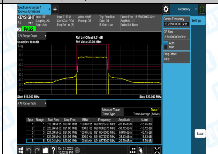
Band26(814-824)-3MHz-16QAM-26705-1RB#14-PASS
