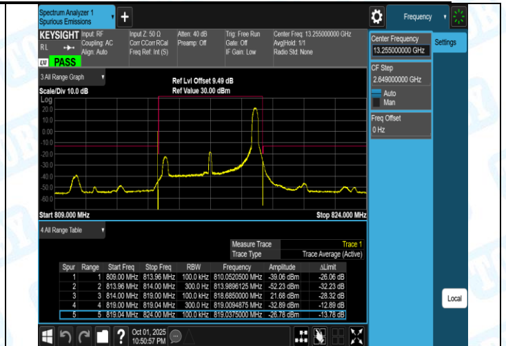
Band26(814-824)-5MHz-QPSK-26765-1RB#0-PASS
