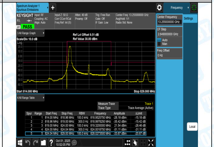
Band26(814-824)-5MHz-QPSK-26765-25RB#0-PASS
