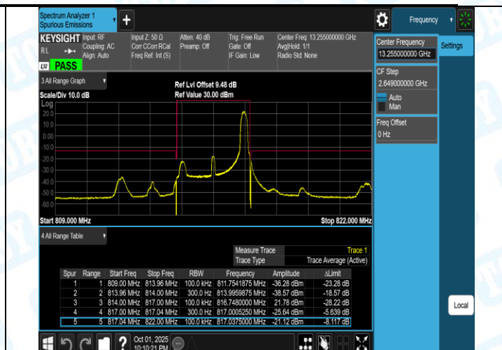
Band26(814-824)-3MHz-QPSK-26775-1RB#0-PASS
