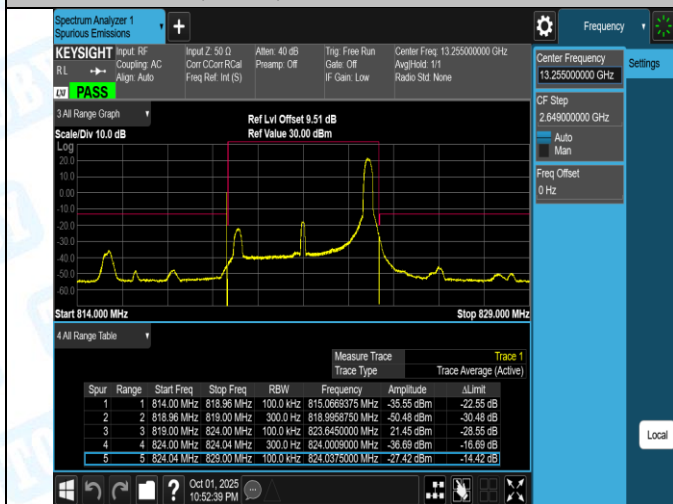
Band26(814-824)-5MHz-16QAM-26715-1RB#0-PASS
