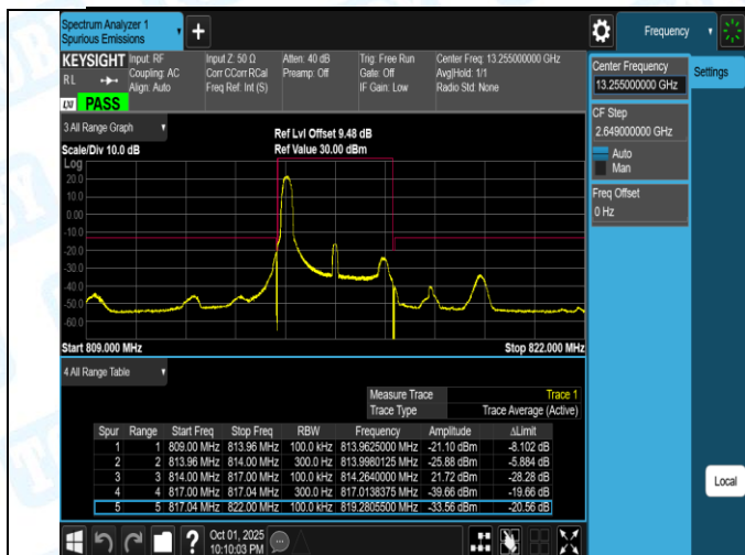
Band26(814-824)-3MHz-16QAM-26705-15RB#0-PASS
