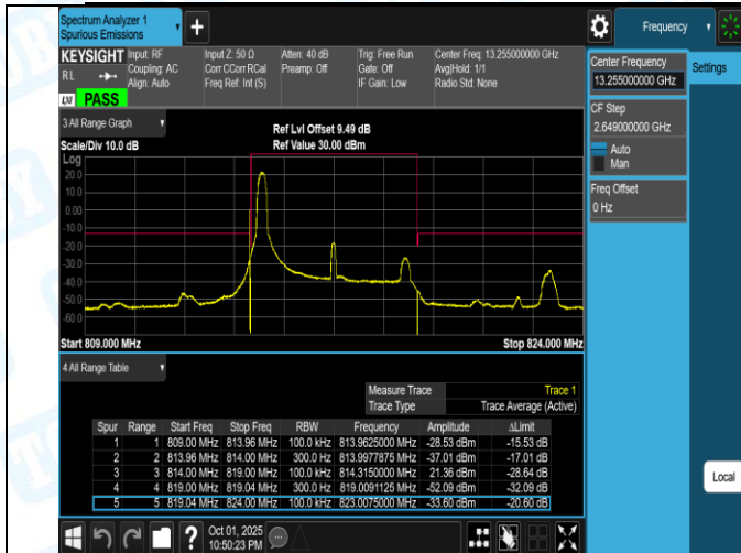
Band26(814-824)-5MHz-QPSK-26715-25RB#0-PASS
