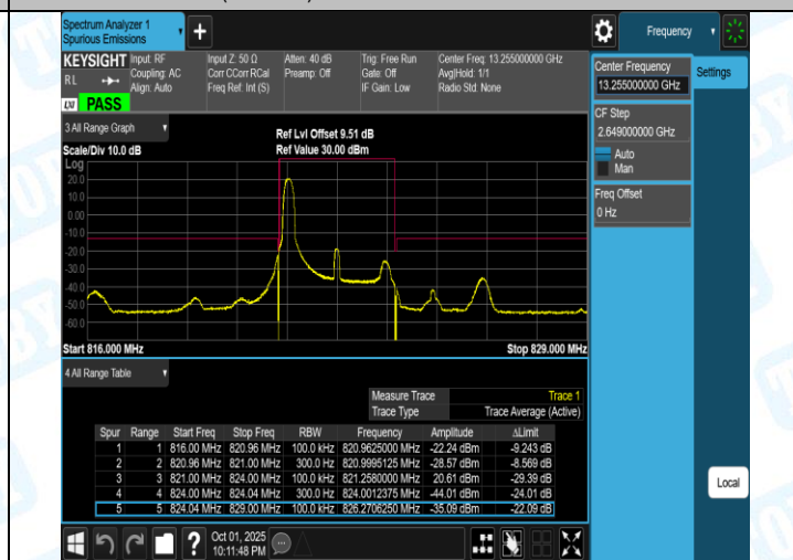
Band26(814-824)-3MHz-16QAM-26775-15RB#0-PASS
