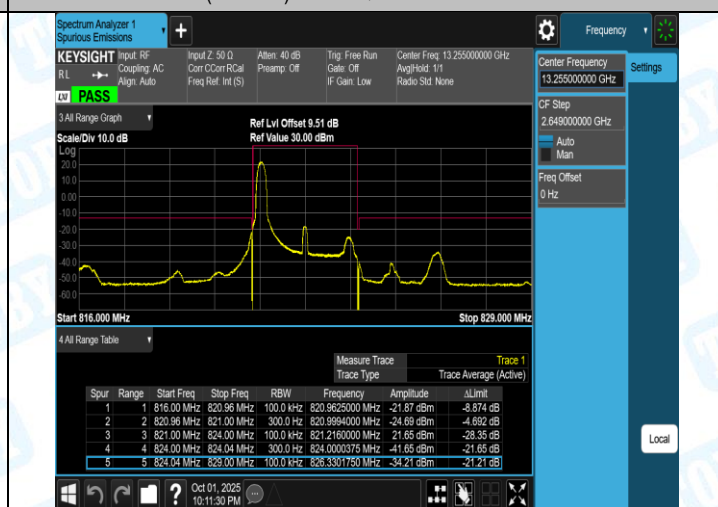
Band26(814-824)-3MHz-QPSK-26775-15RB#0-PASS
