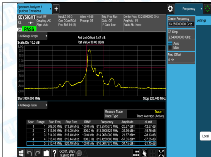
Band26(814-824)-1.4MHz-16QAM-26697-6RB#0-PASS
