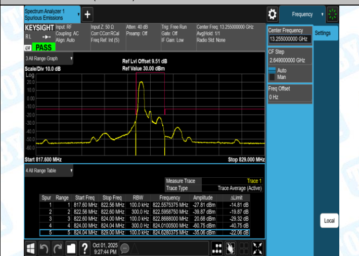
Band26(814-824)-1.4MHz-16QAM-26783-6RB#0-PASS
