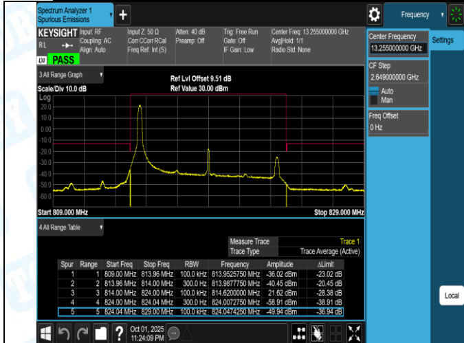
Band26(814-824)-10MHz-QPSK-26740-50RB#0-PASS
