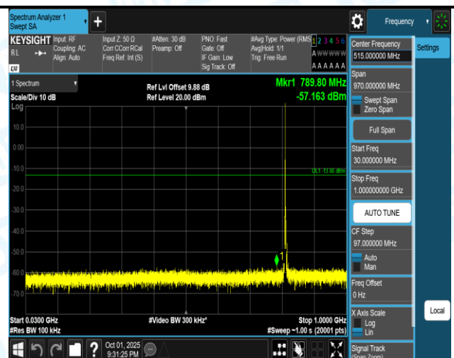
Band26(814-824)-1.4MHz-QPSK-26697-1RB#5-3000-10000-PASS
