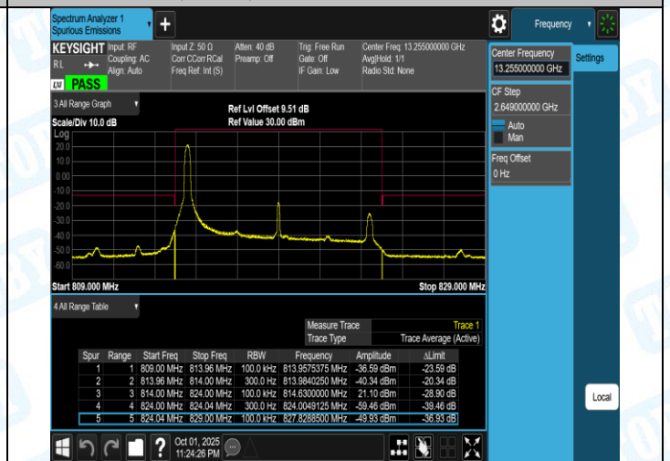
Band26(814-824)-10MHz-16QAM-26740-50RB#0-PASS
