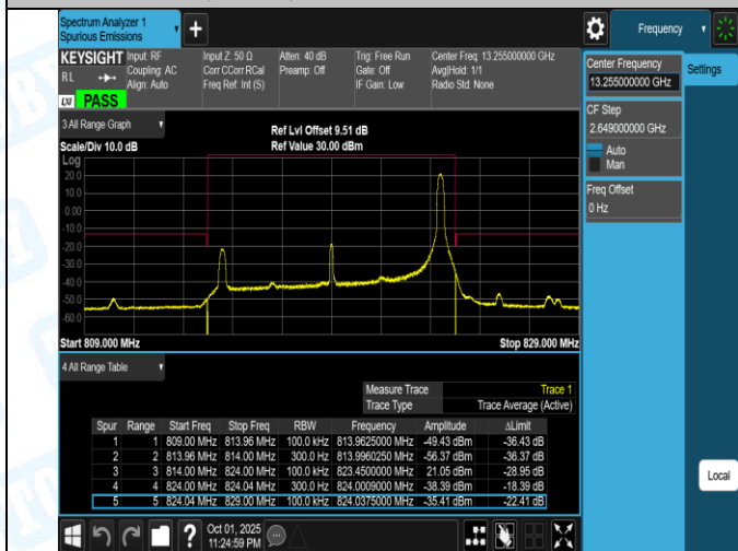
Band26(814-824)-10MHz-16QAM-26740-1RB#49-PASS
