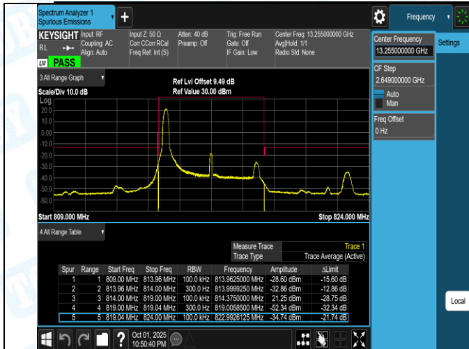
Band26(814-824)-5MHz-16QAM-26715-25RB#0-PASS
