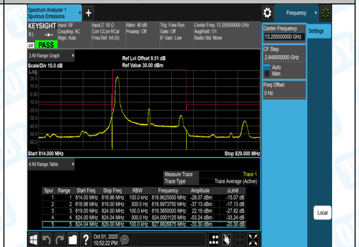
Band26(814-824)-5MHz-16QAM-26765-25RB#0-PASS
