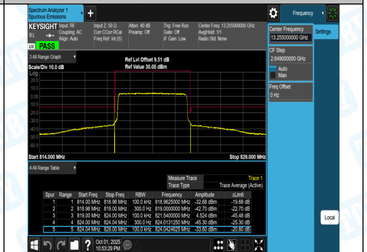
Band26(814-824)-10MHz-QPSK-26740-1RB#49-PASS
