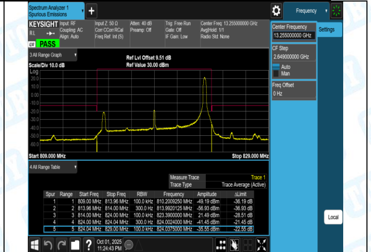
Band26(814-824)-10MHz-16QAM-26740-1RB#0-PASS
