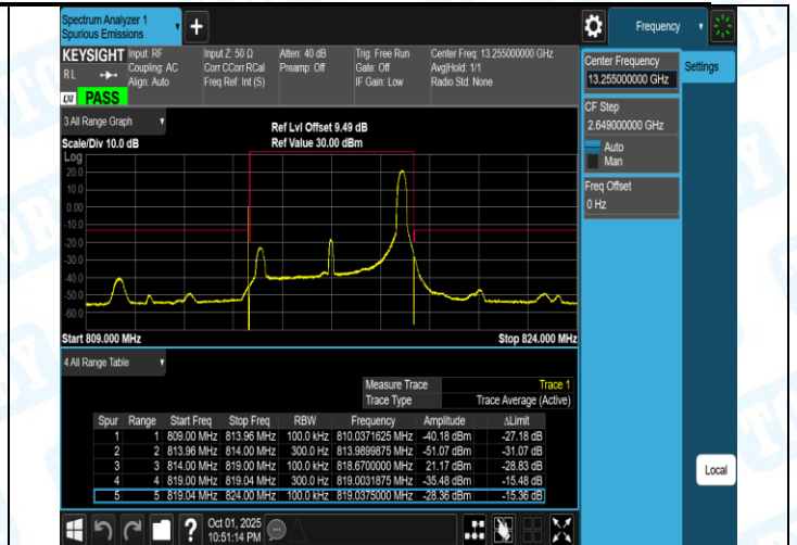
Band26(814-824)-5MHz-16QAM-26765-1RB#0-PASS
