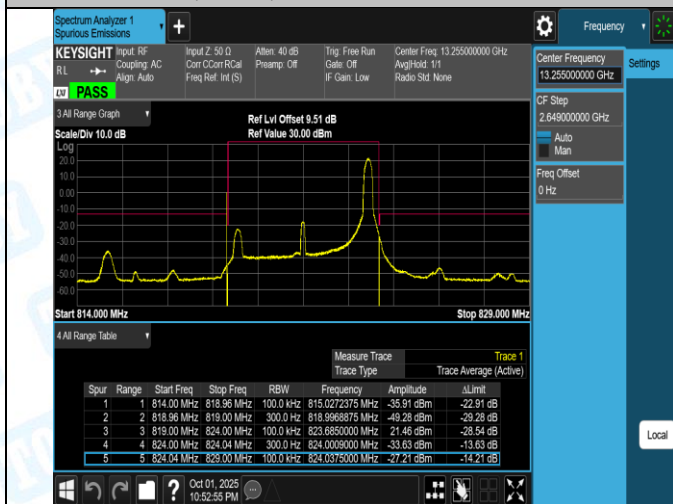
Band26(814-824)-10MHz-QPSK-26740-1RB#0-PASS
