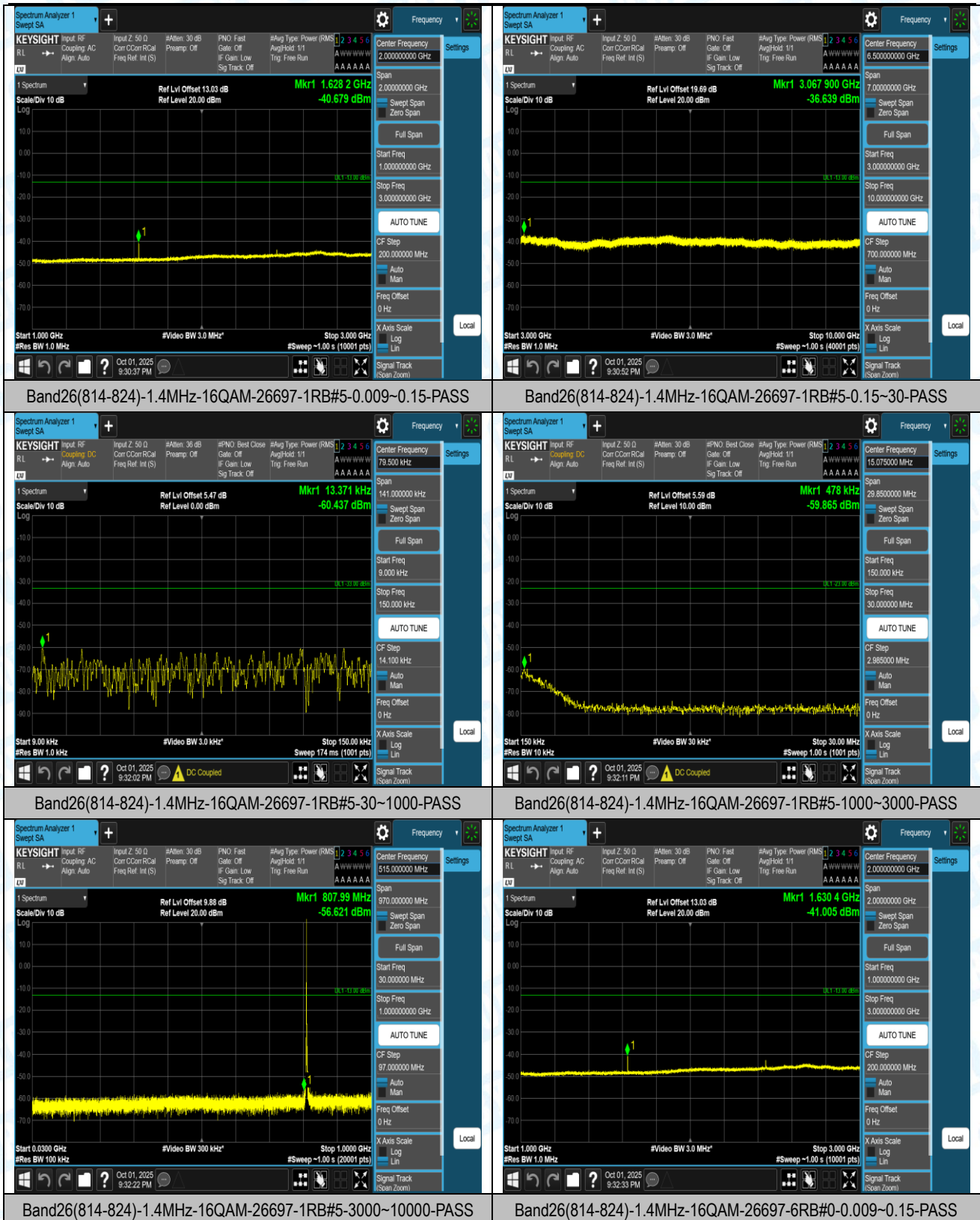
Band26(814-824)-1.4MHz-16QAM-26697-1RB#5-30~1000-PASS
