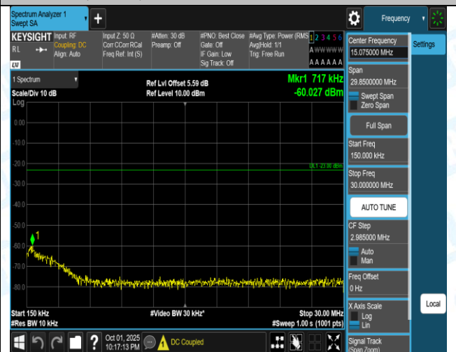
Band26(814-824)-3MHz-QPSK-26705-15RB#0-1000~3000-PASS
