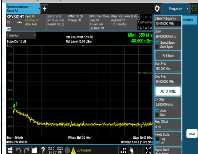
Band26(814-824)-1.4MHz-16QAM-26783-1RB#0-1000-3000-PASS
