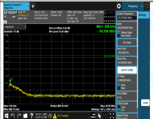
Band26(814-824)-5MHz-QPSK-26715-25RB#0-1000~3000-PASS
