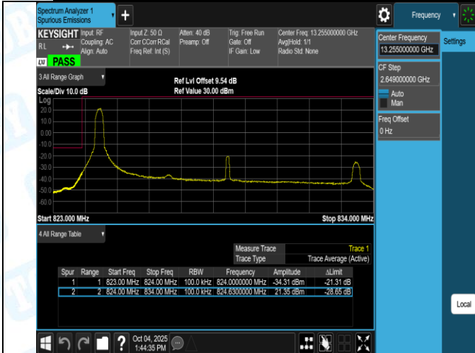
Band26(824-849)-10MHz-16QAM-26840-50RB#0-PASS
