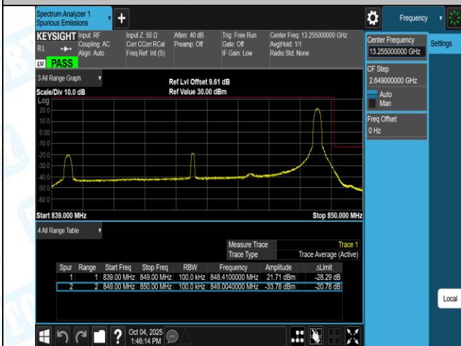
Band26(824-849)-10MHz-16QAM-26840-1RB#0-PASS
