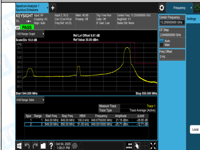
Band26(824-849)-10MHz-QPSK-26840-1RB#0-PASS
