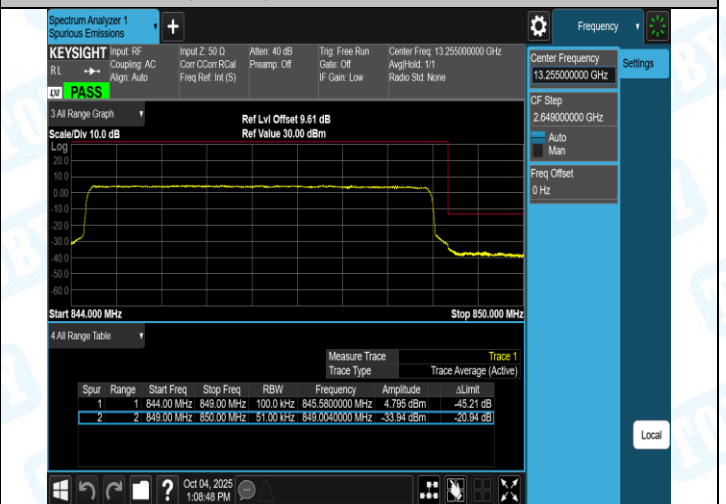
Band26(824-849)-10MHz-QPSK-26840-1RB#49-PASS
