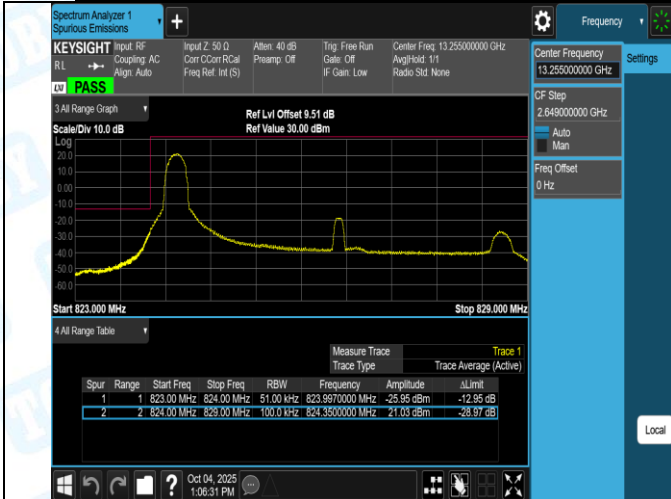
Band26(824-849)-5MHz-16QAM-26815-25RB#0-PASS
