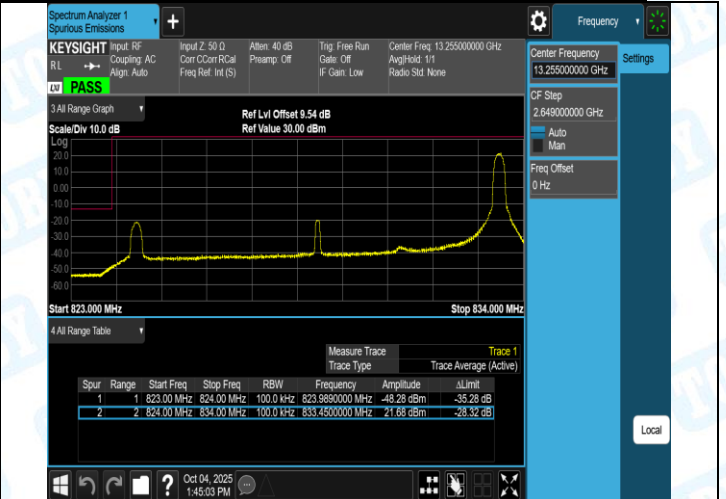
Band26(824-849)-10MHz-16QAM-26990-1RB#0-PASS
