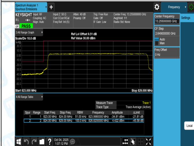
Band26(824-849)-5MHz-QPSK-27015-1RB#24-PASS
