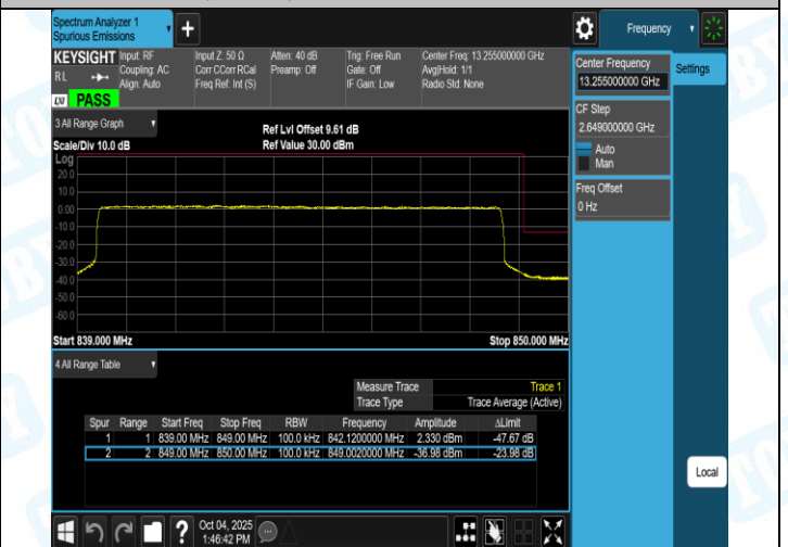
Band26(824-849)-10MHz-16QAM-26840-1RB#49-PASS
