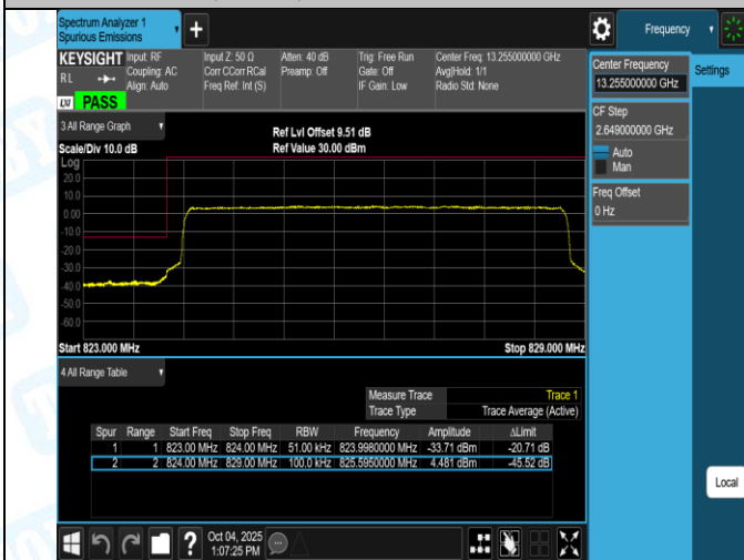
Band26(824-849)-5MHz-16QAM-27015-1RB#24-PASS
