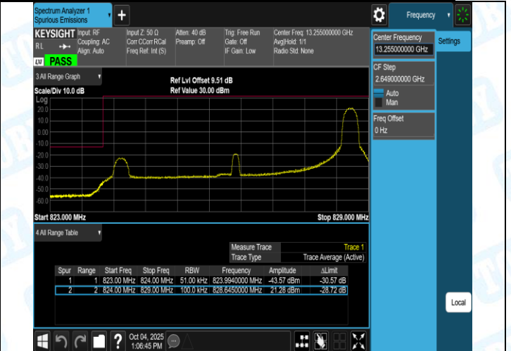
Band26(824-849)-5MHz-QPSK-27015-1RB#0-PASS
