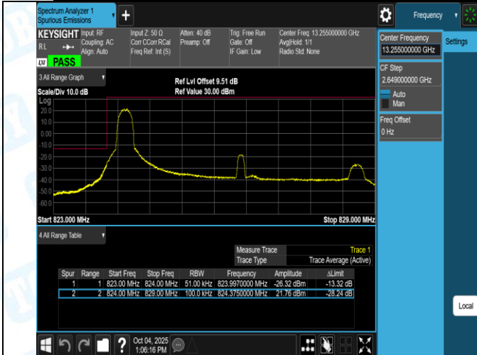
Band26(824-849)-5MHz-QPSK-26815-25RB#0-PASS
