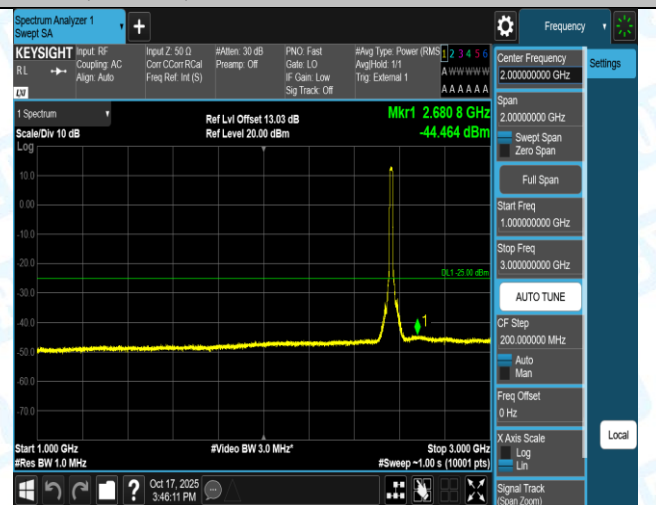
Band41(2555-2655)-15MHz-16QAM-40315-75RB#0-18000~27000-PAS
