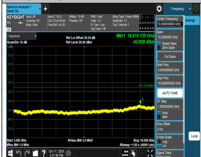
Band41(2555-2655)-15MHz-16QAM-40315-1RB#74-0.009-0.15-PASS
