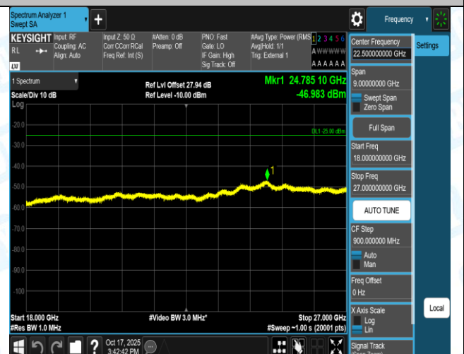
Band41(2555-2655)-15MHz-16QAM-40315-75RB#0-0.15~30-PASS
