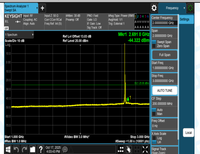
Band41(2555-2655)-15MHz-16QAM-41165-1RB#0-18000~27000-PASS
